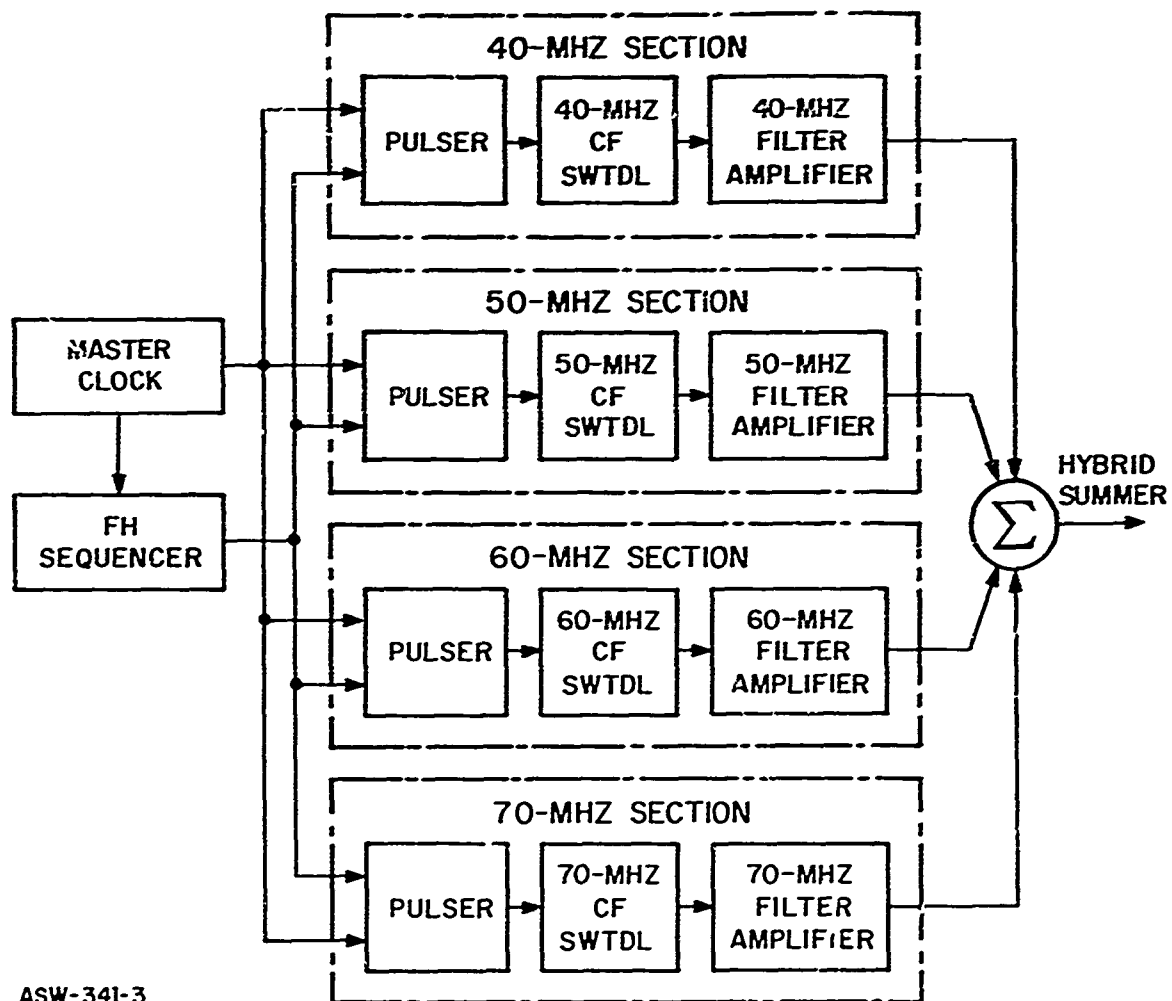
Figure 3. Surface Wave Device FH/PN Synthesizer
