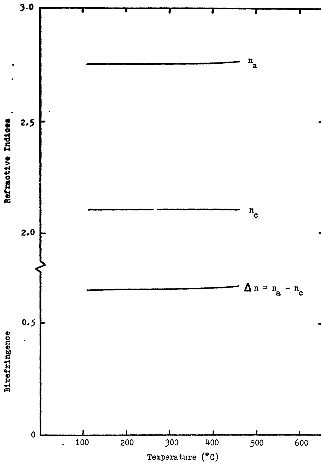
Fig. 13. Refractive Indices and Birefringence vs. Temperature for Full Ionic Tetragonal PbTiO 3 (Theoretical)
