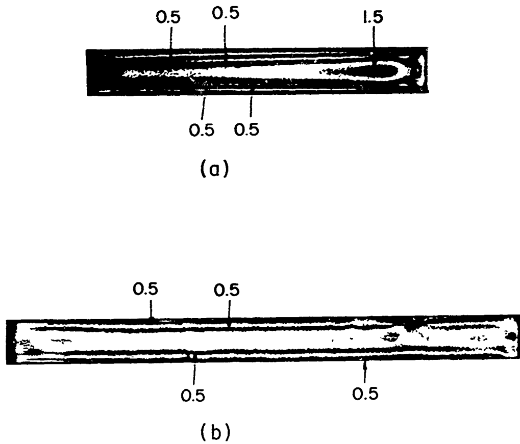
Fig. 16 Fringe Pattern at No Load (a) 2 in. Overlap Specimen (b) 3 in. Overlap Specimen
