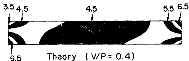
Fig. 25 Comparison of Experimental and Theoretical Fringe Patterns ( a = 2 in., V/P = 0.0, 0.4 )
