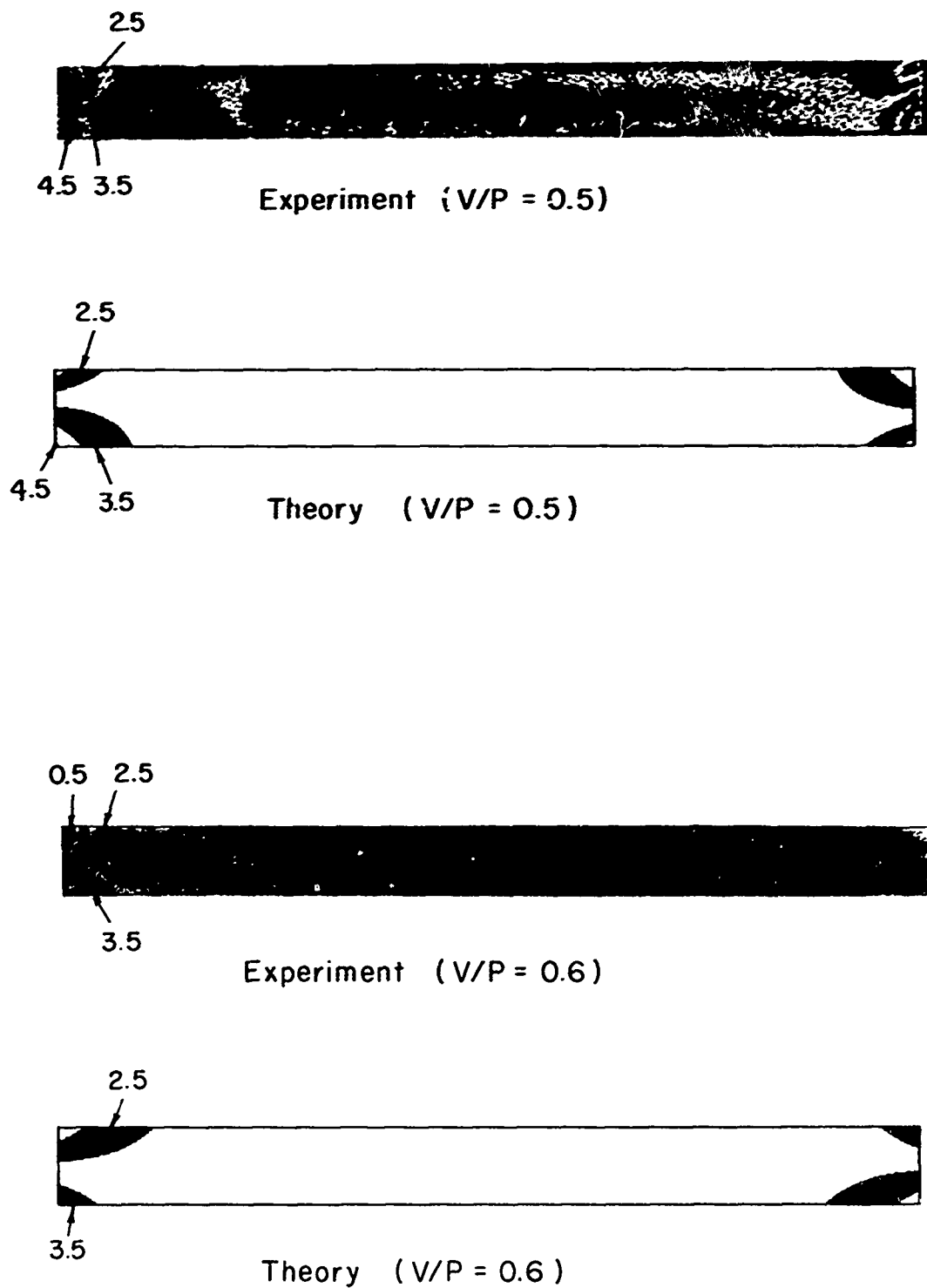
Fig. 29 Comparison of Experimental and Theoretical Fringe Patterns ( a = 3 in., V/P = 0.5, 0.6 )
