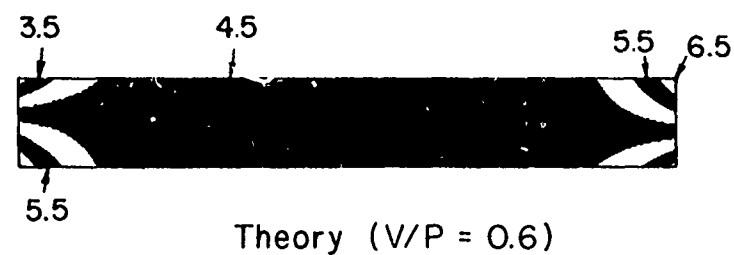
Fig. 26 Comparison of Experimental and Theoretical Fringe Patterns ( a = 2 in., V/P = 0.5, 0.6 )
