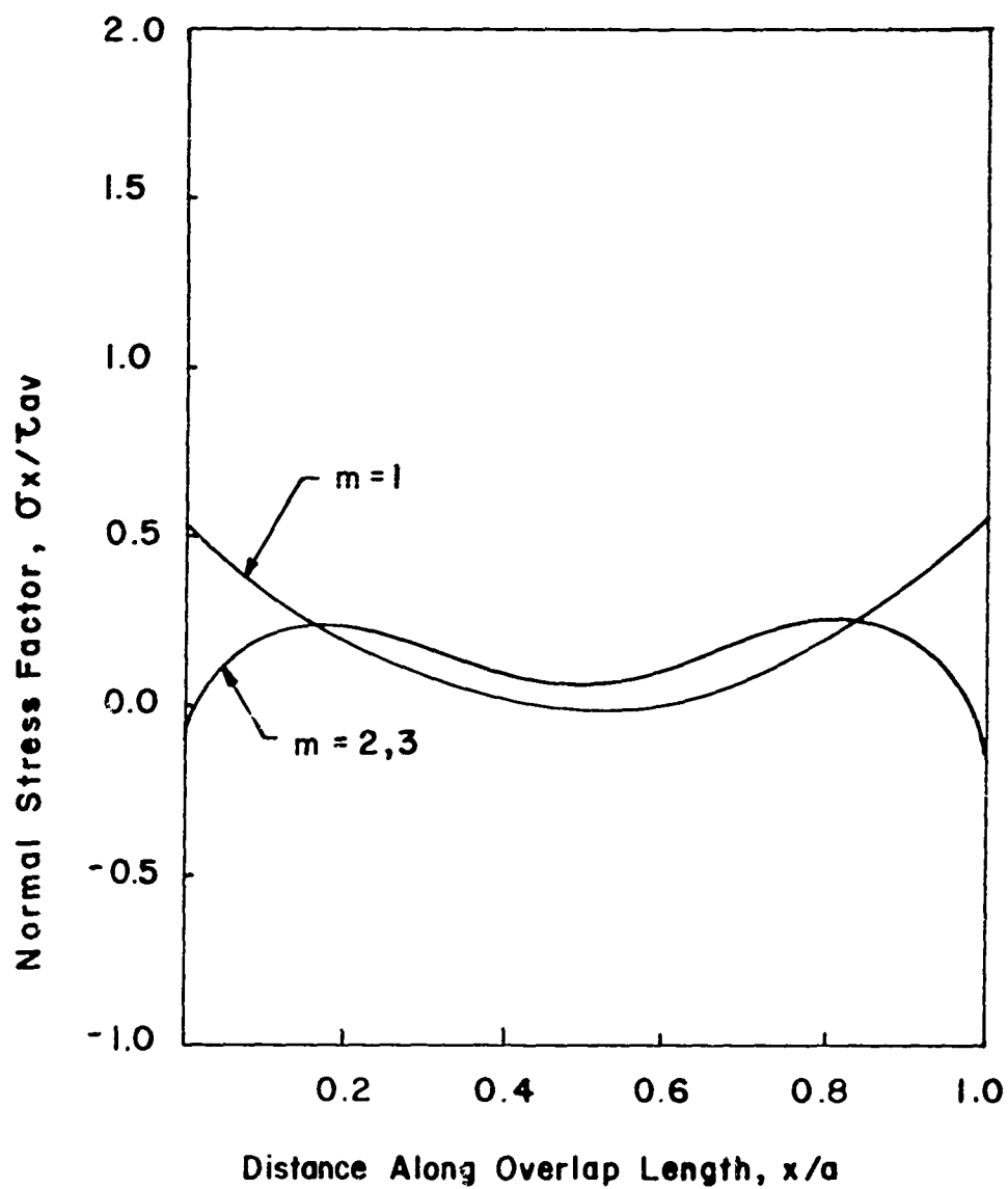
Fig. 14 Theoretical Distribution of \sigma_x at Mid-plane for Different Values of m ( E_1/E = 20 , t_1/t = 4 , t/a = .5 , V = 0 , n = 1 )
