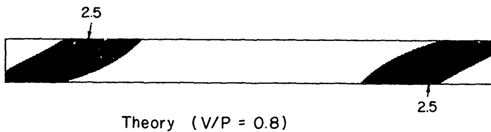
Fig. 30 Comparison of Experimental and Theoretical Fringe Patterns ( a = 3\text{in.} , V/P = 0.7, 0.8)
