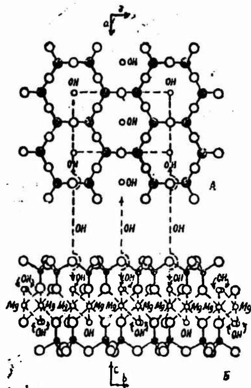
Fig. 1. The crystal structure of chrysotile-asbestos (according to A. V. Fedoseev, L. F. Grigor'yeva, T. A. Makarova, 1966).
