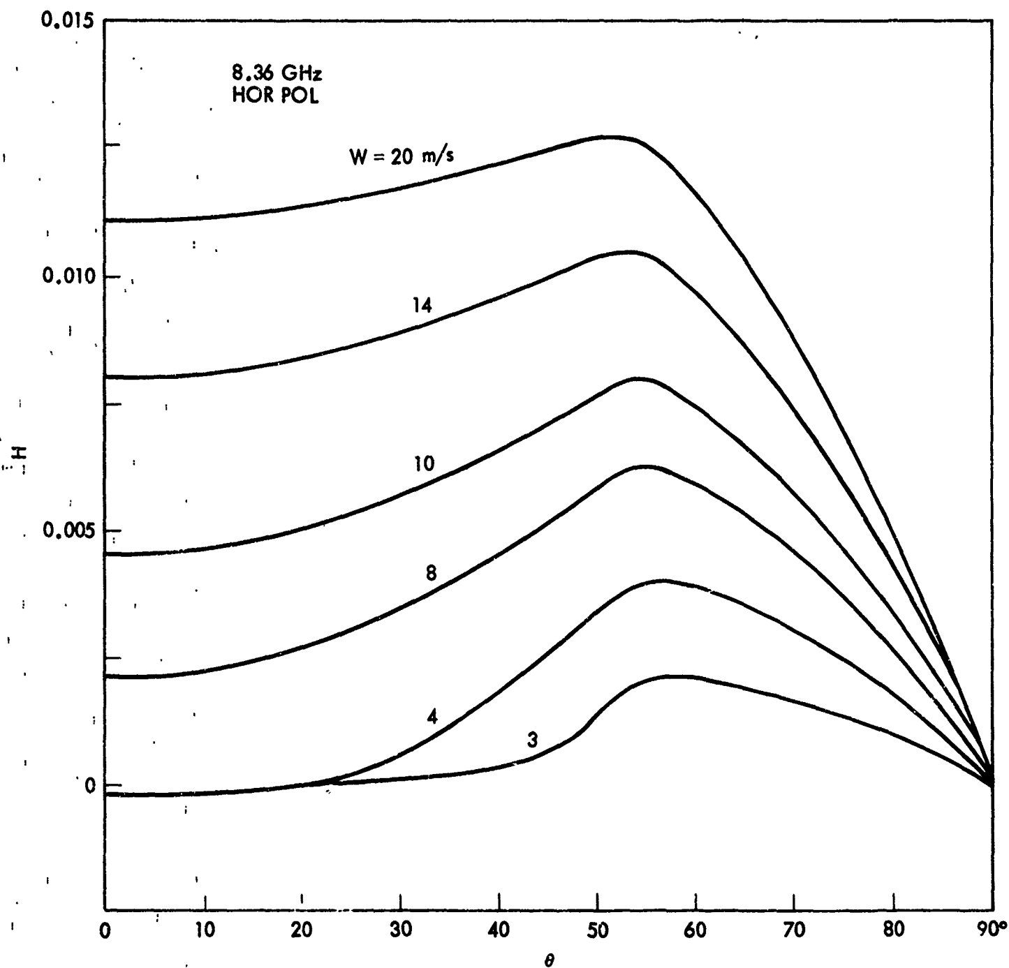
Fig. 3. Roughness dependence of the emissivity of a slightly rough surface. \nu = 8.36 GHz, horizontal polarization.
