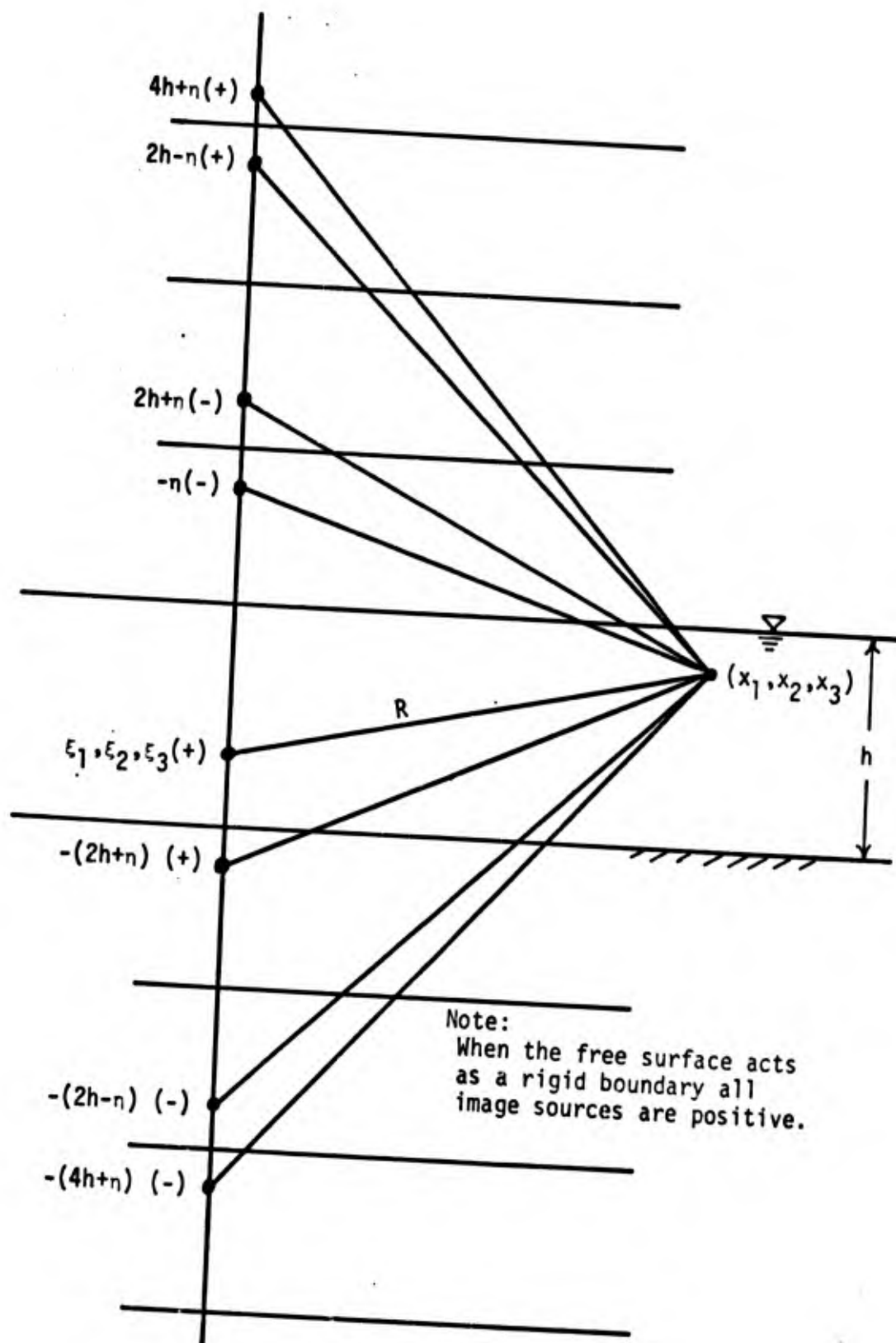
Fig. 2 - Image source layout.
