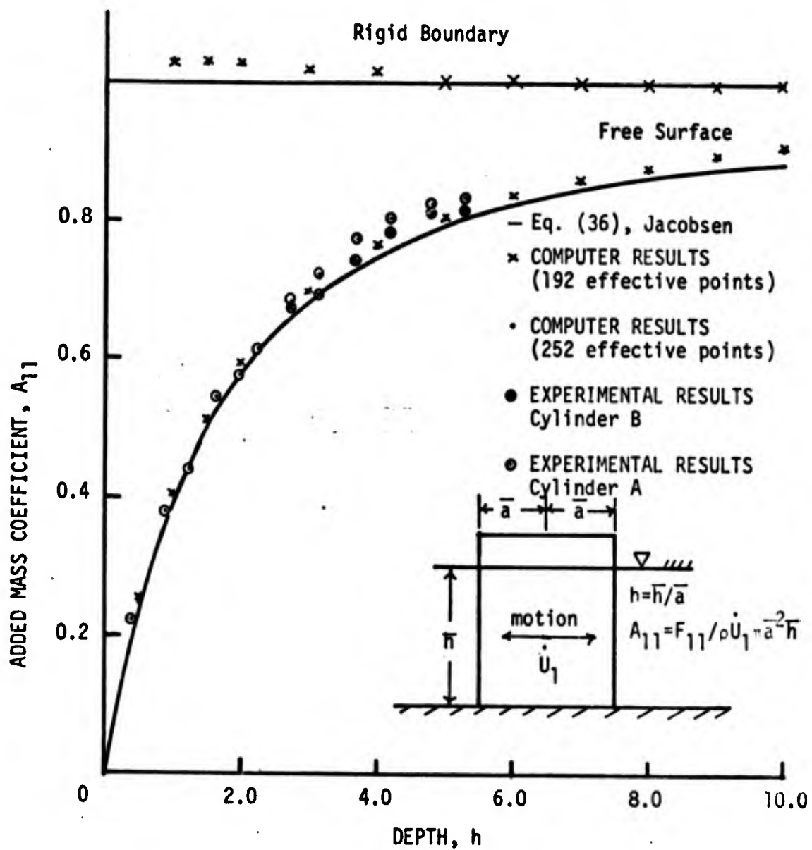
Fig. 9 - Added mass coefficient for a vertical circular cylinder.
