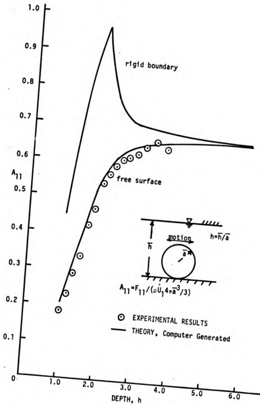
Fig. 17 - Added mass coefficient for a ball mounted sphere.
