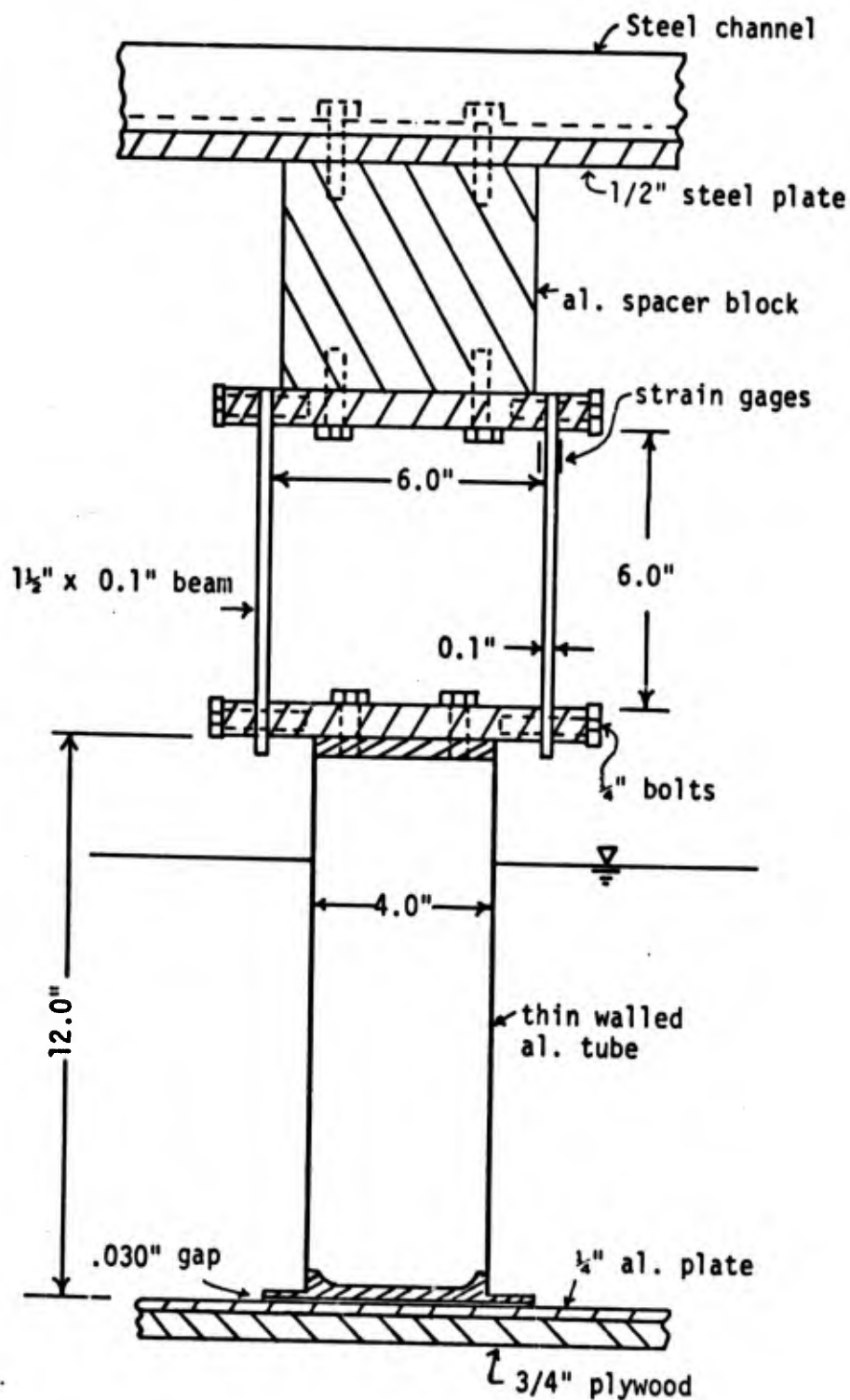
Fig. 3 - Experimental equipment.
