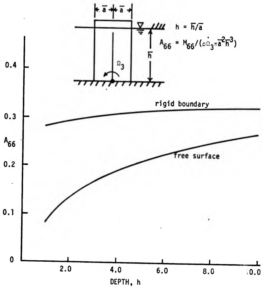
Fig. 11 - Added moment of inertia coefficient for a vertical circular cylinder.
