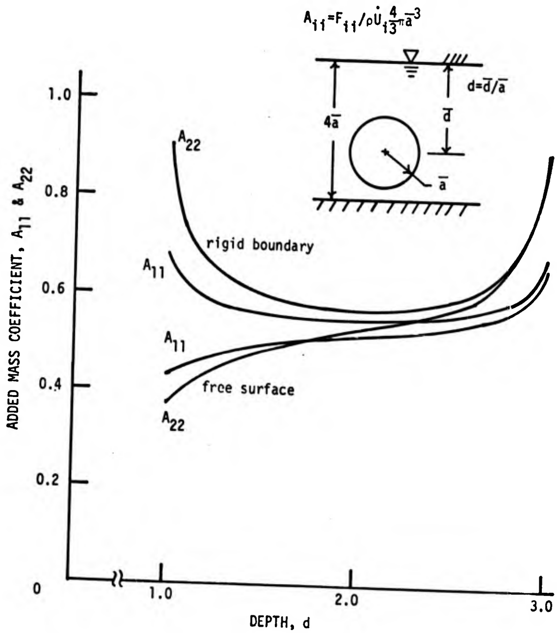
Fig. 16 - Added mass coefficient for a sphere for h = 4.0 .
