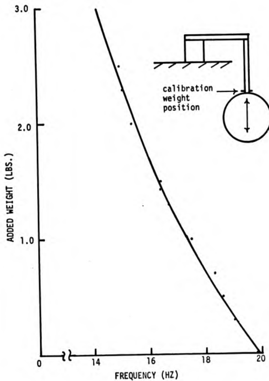
Fig. 13 - Calibration curve (Sphere - Vertical Motion)
