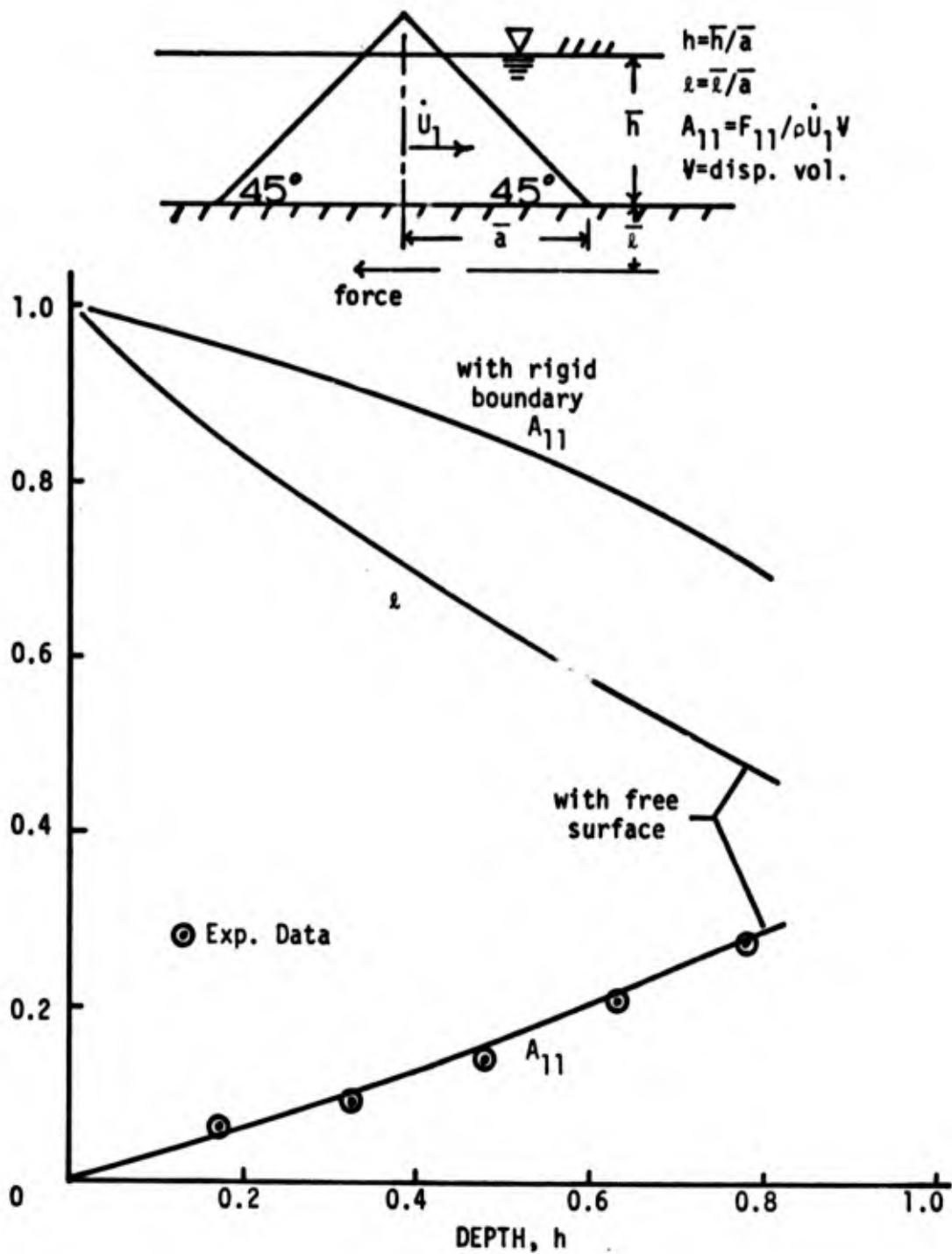
Fig. 19 - Added mass coefficient and line of action of horizontal force for a cone.
