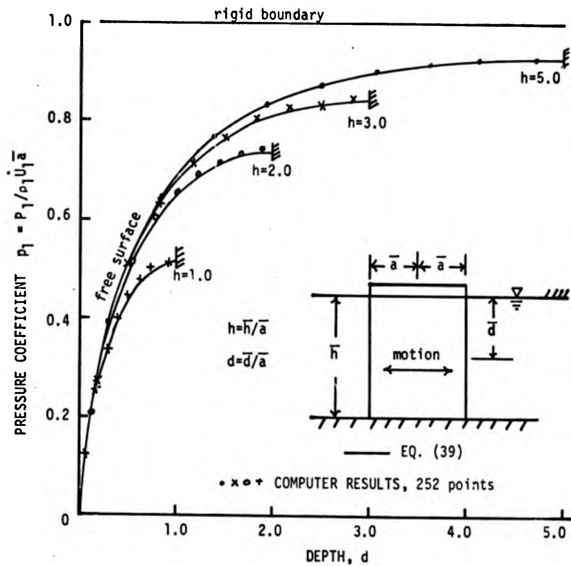
Fig. 12 - Pressure amplitude on meridian of a vertical cylinder.
