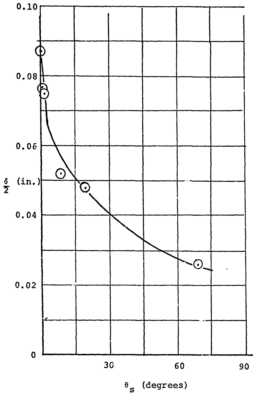
FIGURE 20. JET DEFLECTION ANGLE SENSITIVITY TO CONTROL TUBE MOVEMENT
