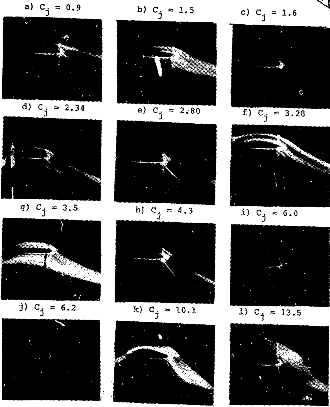
FIGURE 26. PHOTOGRAPHS OF THE SMOKE FLOW ( \delta = .2'' and \theta = 84^\circ )
