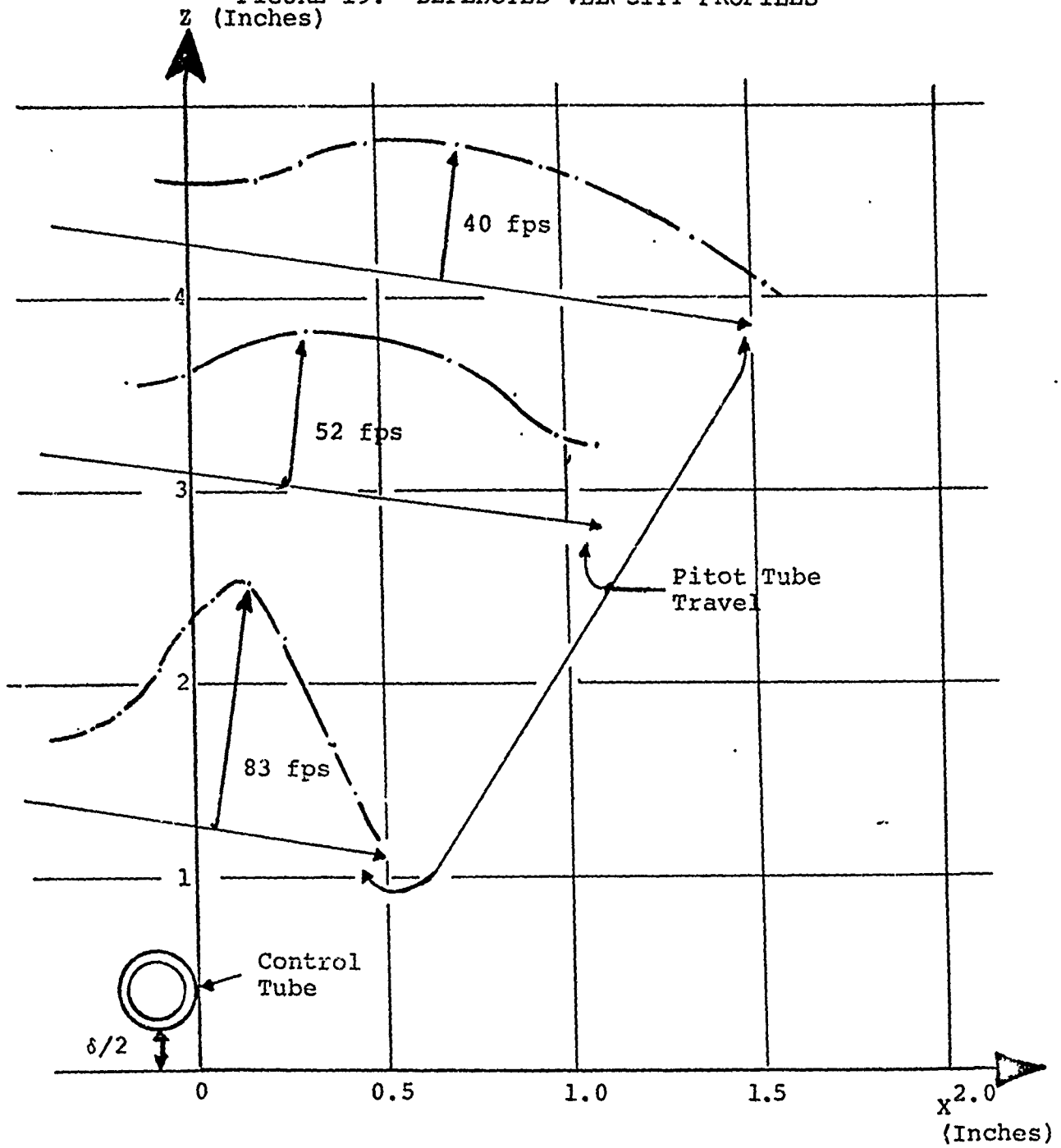
FIGURE 19. DEFLECTED VELOCITY PROFILES
