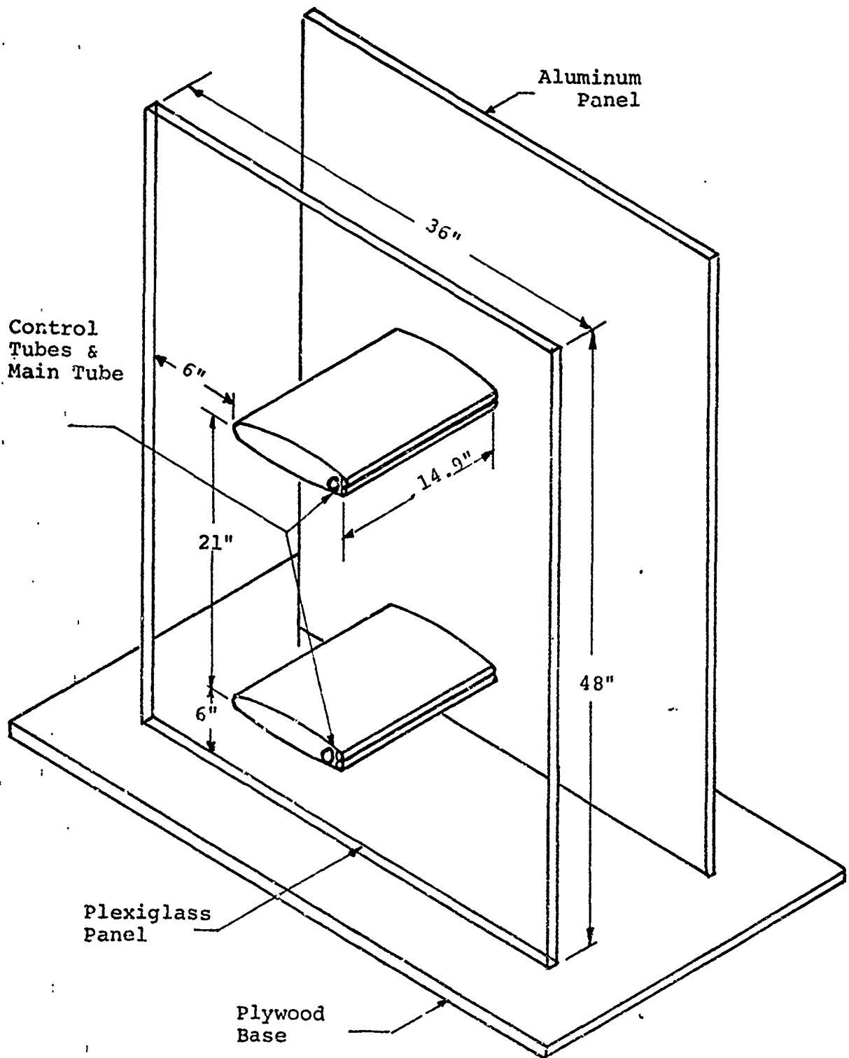
FIGURE 9. SCHEMATIC OF THE MODEL
