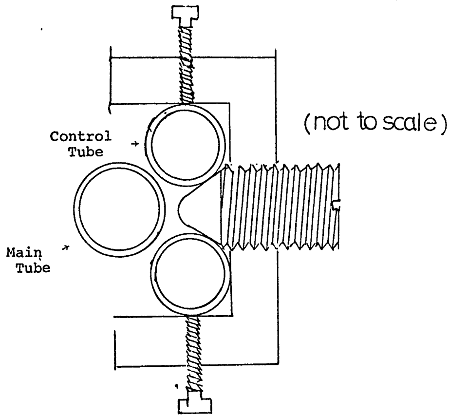
FIGURE 11. CONTROL TUBE SET-SCREW DEVICE
