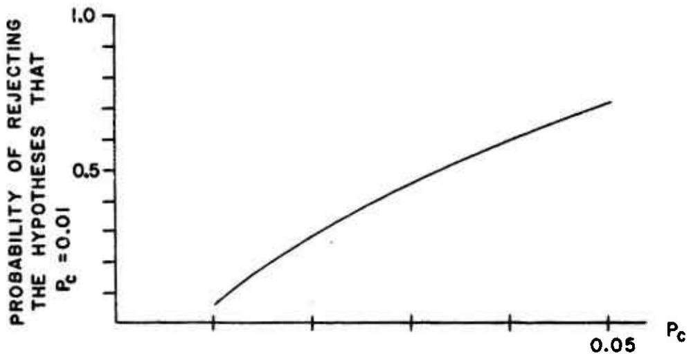
The power of the one tailed test for P_c=0.01 with a confidence level of 0.95, based on 50 runs.
