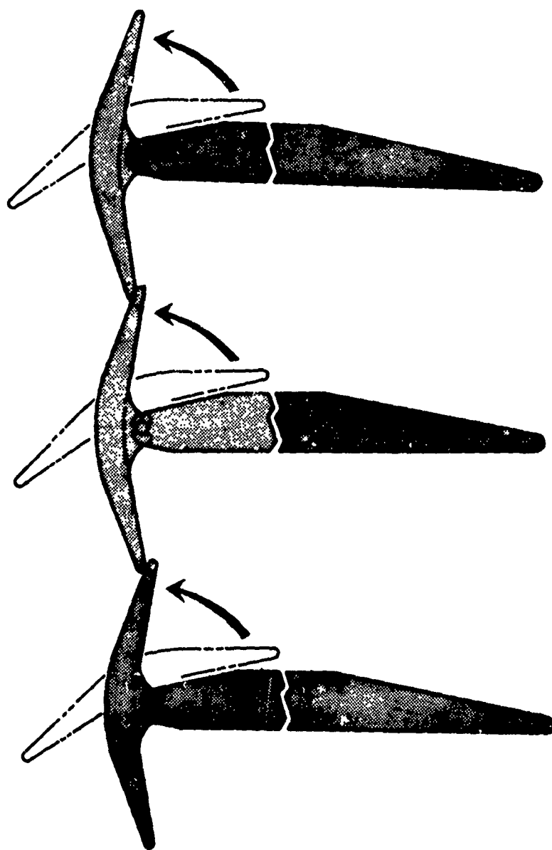
Figure 1.4. --Louver operation.
