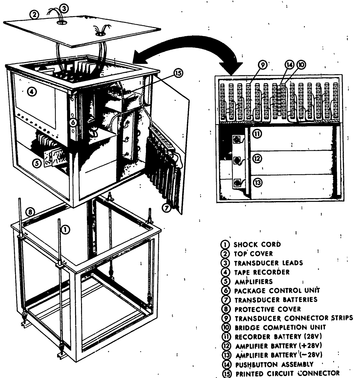
Figure 2.4. --Recording package.
