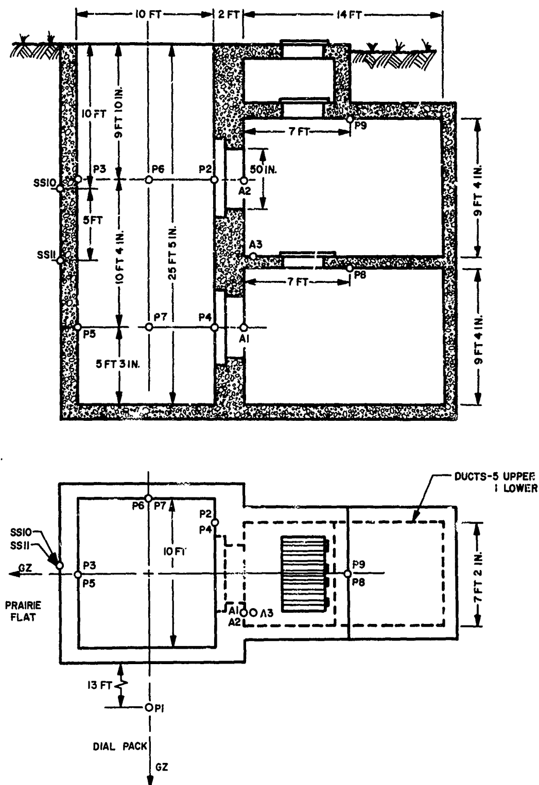
Figure 2.1. --Transducer locations.
