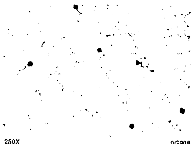
FIGURE III-8. AS-POLISHED MICROSTRUCTURE OF ARC-CAST A-55 TITANIUM WITH 1.2 w/o YTTRIUM METAL. THE PRIOR BETA-PHASE GRAIN BOUNDARIES ARE OUTLINED BY PRECIPITATES (PROBABLY YTTRIUM METAL), WHILE RELATIVELY LARGE PARTICLES OF Y_2O_3 ARE RANDOMLY DISTRIBUTED.
