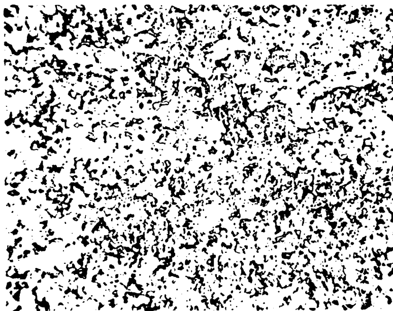
(b) Alloy 2. Ti-3.4Al-8.7Ga-1Mo-1Cb-5Zr-0.5Si, 1000X
