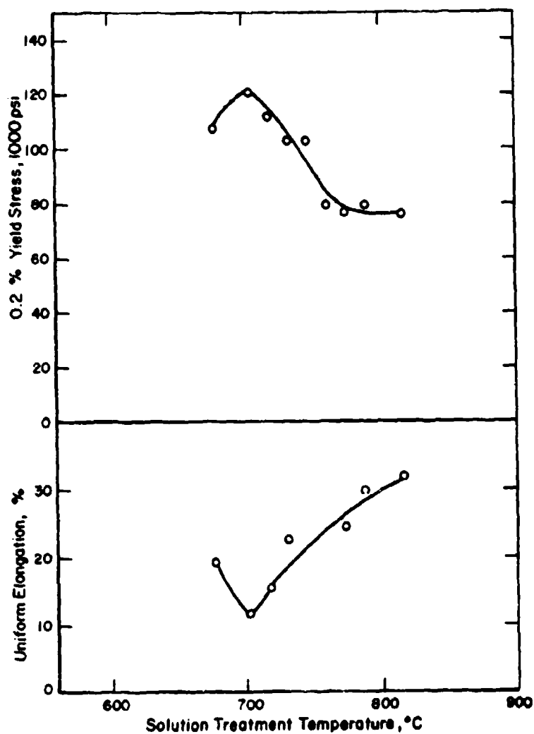
FIGURE VI-2. Yield strength and uniform elongation of Ti-4.5Sn-6Zr-11.5Mo ( \beta -III) as a function of solution treatment temperature. All specimens were quenched and tested at room temperature.
