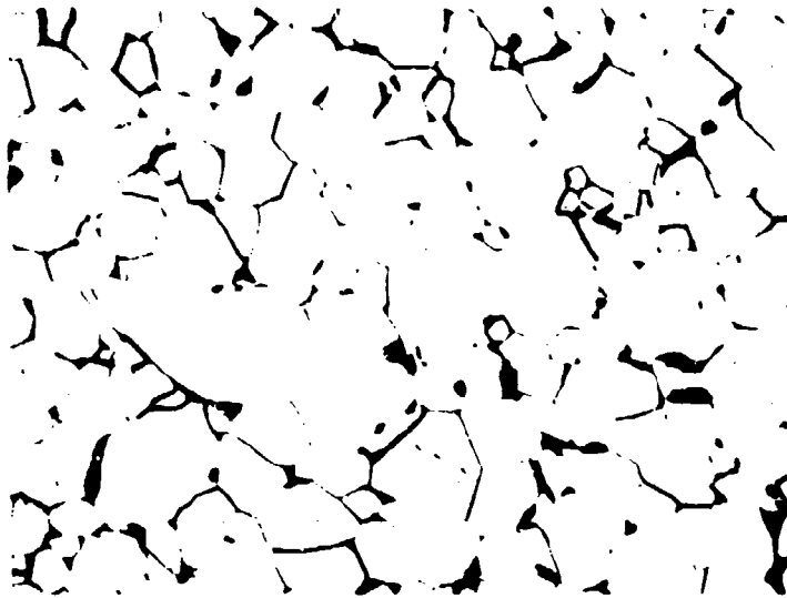
(a) Ti-50Al, annealed 7 hours at 816°C, W.Q., 250X.
