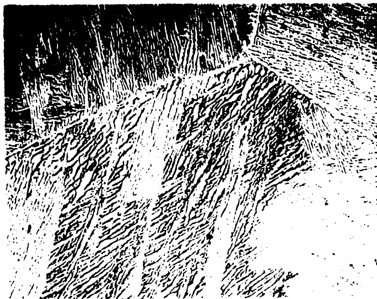
(c) Alloy 3. Ti-3.4Al-8.7Ga-1Mo-0.5Si, 100X
