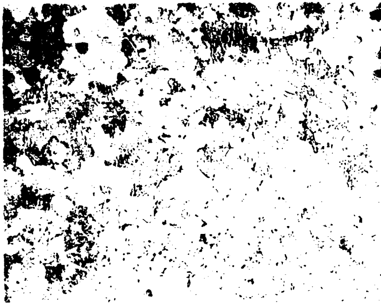
(a) Alloy 1. Ti-3.4Al-8.7Ga-0.5Si, 250X
