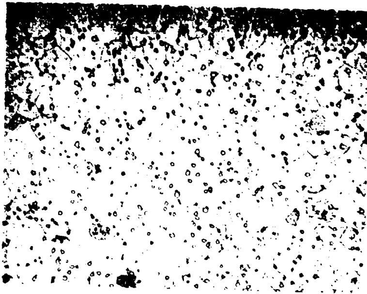
(a) Alloy 2. Ti-3.4Al-8.7Ga-1Mo-1Cb-5Zr-0.5Si, 1000X
