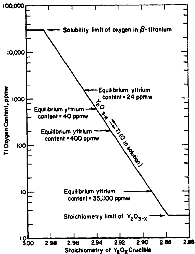
FIGURE III-1. Equilibrium Oxygen Distribution at 1687°C.
