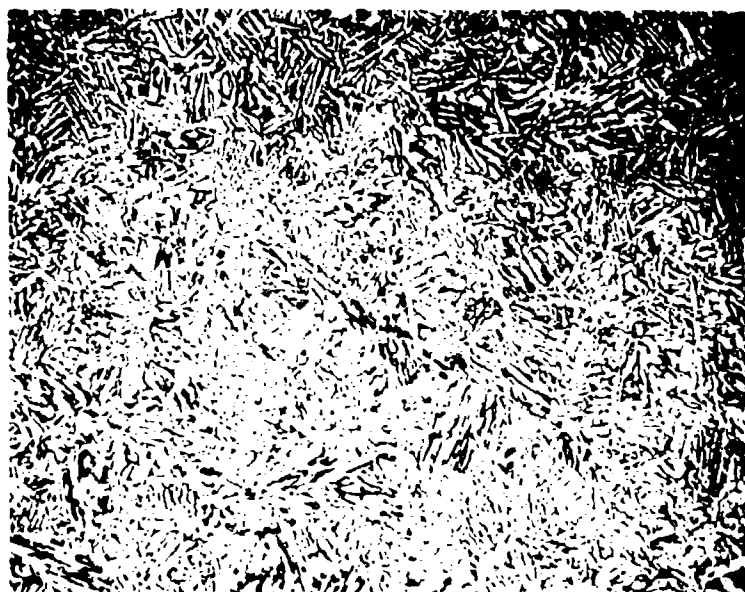
(b) Alloy 2. Ti-3.4Al-8.7Ga-1Mo-1Cb-5Zr-0.5Si, 100X
