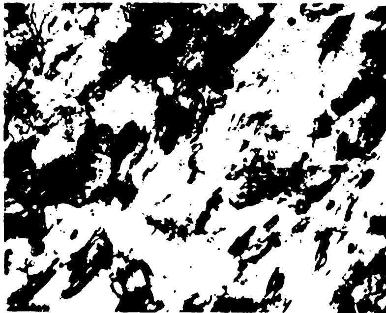
FIGURE A-3. Transmission electron micrograph of as-extruded PH-DS 2024 showing a high density of dispersed \text{Al}_2\text{O}_3 particles, 40,000X.
