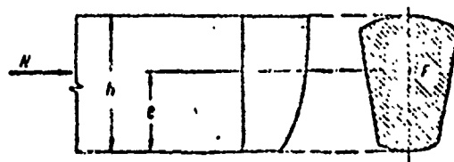
Fig. 6. Diagram of the distribution of forces and diagram of the stresses in a transverse cross section of an eccentrically compressed concrete element with a small eccentricity.
