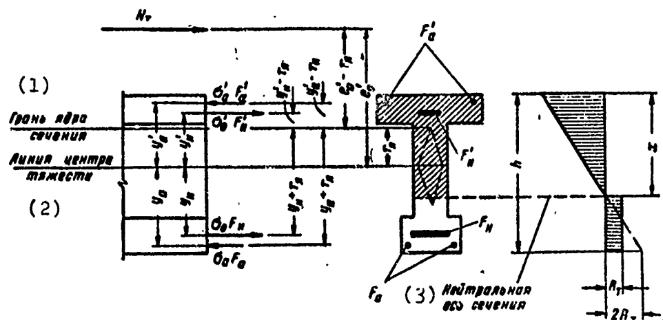
Fig. 33. Diagram of the distribution of forces and stress diagram in the transverse section of an eccentrically compressed pre-stressed reinforced-concrete element in rating the zone tensile-stressed by an external load for crack formation, in which stressed and unstressed reinforcement is contained. KEY: (1) Section core face; (2) Center of gravity line; (3) Neutral axis of the section.
