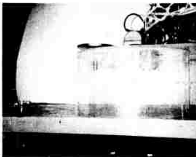
Figure 3. Bell jar injection system for introducing antibiotics and formalin.
