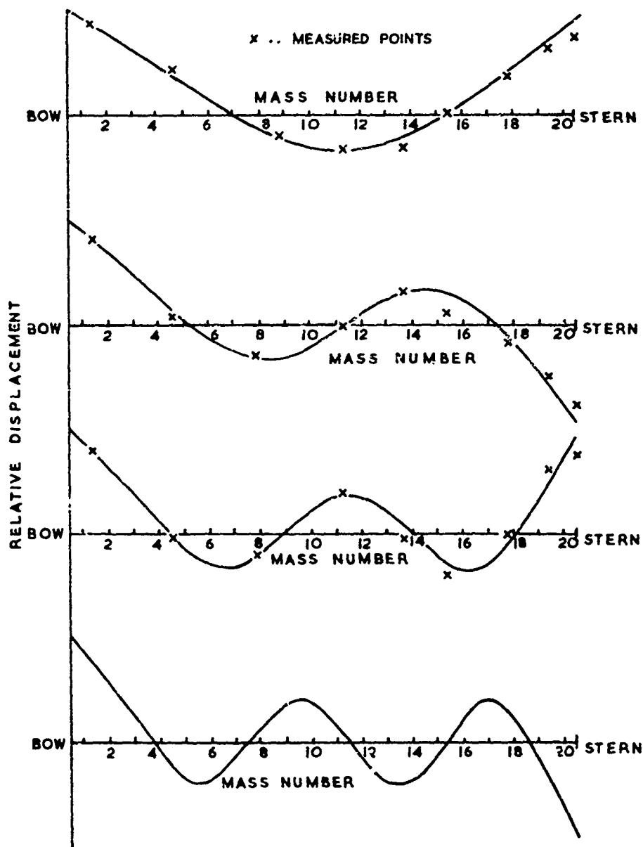
CALCULATED AND MEASURED MODE SHAPES FOR A DESTROYER
