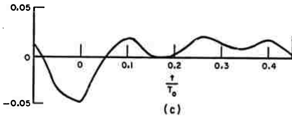
Fig. 11. Ramp response waveforms of a conducting disk: (a) free space, (b) underground - n\omega_0 harmonics, (c) underground - n^2\omega_0 harmonics.
