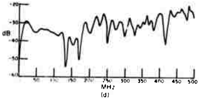
Fig. 20. Orthogonal mode response 2" dielectric pipe. (a) difference waveform (b) gated difference waveform (c) normalized amplitude spectrum (d) normalized amplitude spectrum with incident pulse removed.
