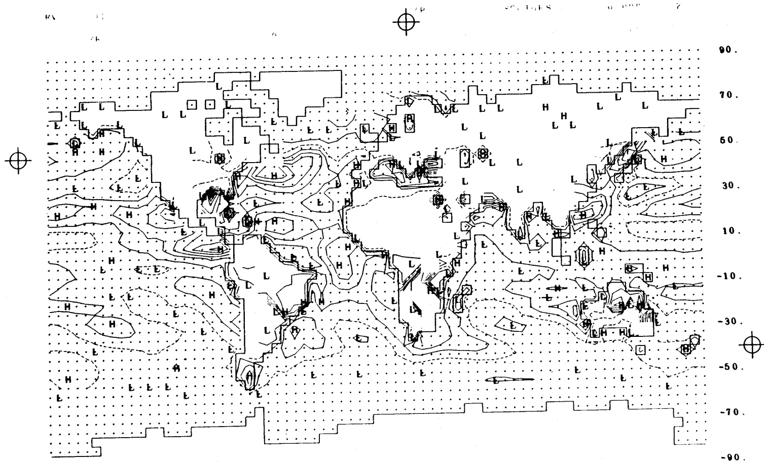
Fig. 41 -- The difference between the simulated and observed evaporation rate (Fig. 40a minus Fig. 40b). The isoline interval is 1 \text{ mm day}^{-1} with the zero isoline dashed.
