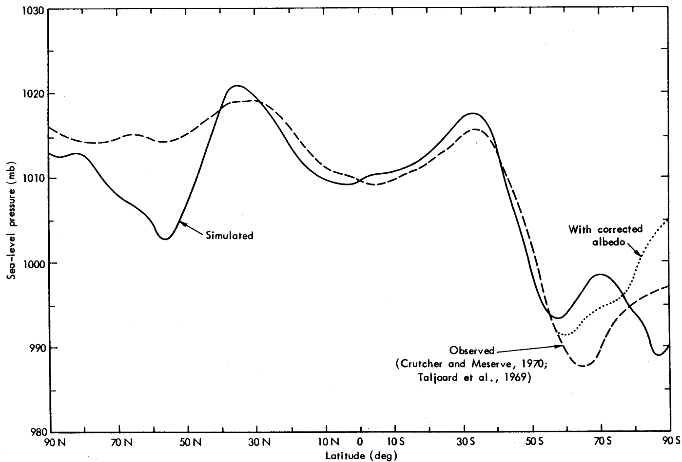
Fig. 6 -- The zonal average sea-level pressure as simulated (full line) and as observed (dashed line), based on the data of Fig. 4. The dotted curve at high southern latitudes in this and later figures is the simulation with a corrected albedo for snow and ice, as obtained from a subsequent January integration (Mintz, private communication); see footnote, p. 8.
