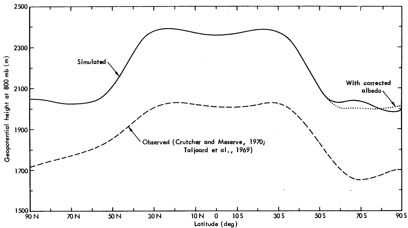
Fig. 9 -- The zonal average 800-mb geopotential height as simulated (full line) and as observed (dashed line), based on the data of Fig. 7. See Fig. 6 for dotted-line identification.
