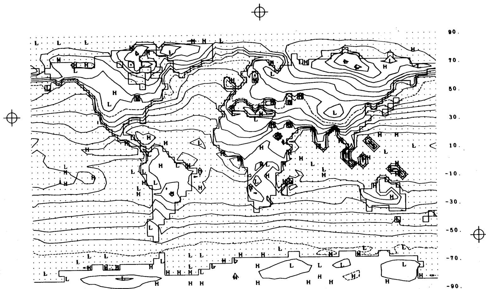
Fig. 13a -- The simulated surface air temperature for January, with isolines at 5 deg C intervals and the 0-deg C isotherm dashed
