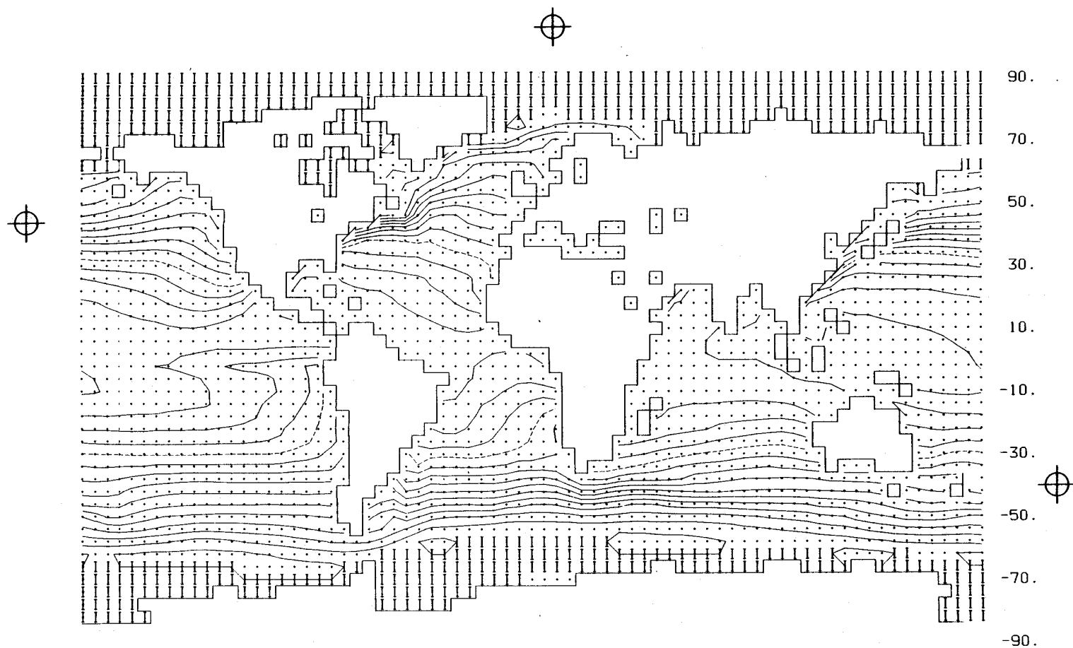
Fig. 3 -- The sea-surface temperature used in the January control experiment, with isolines every 2 deg C and the 20-deg C isotherm dashed. The overprinted symbol I denotes the locations of sea ice. From Gates et al. (1971); see also Fig. 2.
