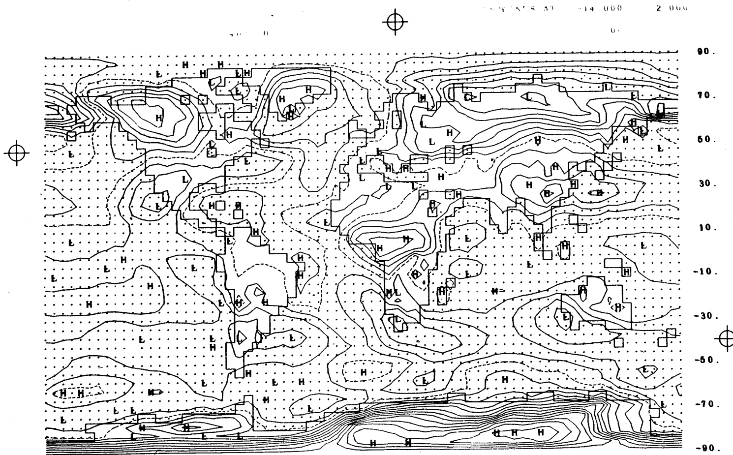
Fig. 17 -- The difference between the simulated and observed 800-mb temperature (Fig. 16a minus Fig. 16b). The isoline interval is 2 deg C with the 0-deg C line dashed.
