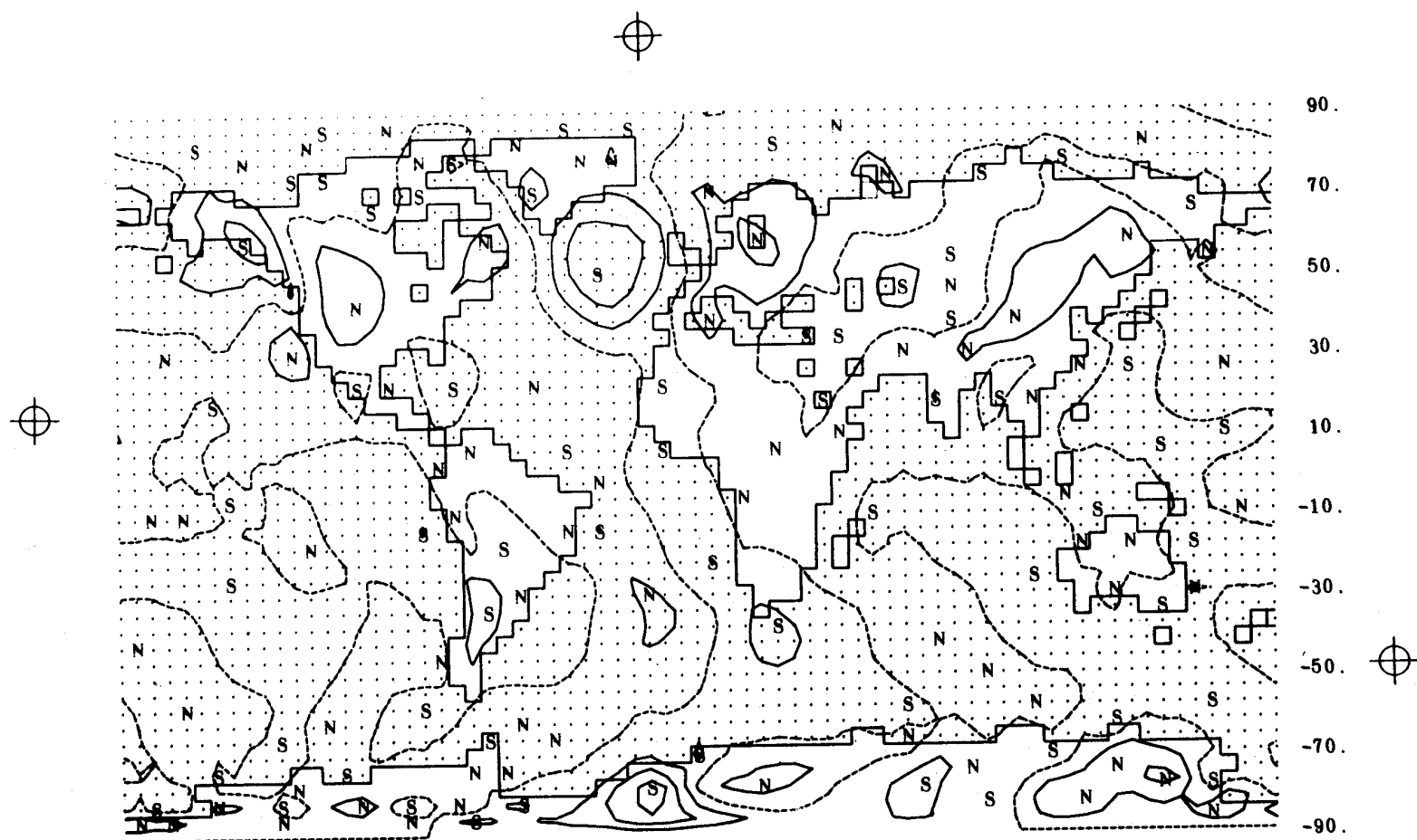
Fig. 26 -- The meridional wind at 800 mb simulated for January. The isolines are at intervals of 5 \text{ m sec}^{-1} , with the zero line dashed. The symbols N and S denote local maxima of winds from the north and south.
