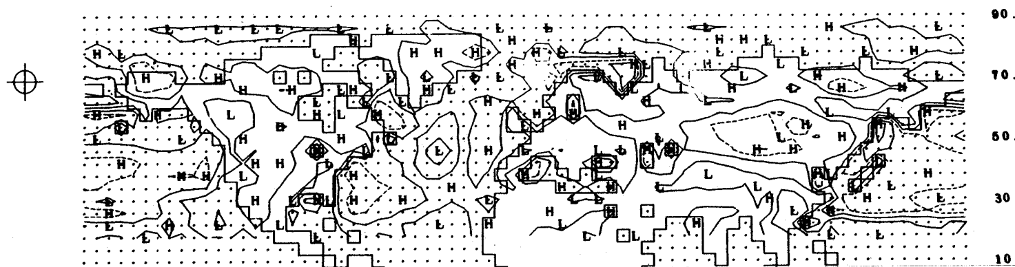
Fig. 35b -- The difference between the simulated and observed cloudiness (Fig. 34 minus Fig. 35a) in the northern hemisphere, with the isolines at 0.2-cloudiness intervals and the zero isoline dashed.
