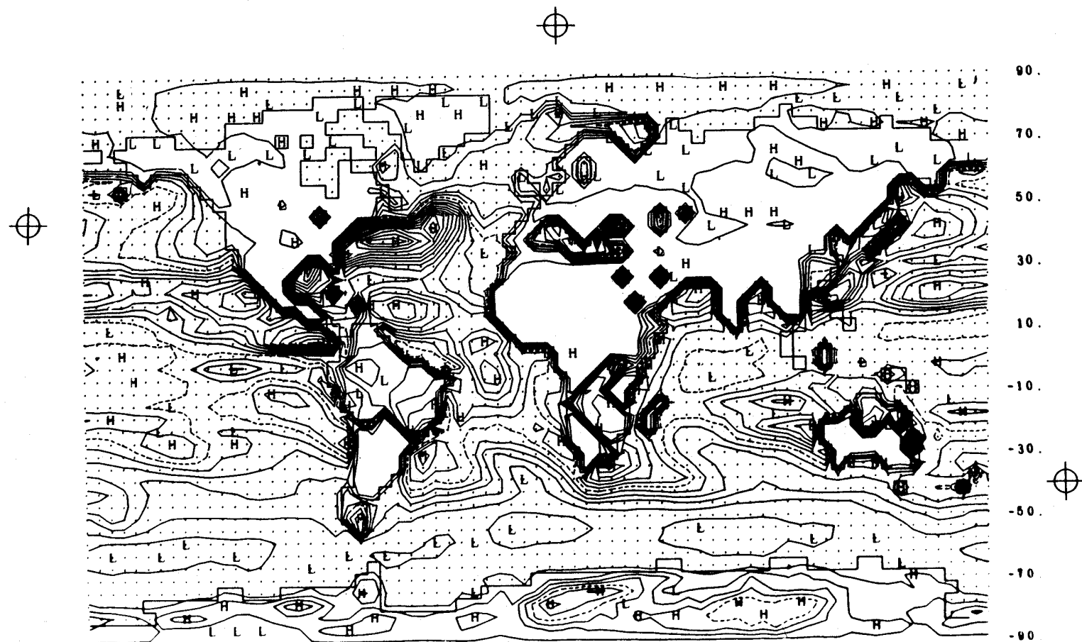
Fig. 40a -- The simulated evaporation rate for January, with isolines at intervals of 1 mm day -1 and the 5 mm day -1 isoline dashed.
