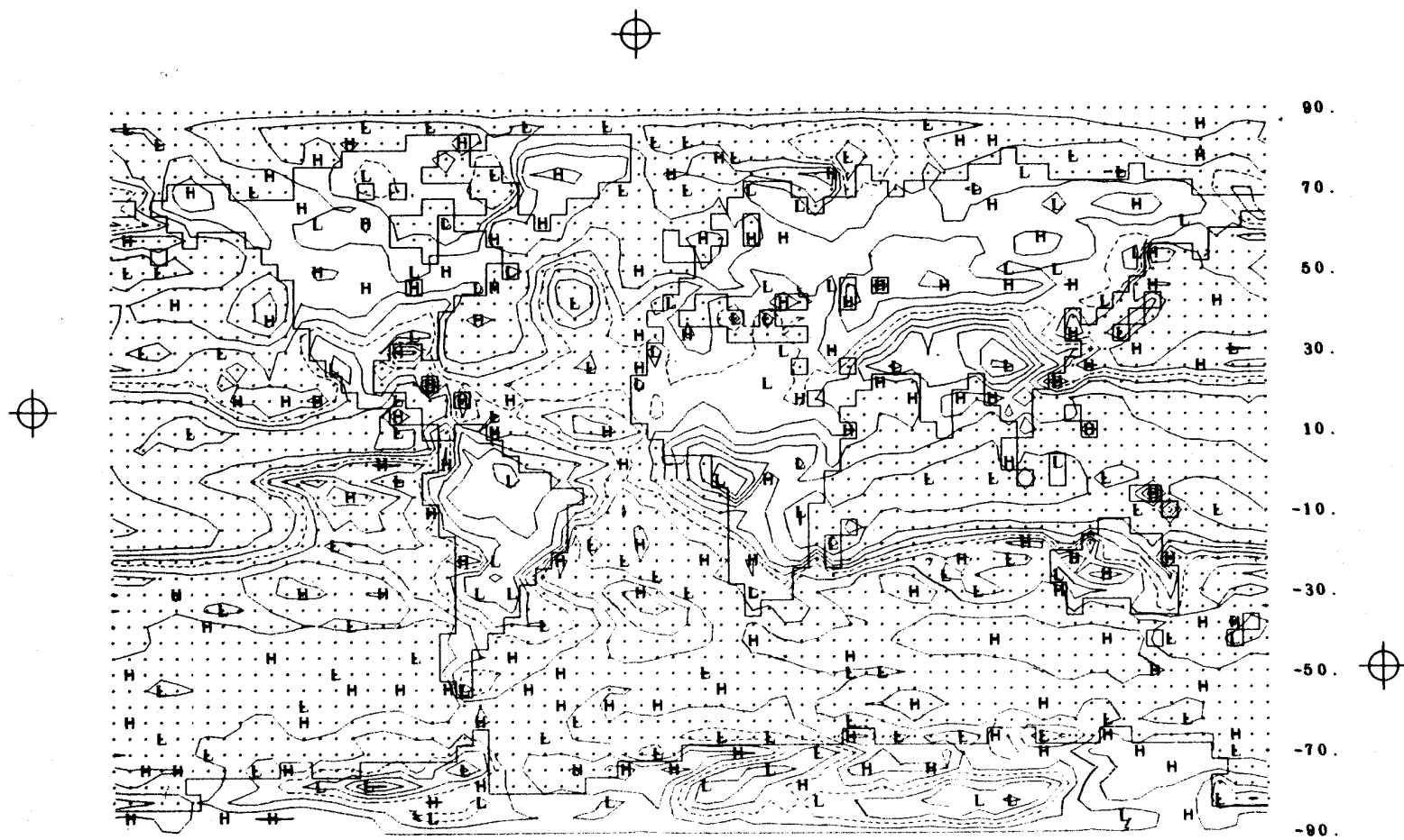
Fig. 32 -- The difference between the simulated and observed 800-mb relative humidity (Fig. 31a minus Fig. 31b). The isoline interval is 10 percent with the zero line dashed.
