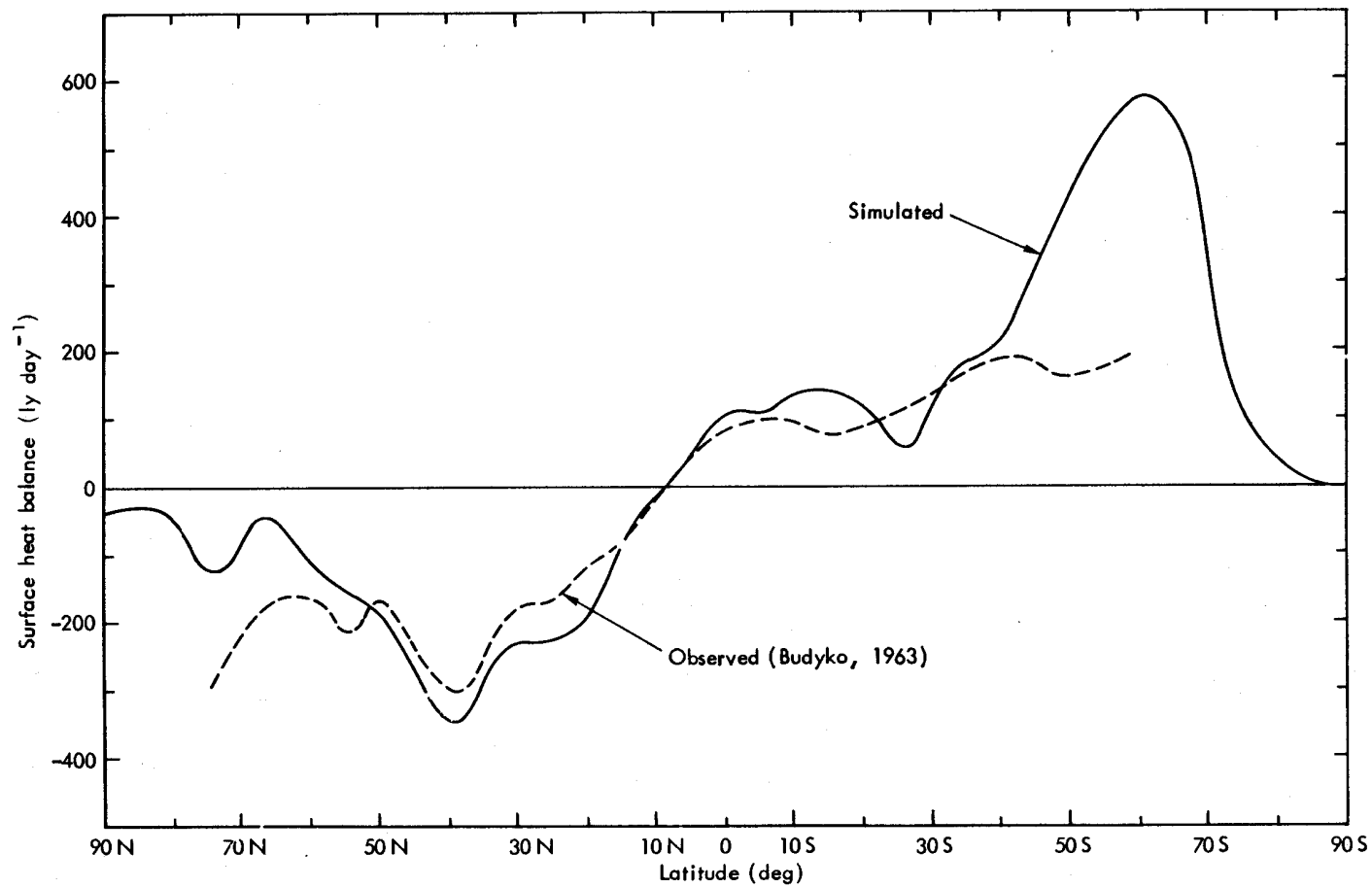
Fig. 52 -- The zonal average of the surface heat balance as simulated for January (full line) and as observed (dashed line), based on the data of Fig. 50.
