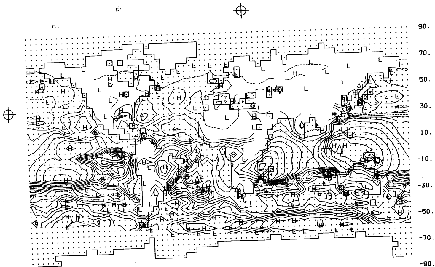
Fig. 48 -- The difference between the simulated and observed shortwave (solar) radiation incident at the surface (Fig. 47a minus Fig. 47b). The isoline interval is 50 \text{ ly day}^{-1} , with the zero isoline dashed.
