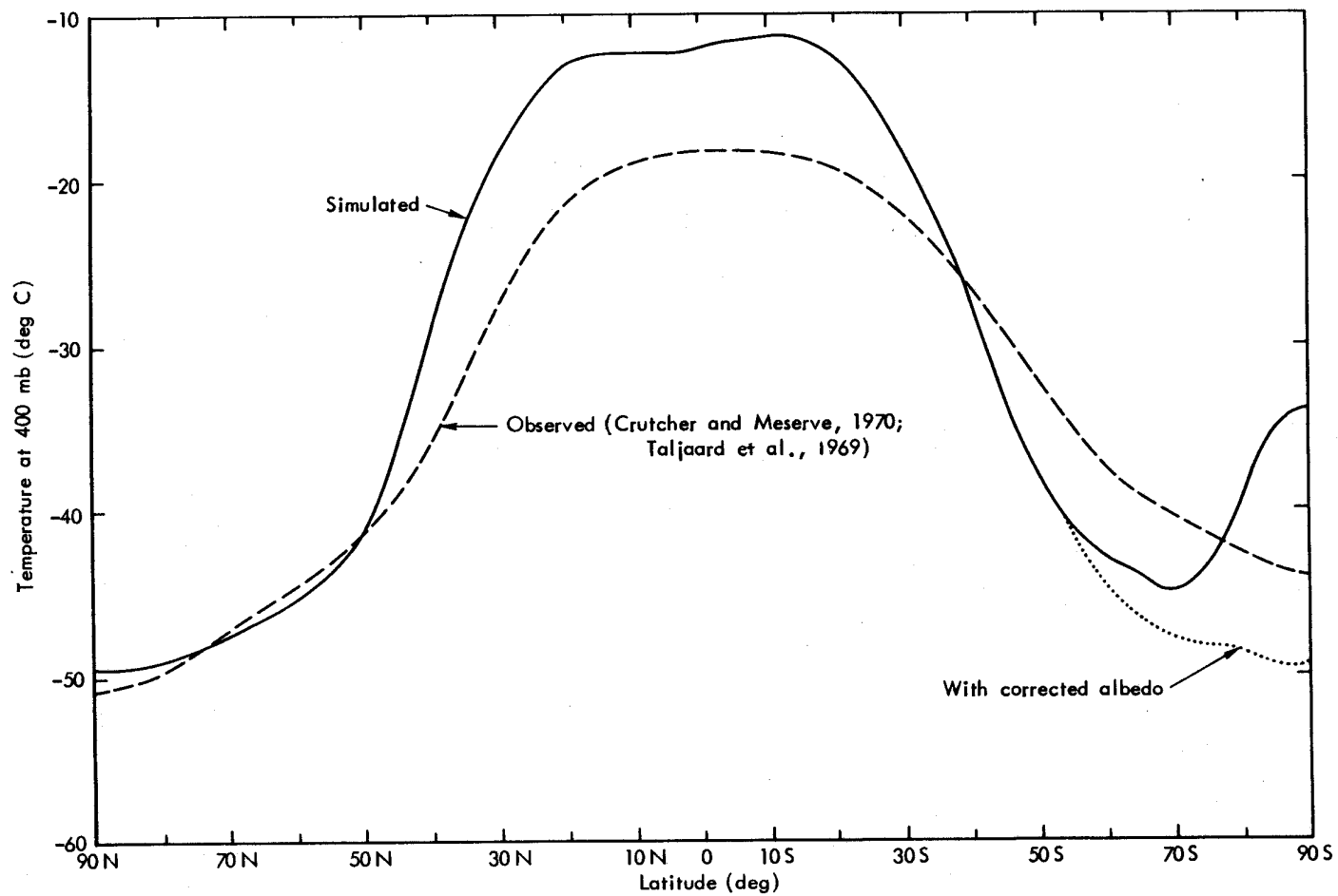
Fig. 21 -- The zonal average January temperature at 400 mb as simulated (full line) and as observed (dashed line), based on the data of Fig. 19.
