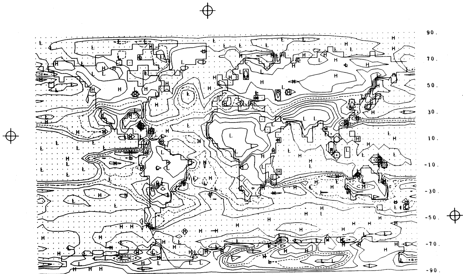
Fig. 31a -- The simulated relative humidity for January at 800 mb, with isolines at 10-percent intervals and the 60-percent isoline dashed.
