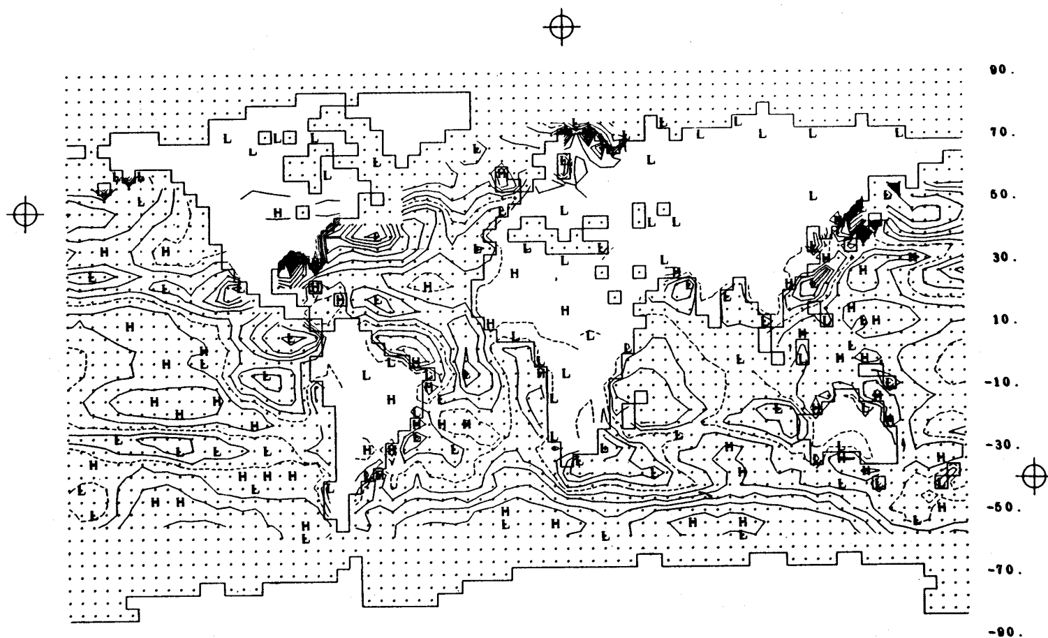
Fig. 51 -- The difference between the simulated and observed surface heat balance (Fig. 50a minus Fig. 50b). The isoline interval is 100 \text{ ly day}^{-1} with the zero isoline dashed.
