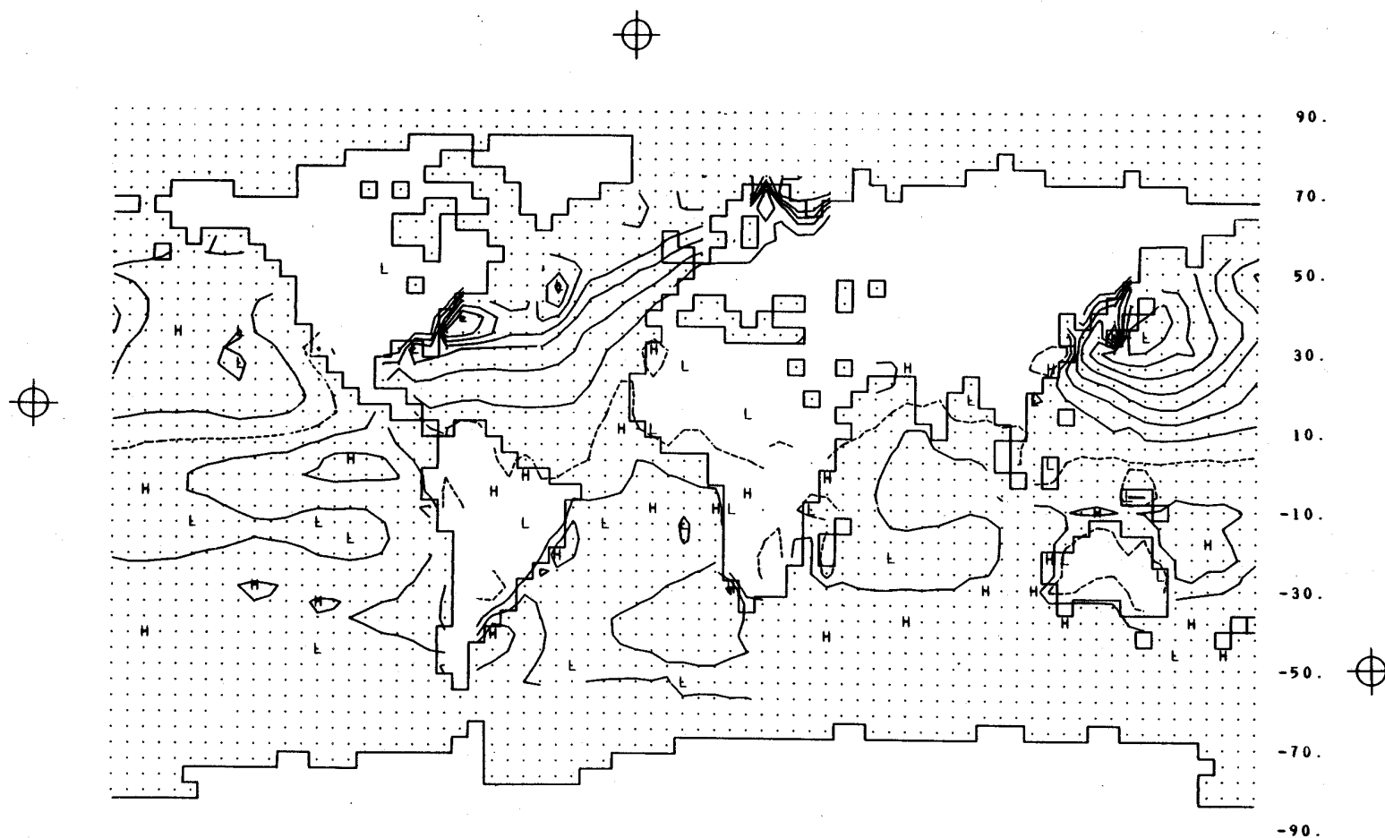
Fig. 50b -- The observed surface heat balance in January, given by the excess of the solar radiation absorbed over the (usual) losses due to evaporative cooling, long-wave radiation, and upward sensible heat flux. The isoline interval is 100 \text{ ly day}^{-1} , with the zero isoline dashed. Based on data of Budyko (1963) as summarized by Schutz and Gates (1971).
