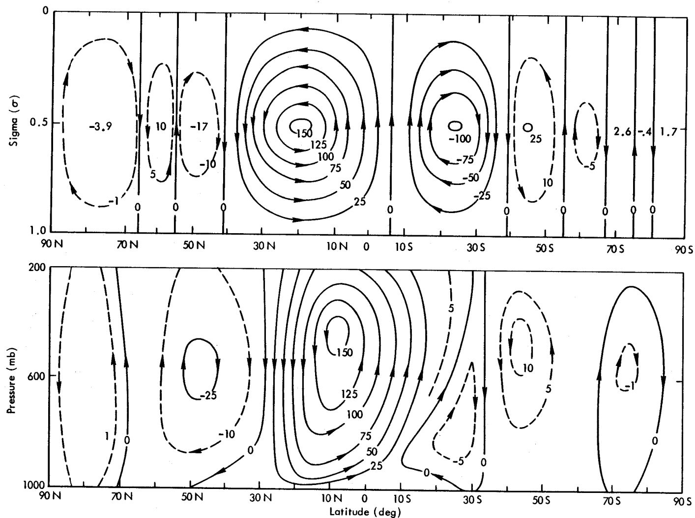
Fig. 30b -- The streamfunction for the time-mean, zonally averaged mass flux in 10^{12} \text{ g sec}^{-1} . That simulated for January is shown above (symmetric about \sigma = 1/2 ), and that observed (for December, January, February) is shown below as given by Newell et al. (1970). The direction of flow is given by the arrows.
