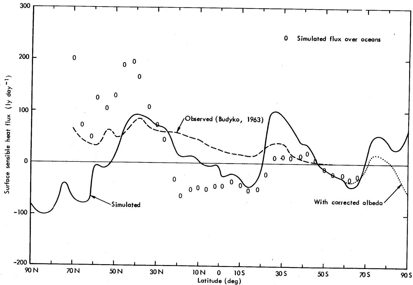
Fig. 46 -- The zonal average of the surface sensible heat flux as simulated for January (full line) and as observed (dashed line) according to the data of Fig. 44. The open circles denote the zonal average over the oceans only.
