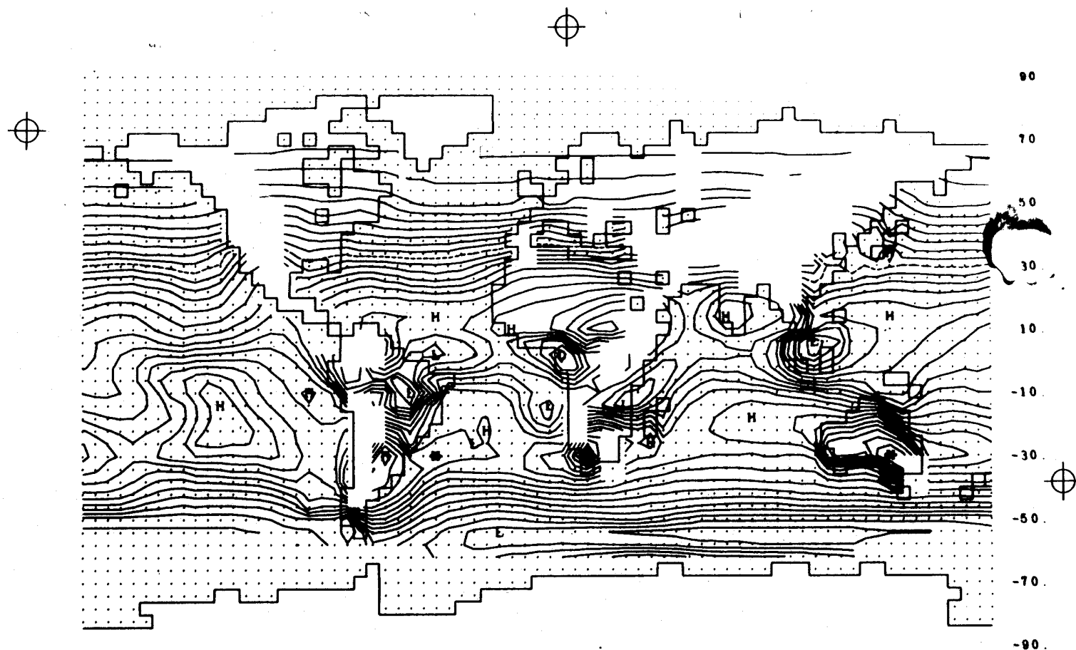
Fig. 47b -- The observed shortwave (solar) radiation incident at the surface in January, with isolines every 25 ly day -1 and the 250 ly day -1 isoline dashed. From data of Budyko (1963) as summarized by Schutz and Gates (1971).
