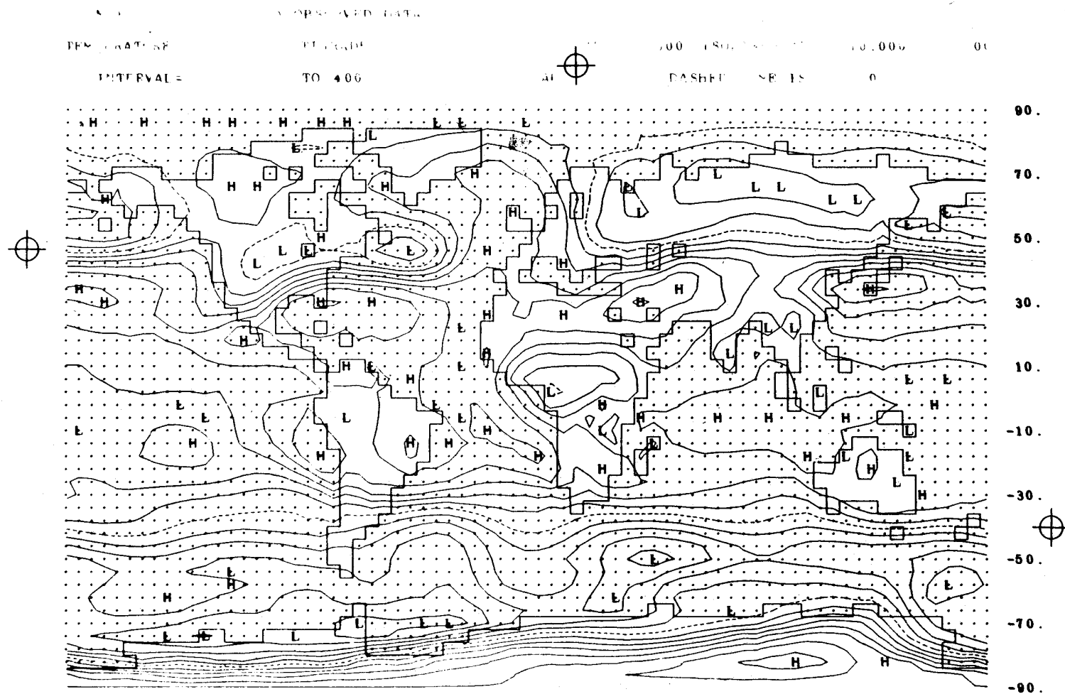
Fig. 20 -- The difference between the simulated and observed 400-mb temperature (Fig. 19a minus Fig. 19b). The isoline interval is 2 deg C with the 0-deg C line dashed.
