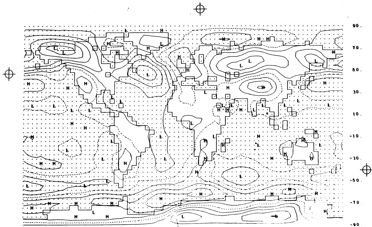
Fig. 5 -- The difference between the simulated and observed sea-level pressure (Fig. 4a minus Fig. 4b). The isobar interval is 5 mb with the zero line dashed.
