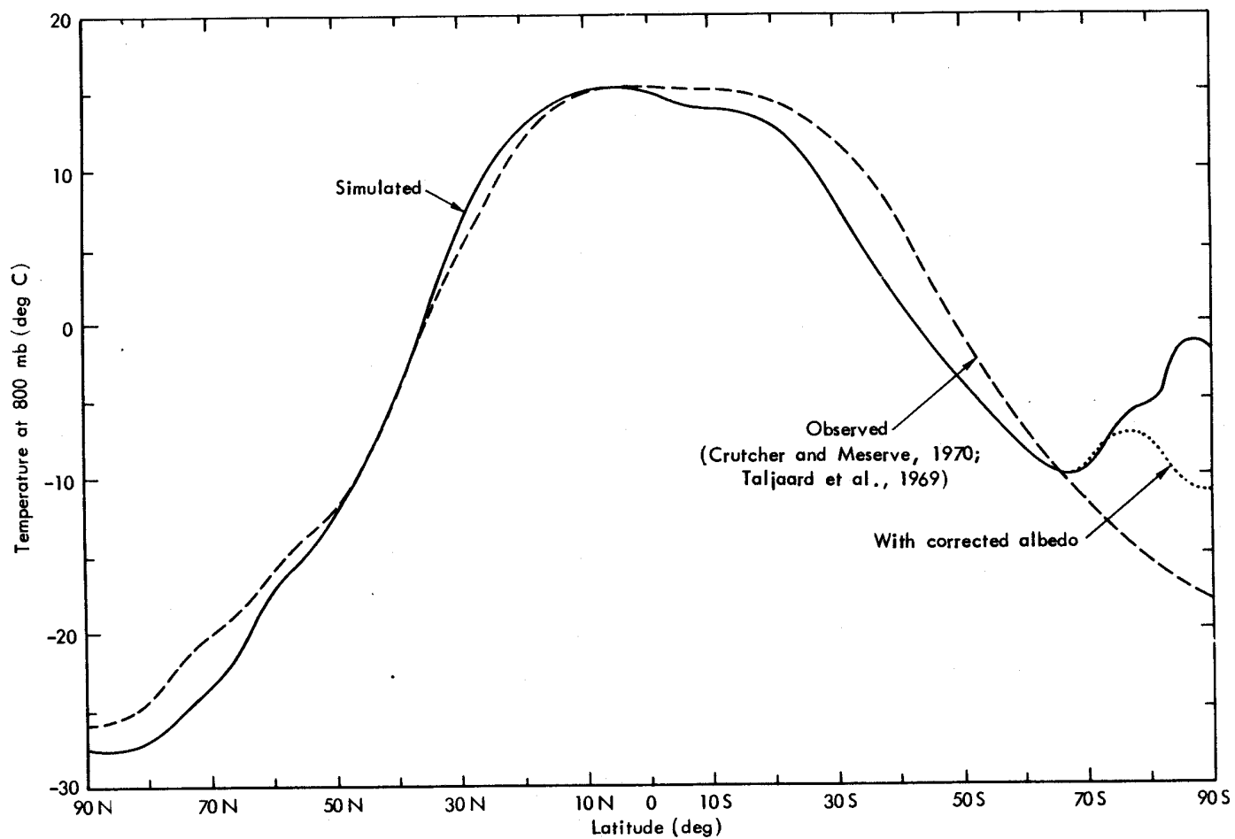
Fig. 18 -- The zonal average January 800-mb temperature as simulated (full line) and as observed (dashed line), based on the data of Fig. 16.
