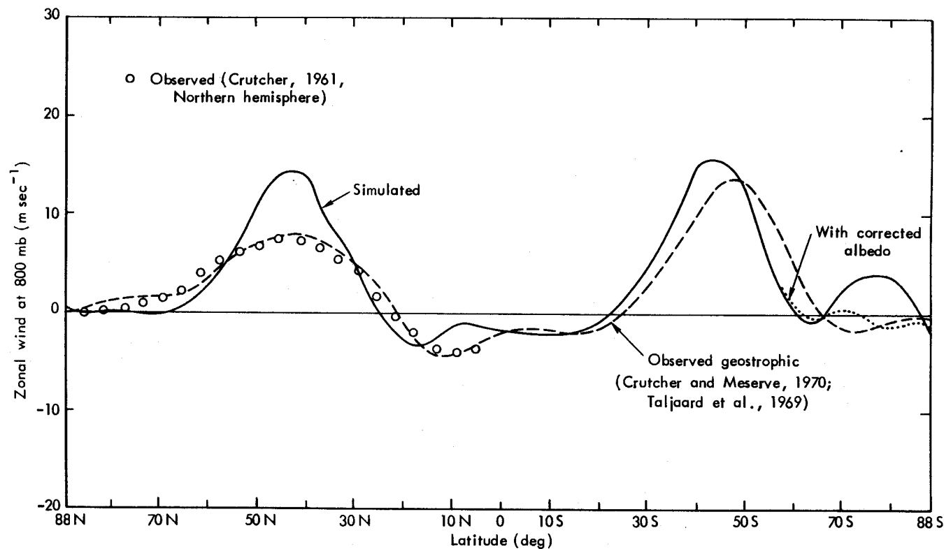
Fig. 24 -- The zonal average of the mean zonal winds at 800 mb simulated for January (full line), together with the distribution of the corresponding observed geostrophic winds (dashed line) as given by Schutz and Gates (1971) based on data of Crutcher and Meserve (1970) and Taljaard et al. (1969). Also shown by the open circles in the northern hemisphere are the zonal averages of the observed zonal wind (for December, January, February) from Schutz and Gates (1971) based on data of Crutcher (1961).
