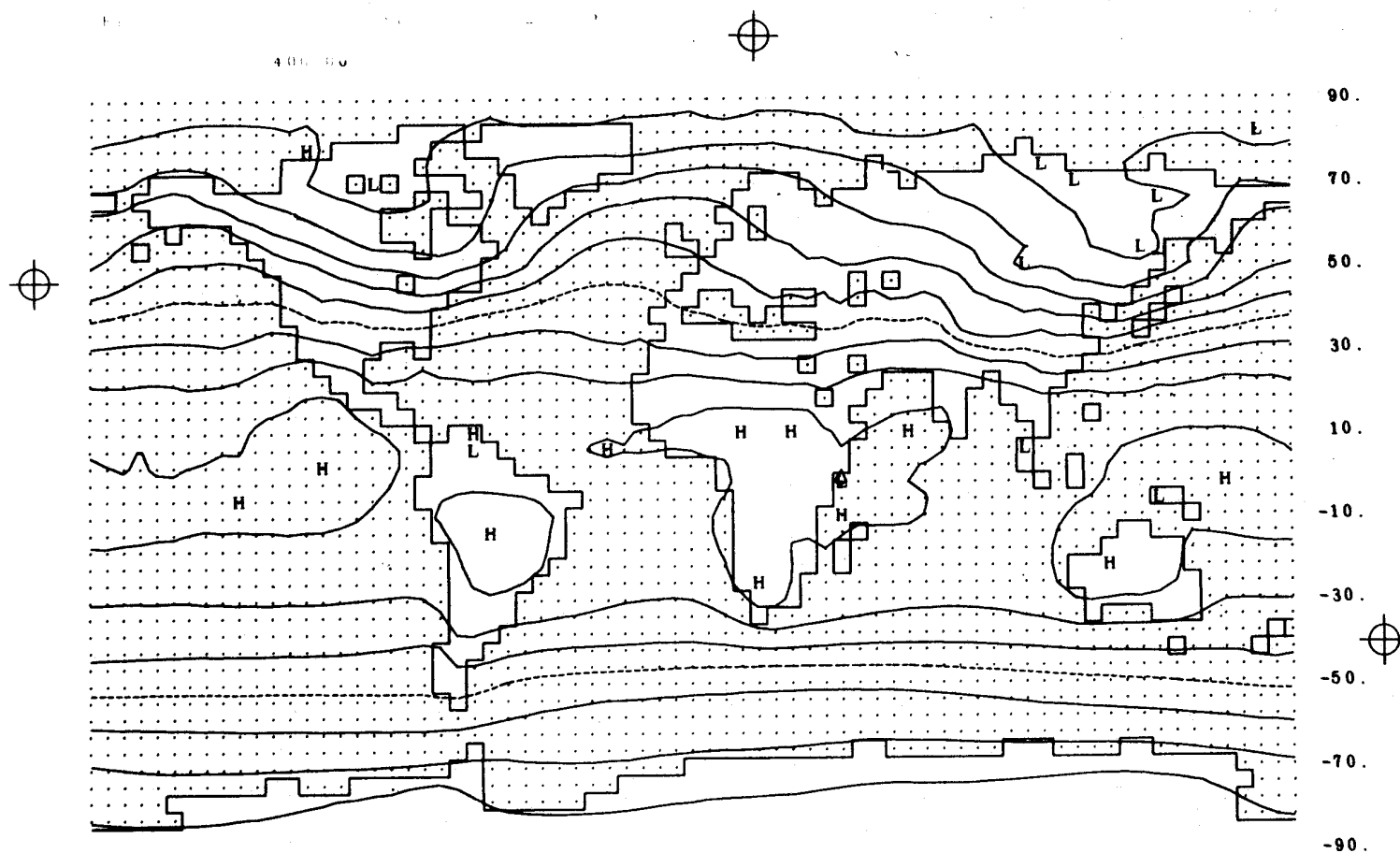
Fig. 16b -- The observed temperature for January at 800 mb, with isolines at 5-deg C intervals and the 0-deg C isotherm dashed. Based on data of Crutcher and Meserve (1970) and Taljaard et al. (1969) as summarized by Schutz and Gates (1971).
