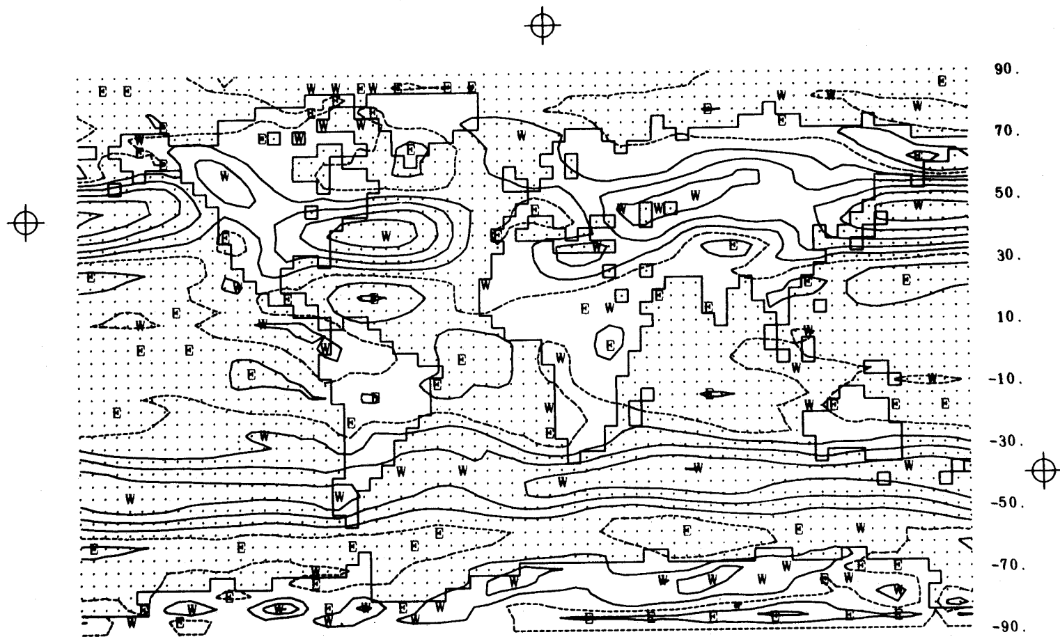
Fig. 22 -- The zonal wind at 800 mb simulated for January. The isolines are at intervals of 5 m sec -1 , with the zero line dashed. The symbols W and E denote local maxima of winds from the west and east.
