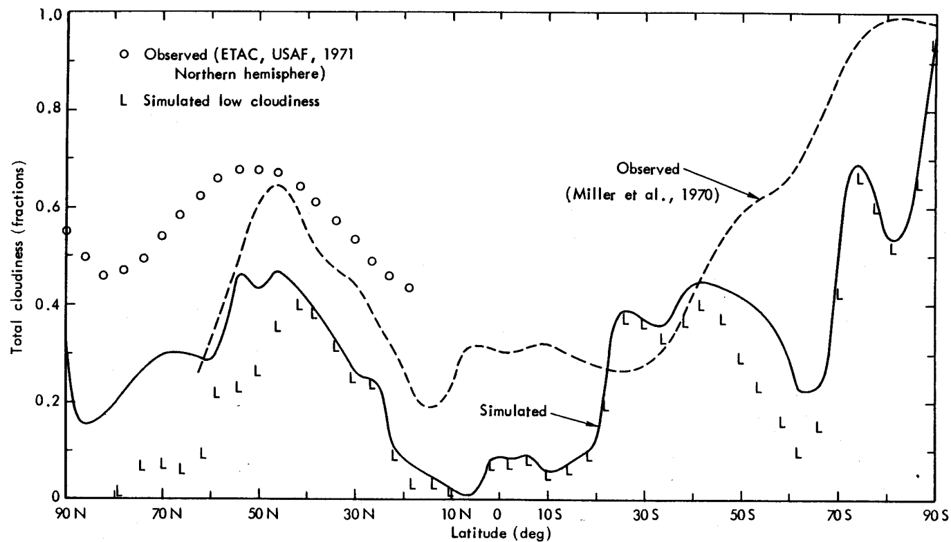
Fig. 36 -- The zonal average of the mean cloudiness as simulated for January (full line), together with the observed distribution (dashed line). From Schutz and Gates (1971), based on satellite data of Miller (1970). Also shown in the northern hemisphere (open circles) are the observed values (from both satellite and conventional observations) based on the data of Fig. 35. The symbol L denotes the simulated low cloudiness only.
