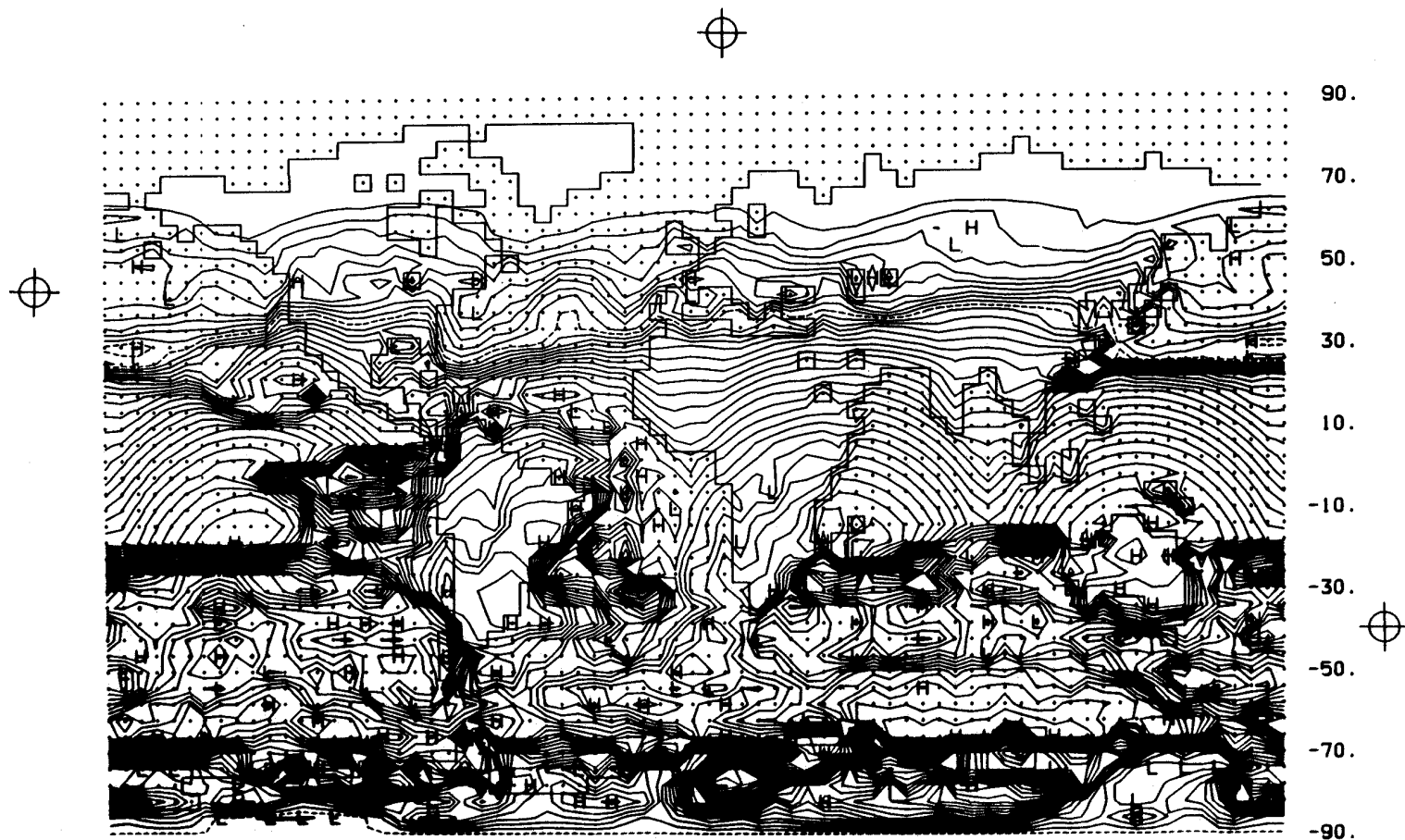
Fig. 47a -- The simulated shortwave (solar) radiation incident at the surface in January, with isolines every 25 ly day -1 and the 250 ly day -1 isoline dashed.
