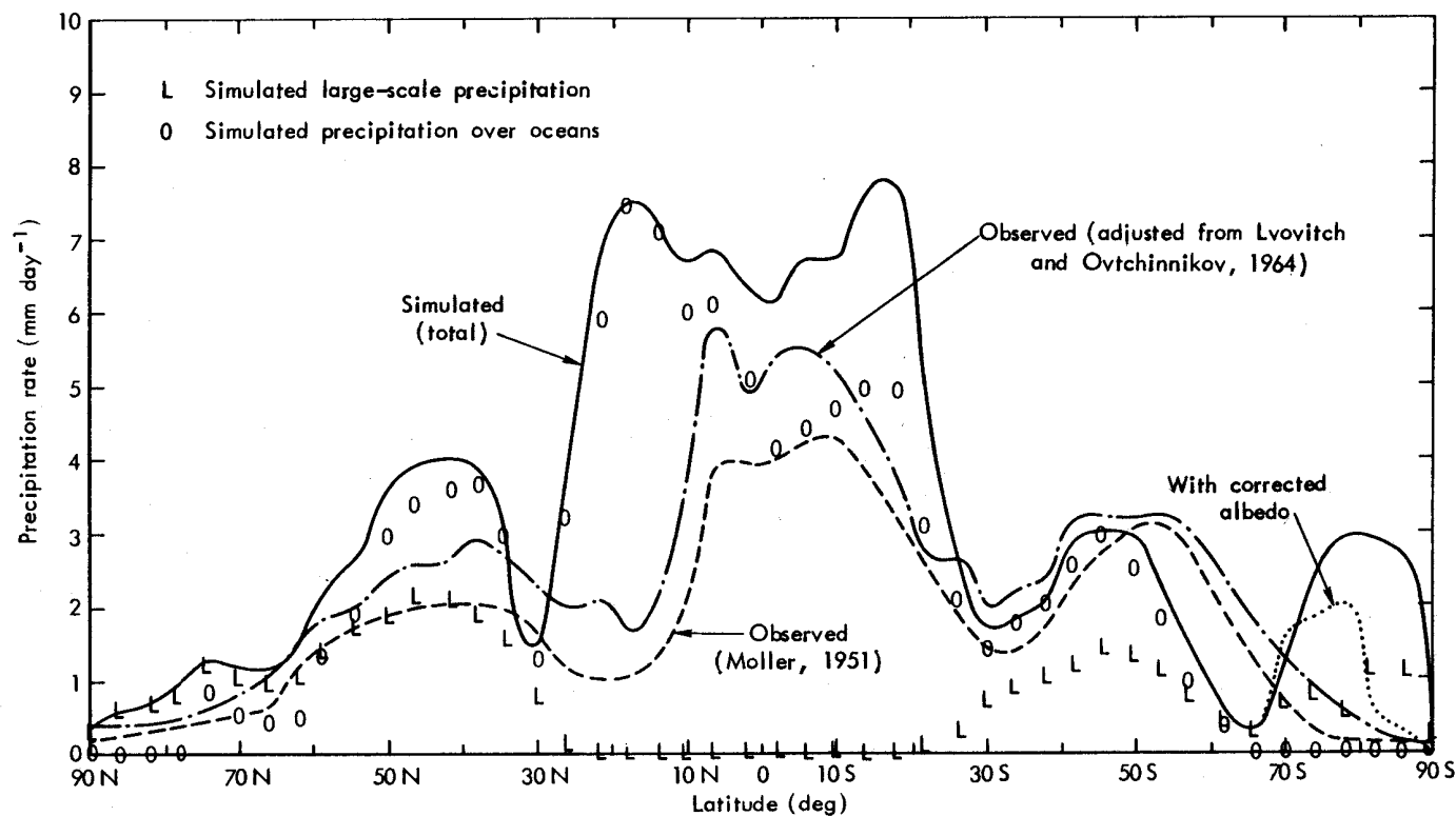
Fig. 39 -- The zonal average of the precipitation rate as simulated for January (full line) and as observed (dashed line), based on the data of Fig. 37. The dash-dotted line gives the observed precipitation from the data of Lvovitch and Ovtchinnikov (1964) as modified by Schutz and Gates (1971) for December, January, and February. The symbol L denotes the zonal averages of the simulated large-scale precipitation rate only, and the open circles denote that portion of the total simulated precipitation that falls over the oceans.
