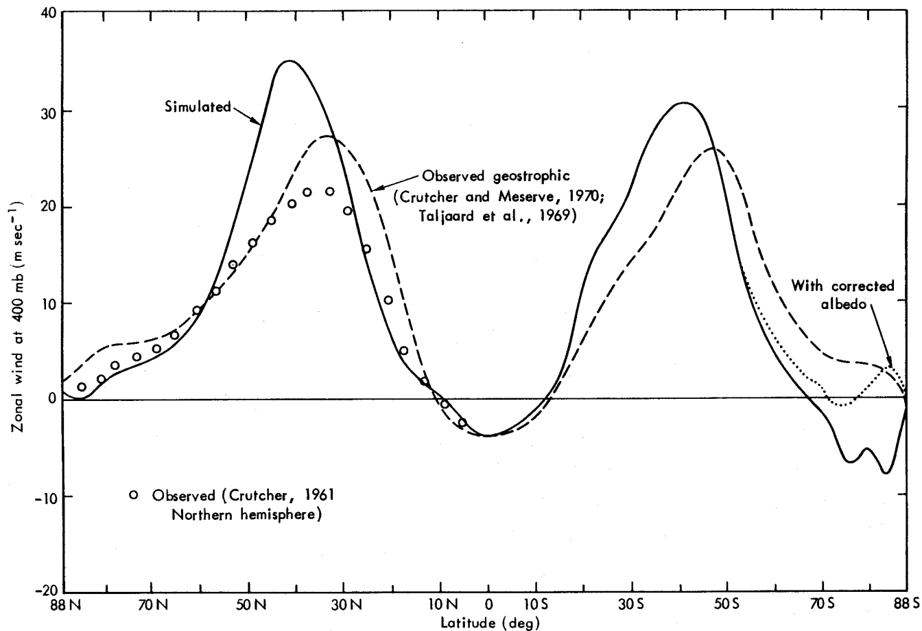
Fig. 25 -- The zonal average of the mean zonal winds at 400 mb simulated for January (full line), together with the distribution of the corresponding observed geostrophic winds (dashed line) as given by Schutz and Gates (1971) based on data of Crutcher and Meserve (1970) and Taljaard et al. (1969). Also shown by the open circles in the northern hemisphere are the zonal averages of the observed zonal wind (for December, January, February) from Schutz and Gates (1971) based on data of Crutcher (1961).
