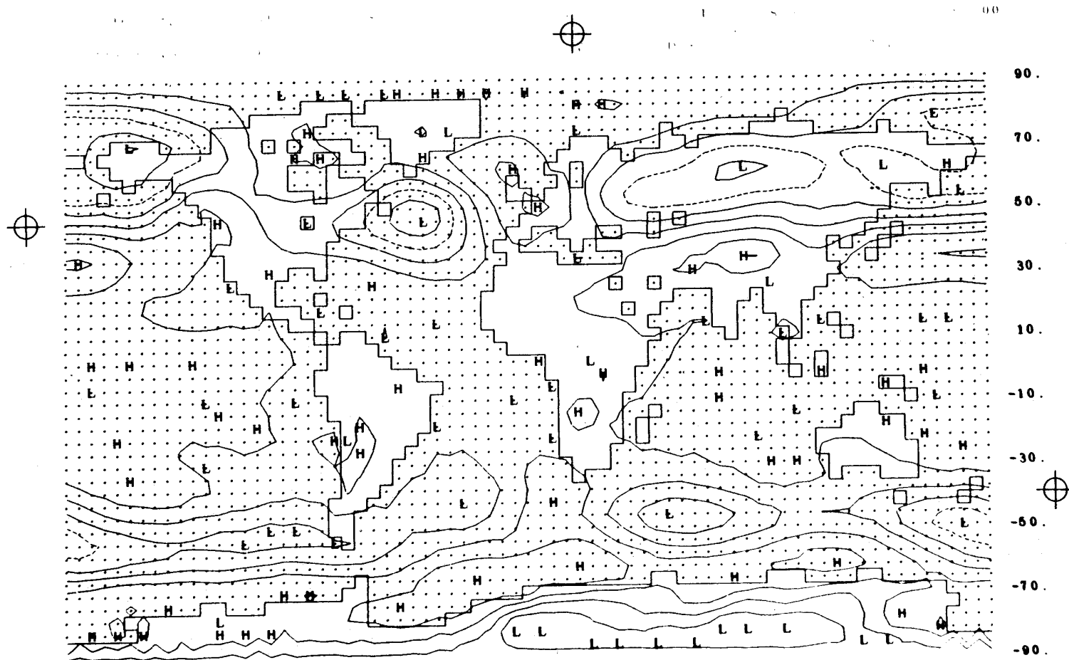
Fig. 8 -- The difference between the simulated and observed 800-mb geopotential height (Fig. 7a minus Fig. 7b). The isoline interval is 50 m with the 200-m line dashed.
