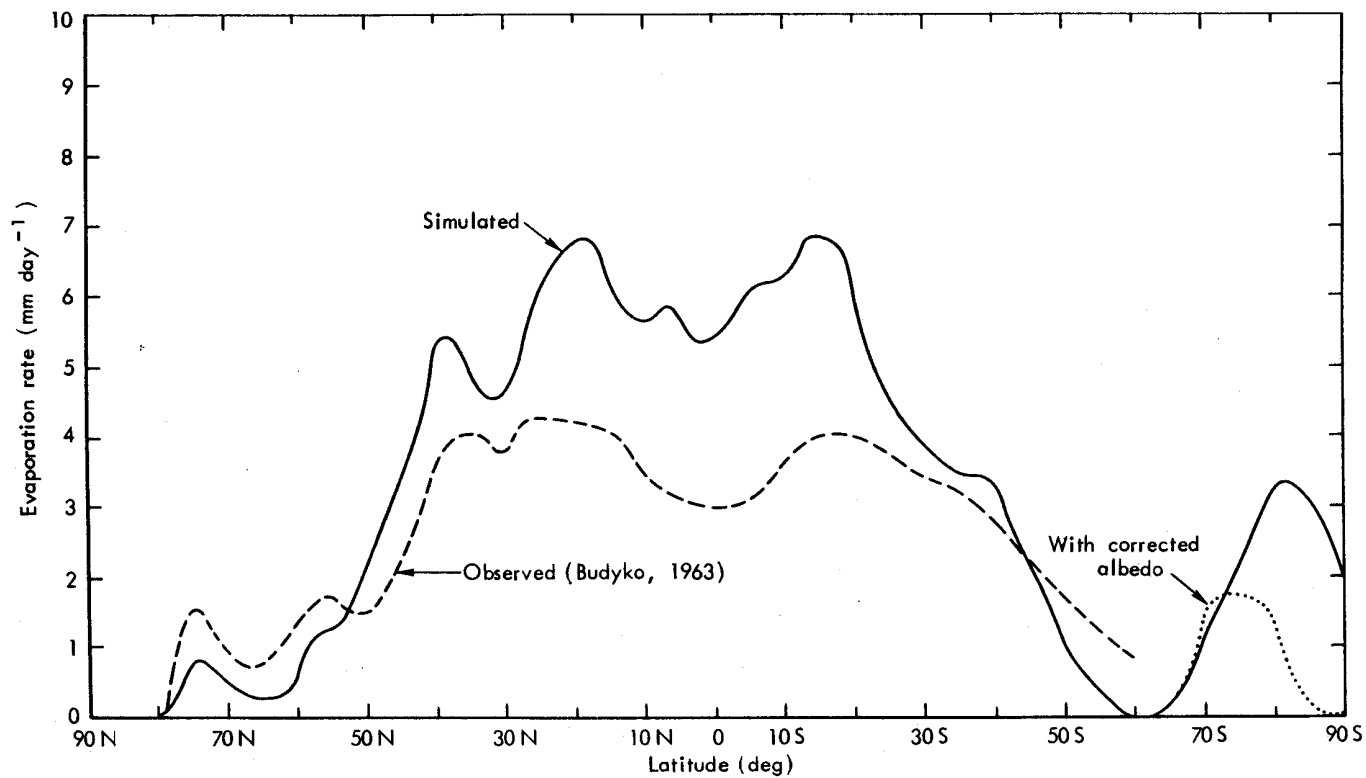
Fig. 42 -- The zonal average of the evaporation rate as simulated for January (full line) and as observed (dashed line), based on the data of Fig. 40.
