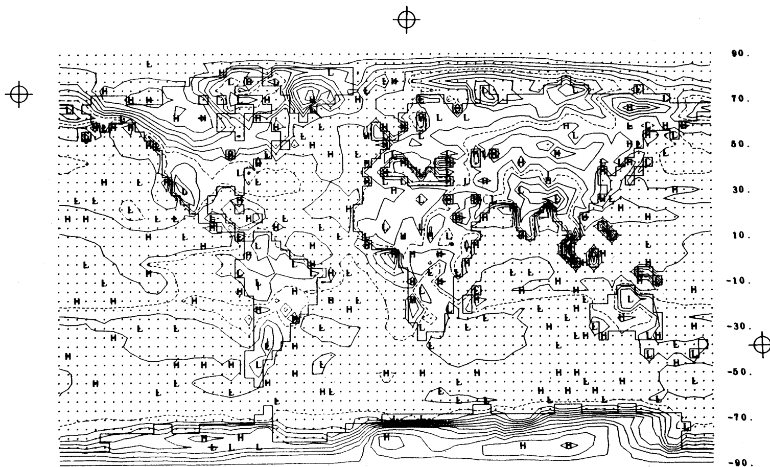
Fig. 14 -- The difference between the simulated and observed surface air temperature (Fig. 13a minus Fig. 13b). The isoline interval is 3 deg C with the zero line dashed.
