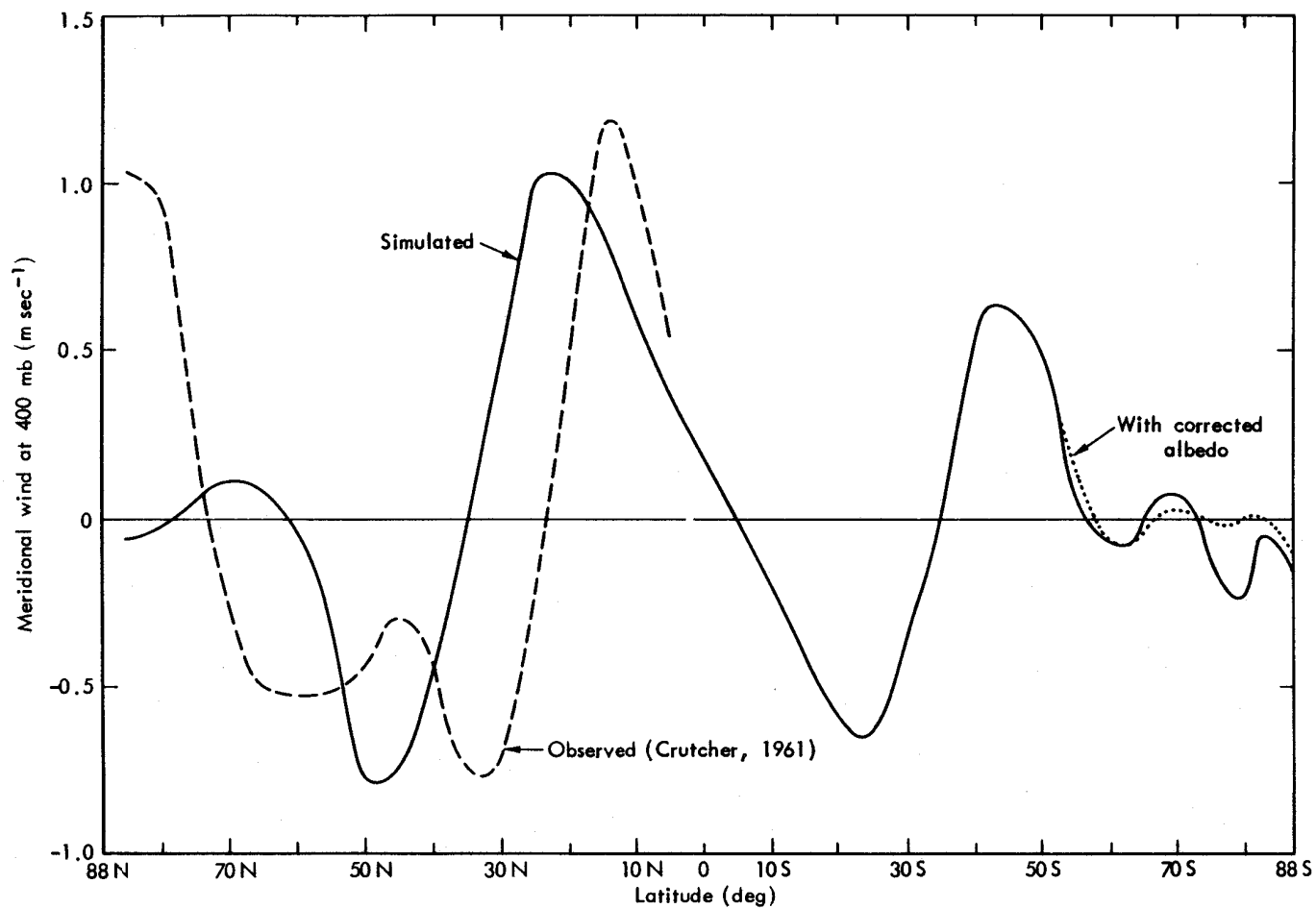
Fig. 29 -- The zonal average of the mean meridional winds at 400 mb simulated for January (full line), with the corresponding observed winds (dashed line) in the northern hemisphere. From Schutz and Gates (1971), based on data of Crutcher (1961).
