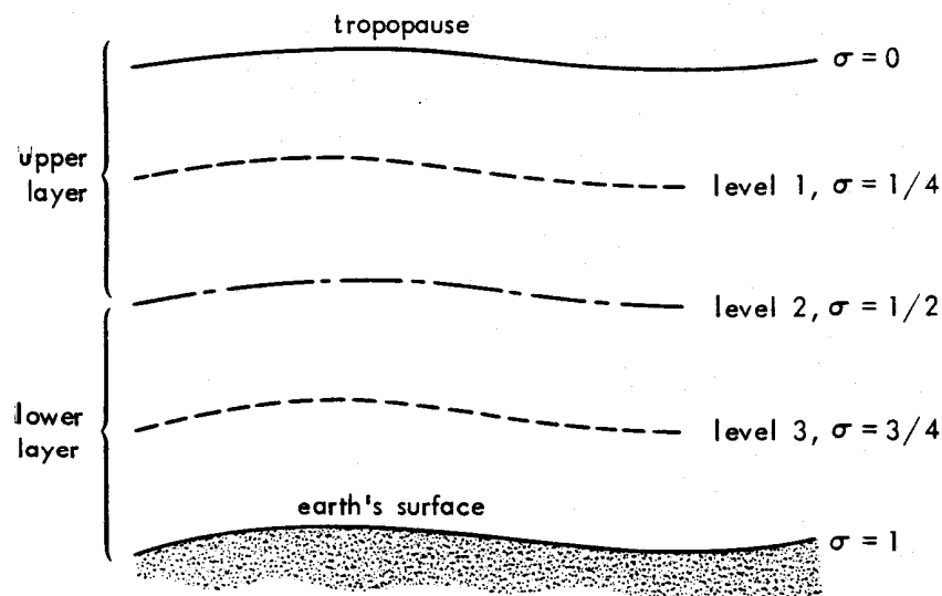
Fig. 1 -- Schematic representation of the model's vertical structure.
