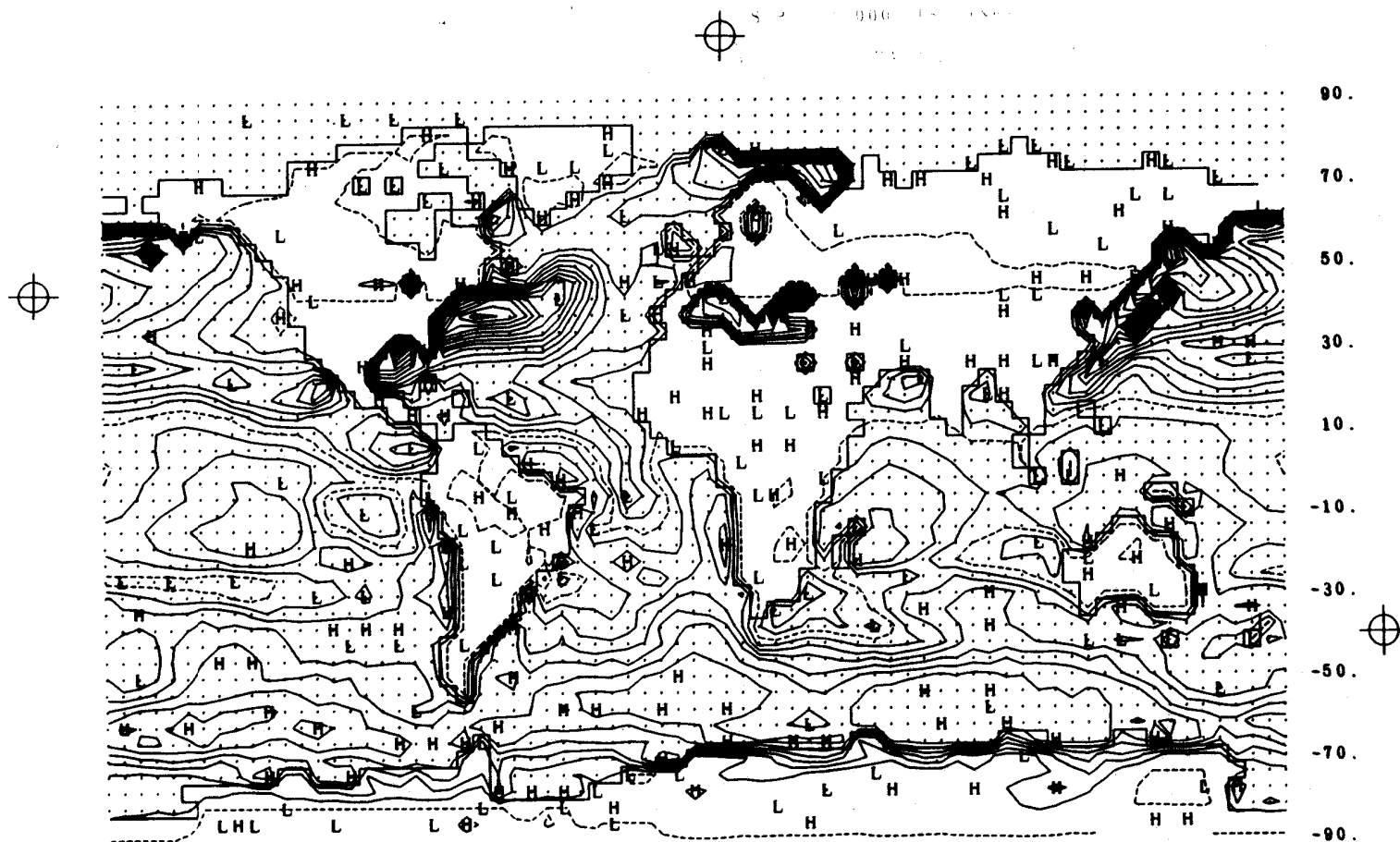
Fig. 50a -- The simulated surface heat balance in January, given by the excess of the solar radiation absorbed over the (usual) losses due to evaporative cooling, long-wave radiation, and upward sensible heat flux. The isoline interval is 100 ly day -1 , with the zero isoline dashed. Data from Figs. 40, 44, and 47.
