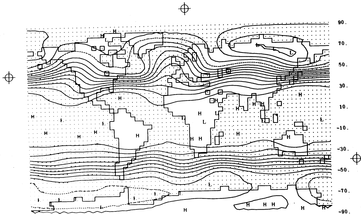
Fig. 10a -- The simulated geopotential height at 400 mb for January, with isolines every 100 m and the 7000-m contour dashed.
