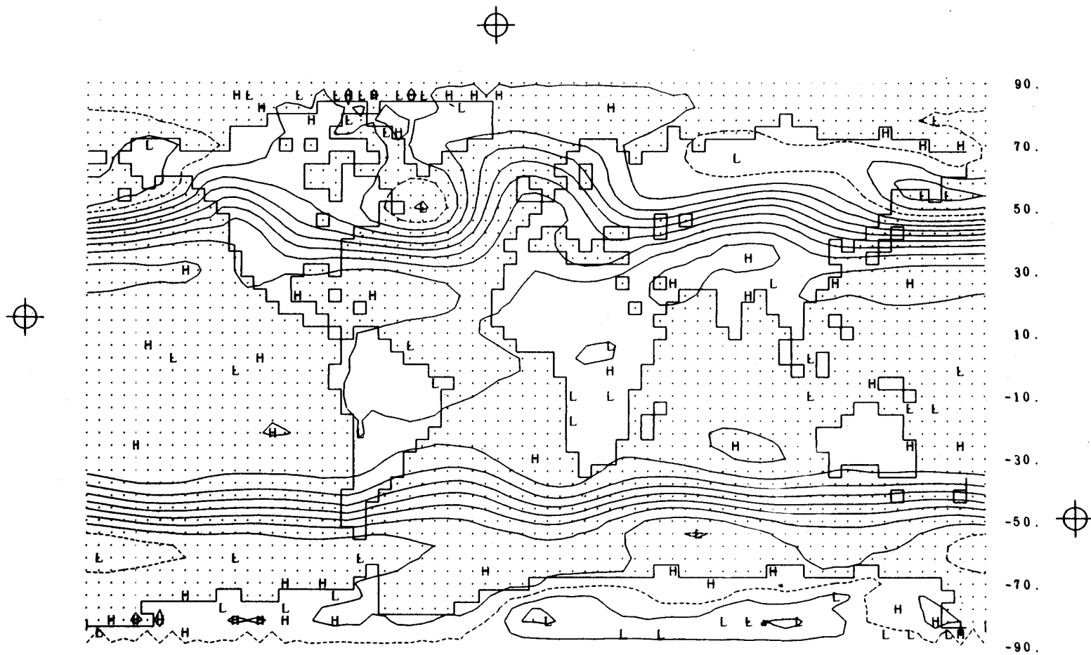
Fig. 7a -- The simulated geopotential height at 800 mb for January, with isolines every 50 m and the 2000-m contour dashed.
