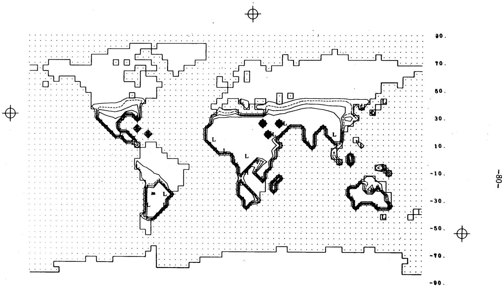
Fig. 43 -- The simulated ground wetness in January, with isolines every 0.2 and the 0.6 isoline dashed. The oceans and all ice-covered surfaces are considered completely wet (ground wetness \equiv 1 ).
