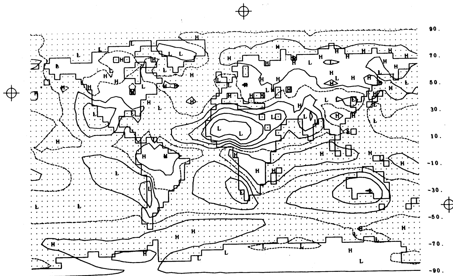
Fig. 31b -- The observed relative humidity for January at 800 mb, with isolines at 10-percent intervals and the 60-percent isoline dashed. From Schutz and Gates (1971), based on data of Crutcher and Meserve (1970) and Taljaard et al. (1969).
