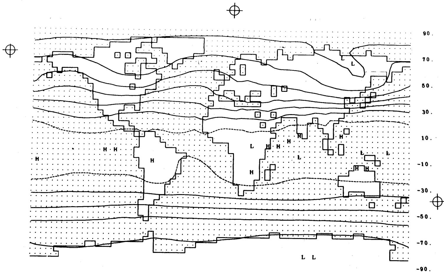
Fig. 19b -- The observed temperature for January at 400 mb, with isolines every 5 deg C and the -20-deg C isotherm dashed. Based on data of Crutcher and Meserve (1970) and Taljaard et al. (1969) as summarized by Schutz and Gates (1971).
