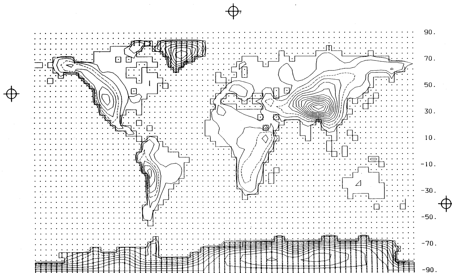
Fig. 2 -- The surface elevation used in the control experiment, with isolines every 1000 ft and the 3000-ft contour dashed. The overprinted symbol I denotes the locations of ice-covered land. The points of the basic 4-deg latitude, 5-deg longitude grid are shown over the oceans, with the latitude given on the right. From Gates et al. (1971).
