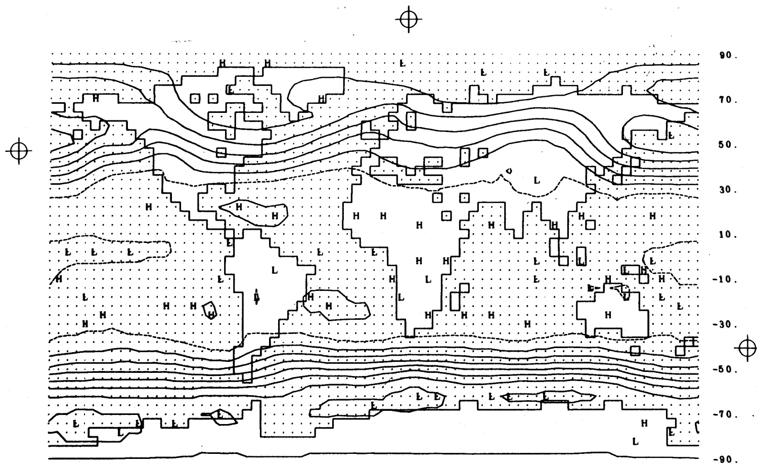
Fig. 7b -- The observed geopotential height at 800 mb for January with isolines every 50 m and the 2000-m contour dashed. From Schutz and Gates (1971), based on data of Crutcher and Meserve (1970) and Taljaard et al. (1969).
