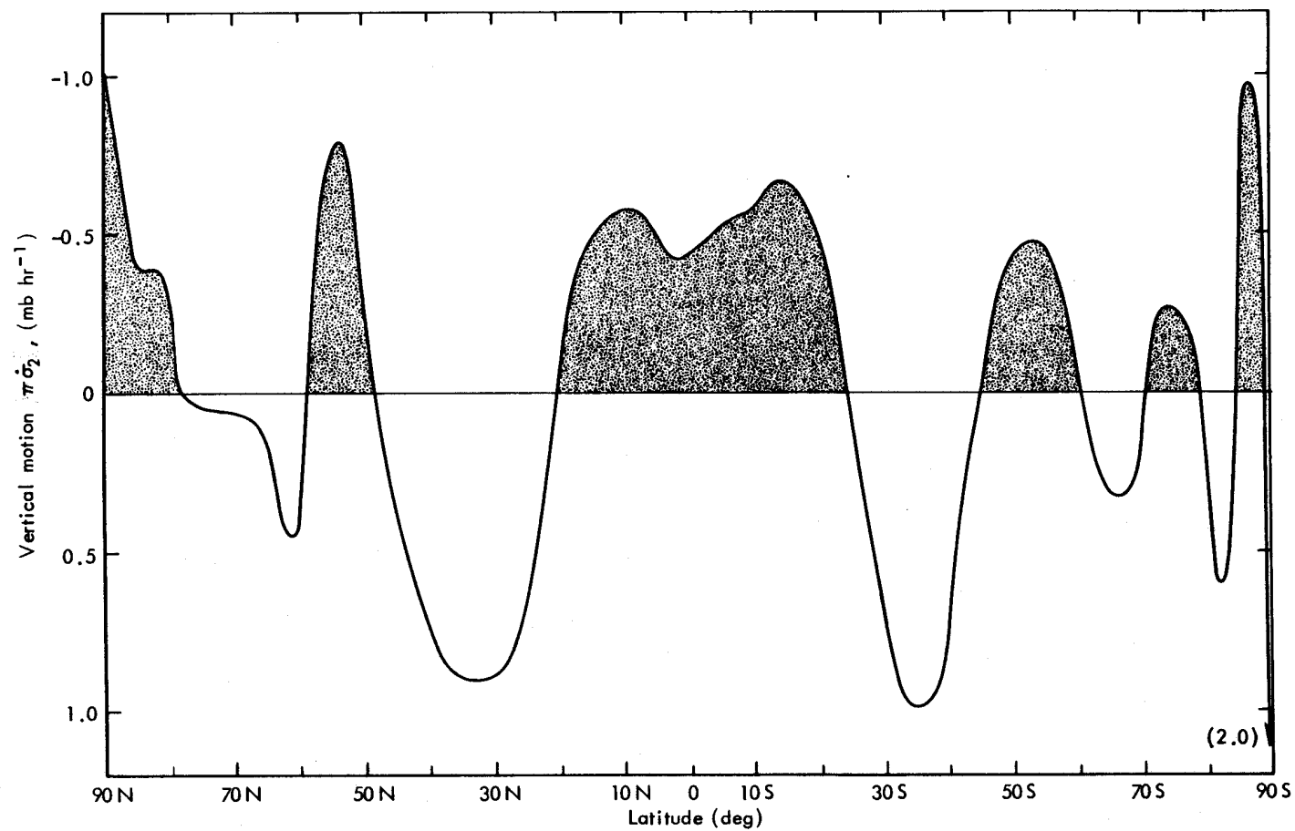
Fig. 30a -- The zonal average of the mean vertical motion simulated for January, as given by the measure \pi \sigma_2 . Neglecting surface pressure variations, 1 \text{ mb hr}^{-1} here corresponds to a vertical velocity of about 0.4 \text{ cm sec}^{-1} at 600 mb. The shading denotes regions of upward vertical motion (see also Fig. 30b).
