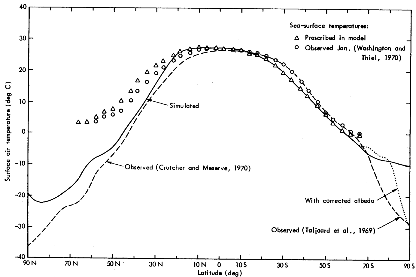
Fig. 15 -- The zonal average surface air temperature as simulated (full line) and as observed (dashed line), based on the data of Fig. 13. Also shown are the zonal averages of the prescribed sea-surface temperature (as used in the simulation) and of the observed sea-surface temperature for January from Schutz and Gates (1971), based on data of Washington and Thiel (1970).
