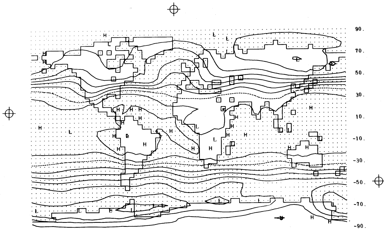
Fig. 19a -- The simulated temperature for January at 400 mb, with isolines every 5 deg C and the -20-deg C isotherm dashed.
