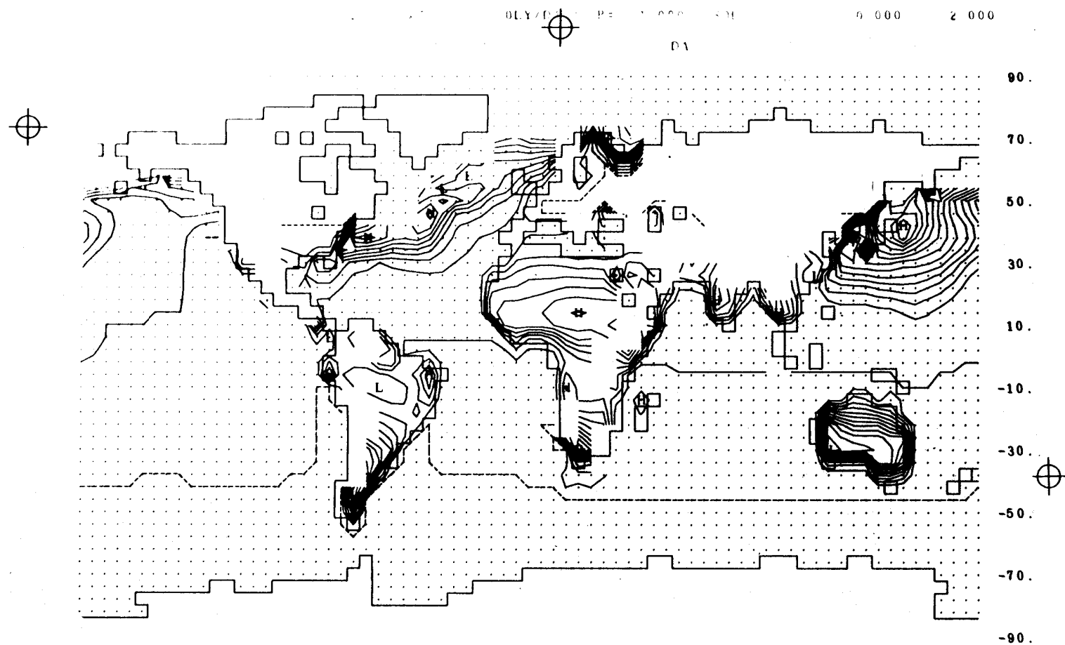
Fig. 44b -- The observed sensible heat flux at the surface for January, with isolines at 20 \text{ ly day}^{-1} intervals and the zero isoline dashed. The blank regions are areas for which observational data are missing. From Schutz and Gates (1971), based on data of Budyko (1963).
