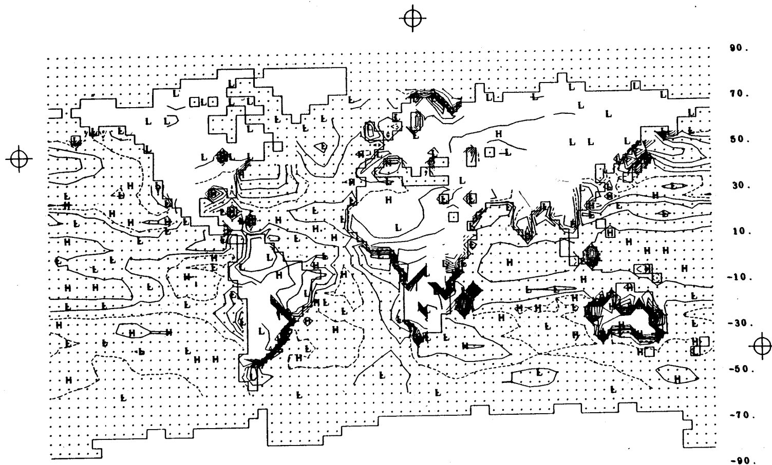
Fig. 45 -- The difference between the simulated and observed surface sensible heat flux (Fig. 44a minus Fig. 44b). The isoline interval is 60 \text{ ly day}^{-1} , with the zero isoline dashed.
