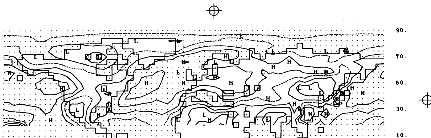
Fig. 35a -- The observed January cloudiness in the northern hemisphere, with isolines at 0.1-cloudiness intervals and the 0.5 isoline dashed. From Schutz and Gates (1971), as prepared from data supplied by the Environmental Technical Applications Center of the U.S. Air Force (1971).
