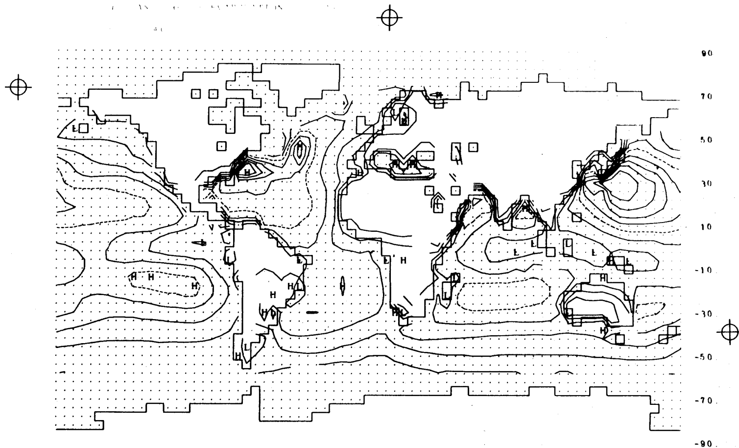
Fig. 40b -- The observed evaporation rate for January, with isolines at intervals of 1 \text{ mm day}^{-1} and the 5 \text{ mm day}^{-1} isoline dashed. The blank regions are areas for which observational data are missing. Based on data of Budyko (1963) as given by Schutz and Gates (1971).
