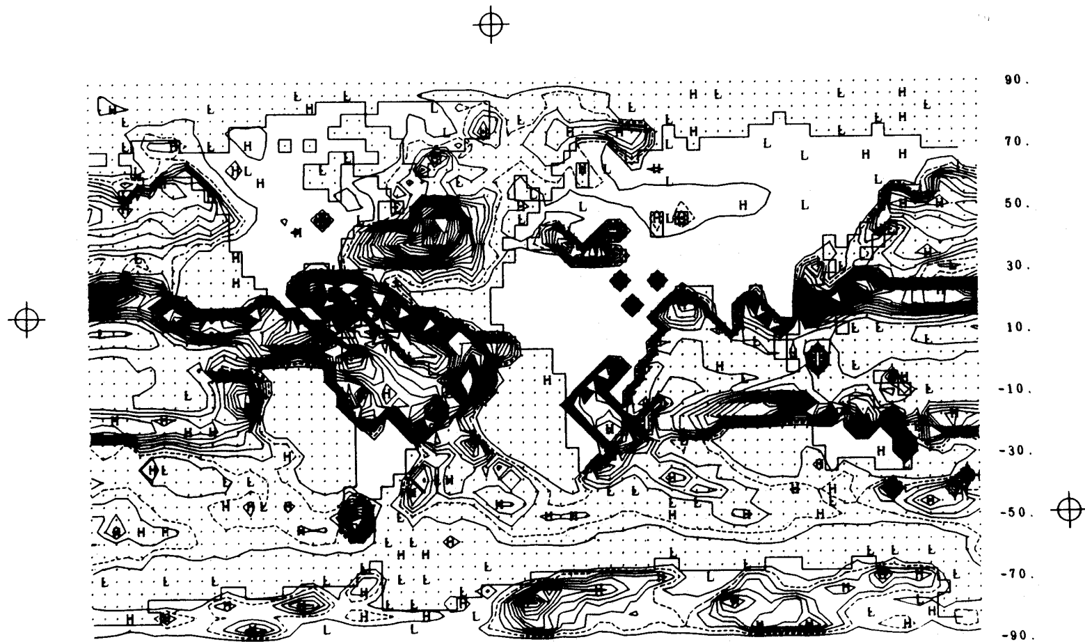
Fig. 37a -- The simulated precipitation rate for January (in a modified version of the control integration), with isolines at intervals of 1 mm day -1 and the 2 mm day -1 isoline dashed.
