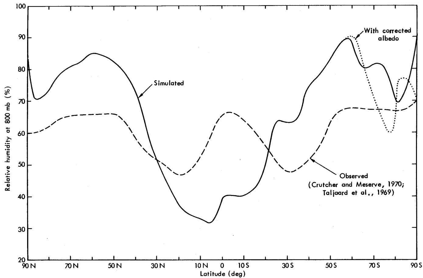
Fig. 33 -- The zonal average of the mean 800 mb relative humidity simulated for January (full line), with the corresponding observed distribution (dashed line), based on the data of Fig. 31.
