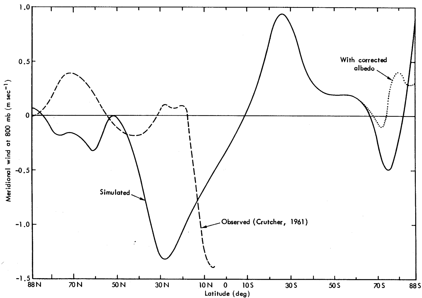
Fig. 28 -- The zonal average of the mean meridional winds at 800 mb simulated for January (full line), with the corresponding observed winds (dashed line) in the northern hemisphere. From Schutz and Gates (1971), based on data of Crutcher (1961).
