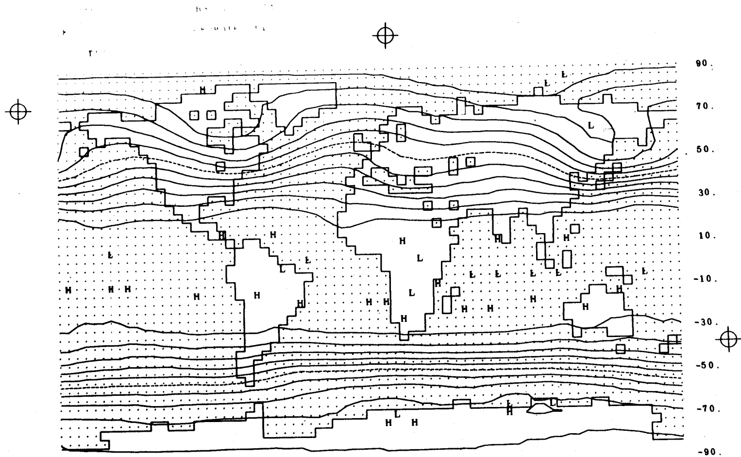
Fig. 10b -- The observed geopotential height at 400 mb for January, with isolines every 100 m and the 7000-m contour dashed. From Schutz and Gates (1971), based on data of Crutcher and Meserve (1970) and Taljaard et al. (1969).
