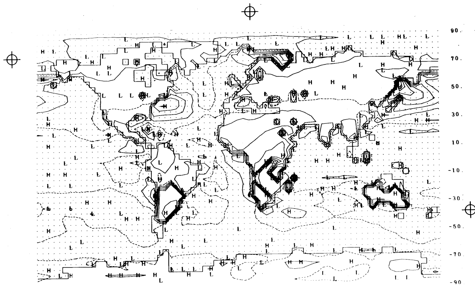
Fig. 44a -- The simulated sensible heat flux at the surface for January, with isolines at intervals of 100 \text{ ly day}^{-1} and the zero isoline dashed.
