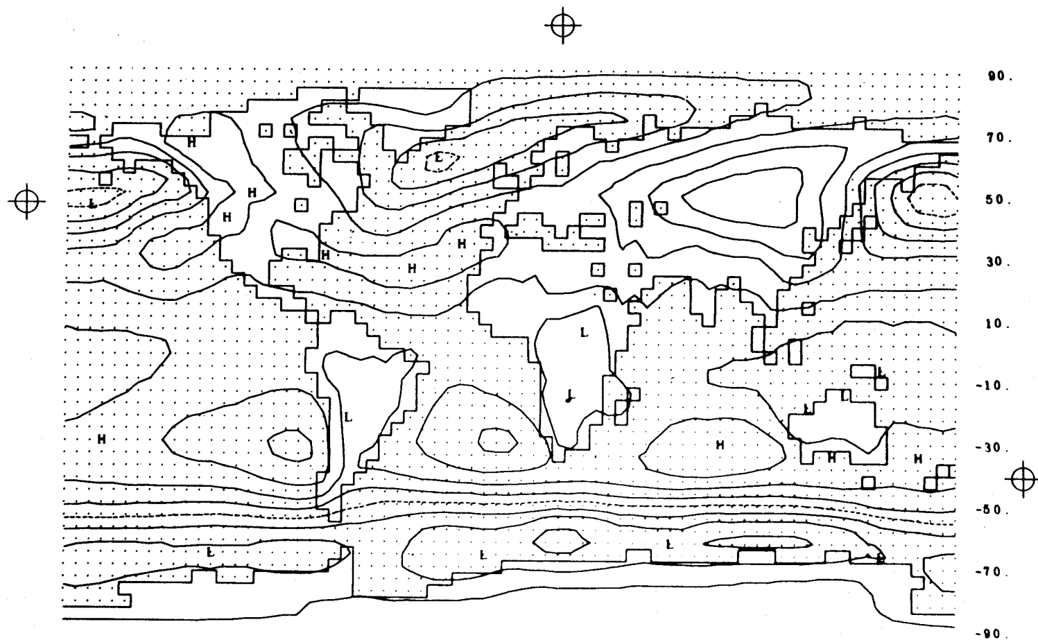
Fig. 4b -- The observed sea-level pressure with isolines every 5 mb and the 1000-mb isobar dashed. From Schutz and Gates (1971), based upon data of Crutcher and Meserve (1970) and Taljaard et al. (1969).
