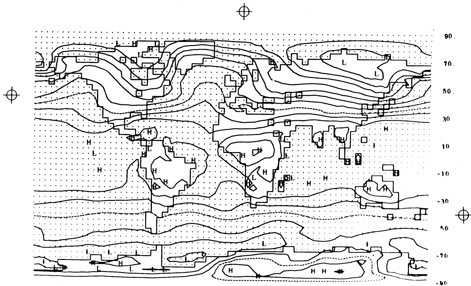
Fig. 16a -- The simulated temperature for January at 800 mb, with isolines at 5-deg C intervals and the 0-deg C isotherm dashed.
