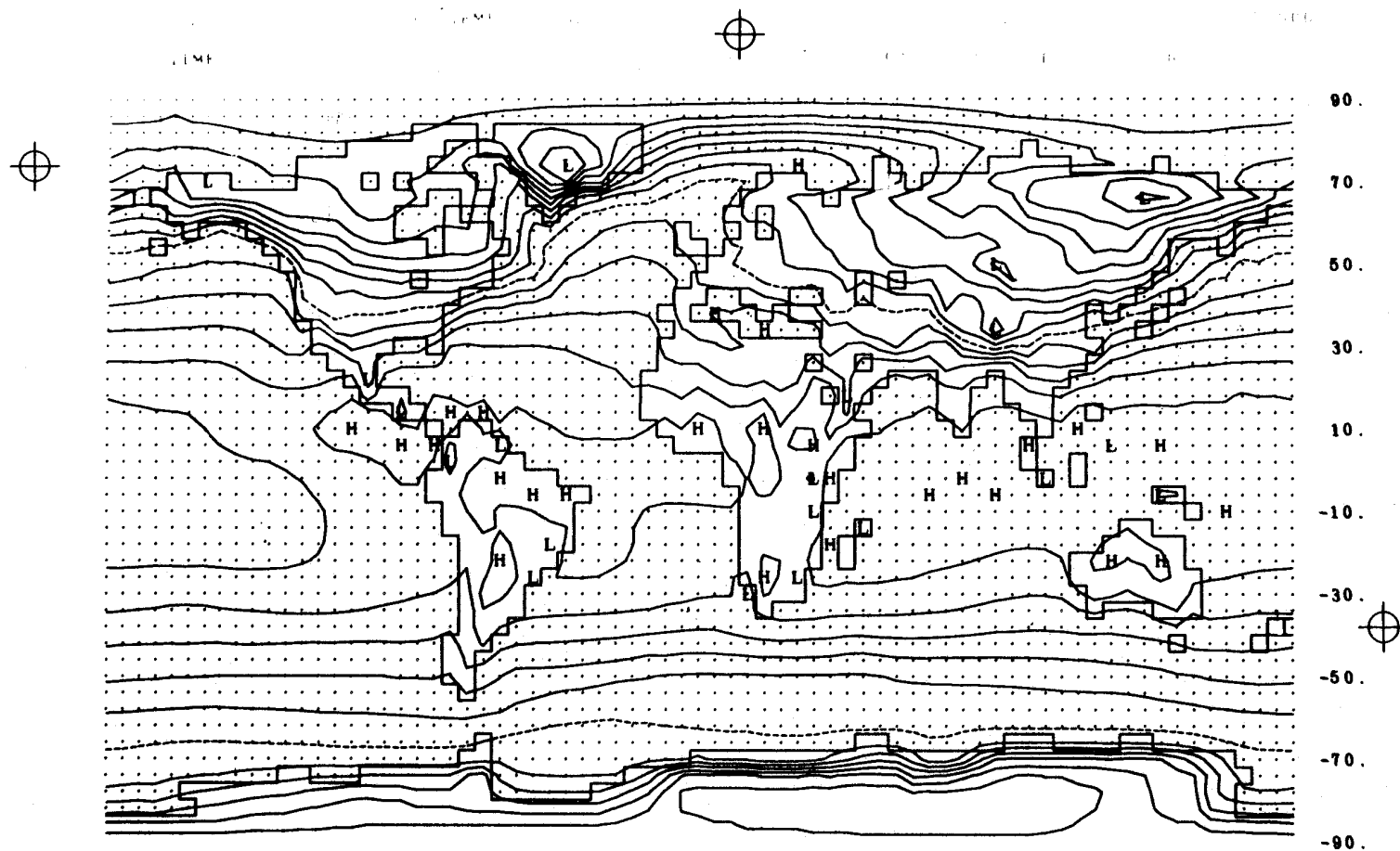
Fig. 13b -- The observed surface air temperature for January, with isolines at 5-deg C intervals and the 0 deg C isotherm dashed. From Schutz and Gates (1971), based on data of Crutcher and Meserve (1970) and Taljaard et al. (1969).
