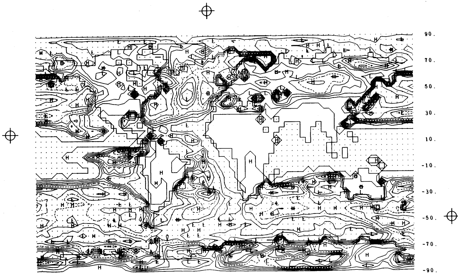
Fig. 34 -- The simulated total cloudiness for January, with isolines at 0.1-cloudiness intervals and the 0.5 isoline dashed.
