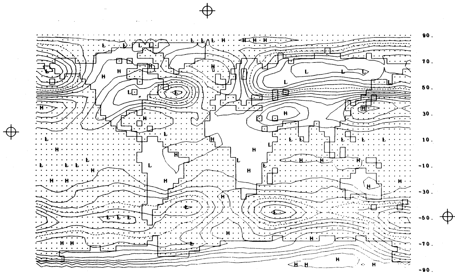
Fig. 11 -- The difference between the simulated and observed 400-mb geopotential height (Fig. 10a minus Fig. 10b). The isoline interval is 50 m with the 200-m line dashed.
