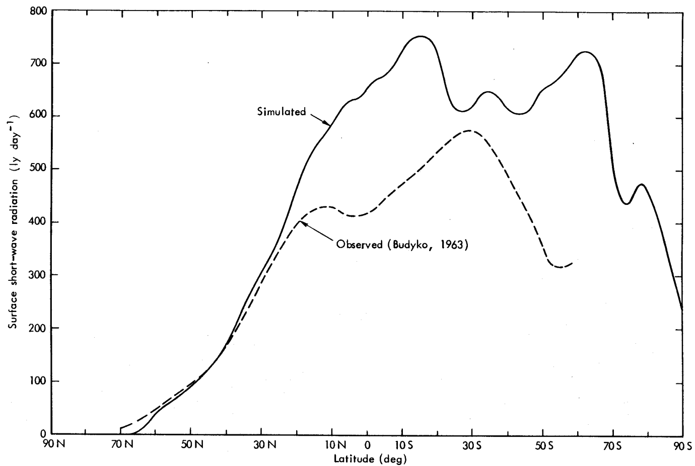
Fig. 49 -- The zonal average of the simulated shortwave radiation incident at the surface (full line) and that observed (dashed line), based on the data of Fig. 47.
