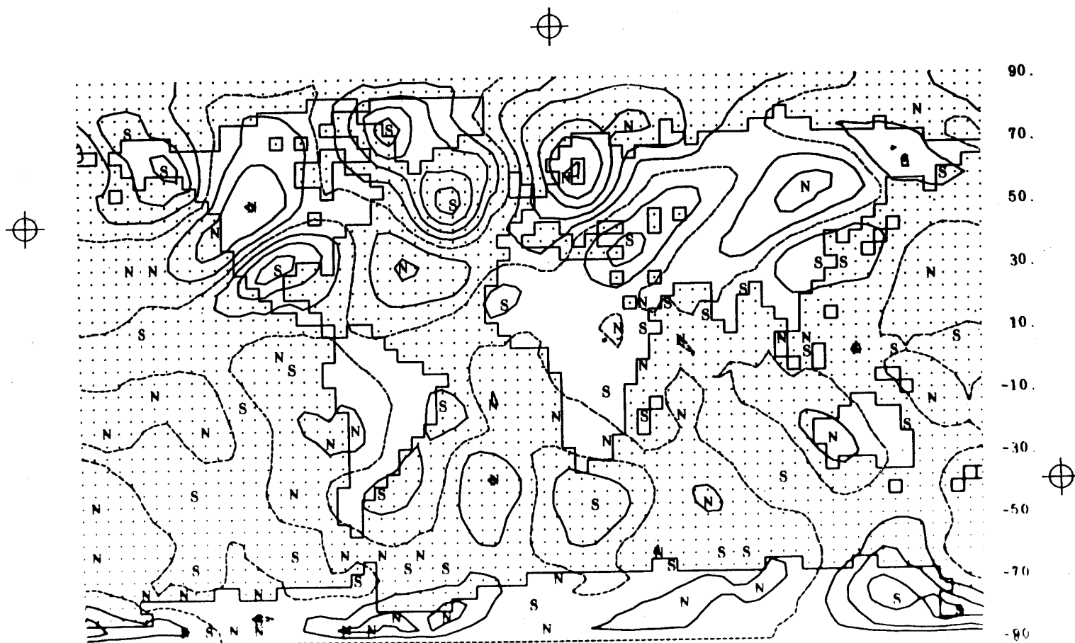
Fig. 27 -- The meridional wind at 400 mb simulated for January. See also Fig. 26.
