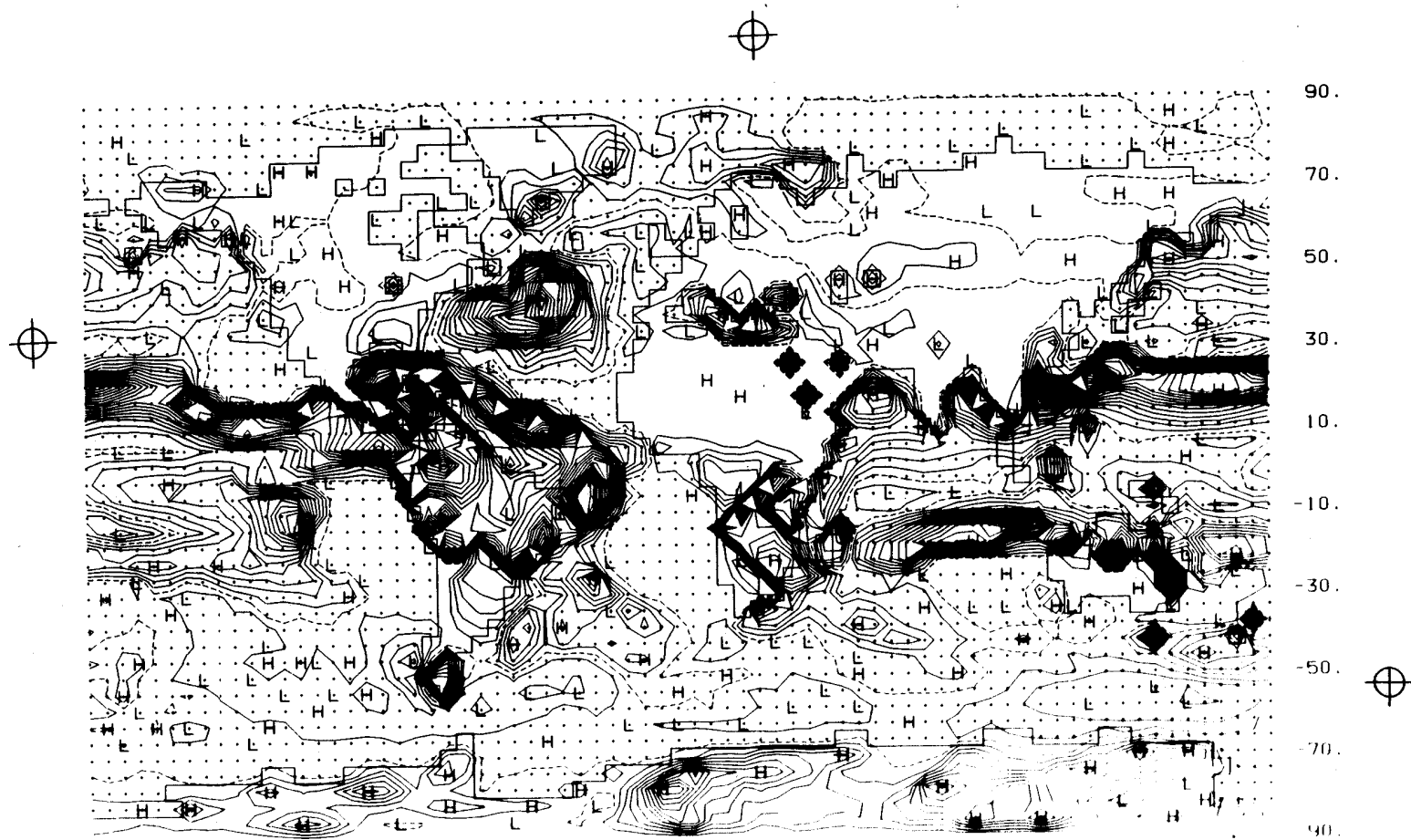
Fig. 38 -- The difference between the simulated and observed precipitation rate (Fig. 37a minus Fig. 37b). The isoline interval is 1 \text{ mm day}^{-1} with the zero isoline dashed.
