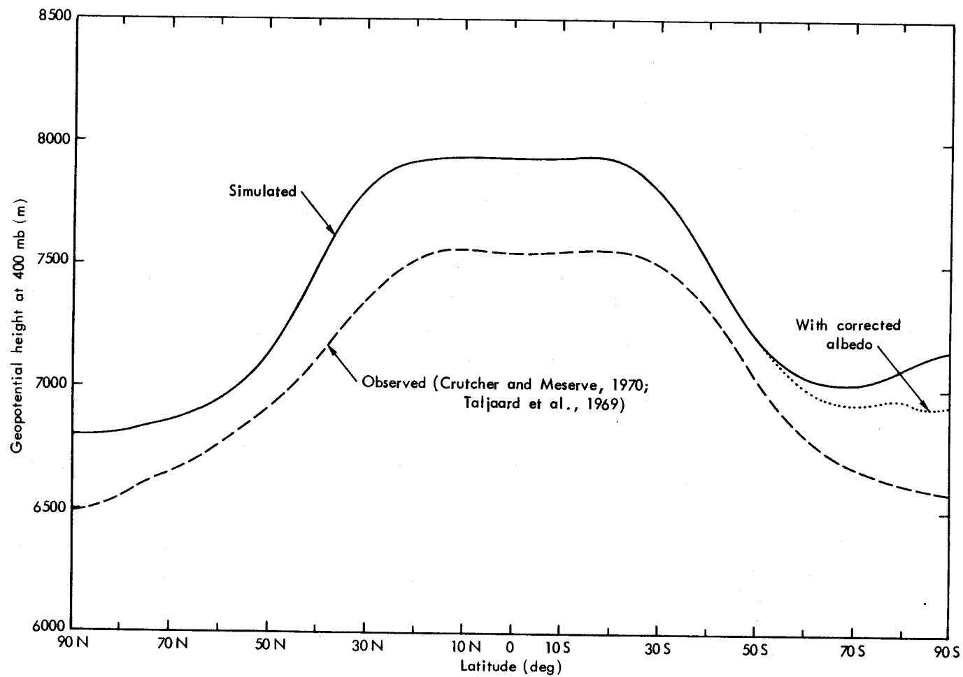
Fig. 12 -- The zonal average 400-mb geopotential height as simulated (full line) and as observed (dashed line), based on the data of Fig. 10.
