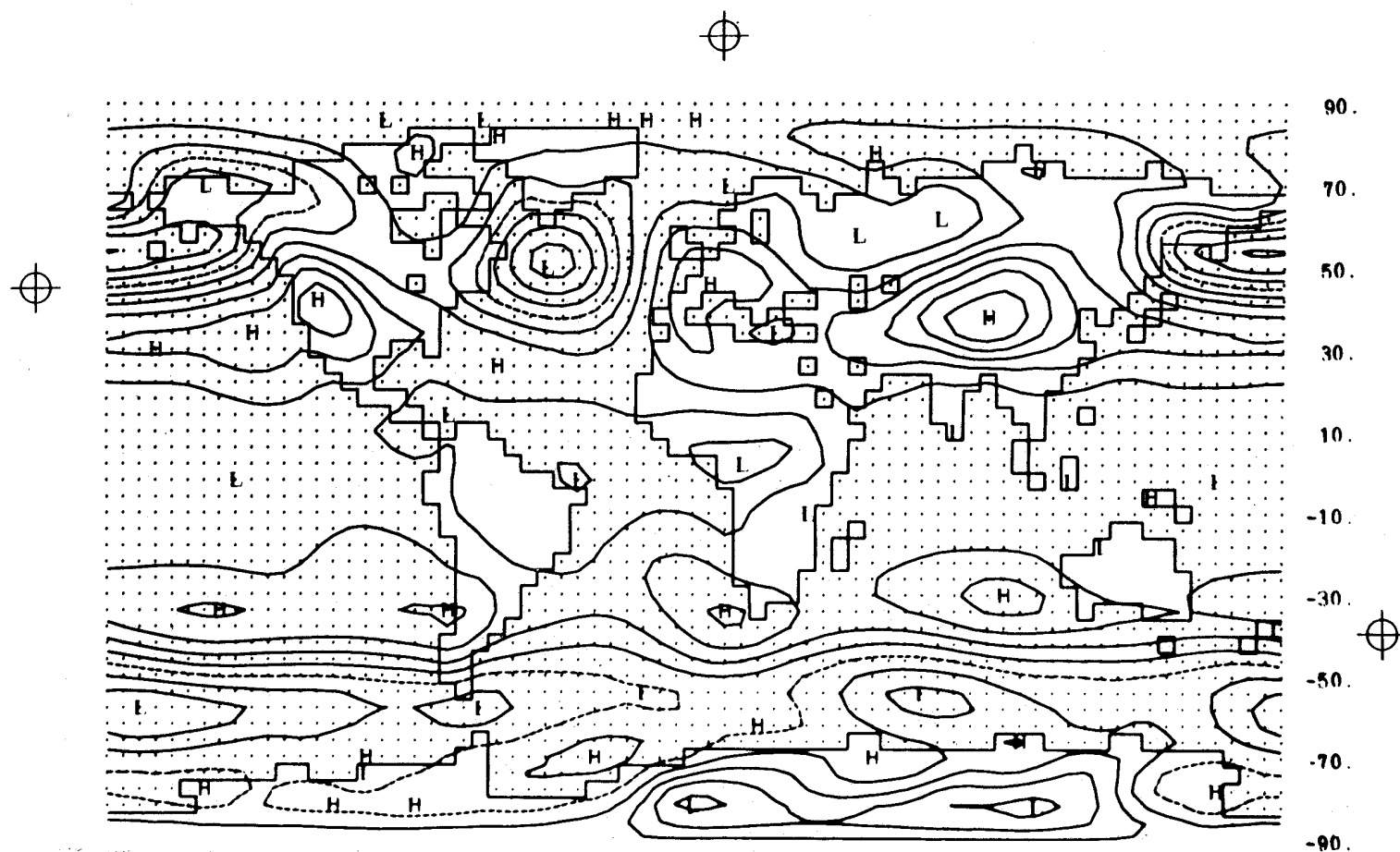
Fig. 4a -- The simulated sea-level pressure for January, with isolines every 5 mb and the 1000-mb isobar dashed. The symbols H and L denote local maxima and minima.
