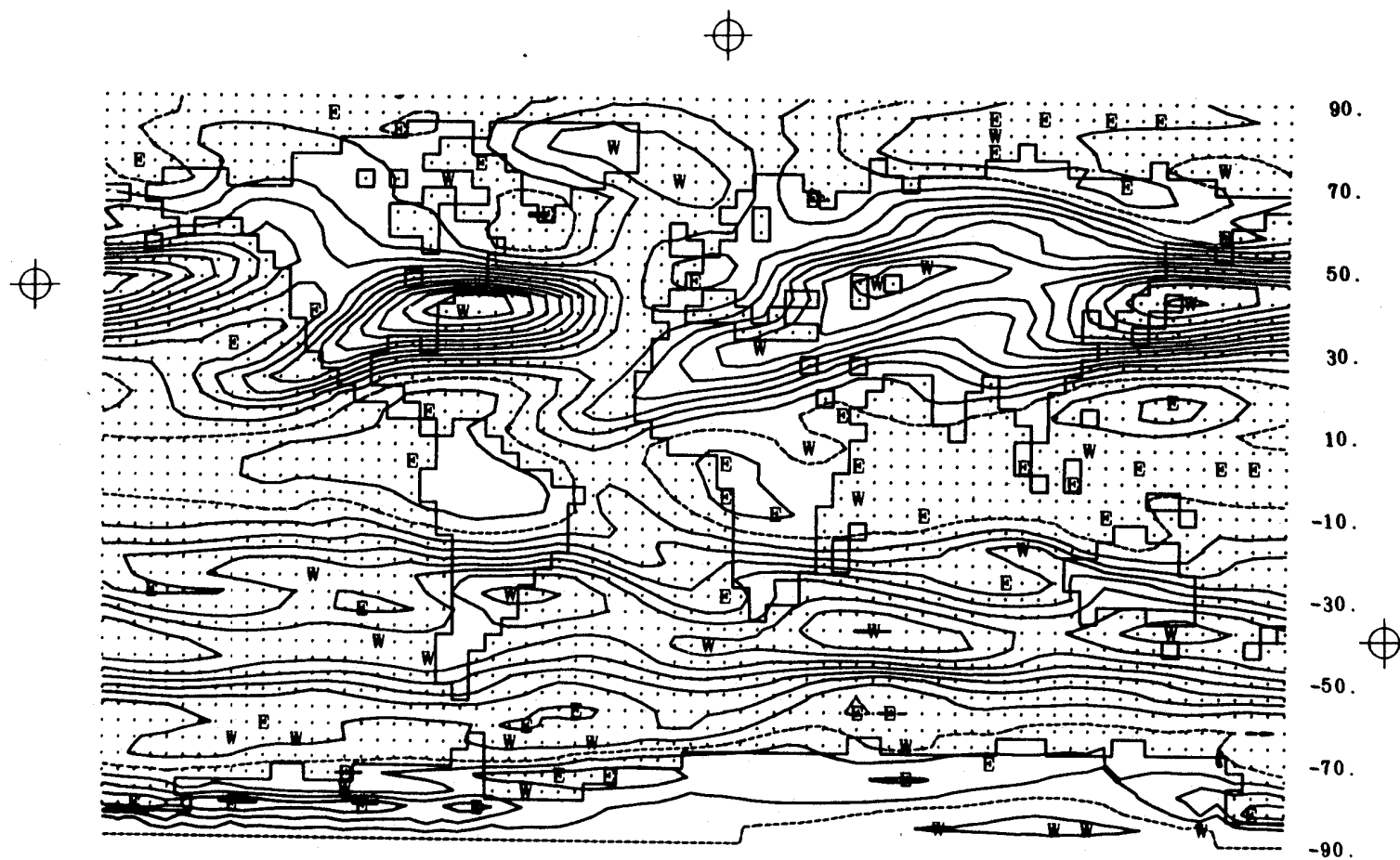
Fig. 23 -- The zonal wind at 400 mb simulated for January. See also Fig. 22.
