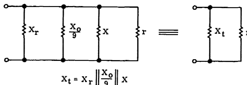
Figure 2-1. Total Junction Impedance.
