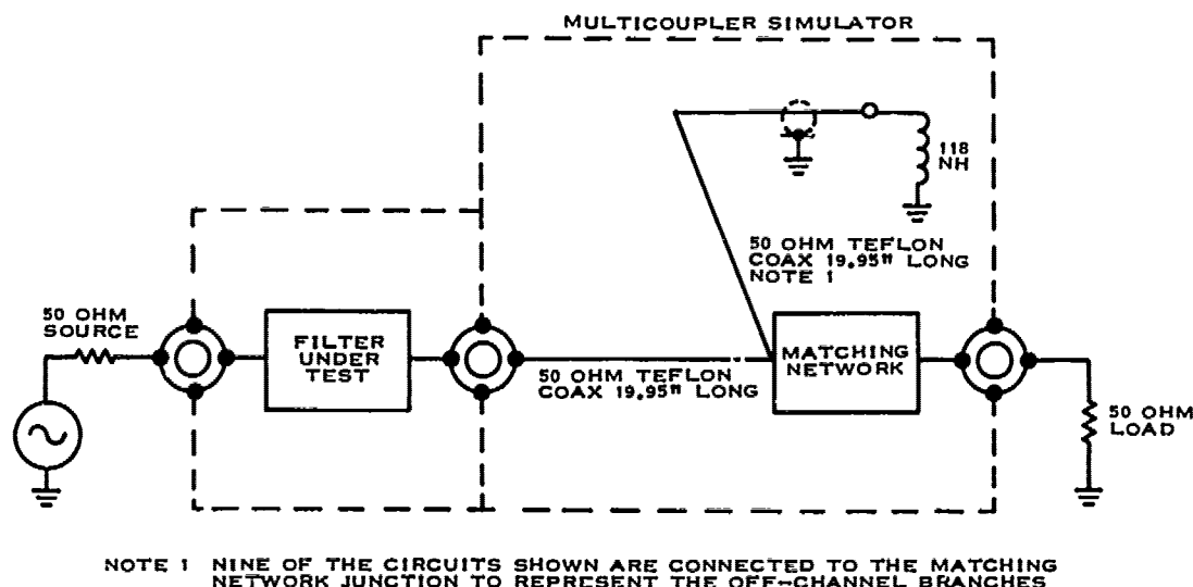
Figure 6-3. Multicoupler Simulator.
