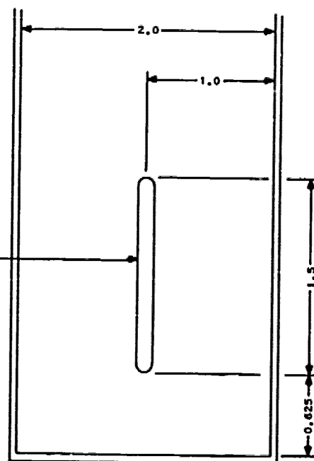
Figure 4-2. Measured Coupling Coefficient.
