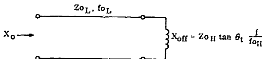
Figure 2-1. Total Junction Impedance.
