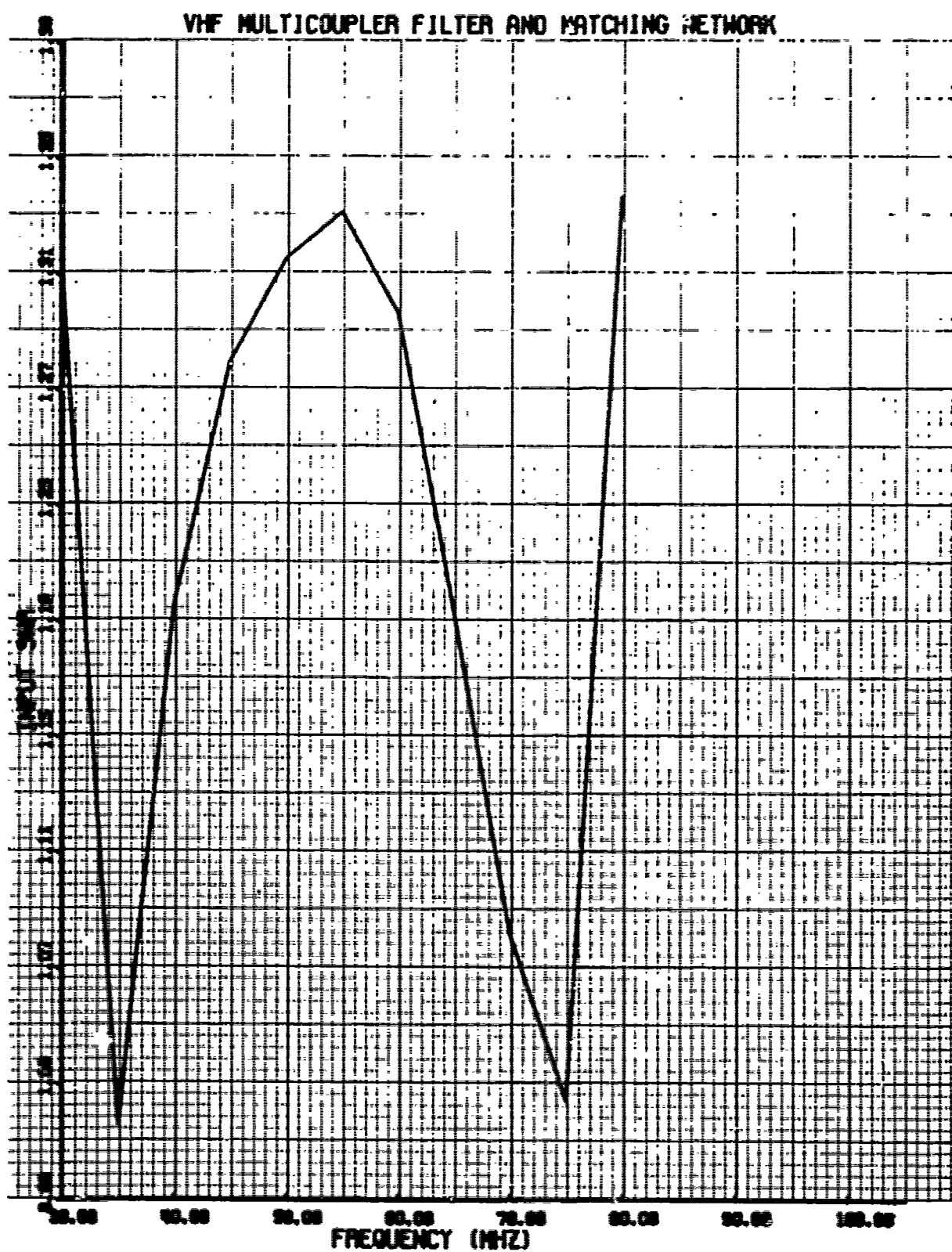
Figure 5-3. Input VSWR.
