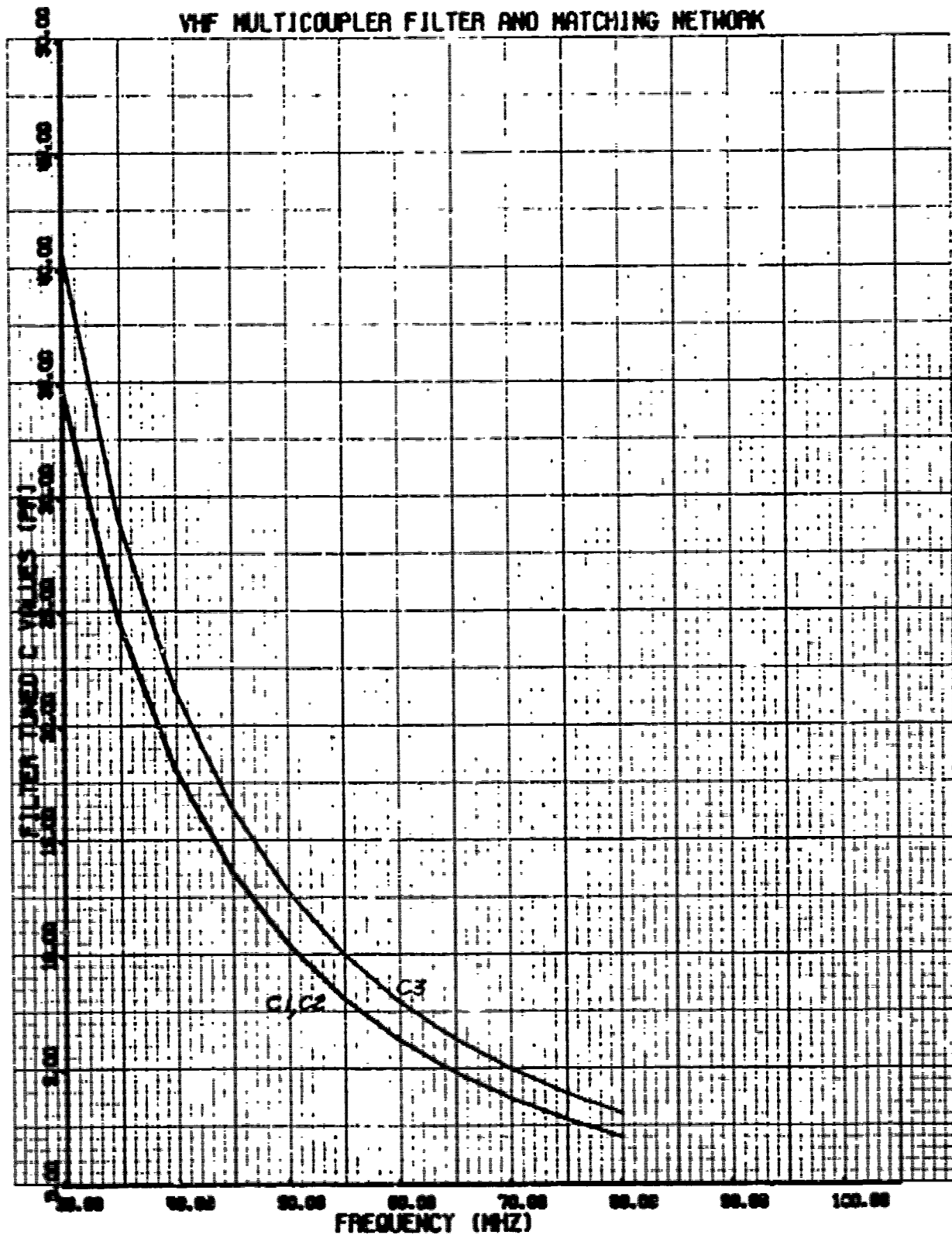
Figure 5-4. Tuning Capacitor Values.
