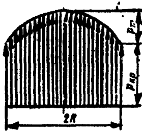
Fig. 15. The pressure diagram of compressed faces and mutually stationary annular rods.
