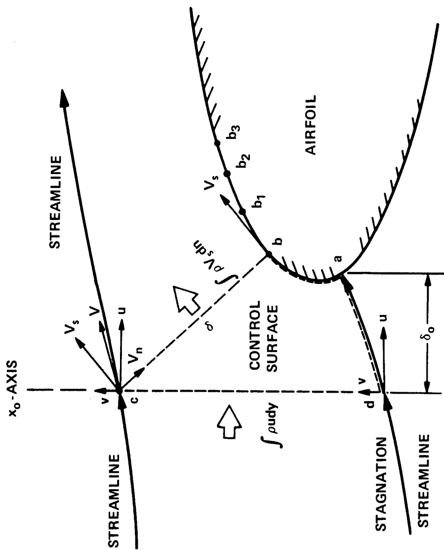
Figure 3 — A Control Surface in the Inner Stagnation Region
