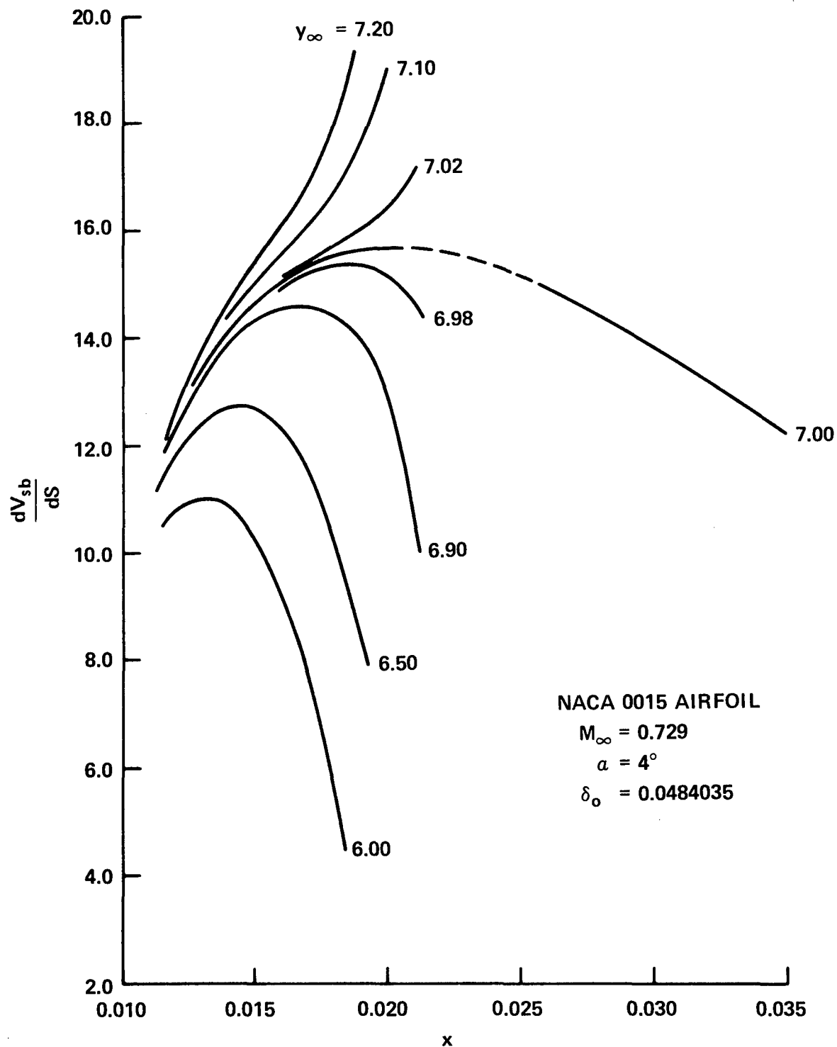
Figure 7a – Varying with Outermost Boundary Location
