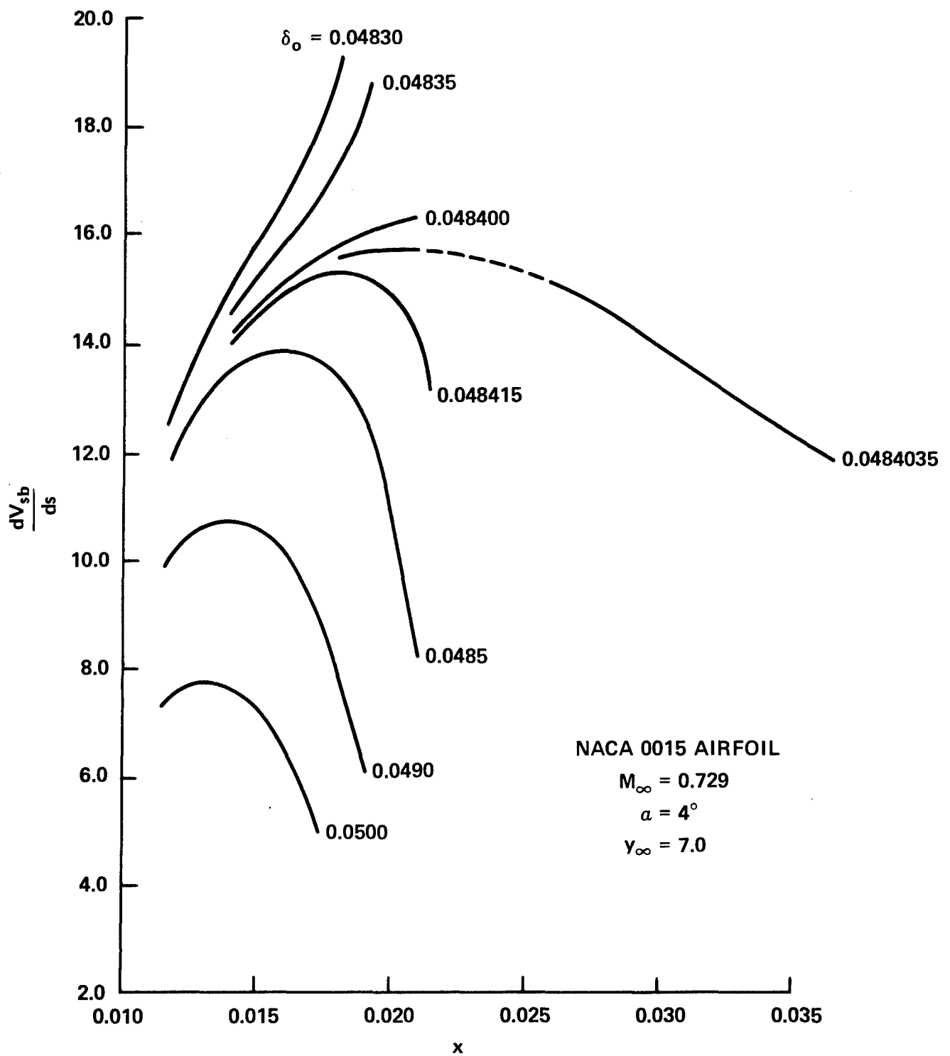
Figure 7b – Varying with Distance \delta_o
