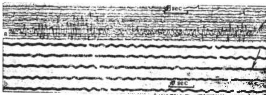
Fig. 3. Earthquake detected at 1357 hours, 15 February 1969; a - borehole, b - Alma-Ata Station seismogram. The arrows denote P-wave arrival.
