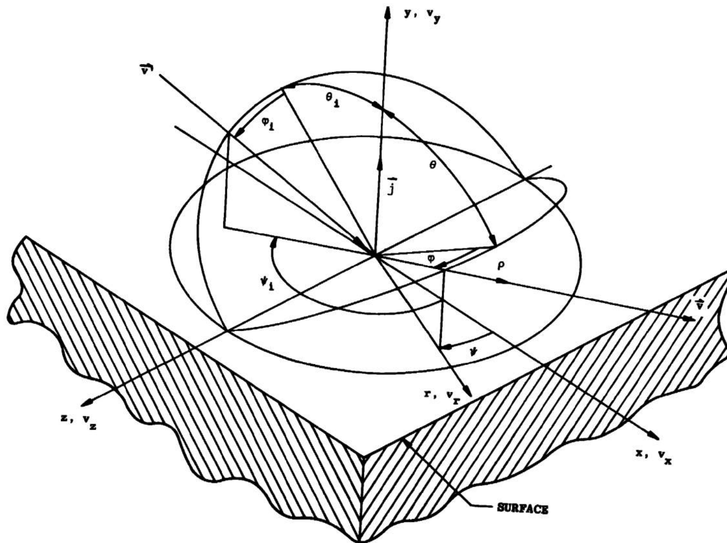
Figure 1. Coordinate Systems.
