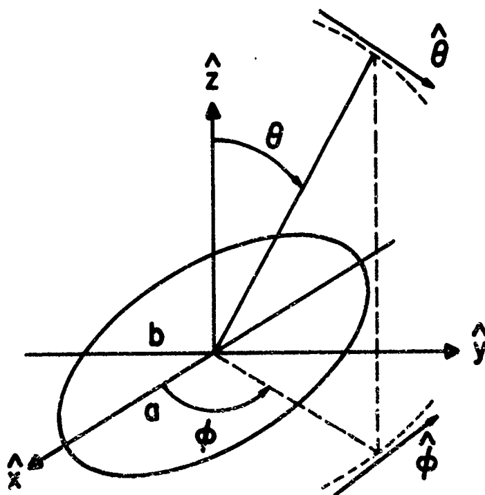
Figure 2.4. Geometry of an elliptical plate
