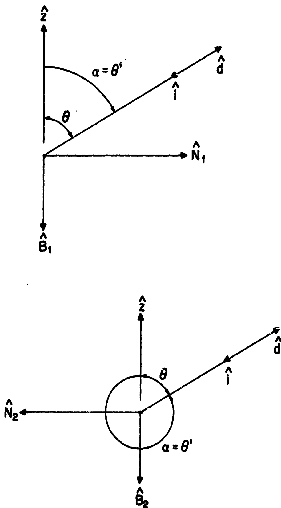
Figure 3.2. The diffraction angles for the elliptical plate
