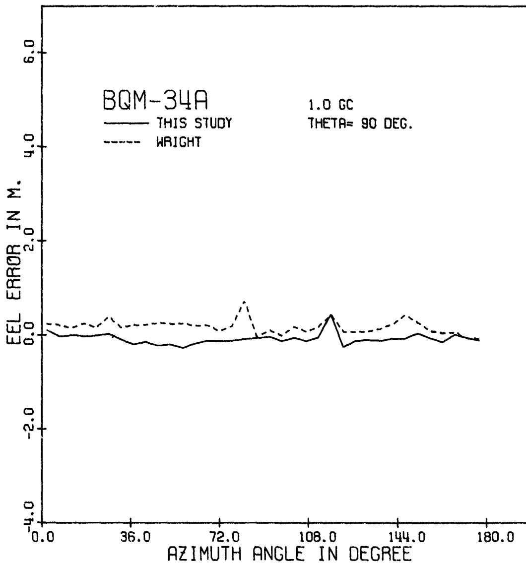
Figure 5.9. Elevation error ( e_e ) in meters of the BQM-34A drone as a function of azimuth angle \phi for a fixed \theta = 90^\circ , for a vertically polarized incident plane wave ( E_\theta = 0 ), and at frequency 1 GHz. The solid line represents the 5 0 -median computation of our model. The dotted line represents the 5 0 -median computation of Wright's model using ellipsoids.
