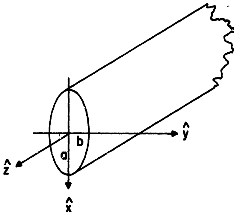
Figure 2.5. The open-end, hollow, semi-infinite elliptical cylinder
