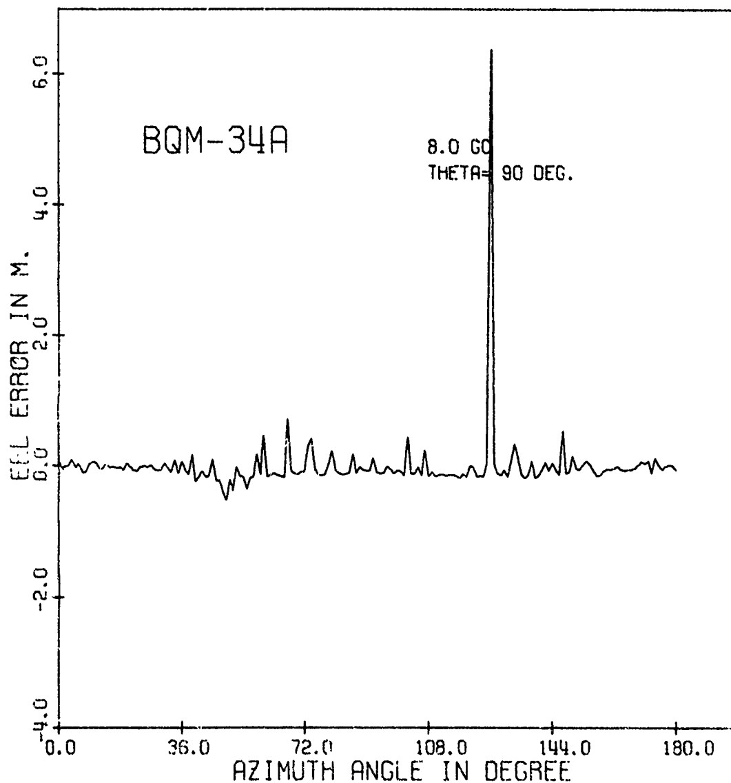
Figure 5.18. Elevation error ( e_e ) in meters of the BQM-34A drone as a function of azimuth angle \phi for a fixed \theta = 90^\circ , for a vertically polarized incident plane wave ( E_\theta = 0 ), and at frequency 8 GHz
