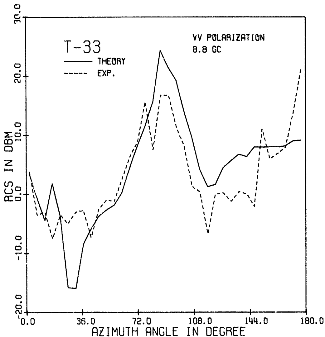
Figure 5.4. RCS in db per square meter of a full-scaled T-33 aircraft as a function of azimuth angle \phi for a tilt angle \psi = 5^\circ , for a vertically polarized incident plane wave ( E_\theta = 0 ), and at frequency 8.8 GHz. The solid line represents the 5^\circ -average of the theoretical computation. The dotted line represents the 5^\circ -median of the experiment reported in reference [33].
