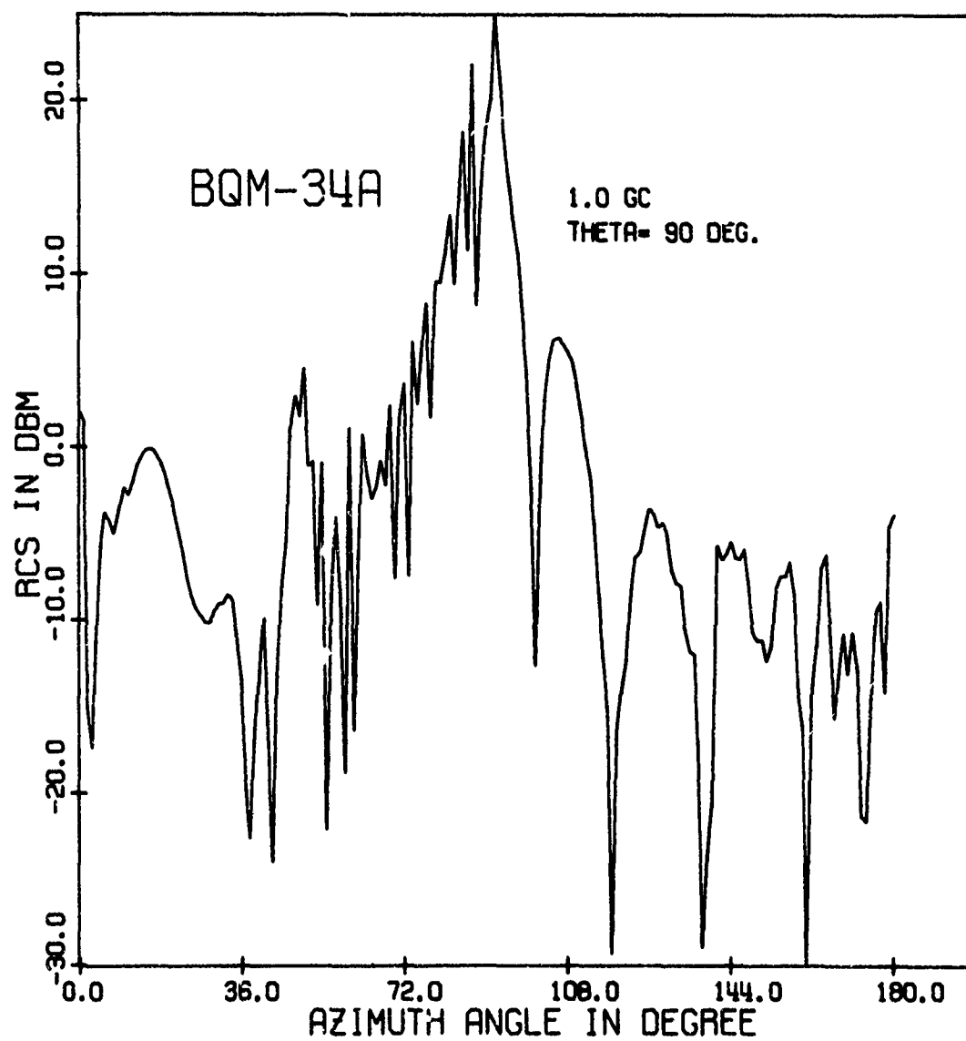
Figure 5.10. RCS in db per square meter of the BQM-34A drone as a function of azimuth angle \phi for a fixed \theta = 90^\circ , for a vertically polarized incident plane wave ( E_\theta = 0 ), and at frequency 1 GHz
