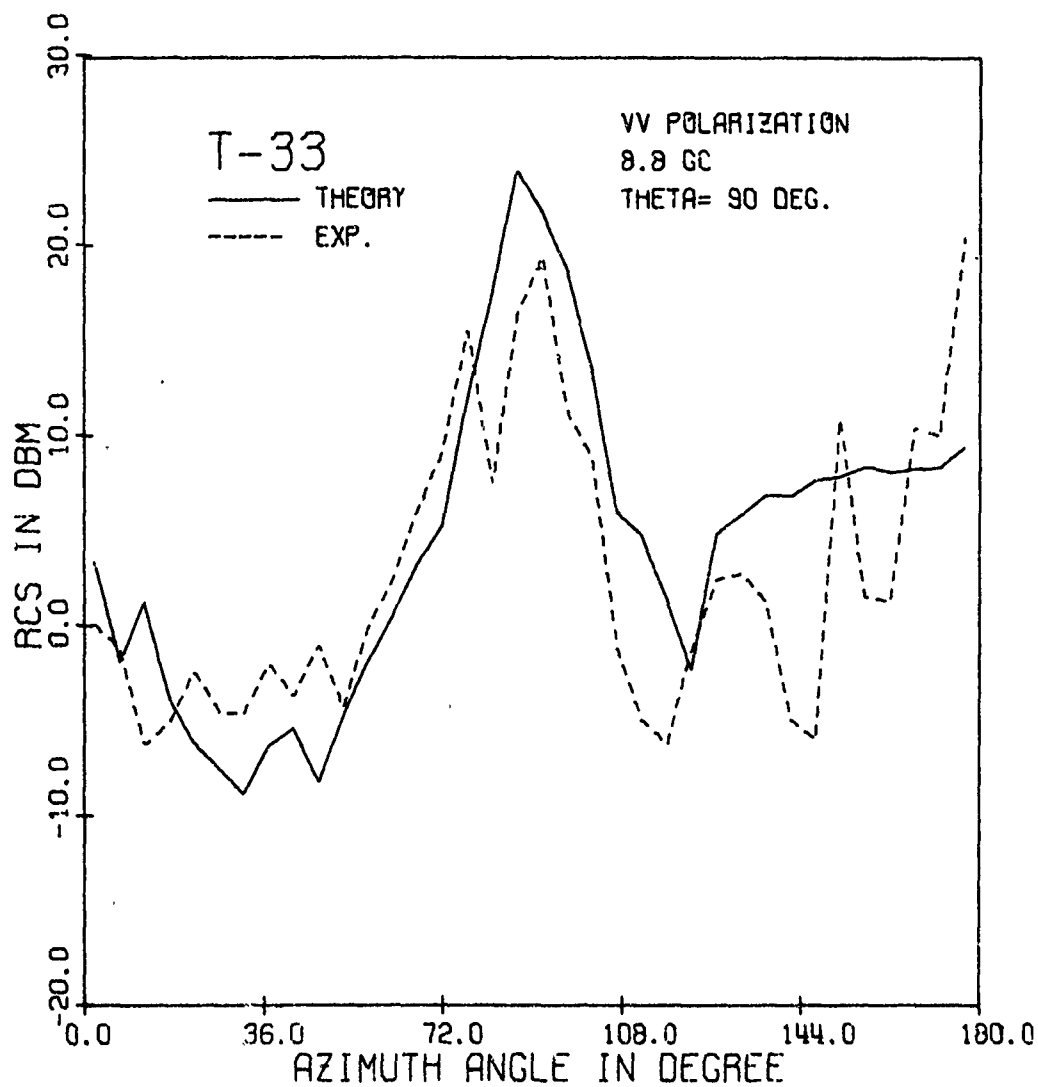
Figure 5.2. RCS in db per square meter of a full-scaled T-33 aircraft as a function of azimuth angle \phi for a fixed \theta = 90^\circ , for a vertically polarized incident plane wave ( E_\theta = 0 ), and at frequency 8.8 GHz. The solid line represents the 5^\circ -average of the theoretical computation. The dotted line represents the 5^\circ -median of the experiment reported in reference [33].
