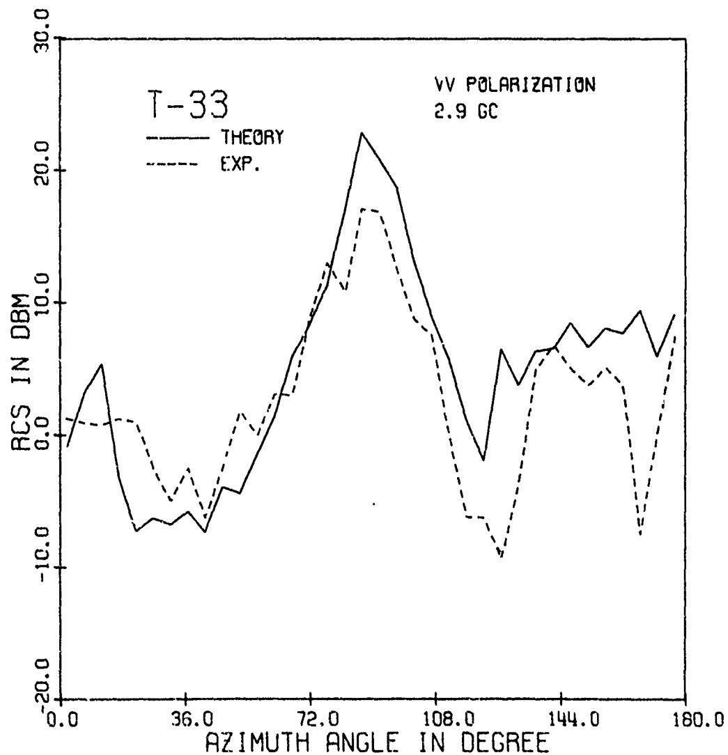
Figure 5.6. RCS in db per square meter of a full-scaled T-33 aircraft as a function of azimuth angle \phi for a tilt angle \psi = 10^\circ , for a vertically polarized incident plane wave ( E_\theta = 0 ), and at frequency 2.9 GHz. The solid line represents the 5^\circ -average of the theoretical computation. The dotted line represents the 5^\circ -median of the experiment reported in reference [33].
