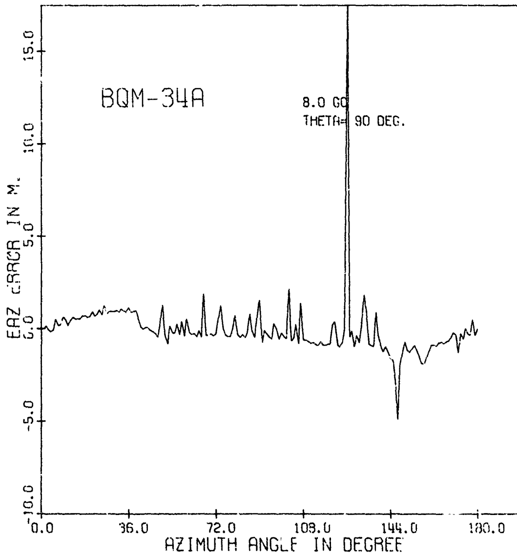
Figure 5.17. Azimuth error ( e_\phi ) in meters of the BQM-34A drone as a function of azimuth angle \phi for a fixed \theta = 90^\circ , for a vertically polarized incident plane wave ( E_\theta = 0 ), and at frequency 8 GHz
