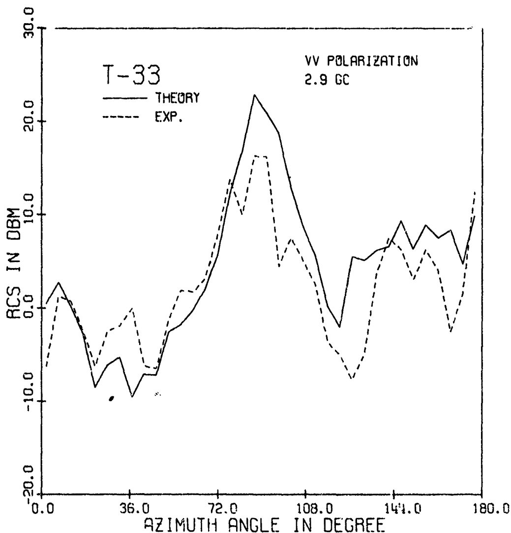
Figure 5.5. RCS in db per square meter of a full-scaled T-33 aircraft as a function of azimuth angle \phi for a tilt angle \psi = 5^\circ , for a vertically polarized incident plane wave ( E_\theta = 0 ), and at frequency 2.9 GHz. The solid line represents the 5^\circ -average of the theoretical computation. The dotted line represents the 5^\circ -median of the experiment reported in reference [33].
