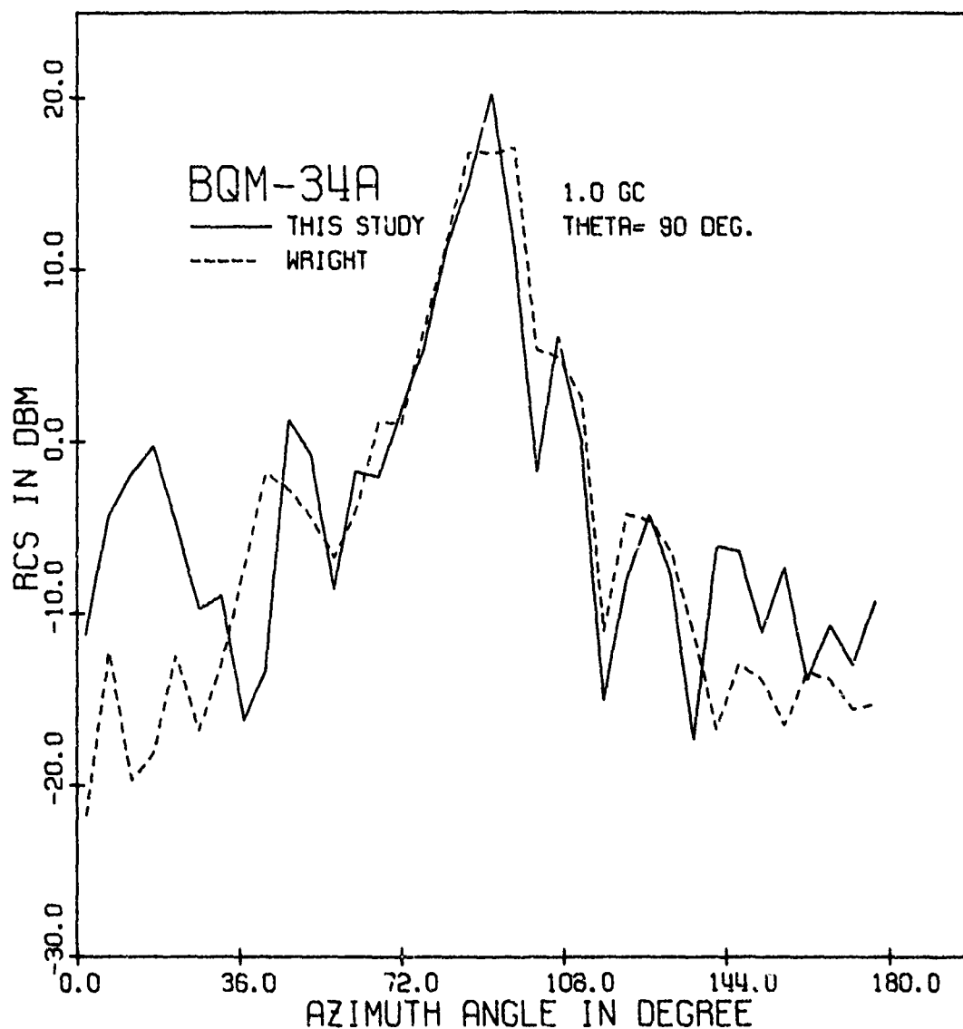
Figure 5.7. RCS in db per square meter of the BQM-34A drone as a function of azimuth angle \phi for a fixed \theta = 90^\circ , for a vertically polarized incident plane wave ( E_\theta = 0 ), and at frequency 1 GHz. The solid line represents the 5 0 -median computation of our model. The dotted line represents the 5 0 -median computation of Wright's model using ellipsoids.
