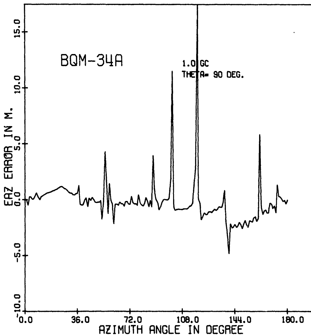
Figure 5.11. Azimuth error ( e_z ) in meters of the BQM-34A drone as a function of azimuth angle \phi for a fixed \theta = 90^\circ , for a vertically polarized incident plane wave ( E_\theta = 0 ), and at frequency 1 GHz
