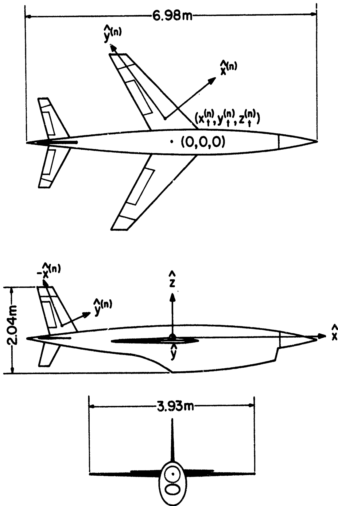
Figure 2.1. BQM-34A target drone
