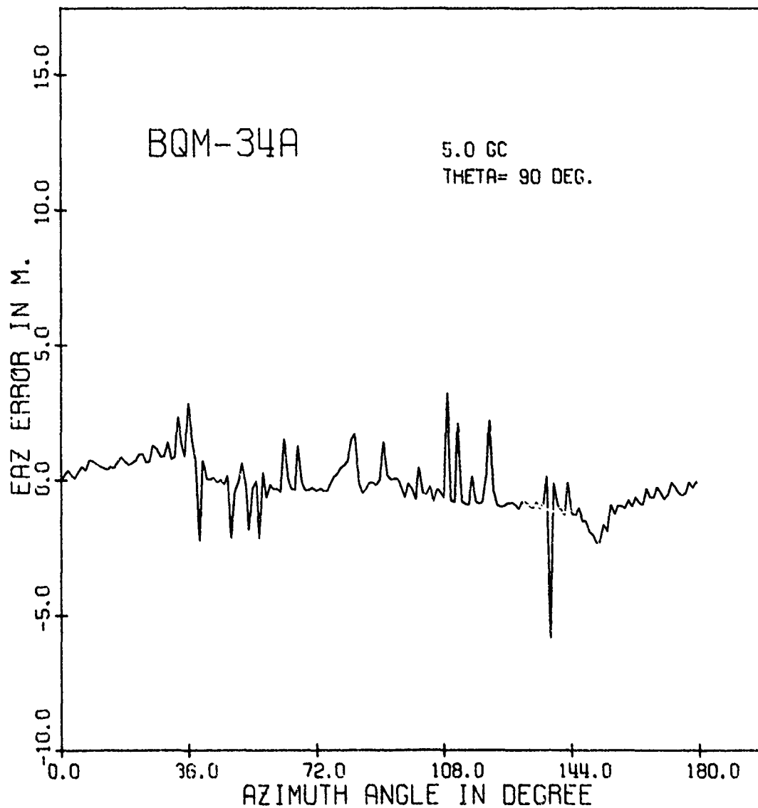
Figure 5.14. Azimuth error ( e_\phi ) in meters of the BQM-34A drone as a function of azimuth angle \phi for a fixed \theta = 90^\circ , for a vertically polarized incident plane wave ( E_\theta = 0 ), and at frequency 5 GHz
