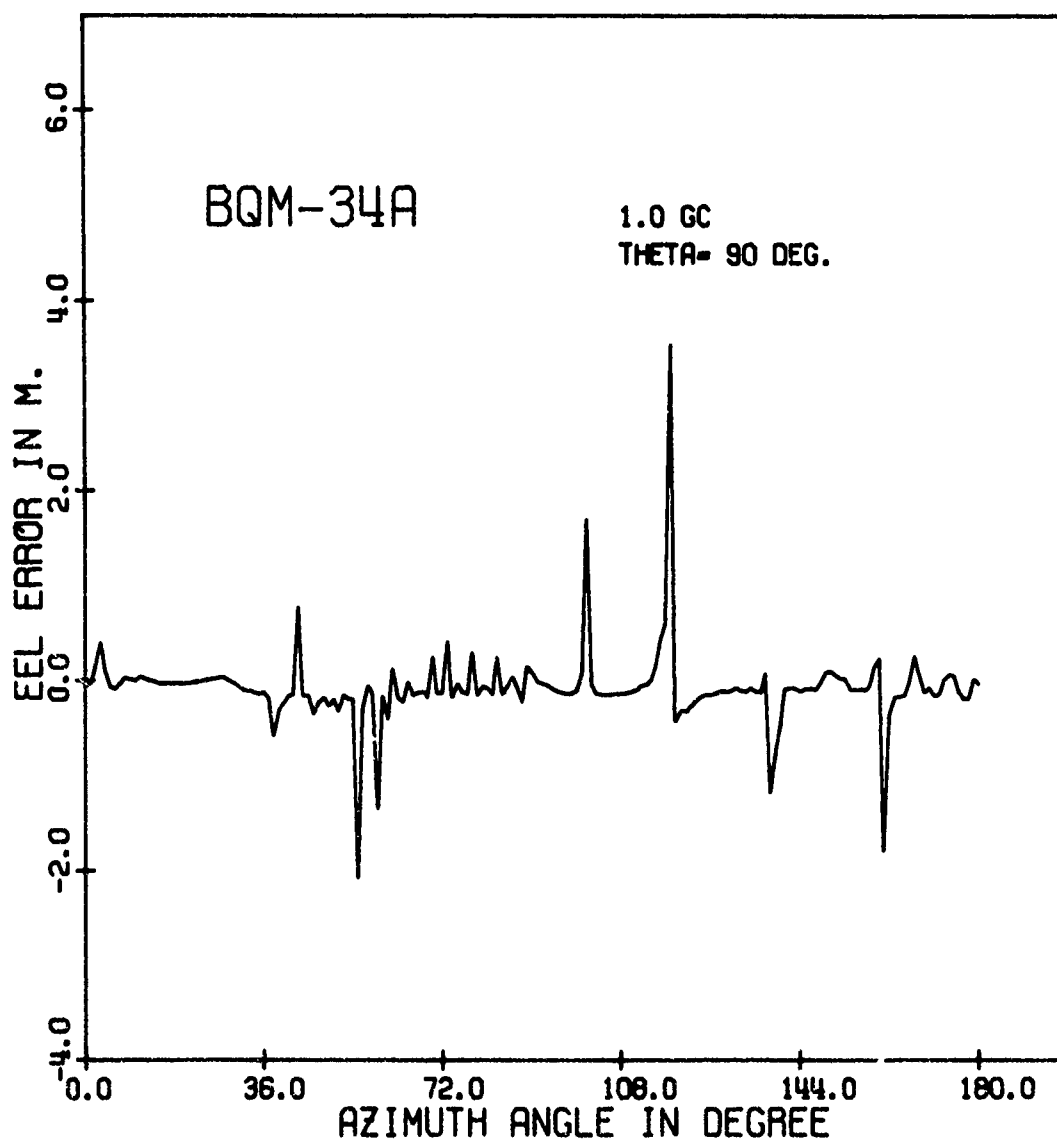
Figure 5.12. Elevation error ( e_e ) in meters of the BQM-34A drone as a function of azimuth angle \phi for a fixed \theta = 90^\circ , for a vertically polarized incident plane wave ( E_\theta = 0 ), and at frequency 1 GHz
