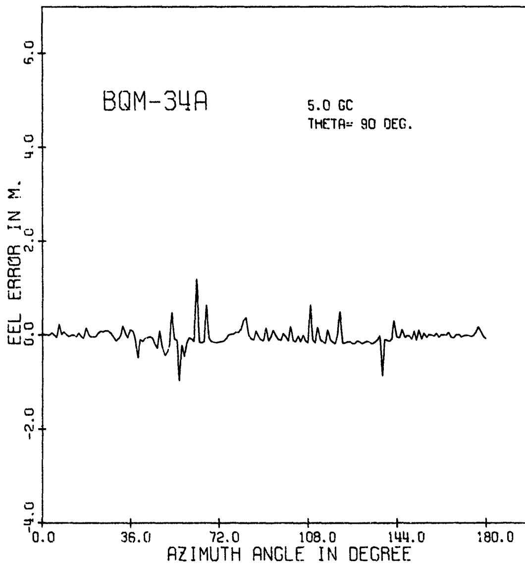
Figure 5.15. Elevation error ( e_\theta ) in meters of the BQM-34A drone as a function of azimuth angle \phi and a fixed \theta = 90^\circ , for a vertically polarized incident plane wave ( E_\theta = 0 ), and at frequency 5 GHz
