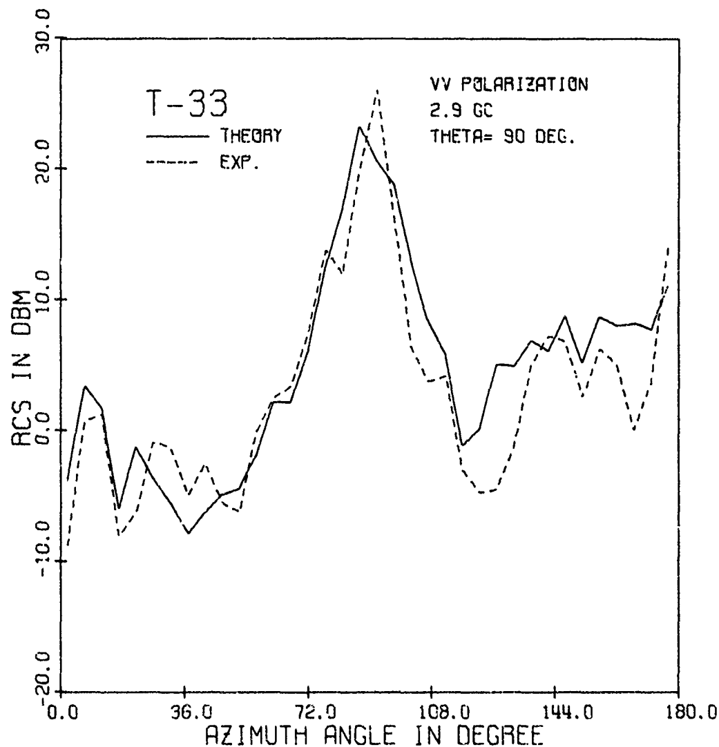
Figure 5.3. RCS in db per square meter of a full-scaled T-33 aircraft as a function of azimuth angle \phi for a fixed \theta = 90^\circ , for a vertically polarized incident plane wave ( E_\theta = 0 ), and at frequency 2.9 GHz. The solid line represents the 5^\circ -average of the theoretical computation. The dotted line represents the 5^\circ -median of the experiment reported in reference [33].
