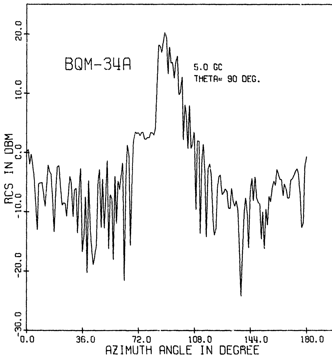
Figure 5.13. RCS in db per square meters of the BQM-34A drone as a function of azimuth angle \phi and a fixed \theta = 90^\circ , for a vertically polarized incident plane wave ( E_\theta = 0 ), and at frequency 5 GHz
