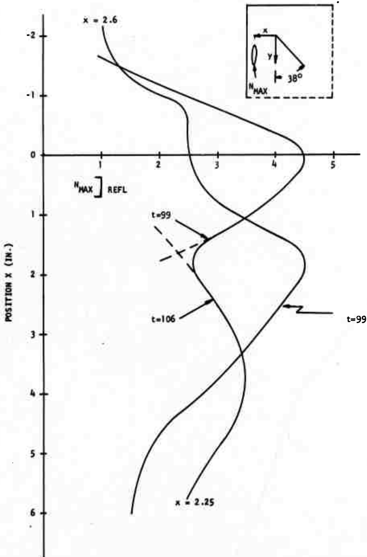
Fig. 4.15 Maximum Fringe Order Associated with Reflected PP and PS Waves
