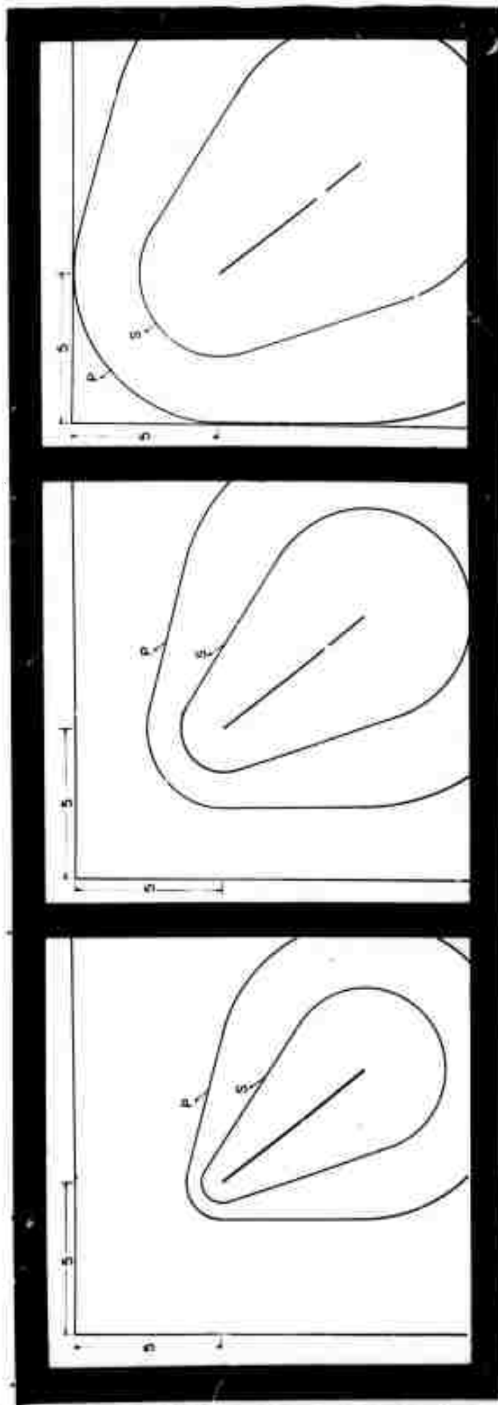
(a) t=70 (b) t=90 (c) t=124 Fig 3.2 Wave Front Diagram at Three Different Times During the Incident Phase of the Dynamic Event
