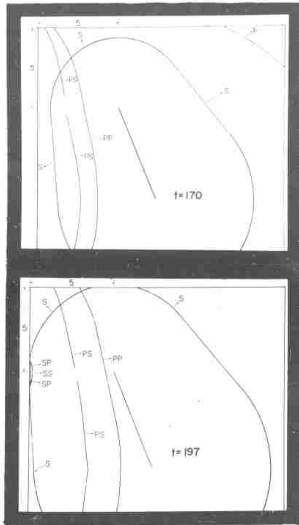
Fig. 3.9 Wave Front Diagrams for the Final Stage of Interaction and the Initiation of the S Wave Reflection
