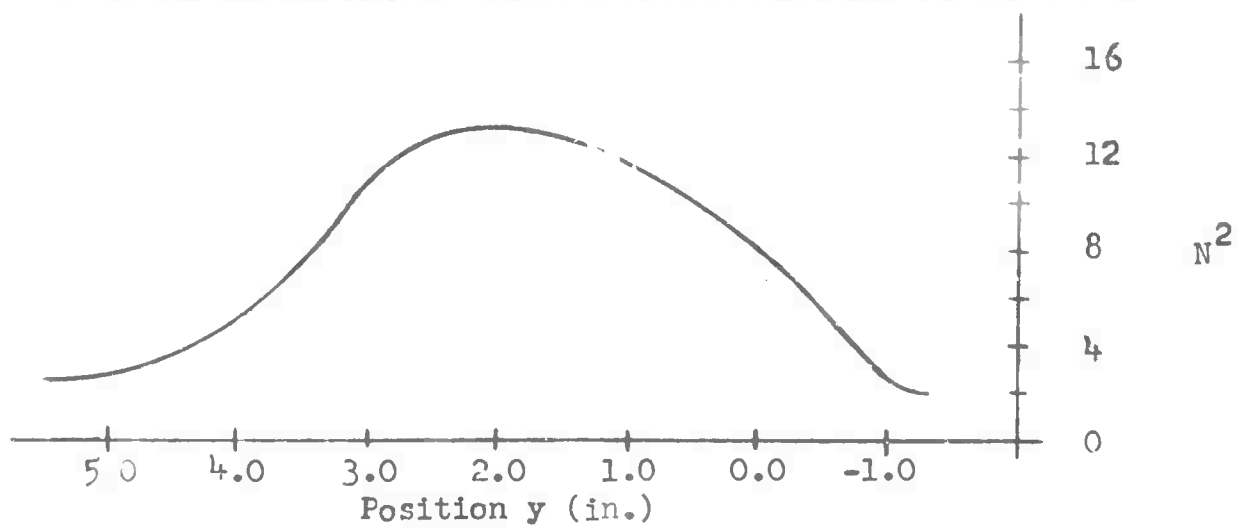
Fig. 4.35 Energy Distribution in Reflected Shear Wave
