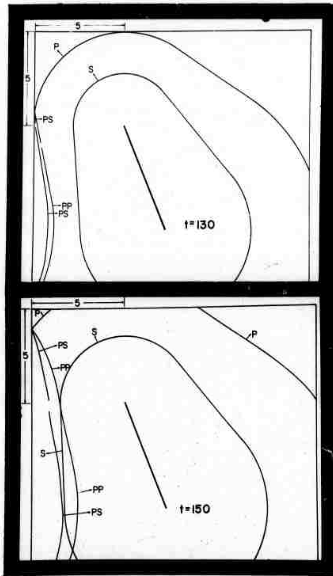
Fig 3.8 Wave Front Diagrams Associated with the Reflecting P Wave and the Interaction of the PP and PS Waves with the Incident S Wave
