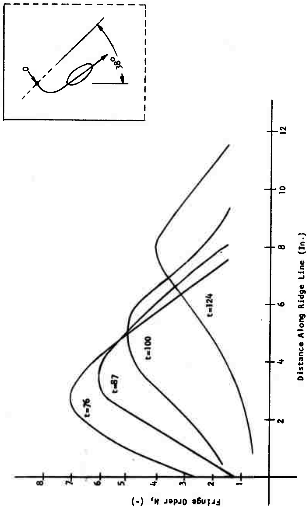
Fig. 4.8 Fringe Order as a Function of Position along the Ridge Line of the S Wave
