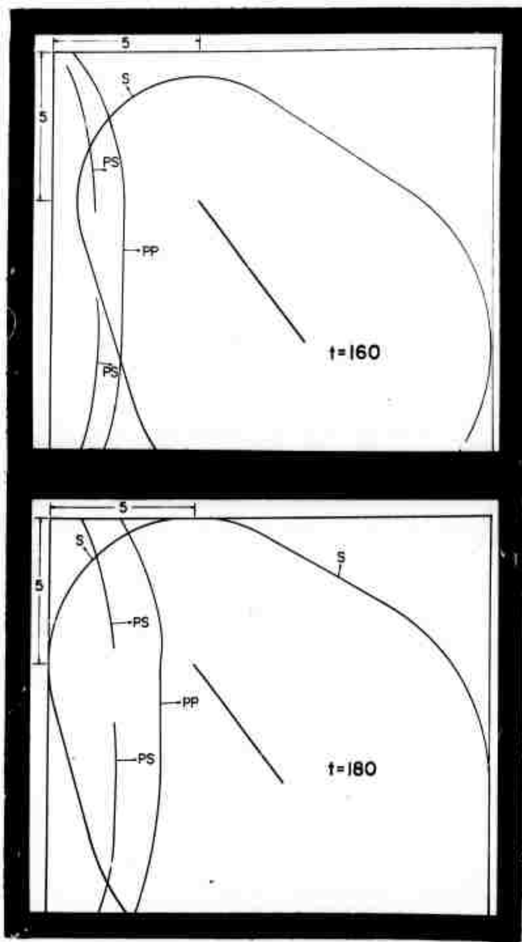
Fig. 3.4 Wave Front Diagrams During the Interaction Phase
