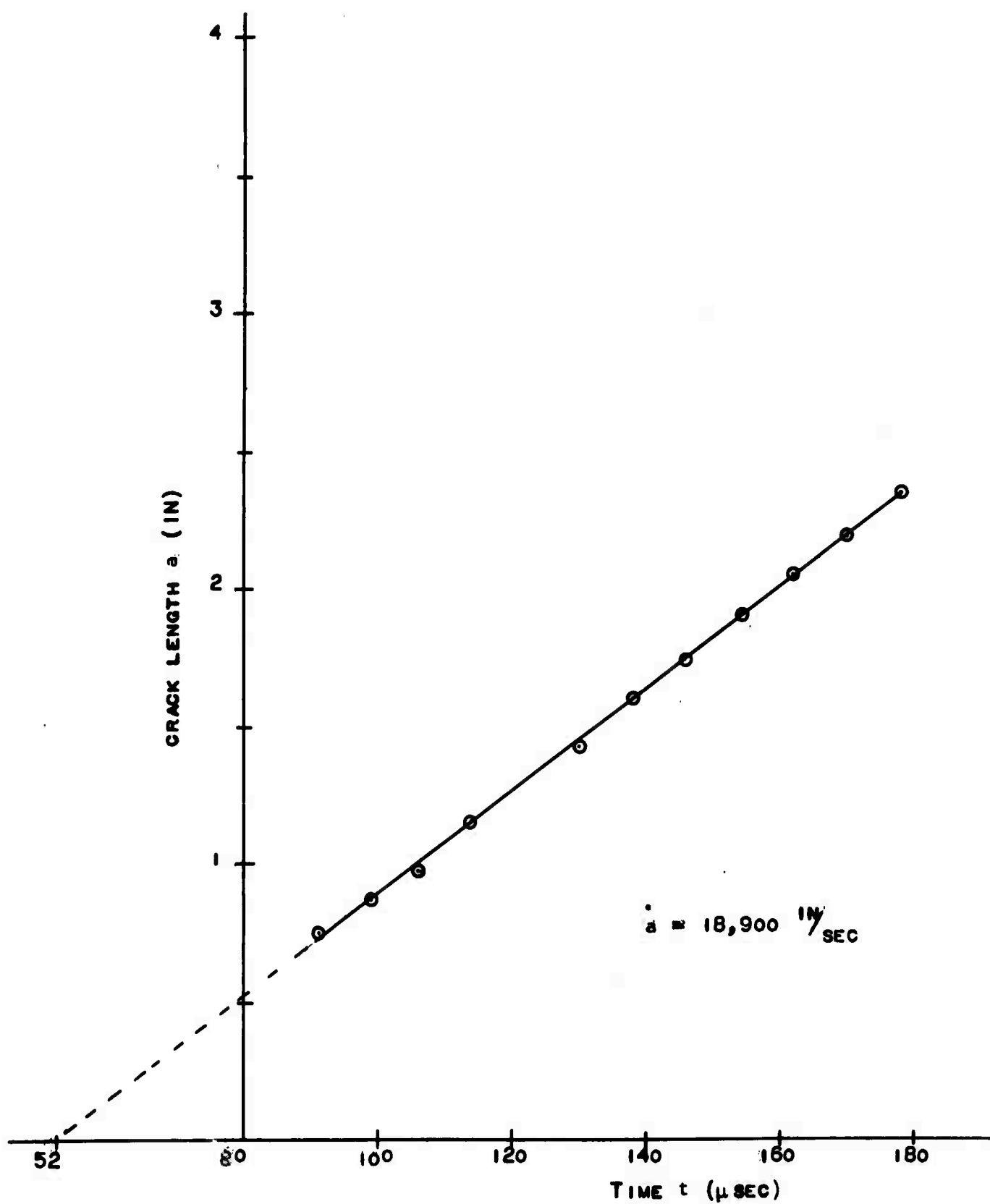
Fig. 4.19 Crack Length as a Function of Time
