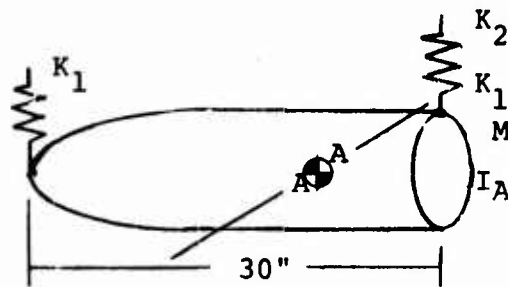
RIGID INERTIAL MASS SUBSYSTEM
