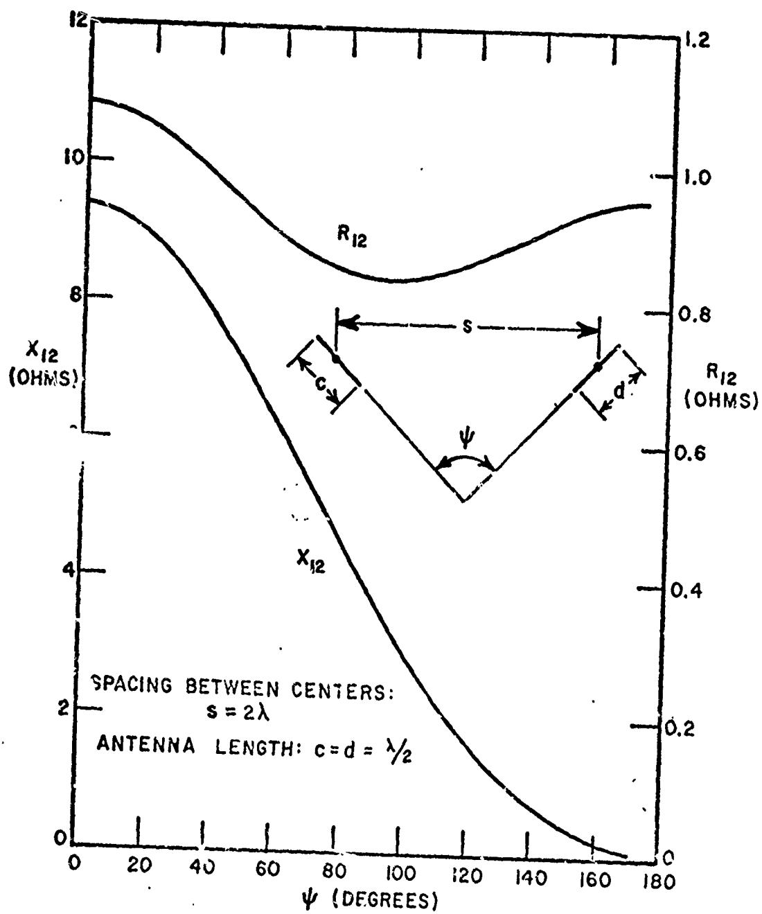
Fig. 3. Mutual impedance between coplanar-sleeve dipoles.
