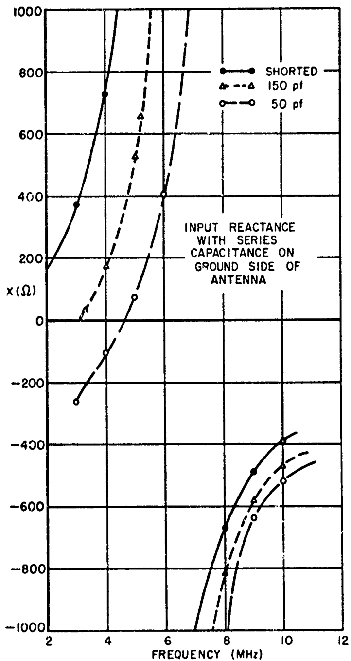
Fig. 12(b). Input reactance showing effect of capacitor between multitrurn loop and ground (Shreve).
