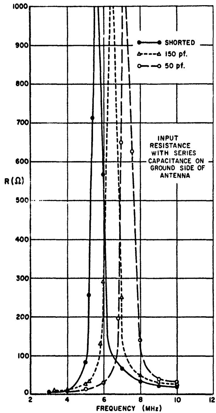
Fig. 12(a). Input resistance showing effect of capacitor between multitrurn loop and ground (Shreve).
