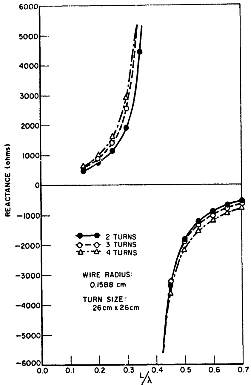
Fig. 5(b). Input reactance near first antiresonance: Square loops of two, three, and four turns (turn spacing = 4 cm, same turn size).
