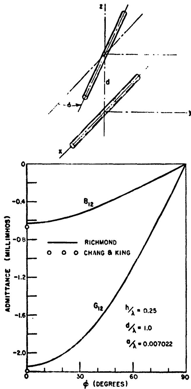
Fig. 7. Mutual admittance vs. rotation angle for half-wave nonplanar-skew antennas.
