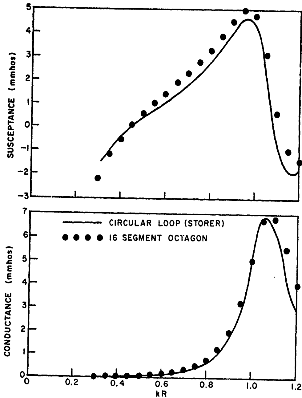
Fig. 3. A comparison of input conductances and susceptances for a planar octagonal loop and a circular loop of equal area. The horizontal scale is the circumference of the circle in wavelengths.
