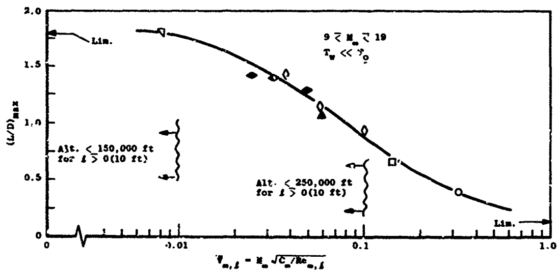
Fig. 9 Lift-to-Drag Ratio of a Slightly Blunted 9-deg Semiangle Cone (Ref. 23)
