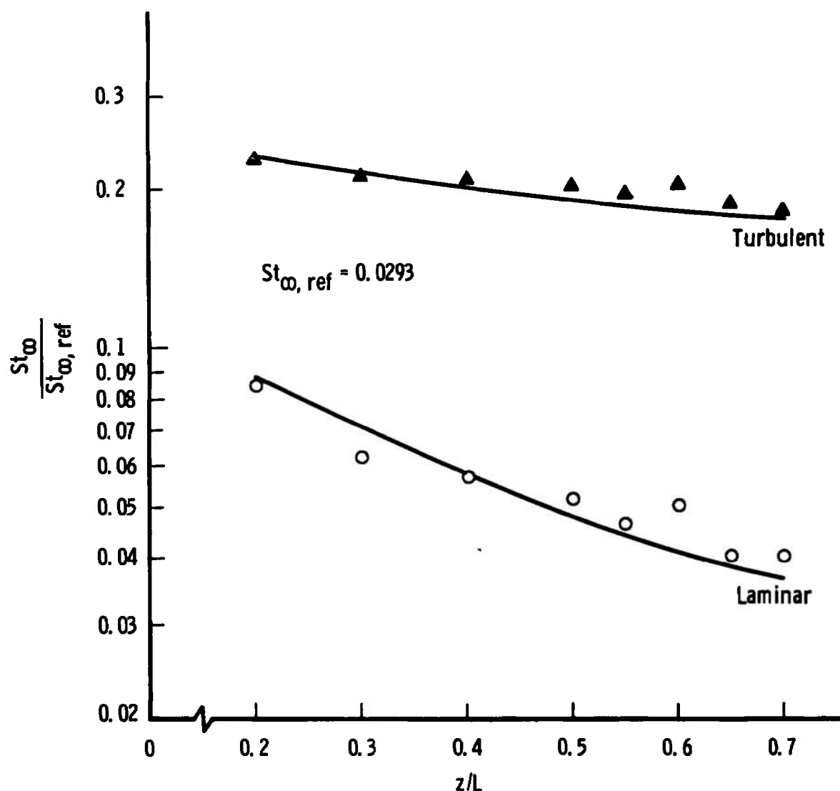
Fig. 30 Windward Centerline Stanton Number Distributions on the NAR Orbiter under AEDC-VKF Tunnel B Conditions
