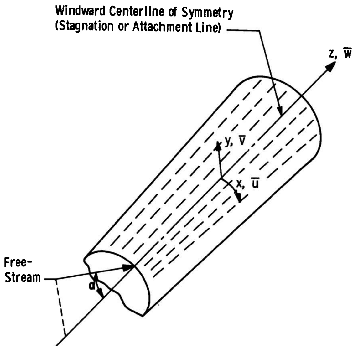
Fig. 1 Windward Surface Orthogonal Coordinate System for General Lifting Body Configurations at Incidence
