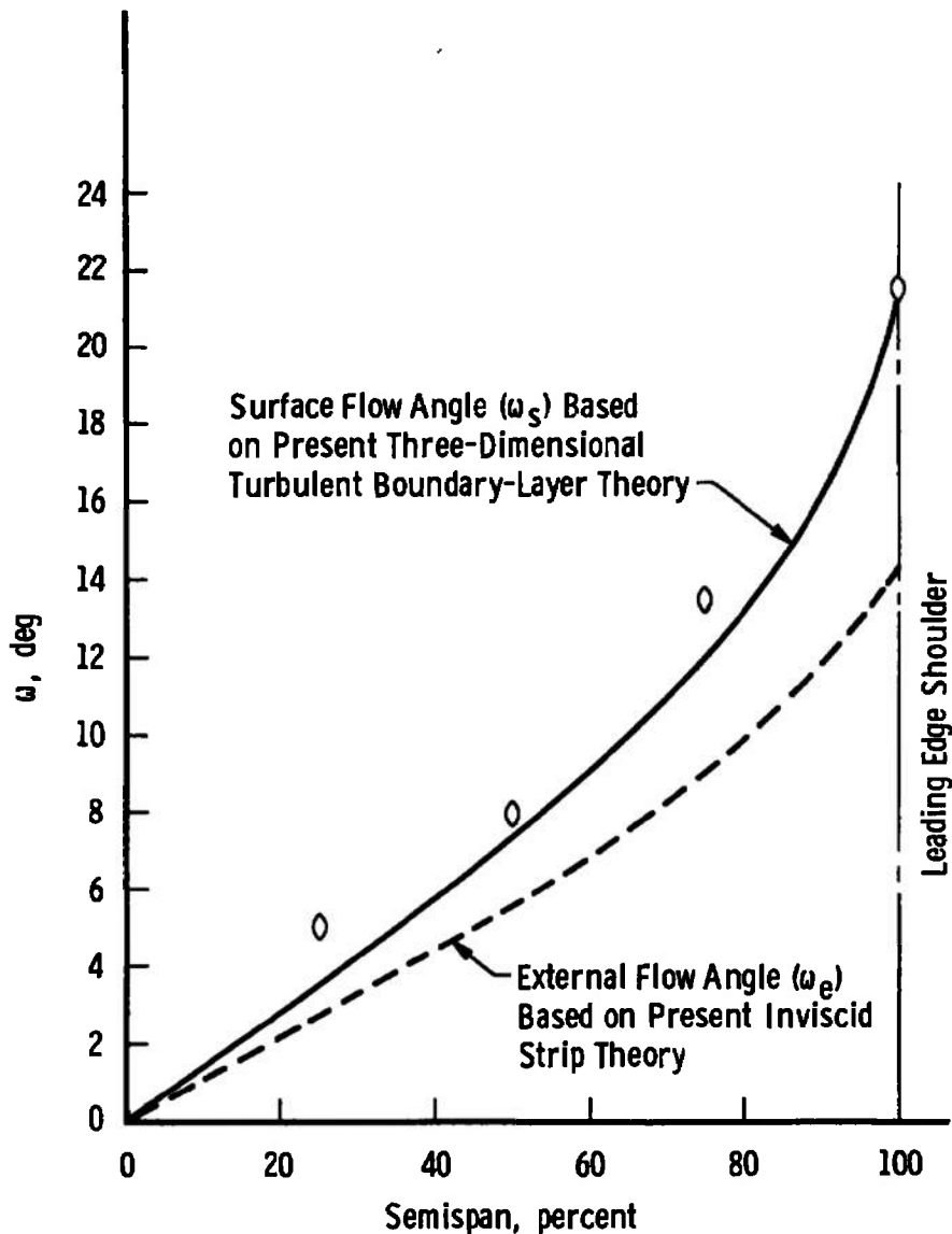
Fig. 24 Spanwise Turbulent Surface Flow Angle and Inviscid Edge Flow Angle Distribution at a High Incidence Angle
