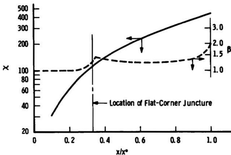
d. Spanwise Crossflow Reynolds Number and Inviscid Velocity Gradient Parameter Distributions
