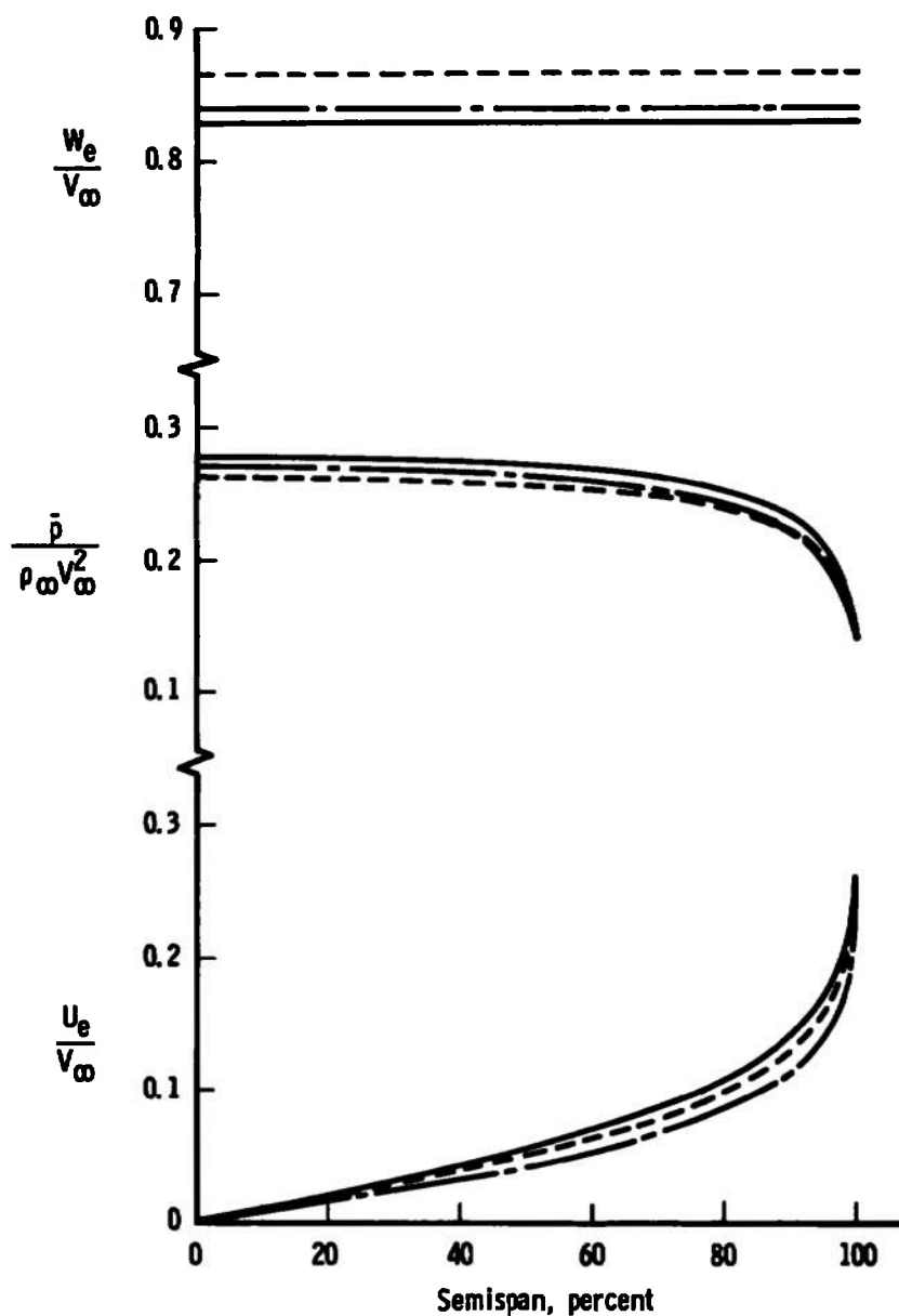
Fig. 17 Spanwise Inviscid Flow Parameters on a Sharp-Leading-Edge Delta Wing at Moderate Incidence
