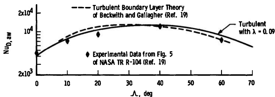
c. Nusselt Number Variation with Yaw Angle
