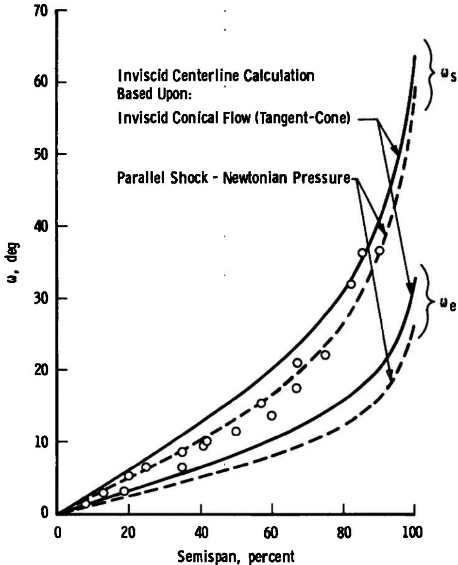
Fig. 20 Spanwise Laminar Surface Flow Angle and Inviscid Edge Flow Angle Distribution at a High Incidence Angle
