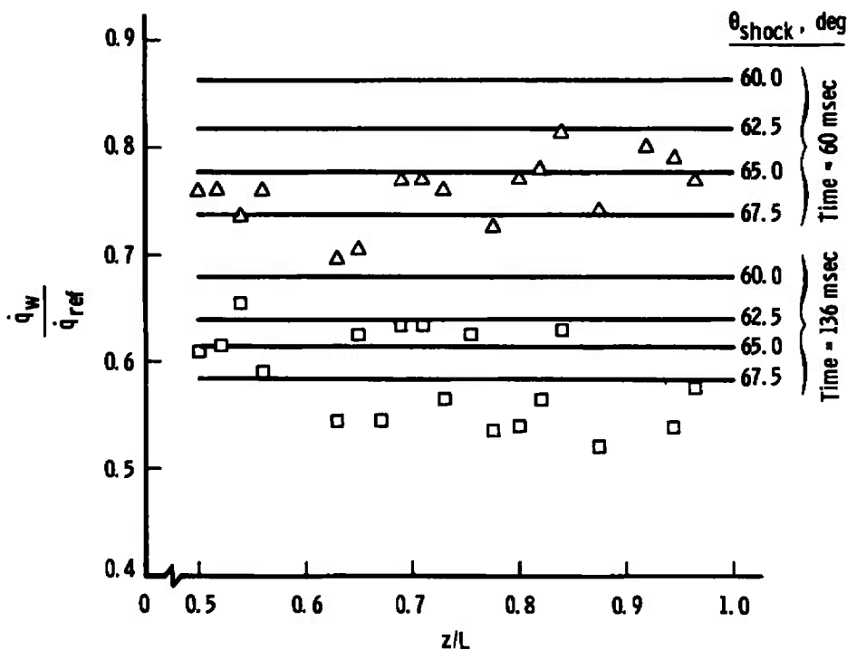
b. Centerline Heat-Transfer-Rate Distribution
