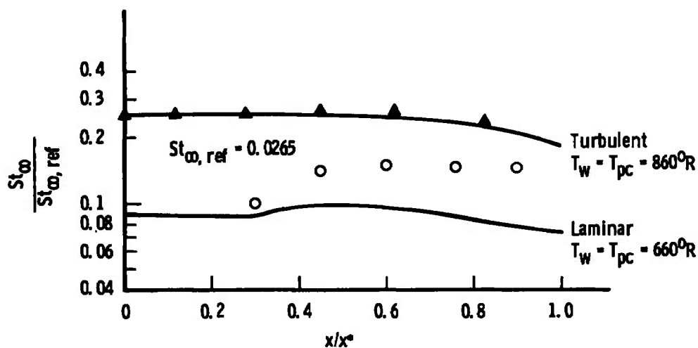
e. Spanwise Stanton Number Distribution
