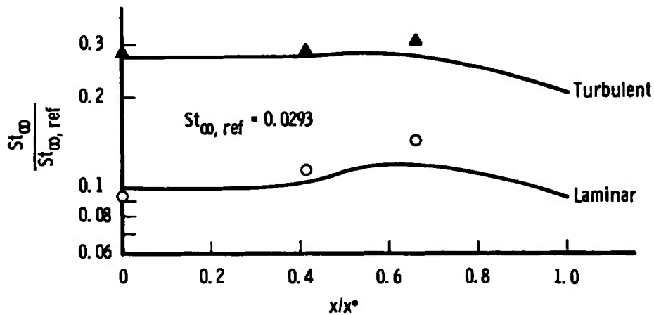
c. Spanwise Stanton Number Distribution
