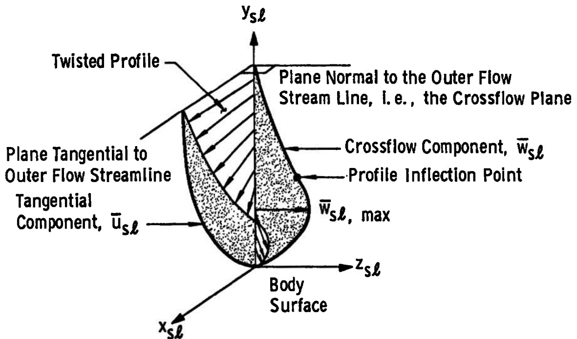
Fig. 2 Three-Dimensional Boundary-Layer Velocity Profiles in Streamline Coordinates
