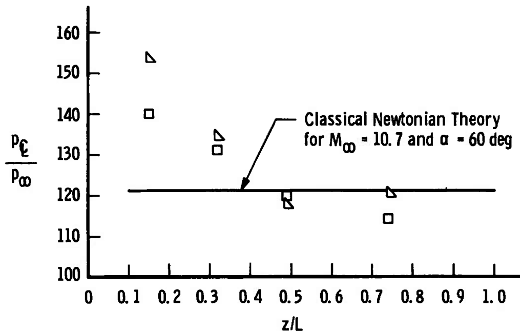
a. Centerline Pressure Distribution
