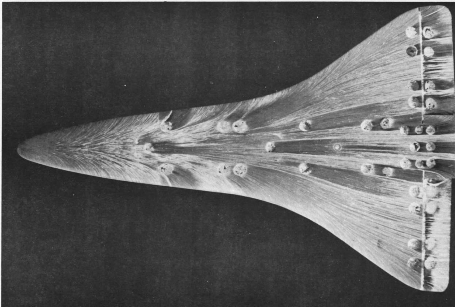
Fig. 49 Windward Surface Flow Visualization Photograph of the MDAC Delta Wing Orbiter at 50-deg Angle of Attack as Taken from Fig. 23a in Mellenthin, Hamilton, and Zoerner (Ref. 103)
