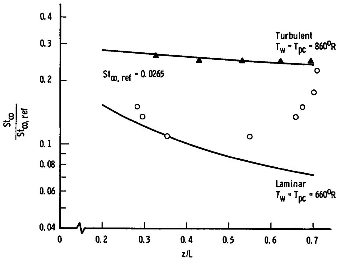
c. 50-deg Angle of Attack Fig. 40 Concluded
