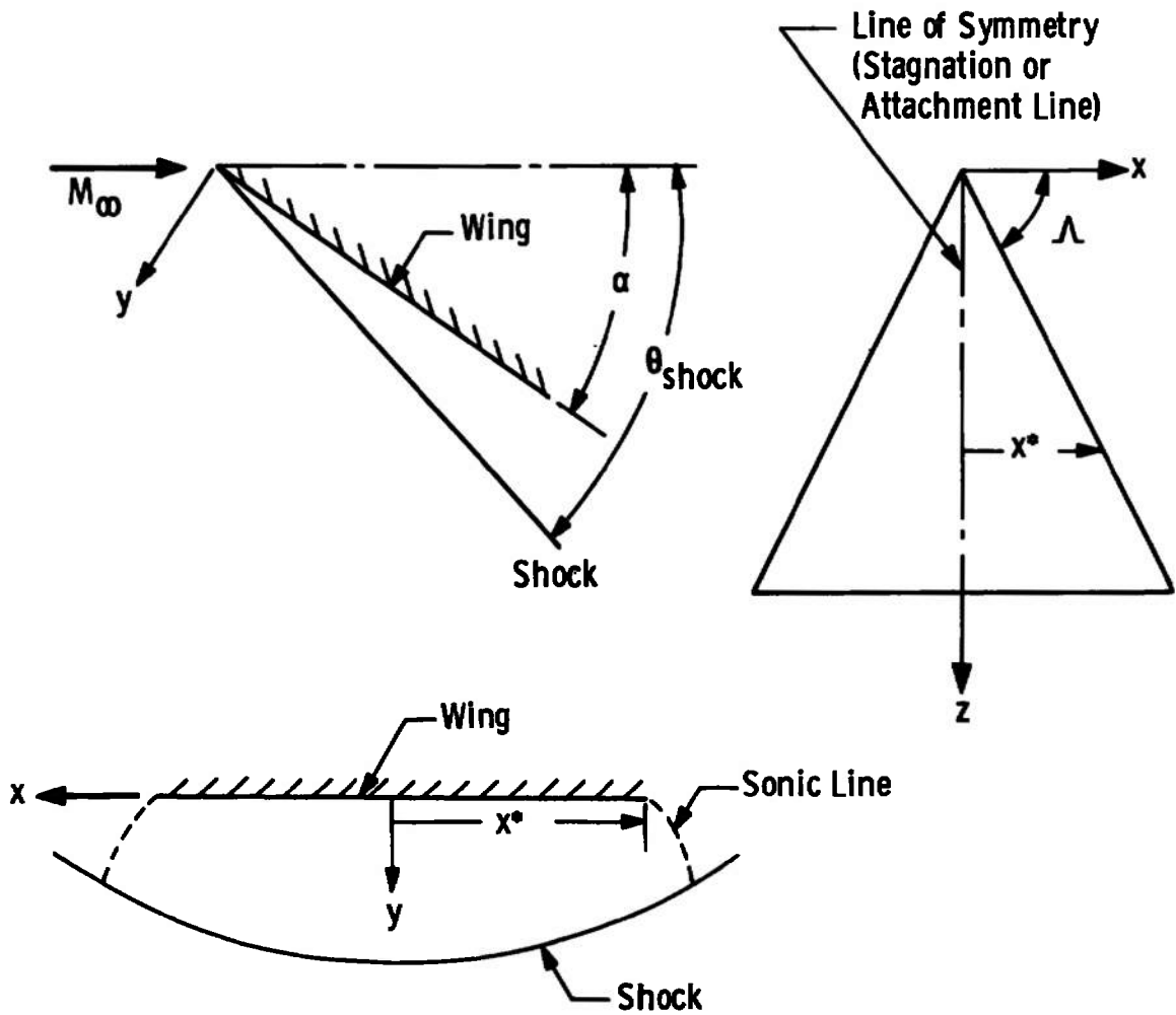
Fig. 4 Coordinate System for Hypersonic Flow Past a Sharp-Leading-Edge Delta Wing at High Angles of Incidence
