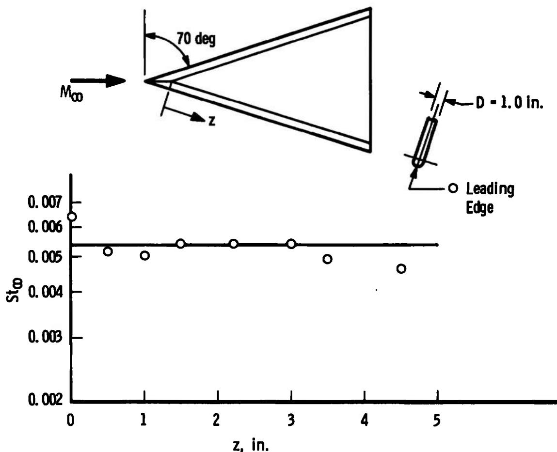
Fig. 9 Comparison of Laminar Heat-Transfer Results for the Cylindrically Blunted Leading Edge of a Sharp-Prow Delta Wing at Zero Angle of Attack
