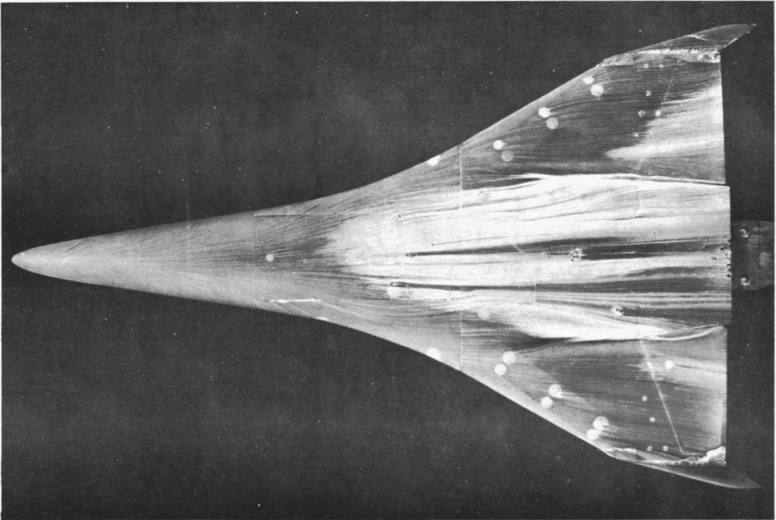
Fig. 7 Windward Surface Flow Visualization Photograph of the NAR Delta Wing Orbiter Configuration 129 at 30-deg Angle of Attack as Taken from Fig. 9c in Seegmiller (Ref. 74)
