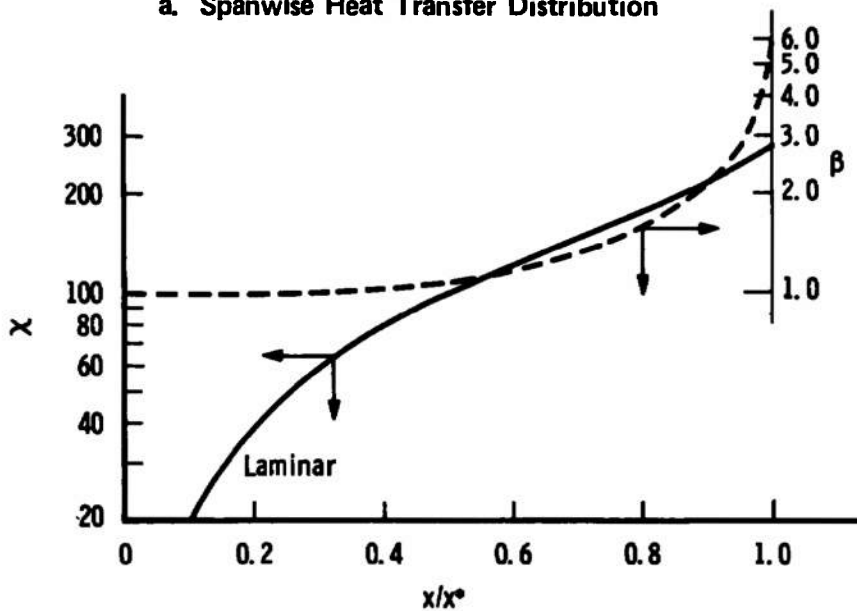
b. Spanwise Crossflow Reynolds Number and Inviscid Velocity Gradient Parameter Distributions
