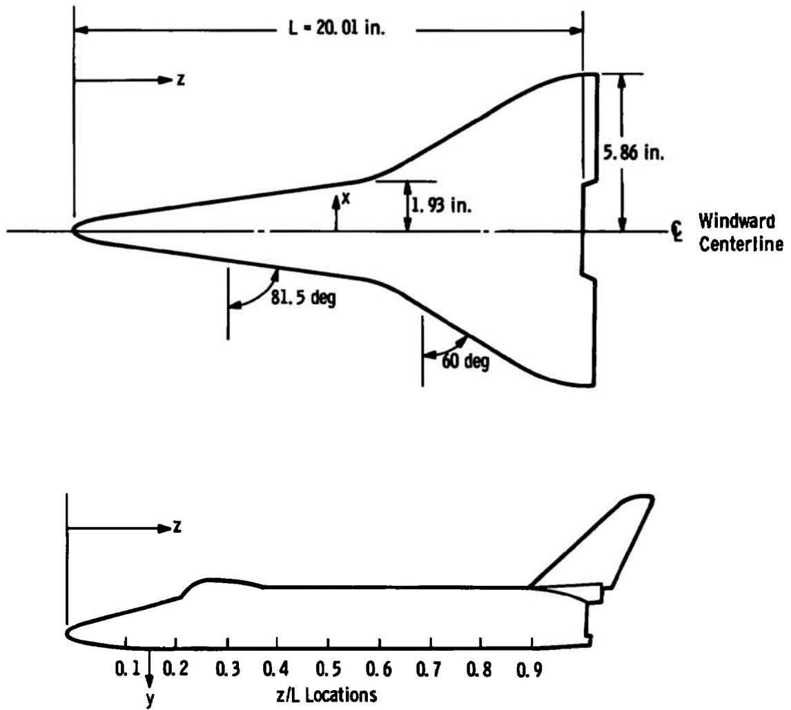
Fig. 26 North American Rockwell (NAR) Delta Wing Orbiter Configuration 161B (0.009-Scale)
