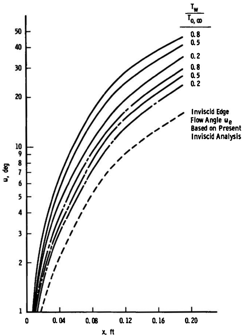
Fig. 44 Wall Temperature Effects on Spanwise Laminar and Turbulent Surface Flow Angle Distributions
