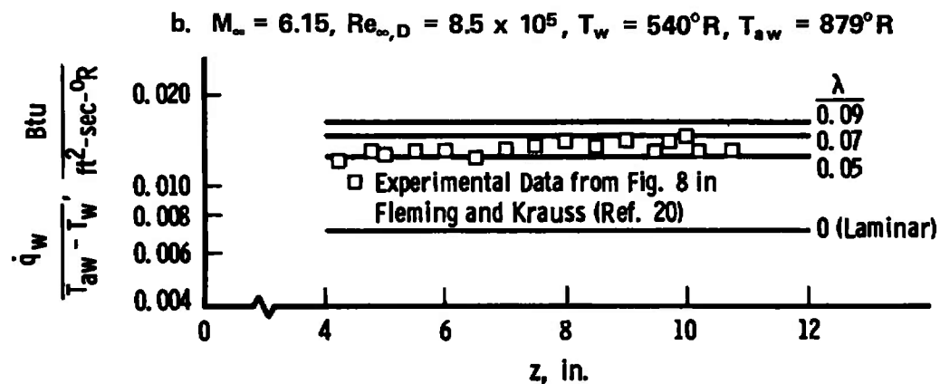
Fig. 11 Effects of Outer Mixing-Length Constant \lambda on Yawed Cylinder Heat Transfer
