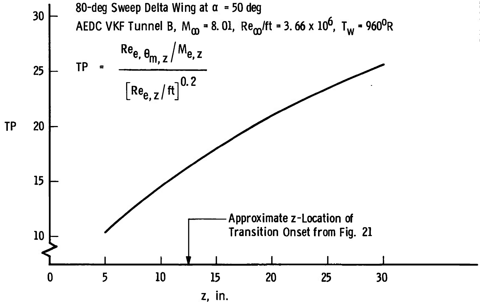
Fig. 22 Centerline Transition Onset Parameter Distribution on a Delta Wing at High Incidence
