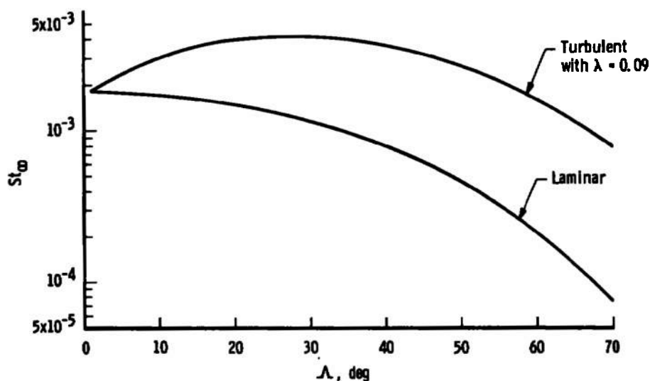
a. Stanton Number Variation with Yaw Angle
