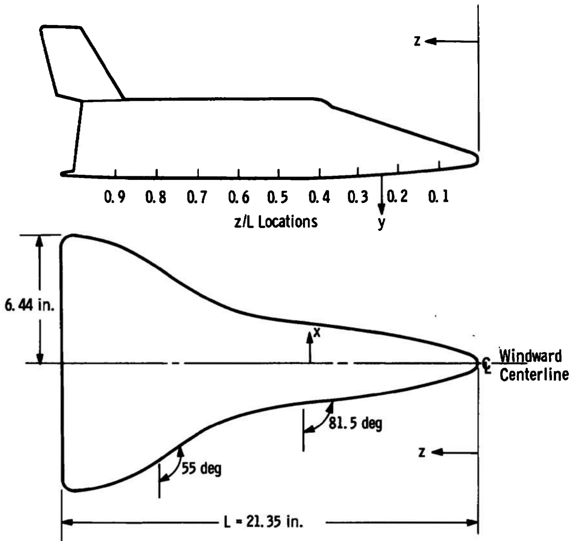
Fig. 38 McDonnell-Douglas (MDAC) Delta Wing Orbiter Configuration (0.011-Scale)
