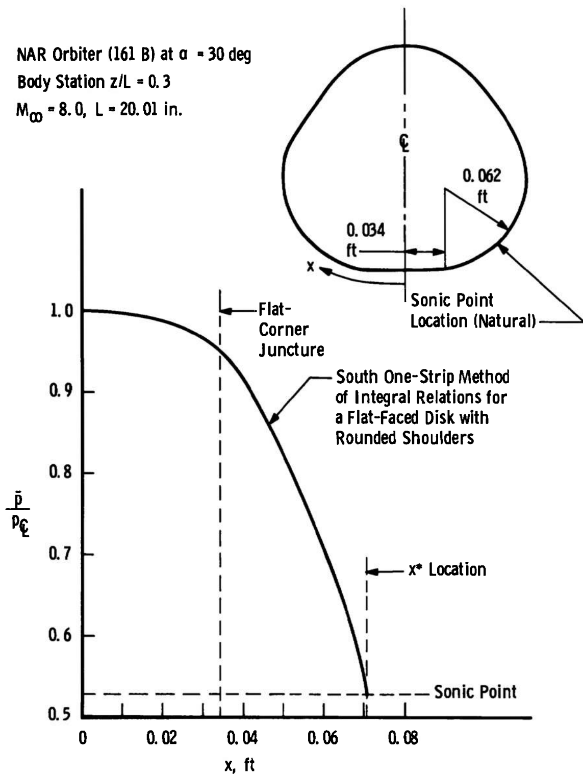
Fig. 29 Spanwise Pressure Distribution on the NAR Orbiter at Incidence
