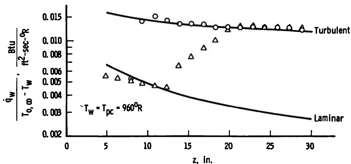
Fig. 21 Centerline Laminar, Transitional, and Turbulent Heat Transfer on a Highly Swept Delta Wing at Moderate to High Angles of Incidence
