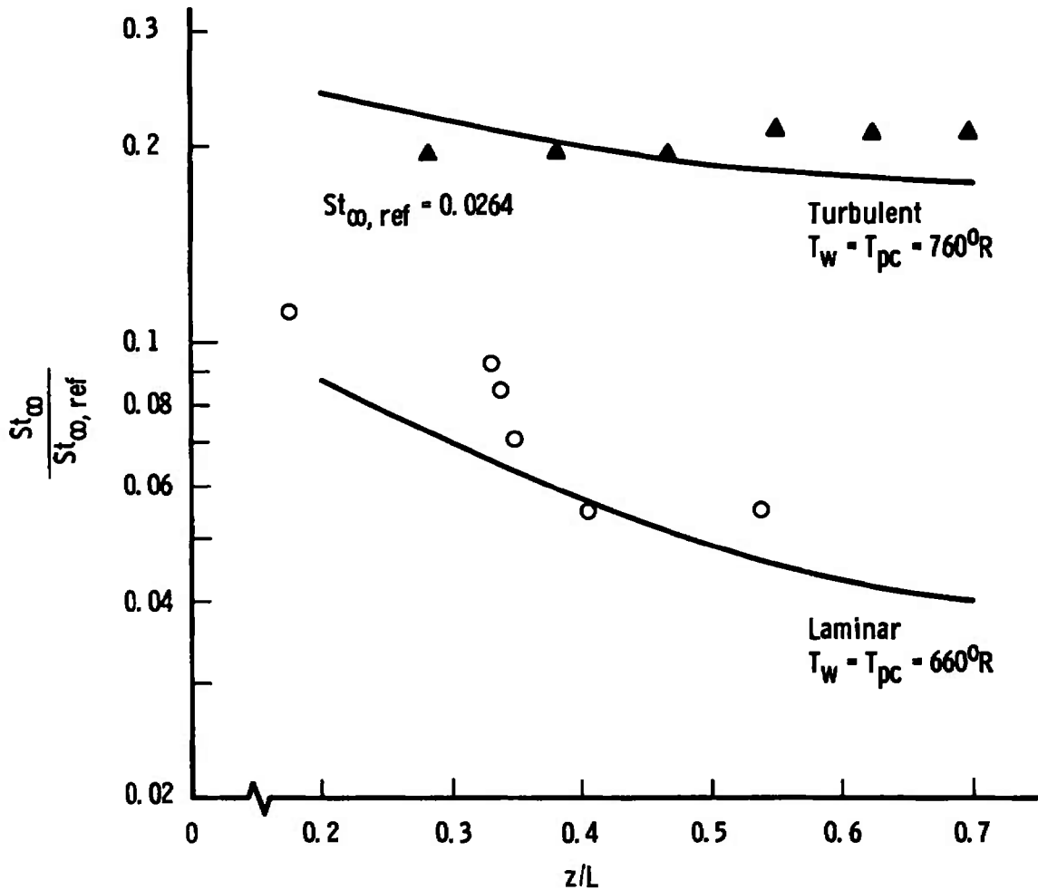
Fig. 40 Windward Centerline Stanton Number Distributions on the MDAC Orbiter under AEDC-VKF Tunnel B Conditions
