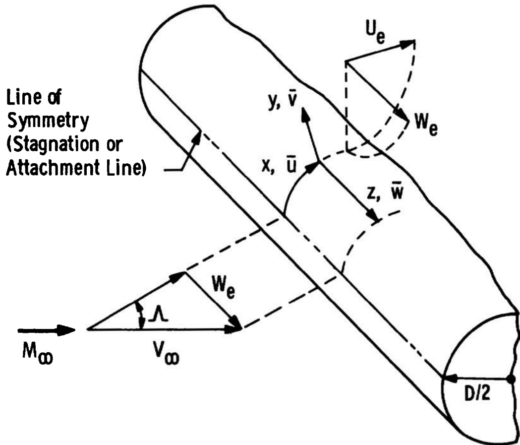
Fig. 3 Coordinate System for Flow over an Infinite Yawed Circular Cylinder
