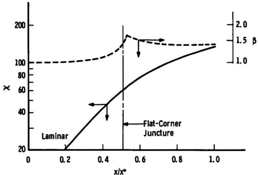
f. Spanwise Crossflow Reynolds Number and Inviscid Velocity Gradient Parameter Distributions
