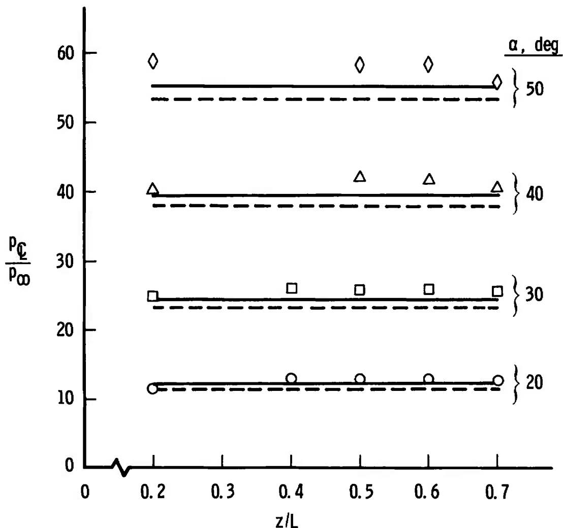
Fig. 27 Centerline Pressure Distribution on the NAR Orbiter at Incidence
