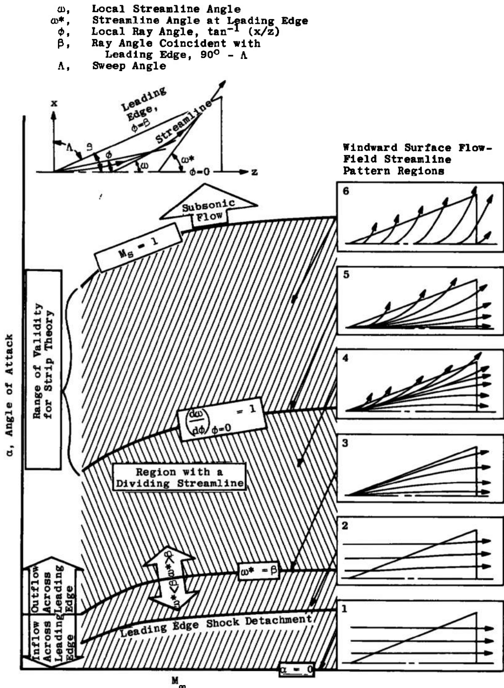
Fig. 5 Schematic of Windward Surface Flow-Field Regimes for Sharp-Edged Delta Wings at Incidence under Hypersonic Conditions as Taken from Fig. C6 in Appendix C of Thomas and Perlbachs (Ref. 58)
