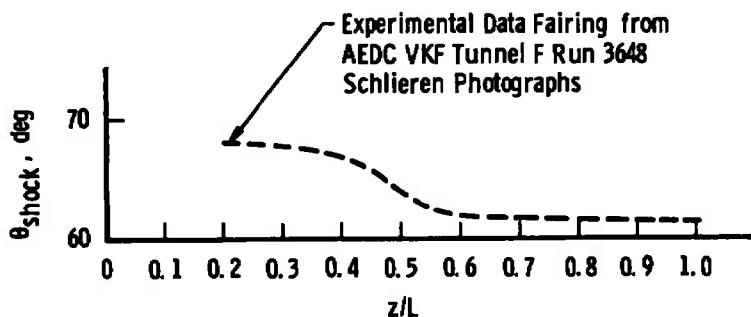
a. Centerline Shock Angle Distribution
