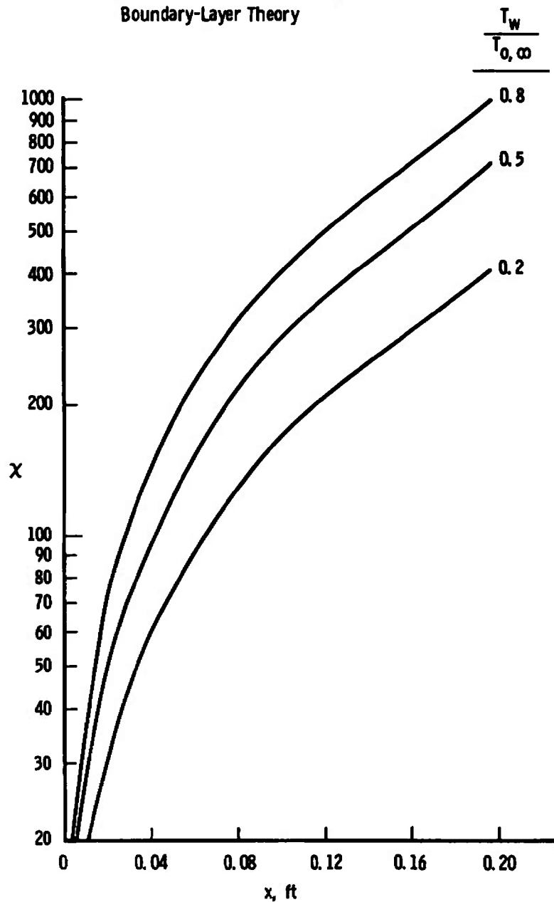
Fig. 45 Wall Temperature Effects on Spanwise Crossflow Reynolds Number Distributions
