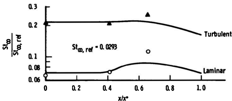
a. Spanwise Stanton Number Distribution
