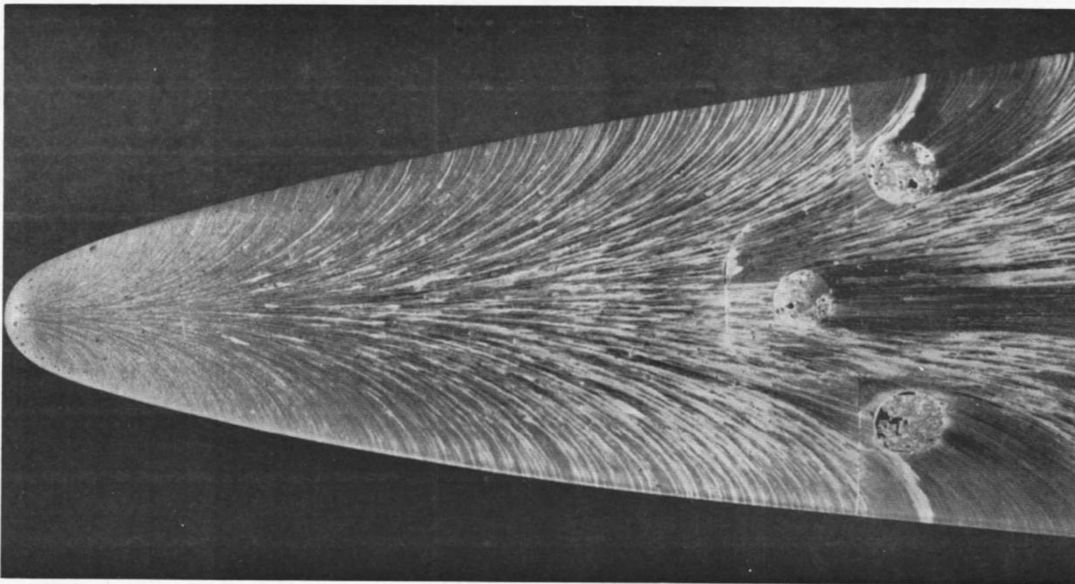
Fig. 48 Nose Region Windward Surface Flow Visualization Photograph of the MDAC Delta Wing Orbiter at 50-deg Angle of Attack as Taken from Fig. 23c in Mellenthin, Hamilton, and Zoerner (Ref. 103)
