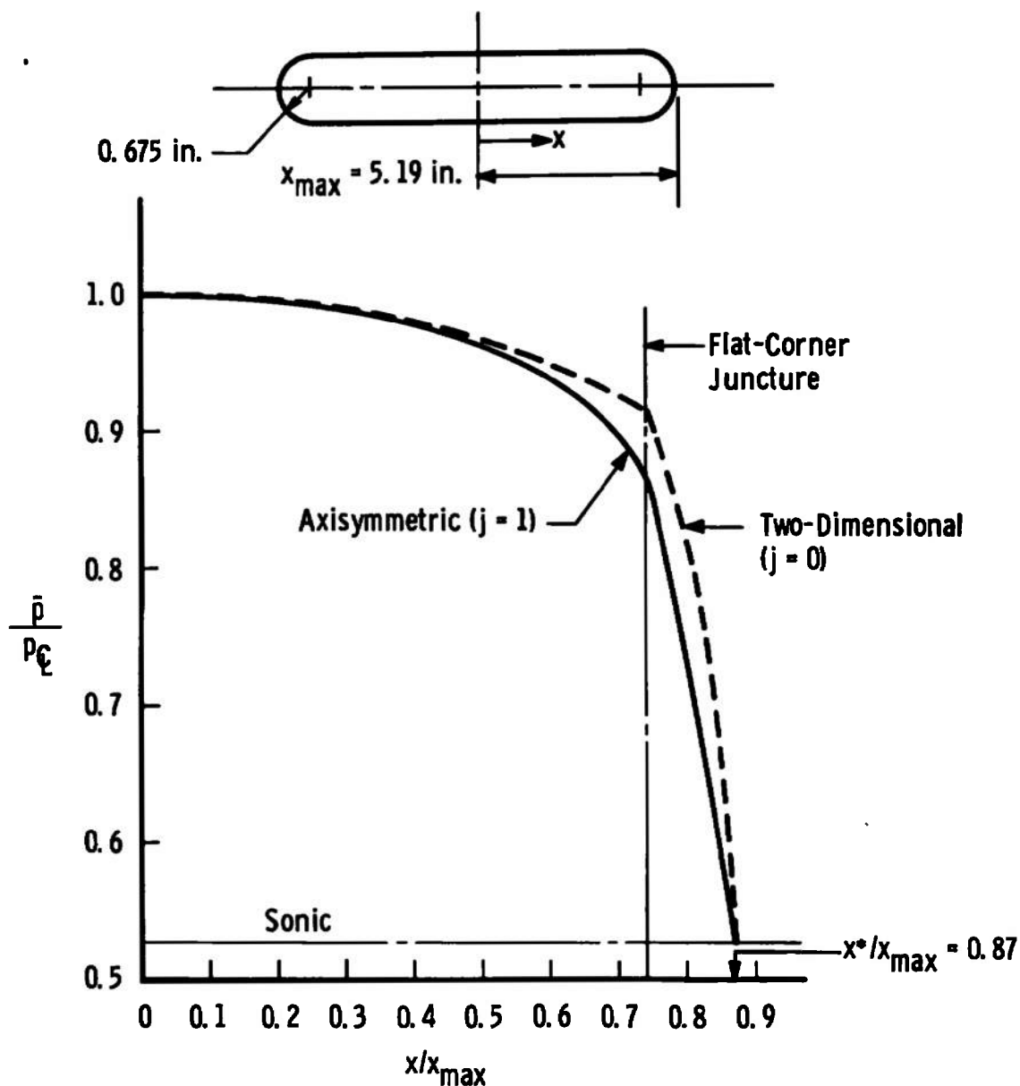
Fig. 35 Effects of Body Type on Spanwise Pressure Distribution
