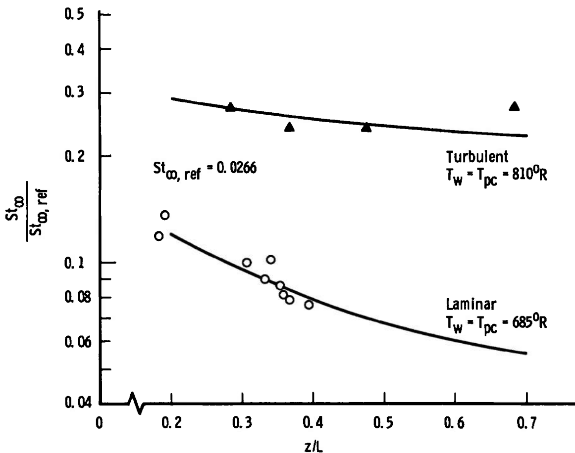
b. 40-deg Angle of Attack Fig. 40 Continued
