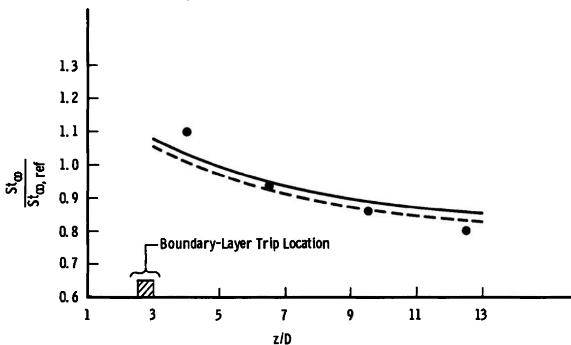
Fig. 23 Comparison of Present Three-Dimensional Turbulent Boundary-Layer Theory with Boeing \rho_r \mu_r Approach along Delta Wing Centerline
