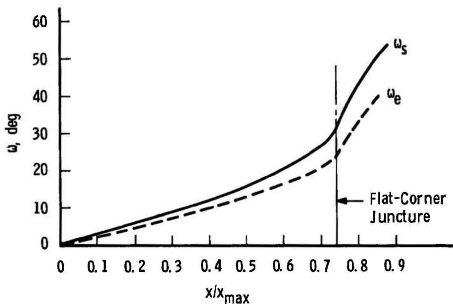
b. Spanwise Surface and Edge Flow Directions
