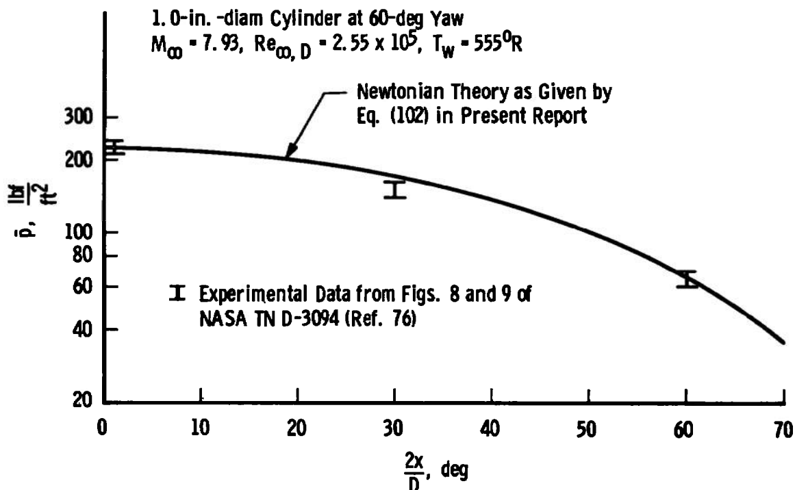
a. Circumferential Pressure Distribution
