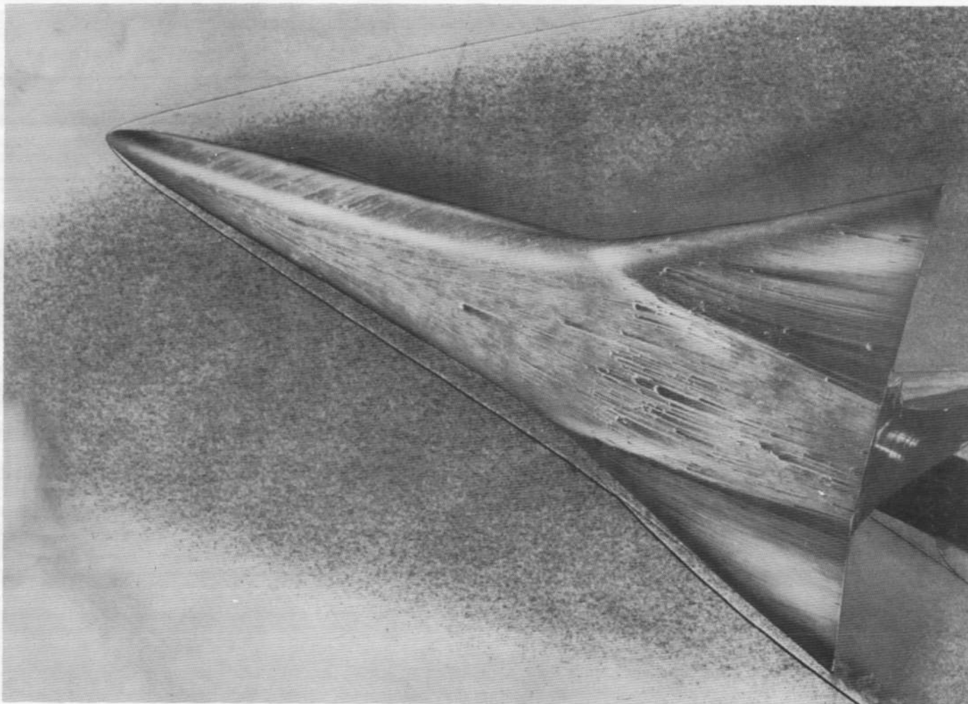
Fig. 8 Oblique View Windward Surface Flow Visualization Photograph of the NAR Delta Wing Orbiter Configuration 134 at 30-deg Angle of Attack as Taken from Fig. 4b in Cleary (Ref. 75)
