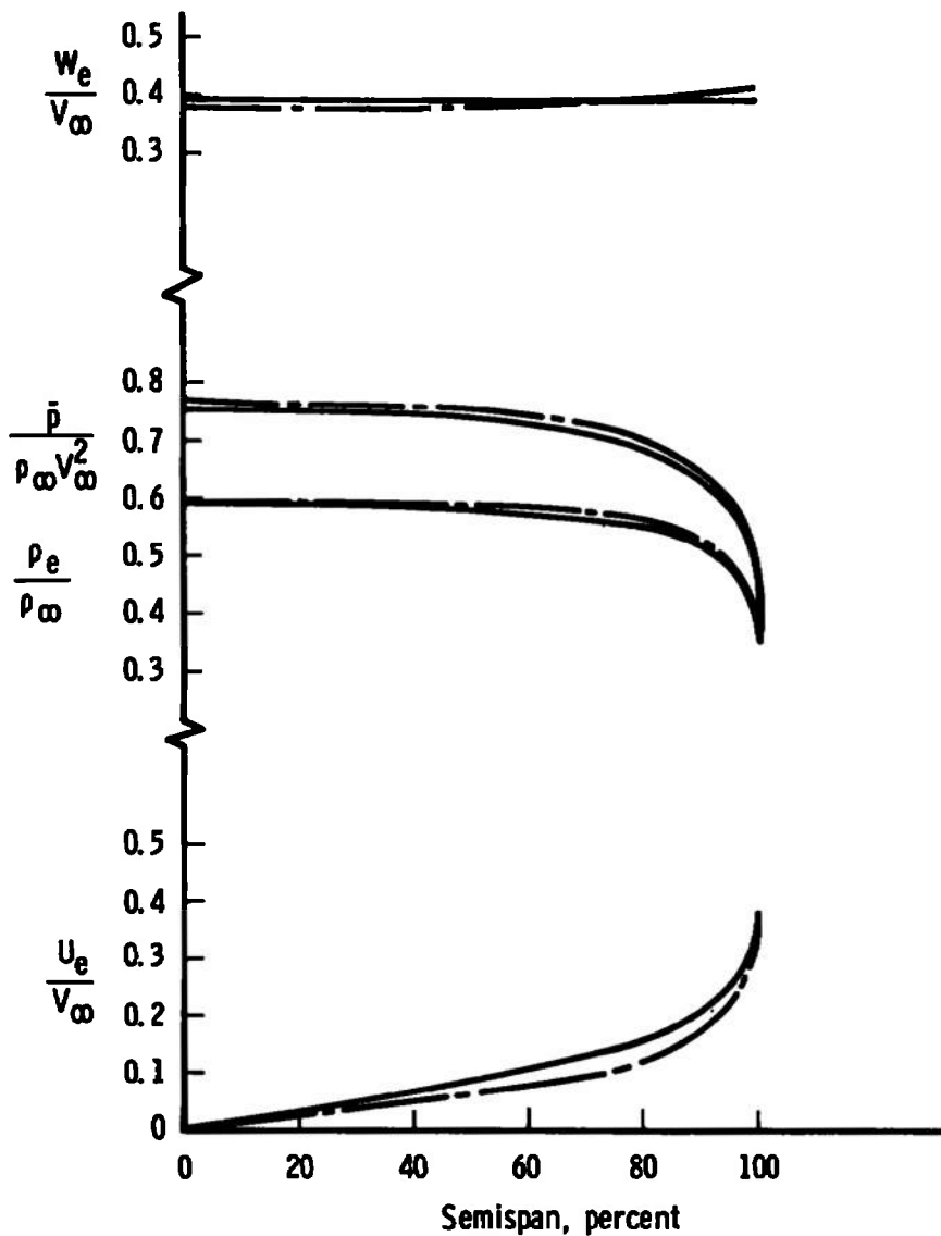
Fig. 16 Spanwise Inviscid Flow Parameters on a Sharp-Leading-Edge Delta Wing at High Incidence
