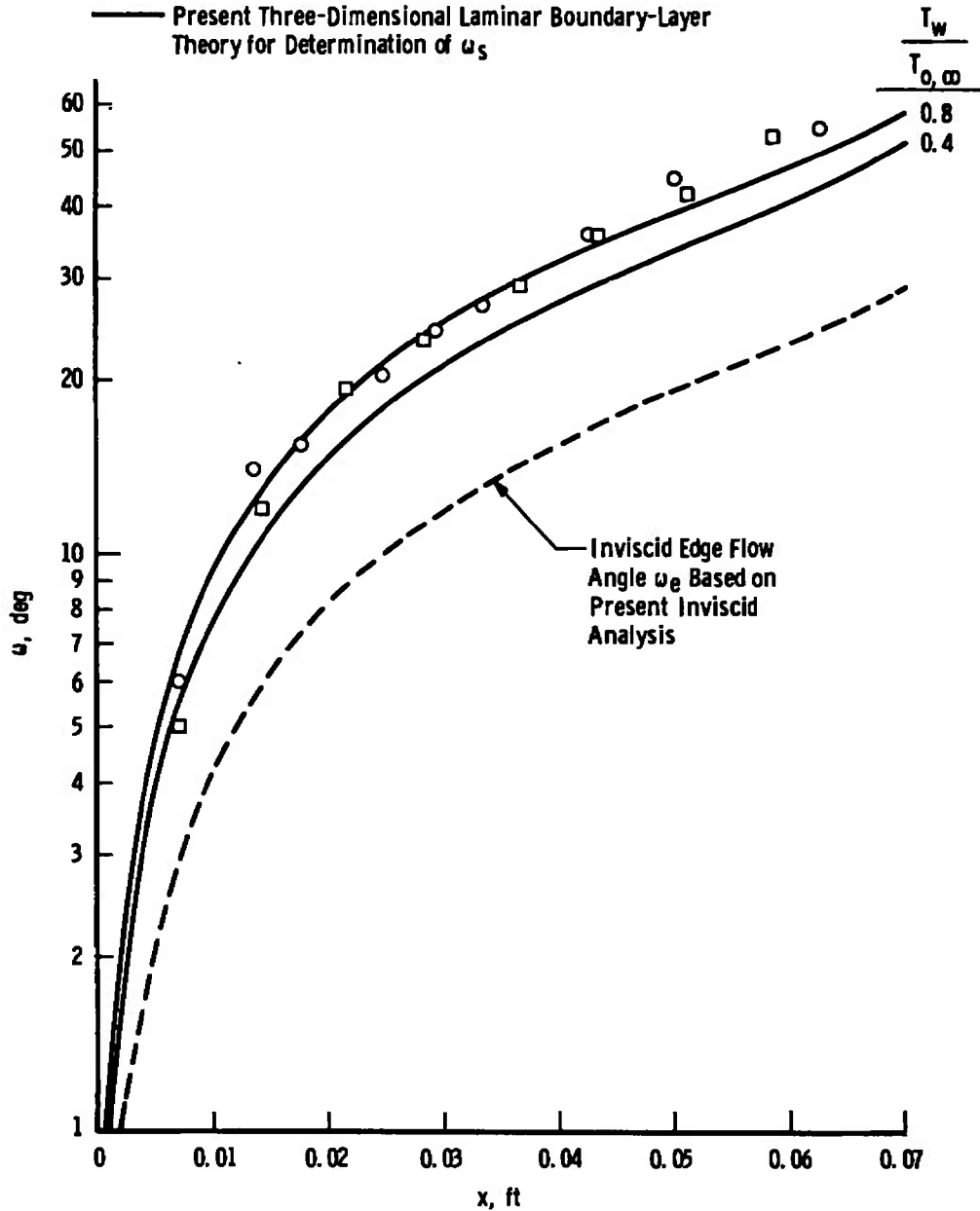
Fig. 46 Spanwise Surface Flow Angle Distribution in the Nose Region of the MDAC Orbiter under High Angle-of-Attack Conditions
