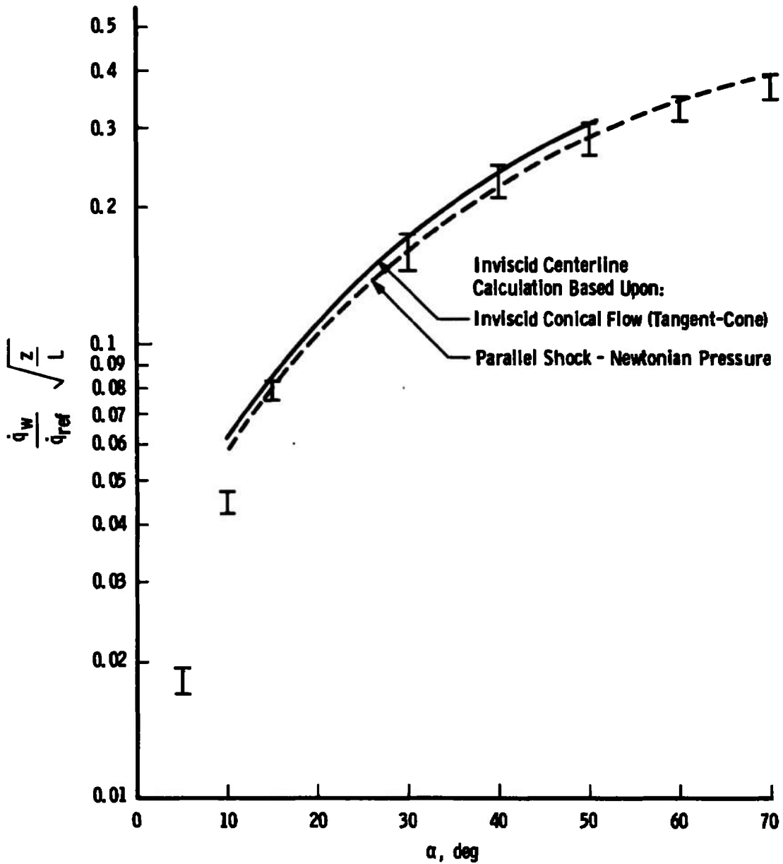
Fig. 18 Angle-of-Attack Effects on Centerline Laminar Heat Transfer
