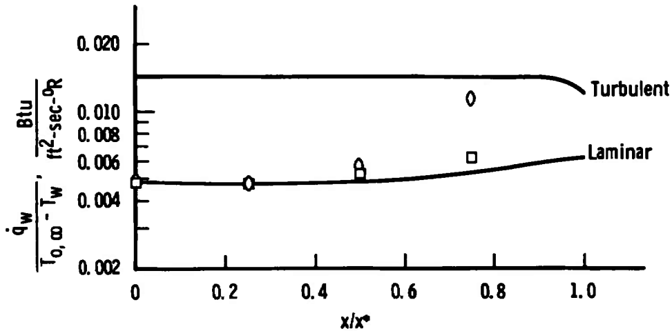
a. Spanwise Heat Transfer Distribution
