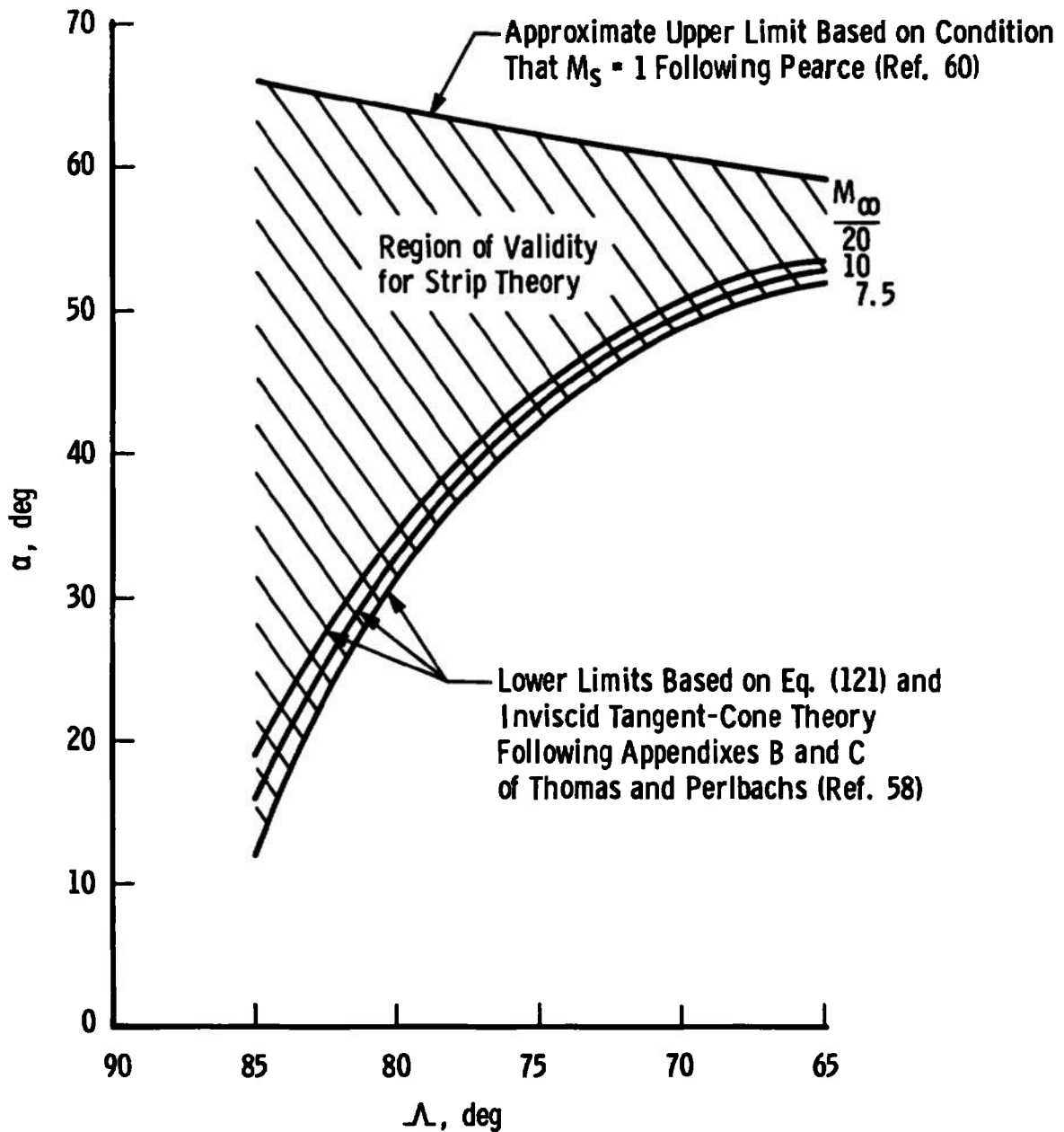
Fig. 6 Range of Applicability of Strip Theory for Sharp-Edged Delta Wings at Incidence under Hypersonic Conditions
