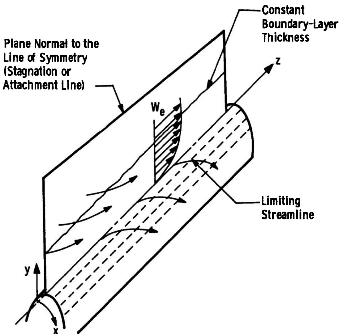
Fig. 13 Schematic of Stagnation or Attachment Line Flow over an Infinite Extent Yawed Circular Cylinder
