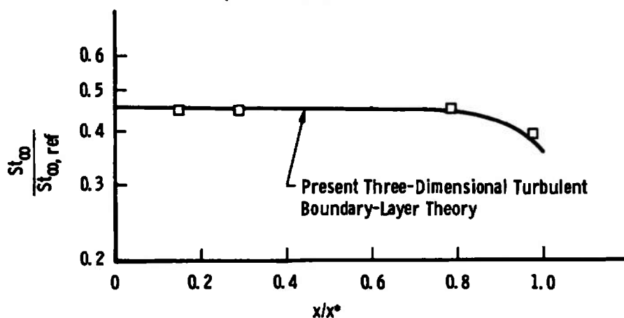
a. Spanwise Heat Transfer Distribution at Body Location z/L = 0.5
