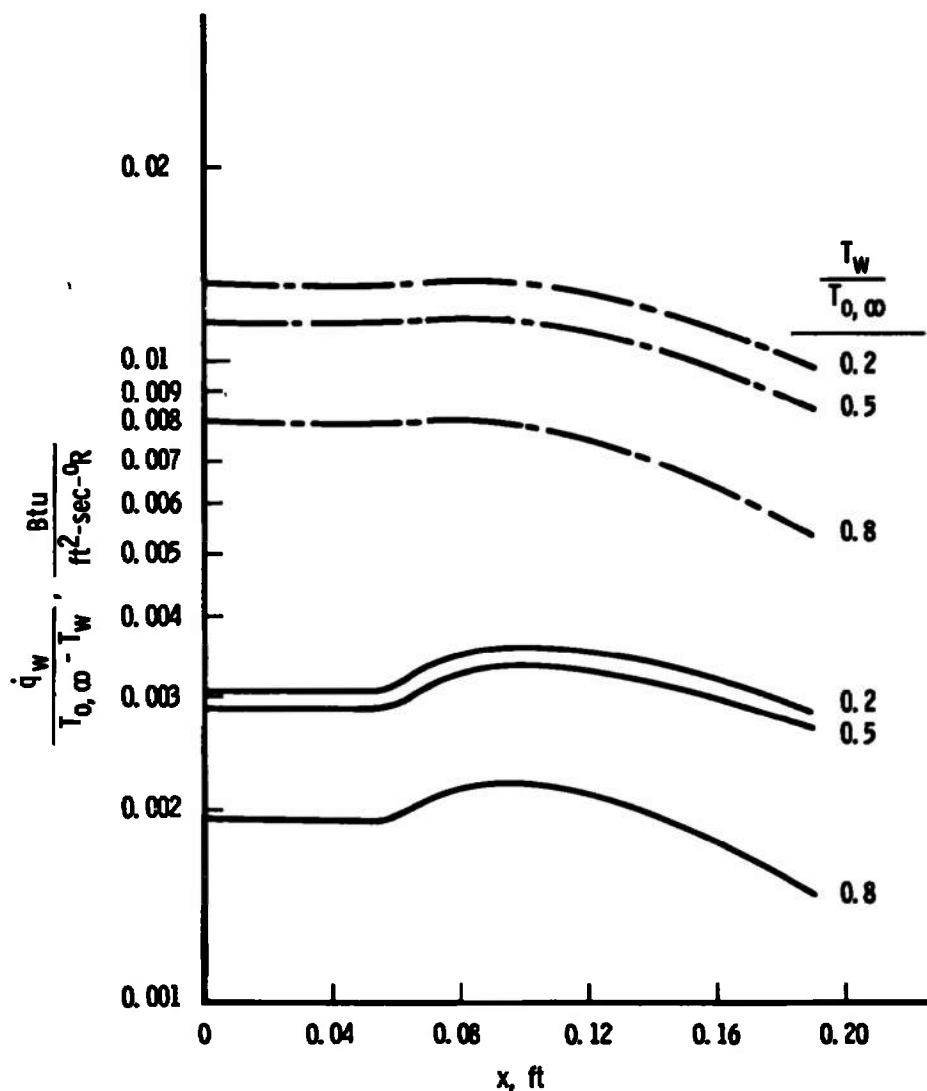
Fig. 43 Wall Temperature Effects on Spanwise Laminar and Turbulent Heat-Transfer Distributions
