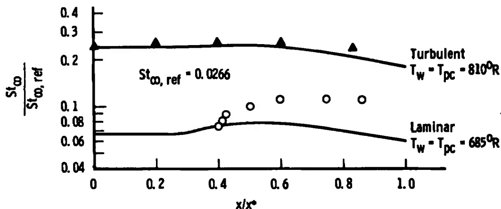
c. Spanwise Stanton Number Distribution
