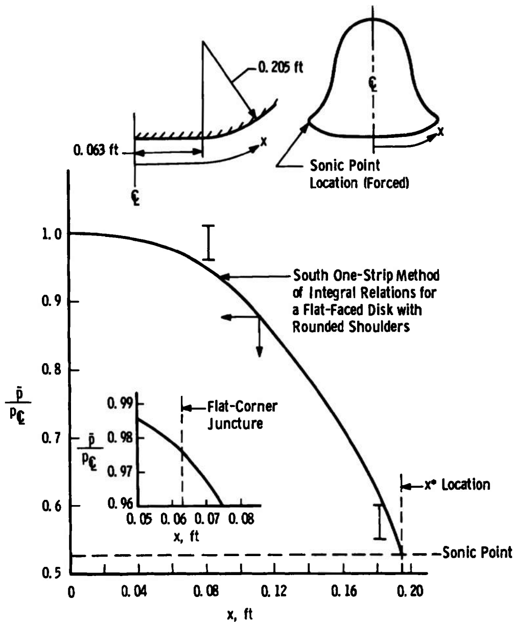
Fig. 39 Spanwise Pressure Distribution on the MDAC Orbiter at Incidence
