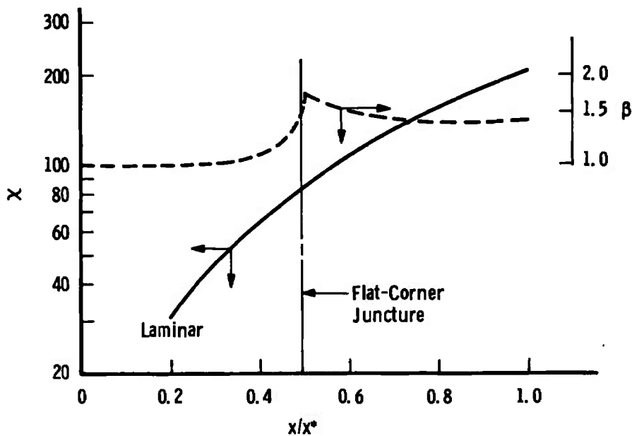
d. Spanwise Crossflow Reynolds Number and Inviscid Velocity Gradient Parameter Distributions
