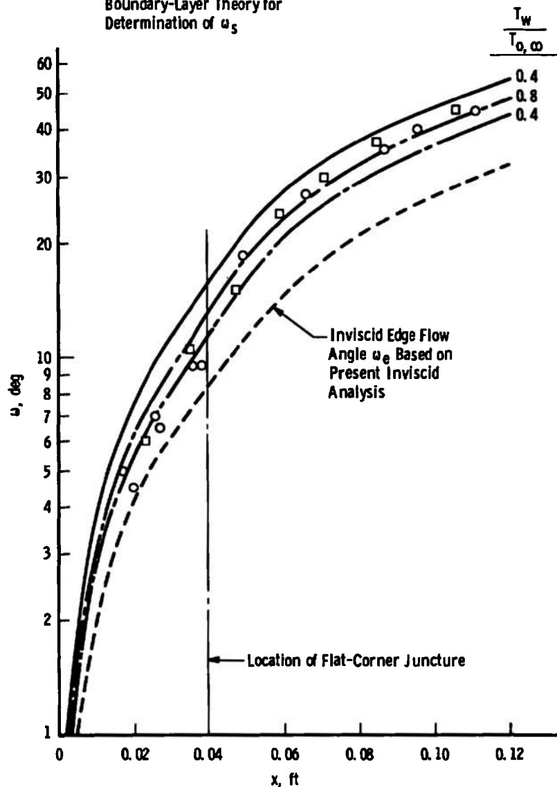
Fig. 47 Spanwise Surface Flow Angle Distribution at Mid-Body on the MDAC Orbiter under High Angle-of-Attack Conditions
