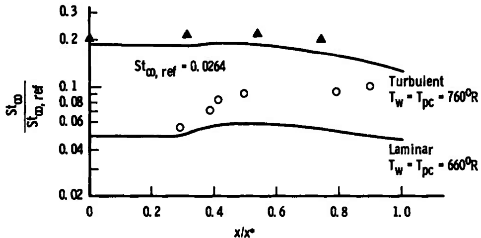
a. Spanwise Stanton Number Distribution
