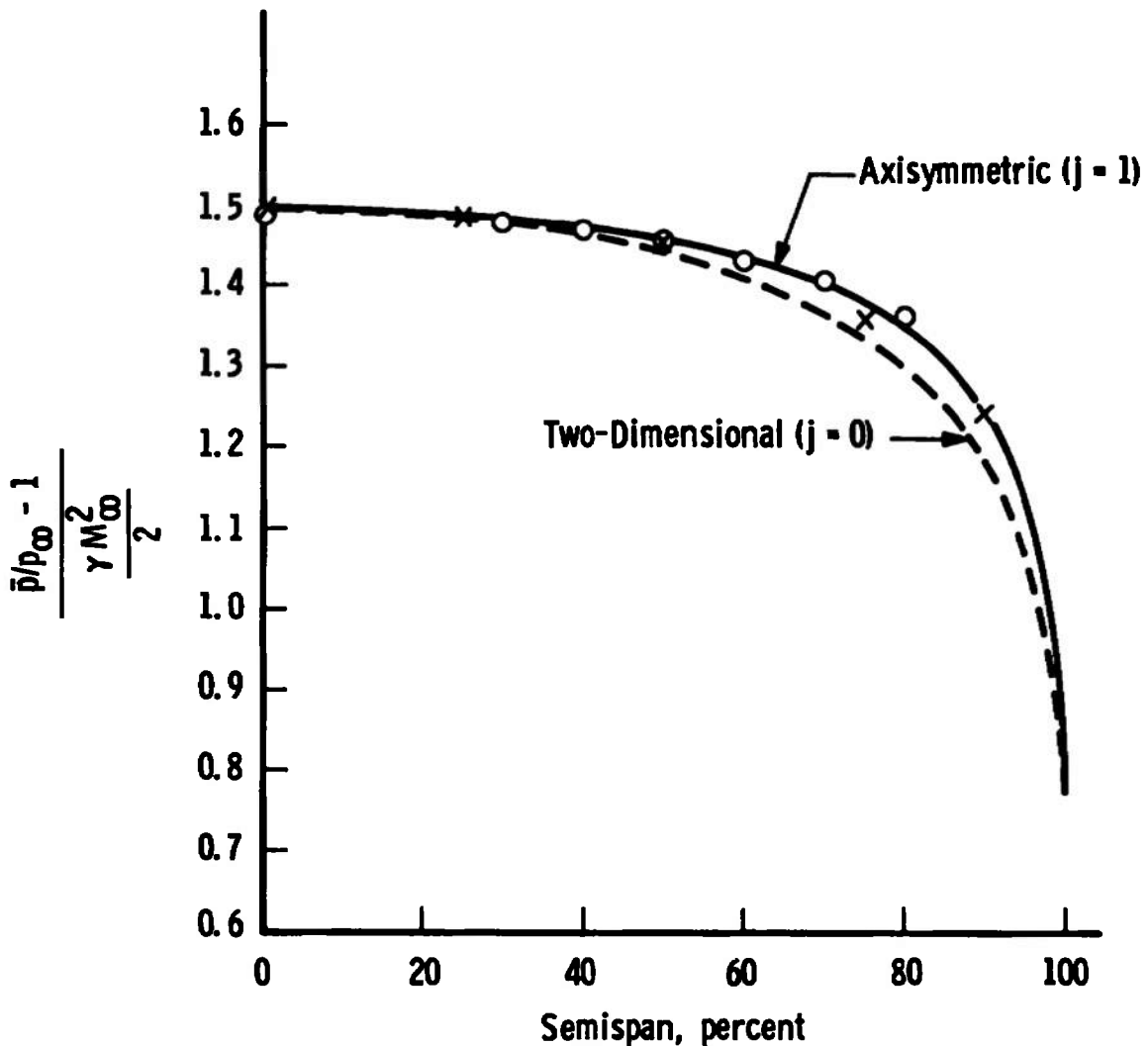
Fig. 14 Spanwise Surface Pressure Distribution on a Sharp-Leading-Edge Delta Wing at High Incidence
