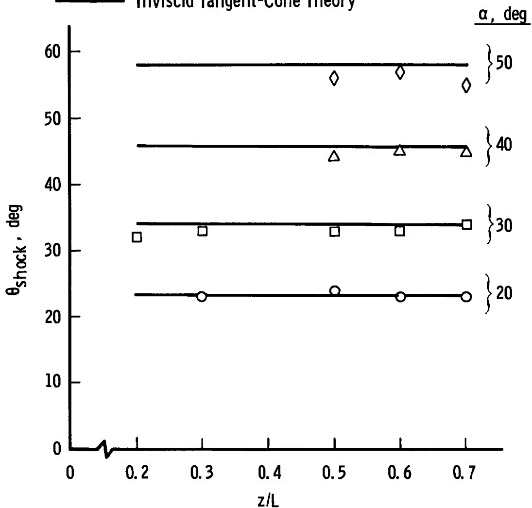
Fig. 28 Centerline Shock Angle Distribution on the NAR Orbiter at Incidence
