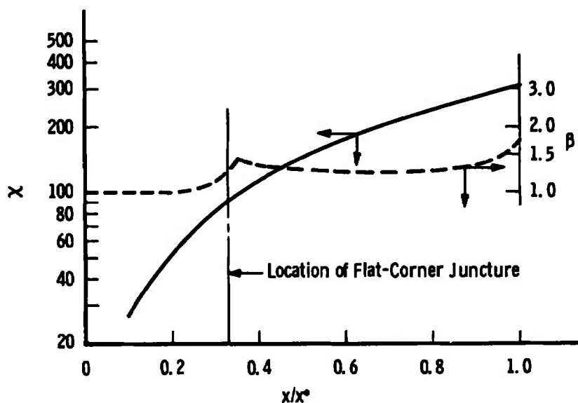
f. Spanwise Crossflow Reynolds Number and Inviscid Velocity Gradient Parameter Distributions
