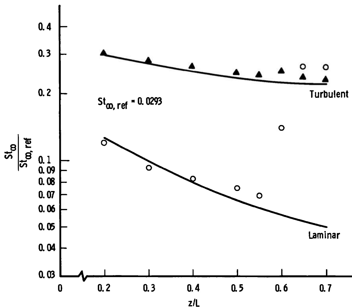
b. 40-deg Angle of Attack Fig. 30 Continued
