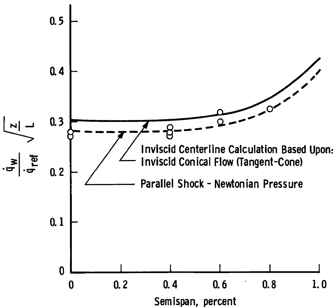
Fig. 19 Spanwise Laminar Heat-Transfer Distribution at a High Incidence Angle
