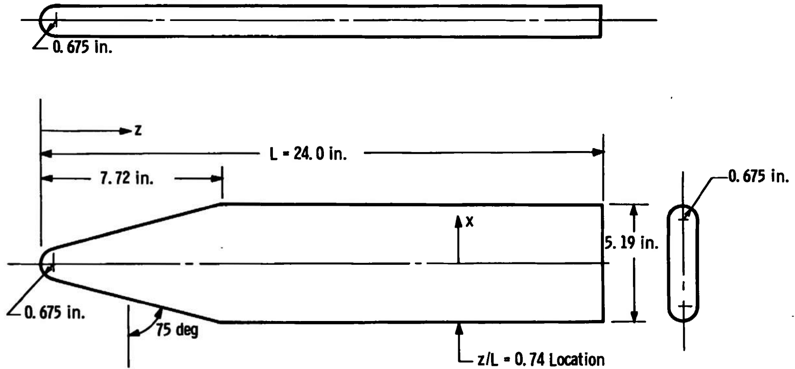
Fig. 33 NASA-Langley Research Center Straight Body (NASA LRC-SB) Delta Wing Configuration
