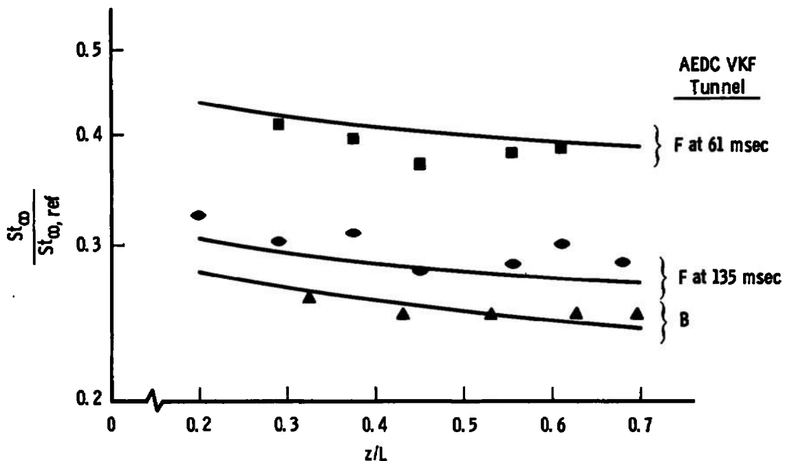
Fig. 42 Effects of Mach Number, Reynolds Number, and Wall Temperature Ratio on MDAC Orbiter Windward Centerline Turbulent Heat Transfer under High Angle-of-Attack Conditions
