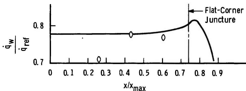
a. Spanwise Heat-Transfer Distribution for Body Location z/L = 0.74
