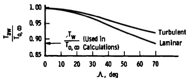
b. Adiabatic Wall Temperature Variation with Yaw Angle
