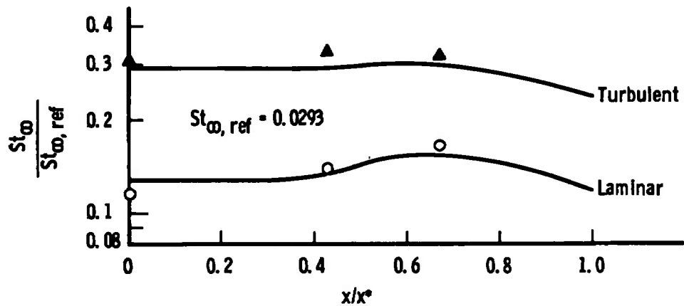
e. Spanwise Stanton Number Distribution
