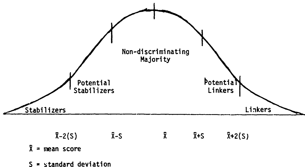
Figure 5. Categorization of the Population Assuming a Normal Distribution
