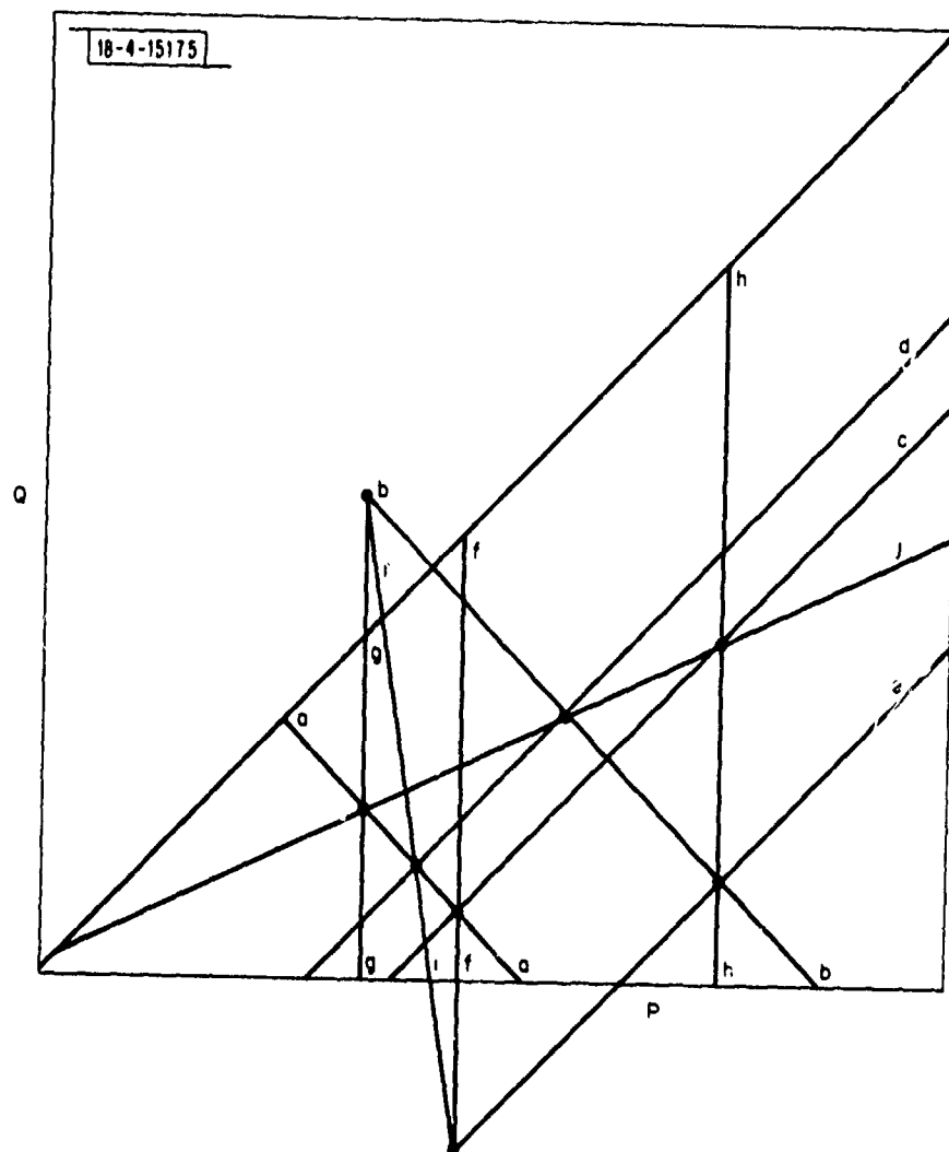
Fig. 2. Decision boundaries.
