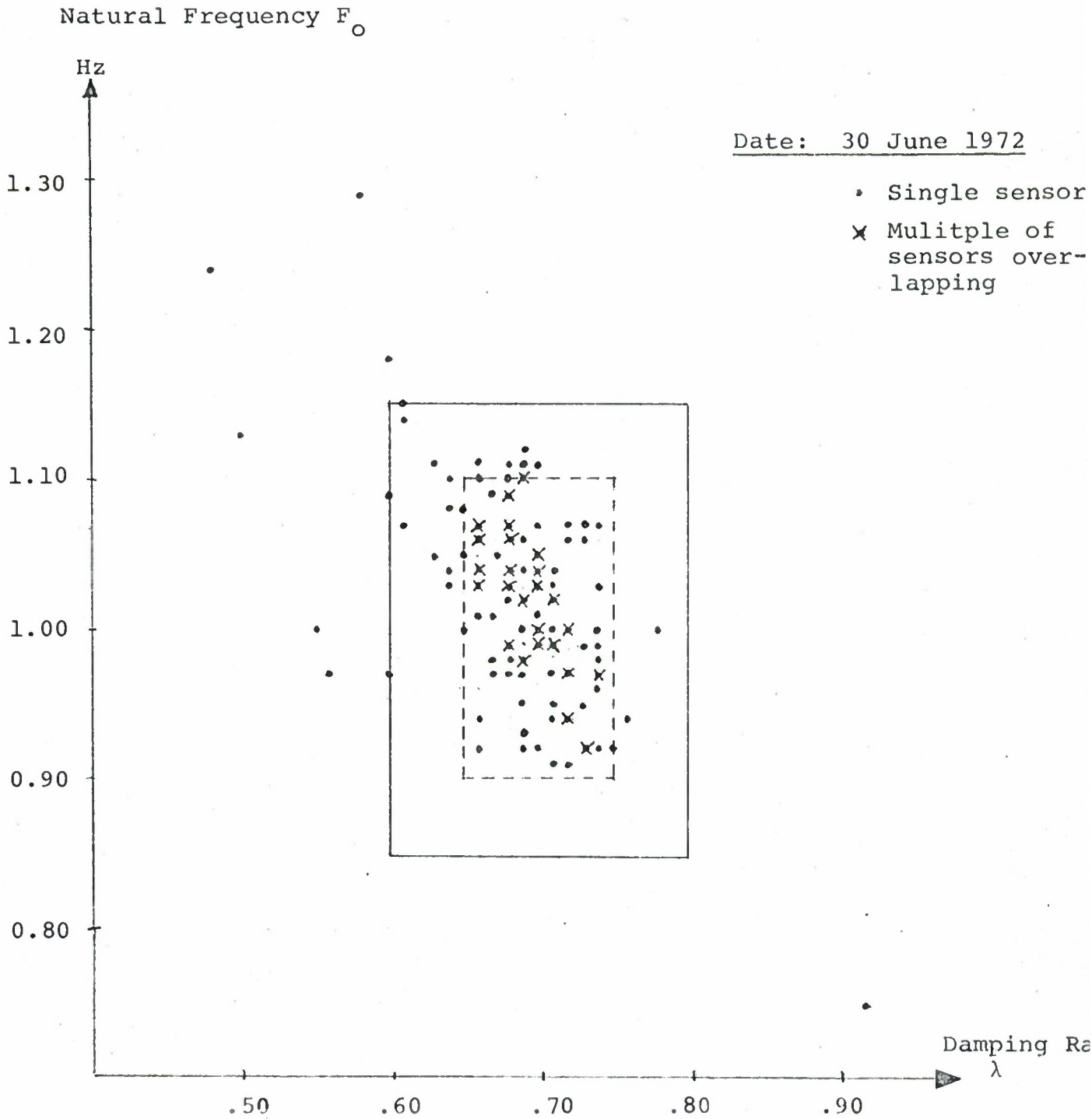
Figure 3.25 Damping and Natural Frequency of SP Seismometers.
