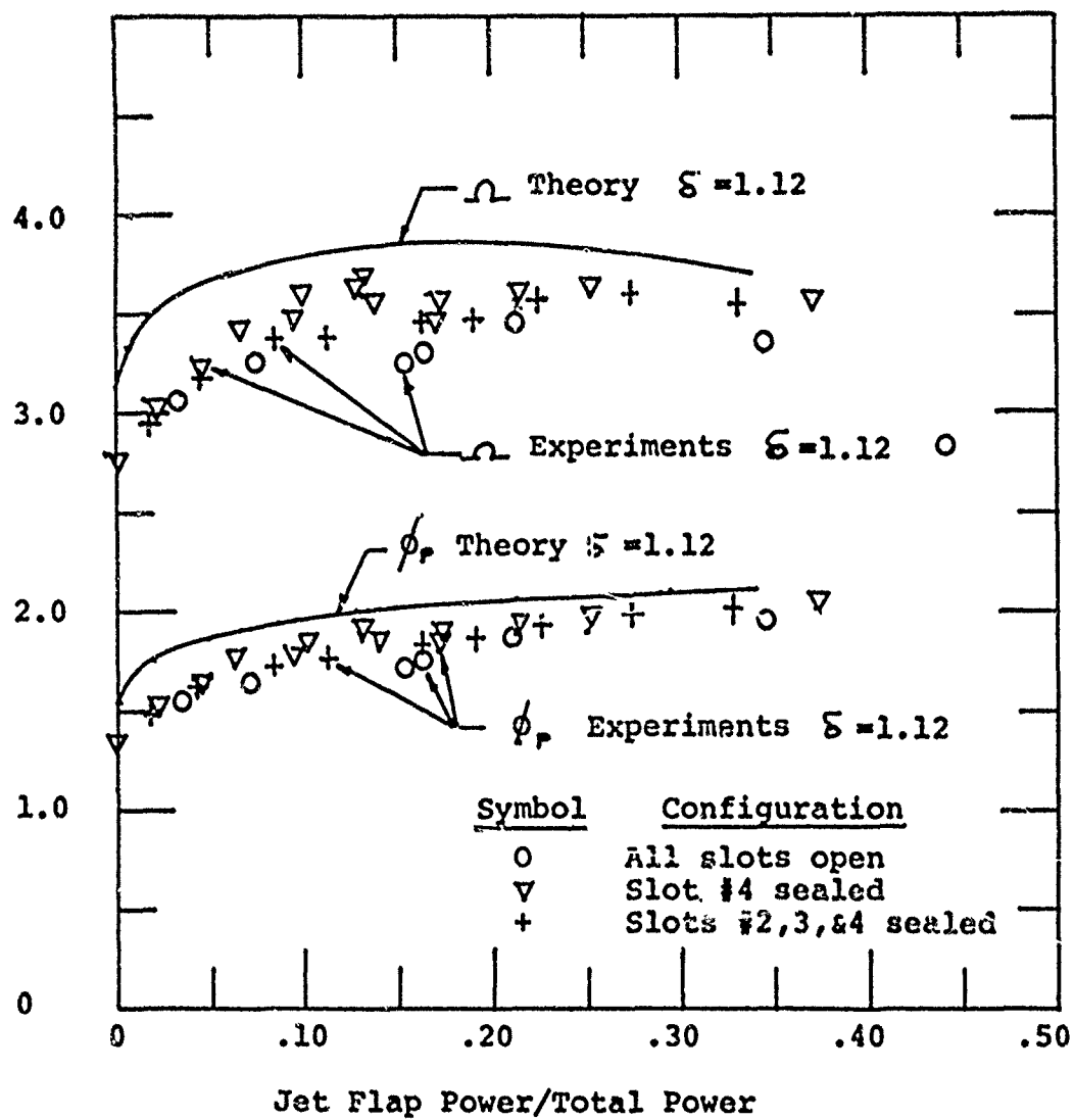
Figure 5. Coanda/JFD Ejector Performance A/a=16 s/a=3.0 \beta=30 degrees \zeta=1.12
