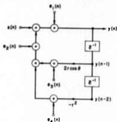
Fig. 6. Noisy second-order filter (floating point).
