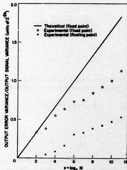
Fig. 15. Errors due to coefficient quantization in FFT.
