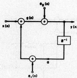
Fig. 5. Noisy first-order filter (floating point).
