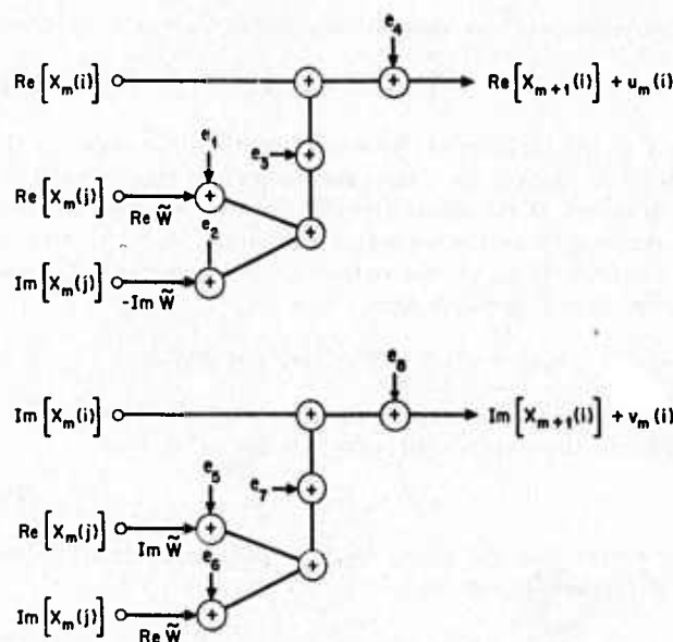
Fig. 12. Noisy butterfly computation (floating point).
