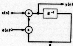
Fig. 3. Noisy first-order filter (fixed point).
