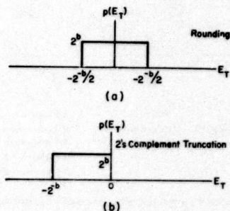
Fig. 2. (a) Probability density function for rounding noise. (b) Probability density function for noise due to two's-complement truncation.
