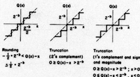
Fig. 1. Transfer characteristics for rounding and truncation.
