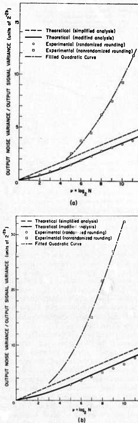
Fig. 13. (a) Experimental and theoretical noise-to-signal ratios for floating point FFT. (b) Experimental and theoretical noise-to-signal ratios for floating-point FFT and inverse.
