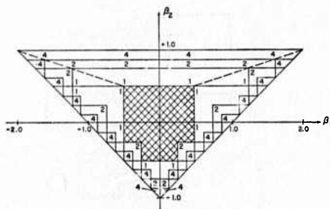
Fig. 7. Deadband subregions
