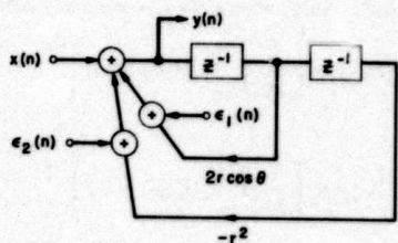
Fig. 4. Noisy second-order filter (fixed point).
