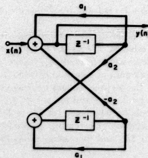
Fig. 18. Coupled form for second-order section.
