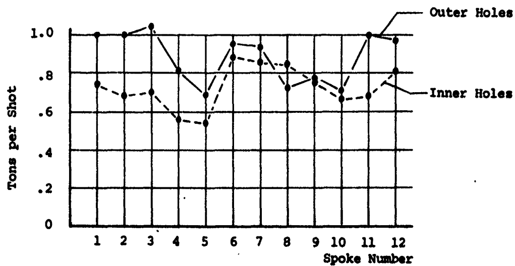
Figure 7 Blast Distribution Estimate
