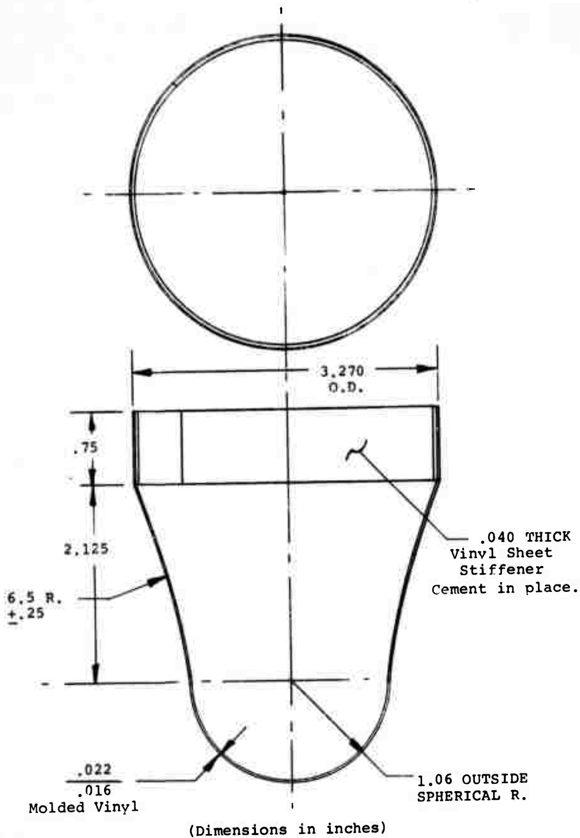
FIG. 7. WATER PACKAGE
