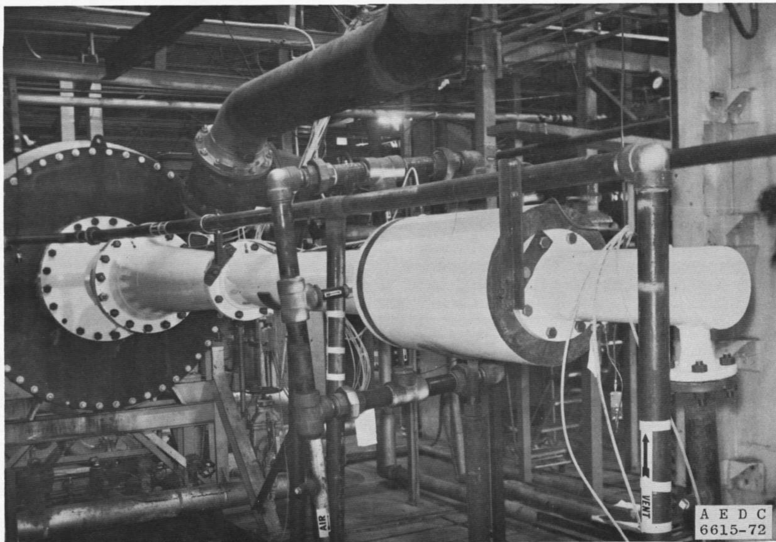
Fig. 3 Photograph of Model Induction Test Facility for Turbofan Engines
