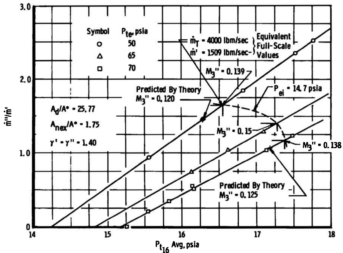
Fig. 5 Variation of Secondary-to-Primary Mass Flow Ratio ( \dot{m}''/\dot{m}' ) with Ejector Exit Total Pressure ( P_{t16} , avg)
