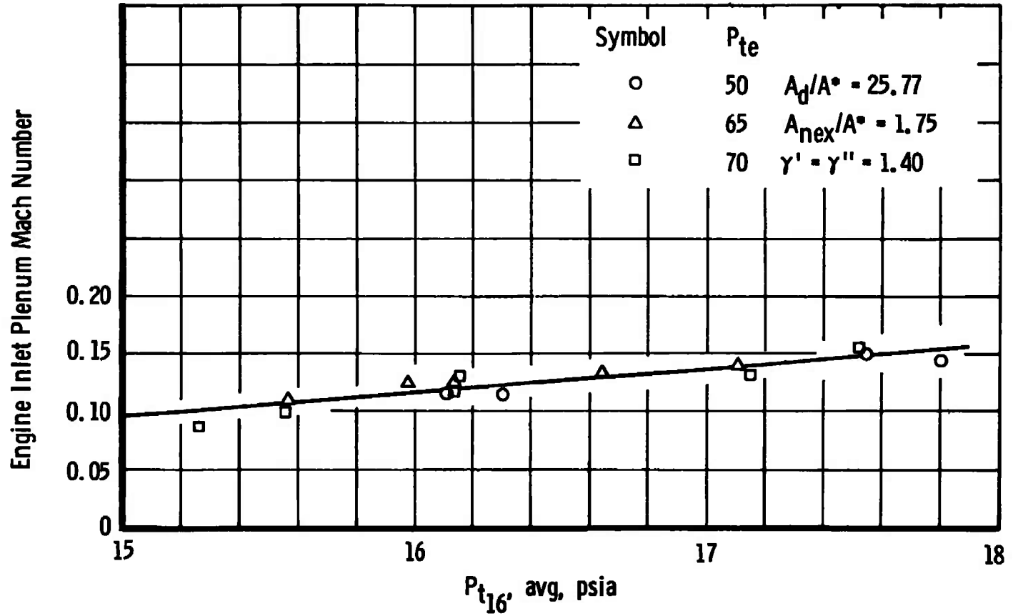
Fig. 6 Variation of Simulated Turbofan Engine Inlet Mach Number with Turbofan Engine Inlet Total Pressure ( P_{t16}, \text{ avg} )
