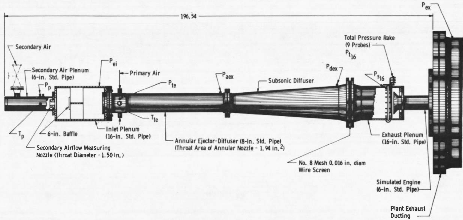
Fig. 2 Model Induction Test Facility for Turbofan Engines
