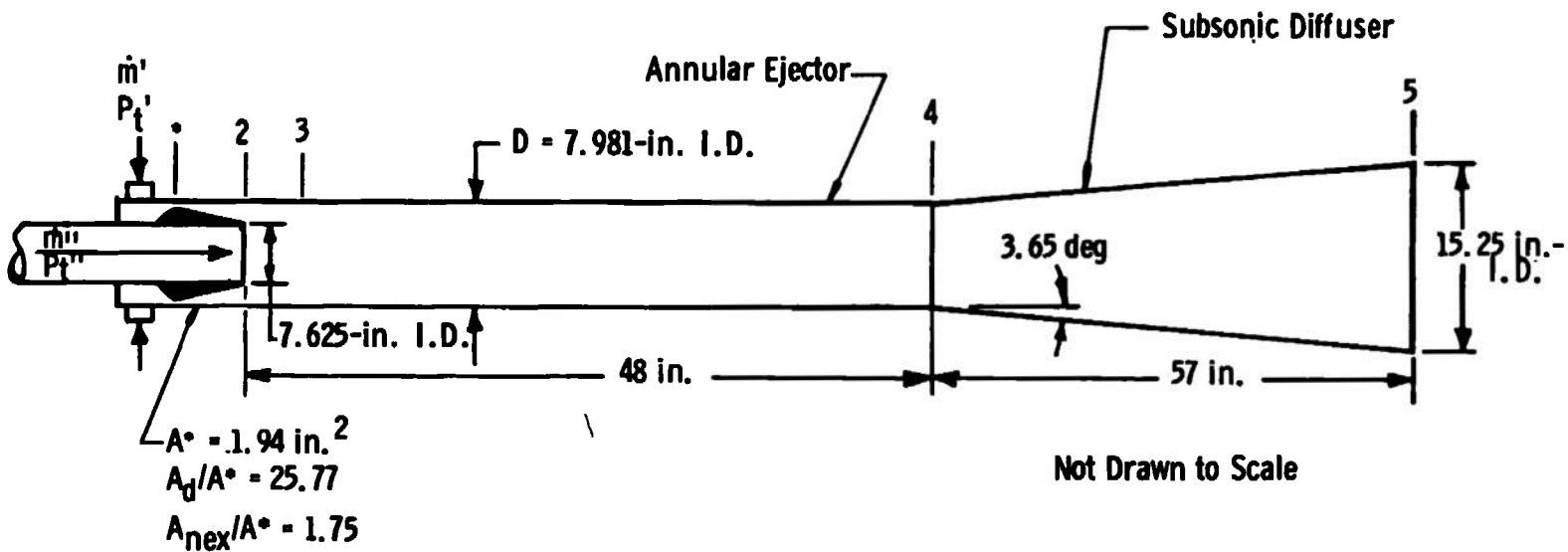
Fig. 1 Model Air-Driven Annular Ejector
