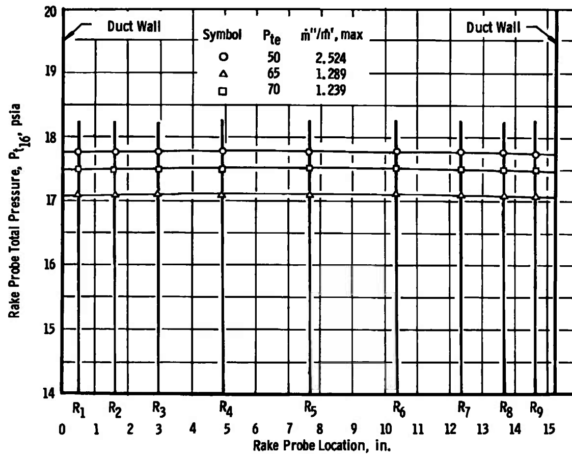
Fig. 7 Simulated Turbofan Engine Inlet Total Pressure Profile
