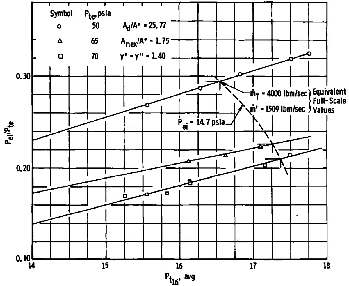
Fig. 4 Variation of Ratio of Ejector Inlet to Ejector Driving Pressure ( P_{ei}/P_{te} ) with Ejector Exit Total Pressure ( P_{t16}, \text{ avg} )
