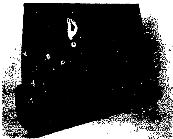
Fig. 14 Exit Damage from 7.62 mm Ball Ammunition
