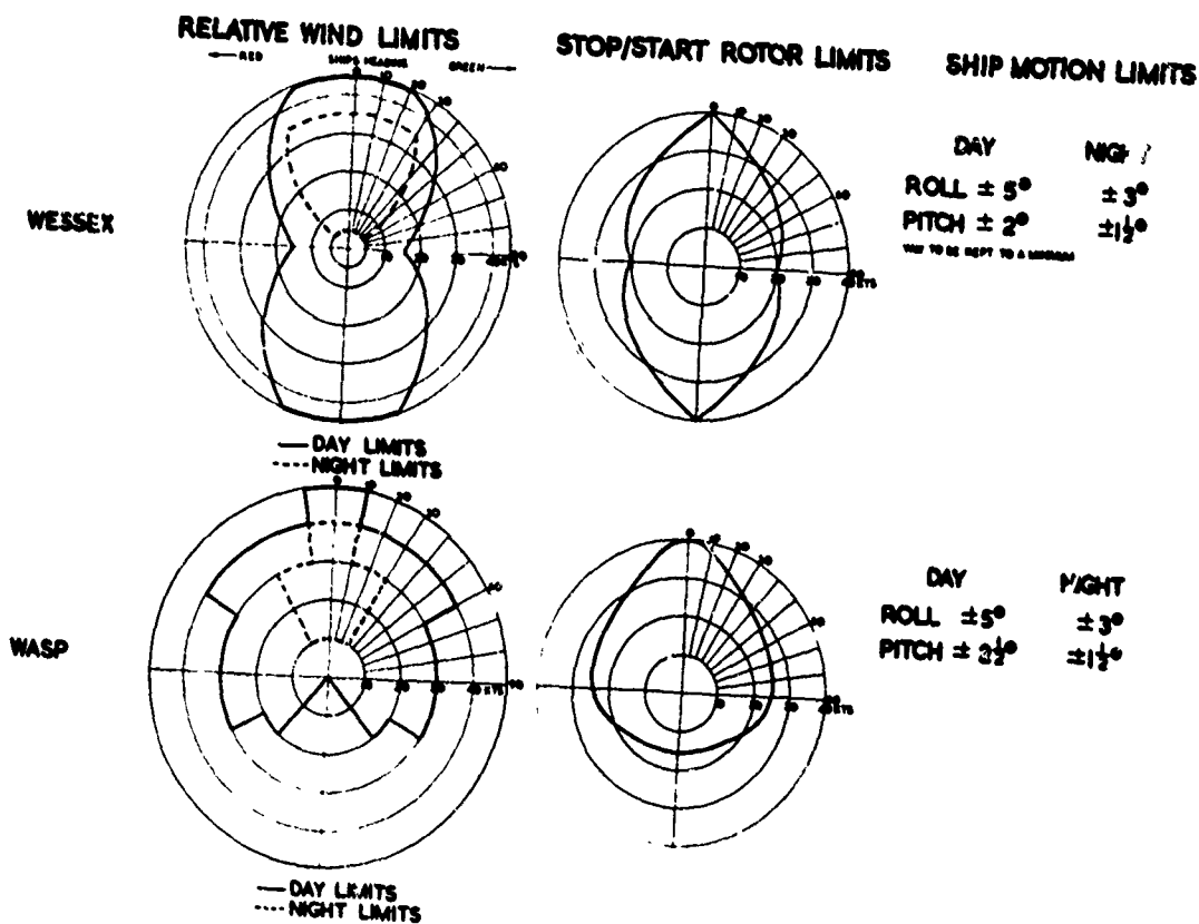
FIG. 5 RELATIVE WIND AND SHIP MOTION LIMITS
