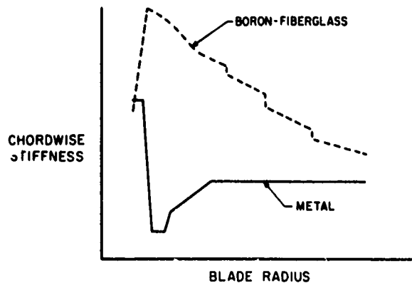
Figure 7. Stiffening Effect of Composite Construction.
