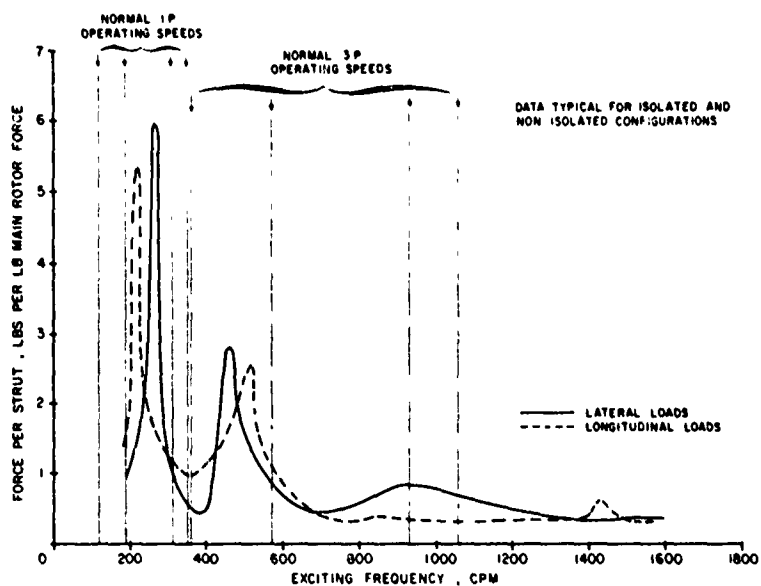
TRANSMISSIBILITY OF ROTOR INPLANE LOADS TO THE FORWARD MODULE SUPPORTS
