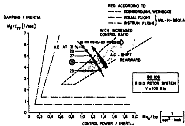
Fig. 15 Effect of A.C. Offset on Control Characteristics (Pitching)
