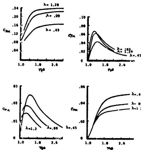
11-222 VARIATION OF DERIVATIVES WITH FLAP FREQUENCY, LAG FREQUENCY CONSTANT (=10.0)
