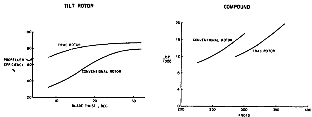
Figure 11. Pay-off From Retractable Rotor.
