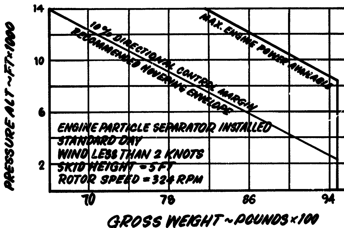
FIGURE 3 AH-1G ICE HOVERING PERFORMANCE
