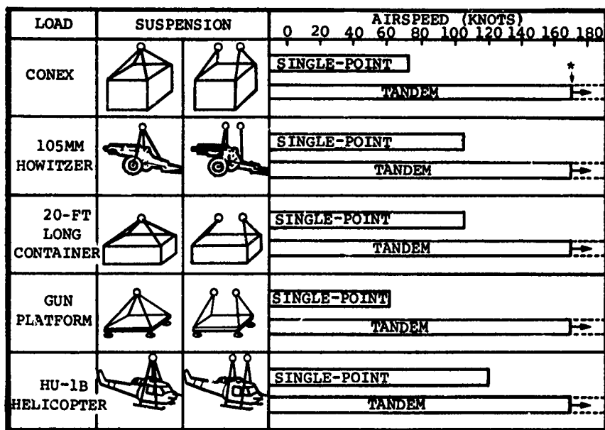
Figure 3. Stability Comparison of Single-Point and Tandem Suspensions
