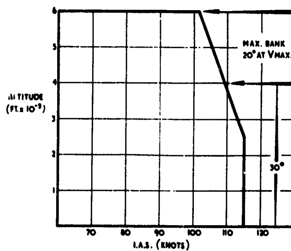
FIG. 18. FLIGHT ENVELOPE
