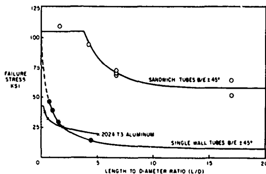
Figure 12. Effect of Sandwich Construction on Torsional Elastic Stability Limits.
