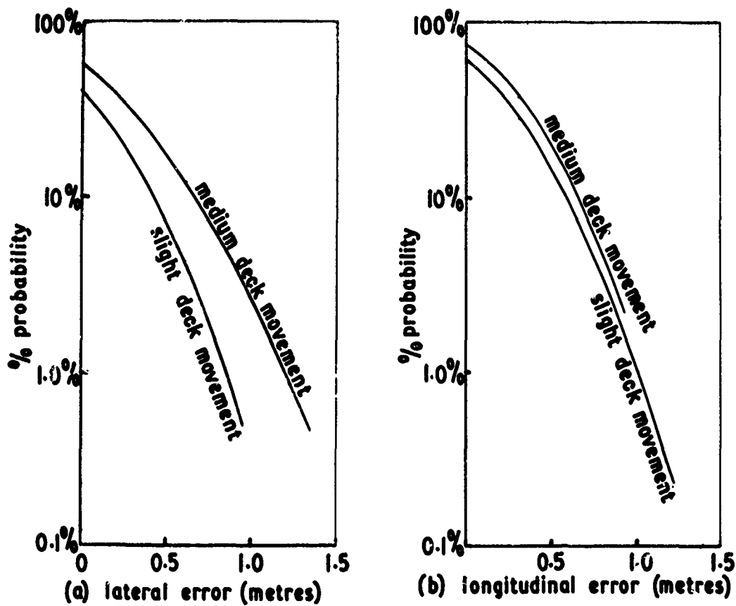
FIG.11 EFFECT OF SEA STATE ON PROBABILITY OF LANDING POSITION ERROR
