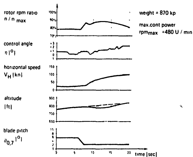
Fig. 13 Printed simulator flight, forward transition for H3
