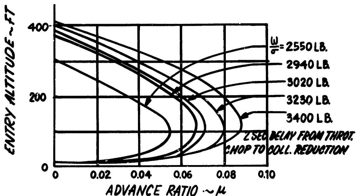
FIGURE 4 OH-58A MAX. PERFORMANCE HEIGHT VELOCITY PROFILES
