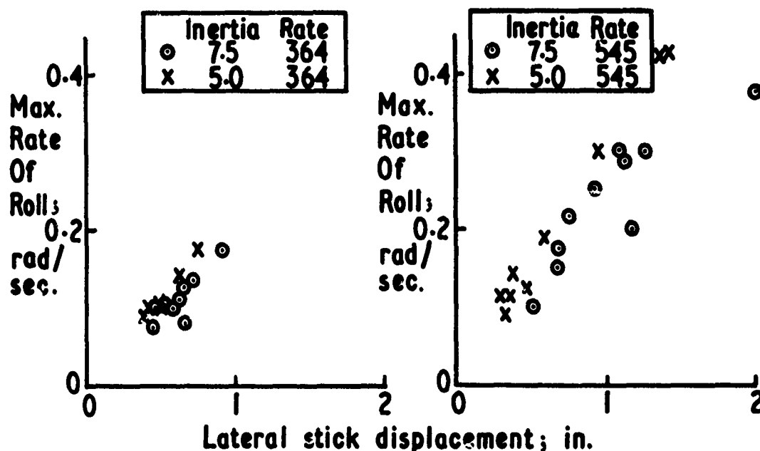
FIG.5 THE VARIATION OF MAX. ROLL RATE WITH STICK DISPLACEMENT FOR VARIOUS GYRO INERTIA & SPRING RATES IN HOVERING
