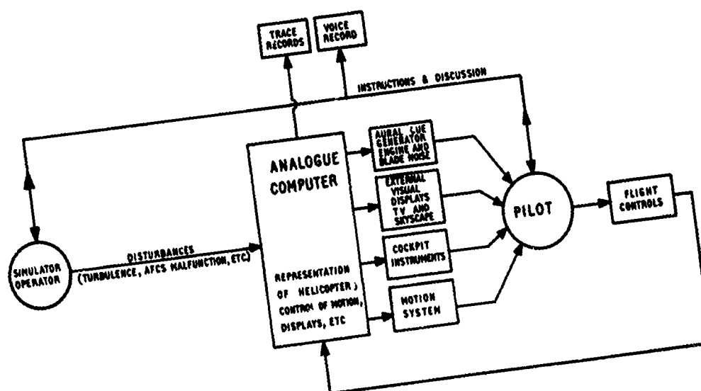
Fig 2 Westland Lynx
