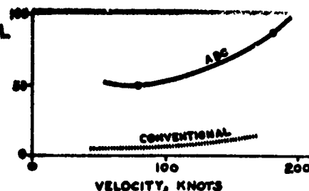
Fig. 35 Pitch Control Moment Normalized by Inertia (rad/sec 2 /rad) vs. Speed (knots)
