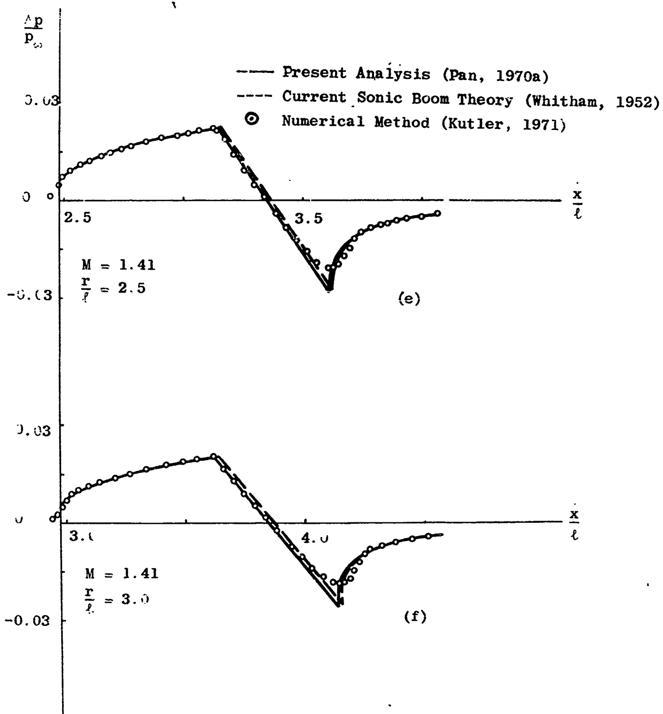
FIGURE 2.1.7 Near-field pressure signatures
