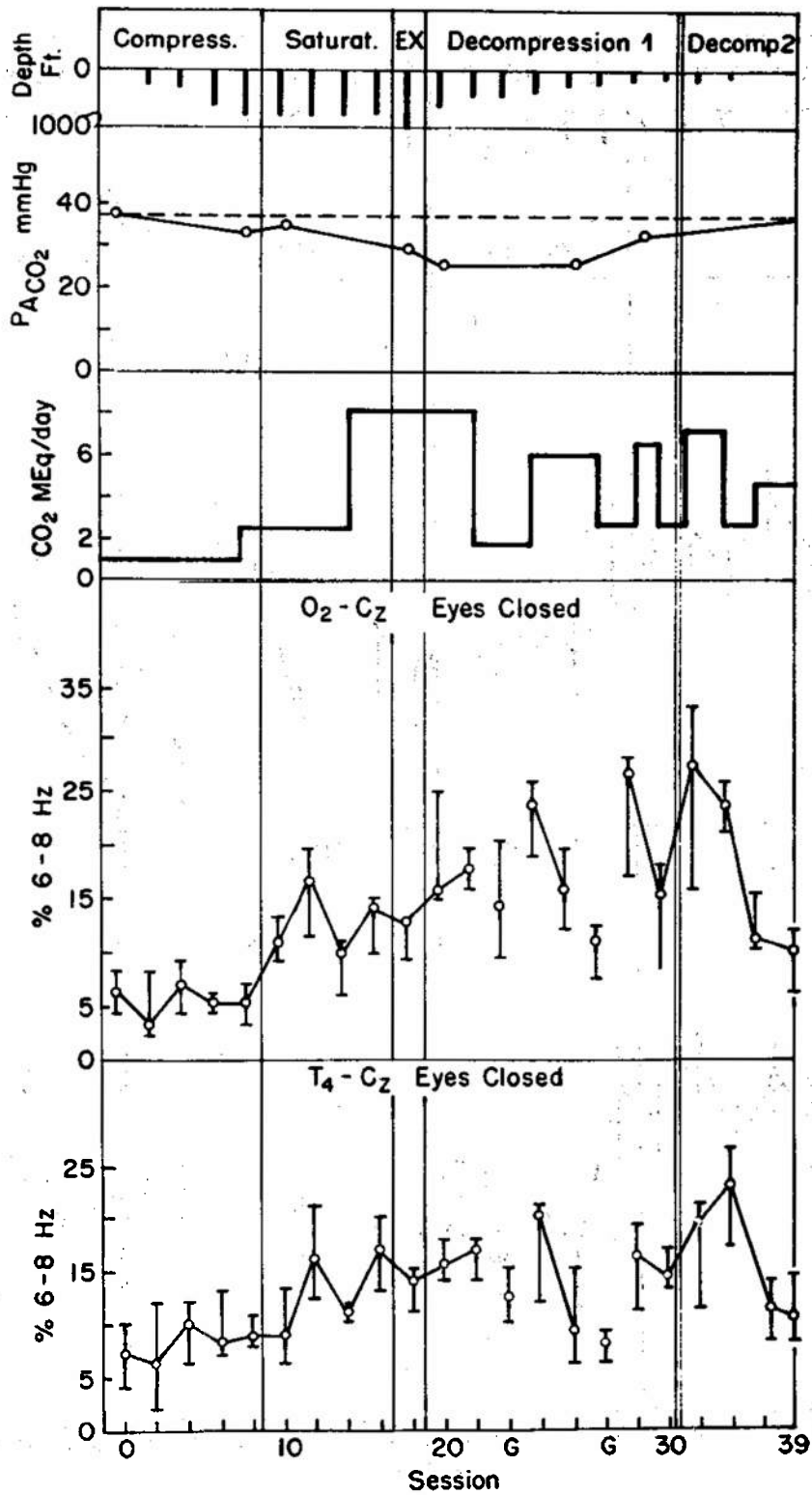
Fig. 4. Subject C. D. Time course in alveolar carbon dioxide tension, urinary \text{CO}_2 excretion and EEG changes, (percent 6-8 Hz frequency), two electrode positions \text{O}_2 - \text{C}_z and \text{T}_4 - \text{C}_z , eyes closed.
