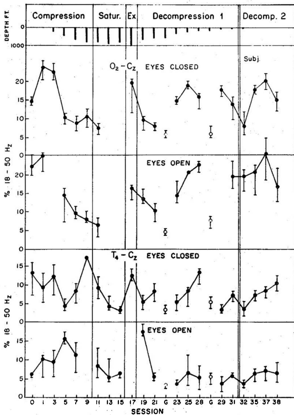
Fig. 10. Subject D. F. Time course of changes in the high frequency band (18-50 Hz) during saturation-diving experiment. Two electrode positions O_2 - C_z and T_4 - C_z . Eyes closed and open, marked changes during compression period and during inhalation of nitrogen-oxygen gas mixtures.
