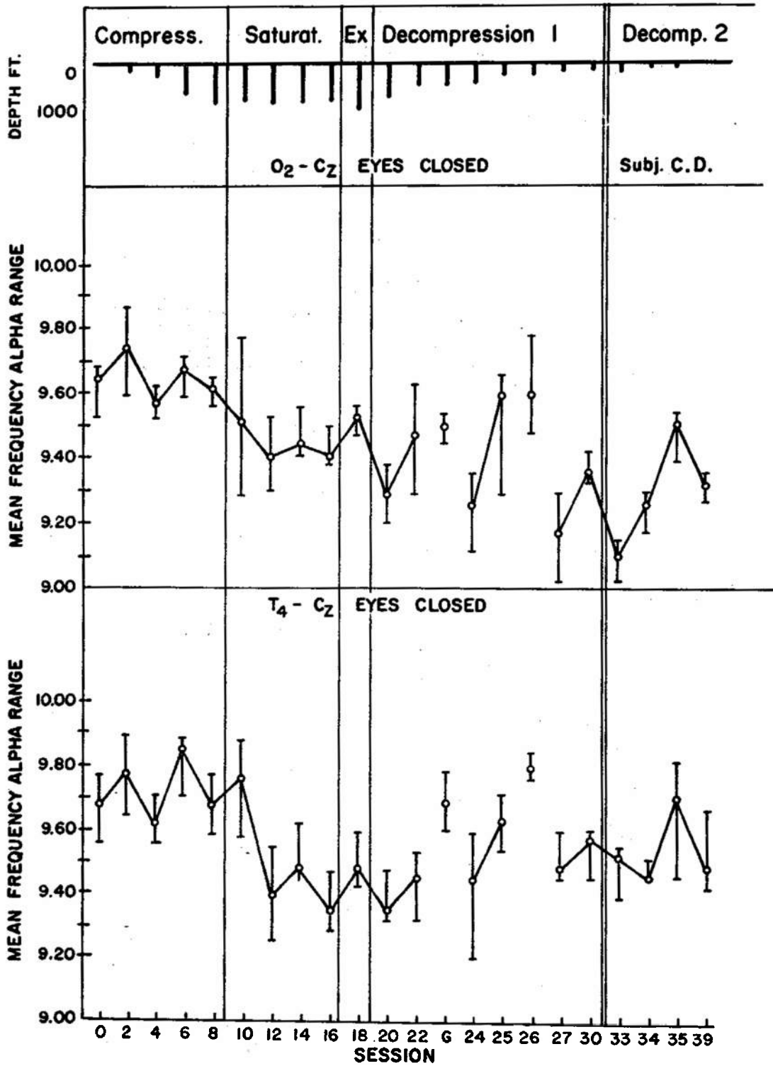
Fig. 3. Subject C. D. Mean frequency changes in the alpha range during the saturation diving experiment. Eyes closed. Two electrode positions: O_2 - C_z and T_4 - C_z . Sessions with exercise are not included.
