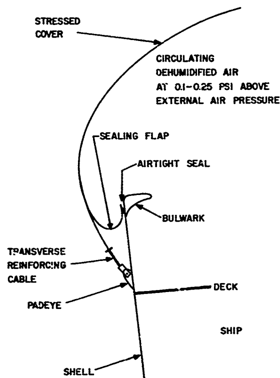
Figure 1 Topside Encapsulation Concept
