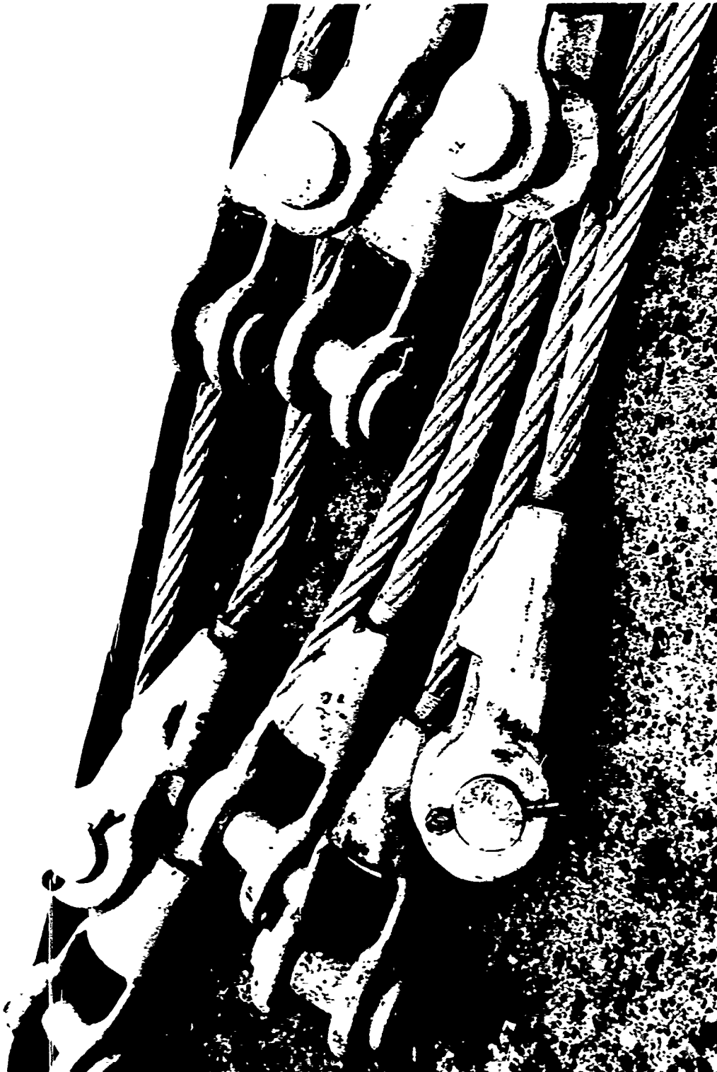
Figure 6-M Transverse Cables Fitted into Sockets of Clevis Assemblies
