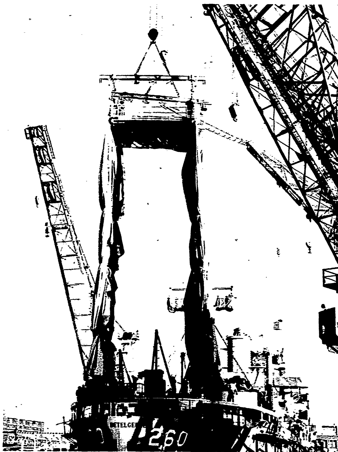
Figure 10-M Cover Lifted Over Stern
