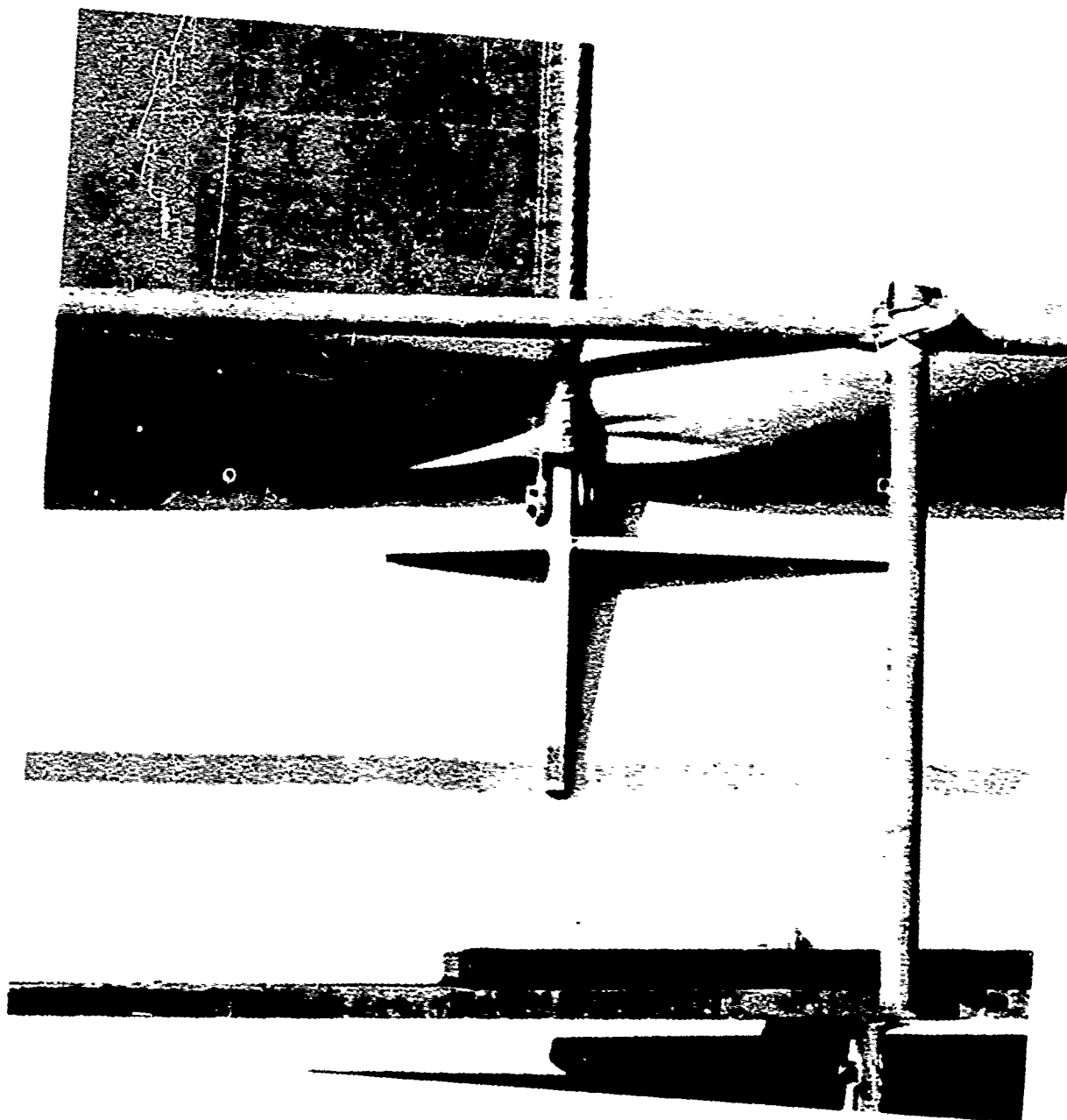
Figure 7-M Attachment of Transverse Cable to Padeye
