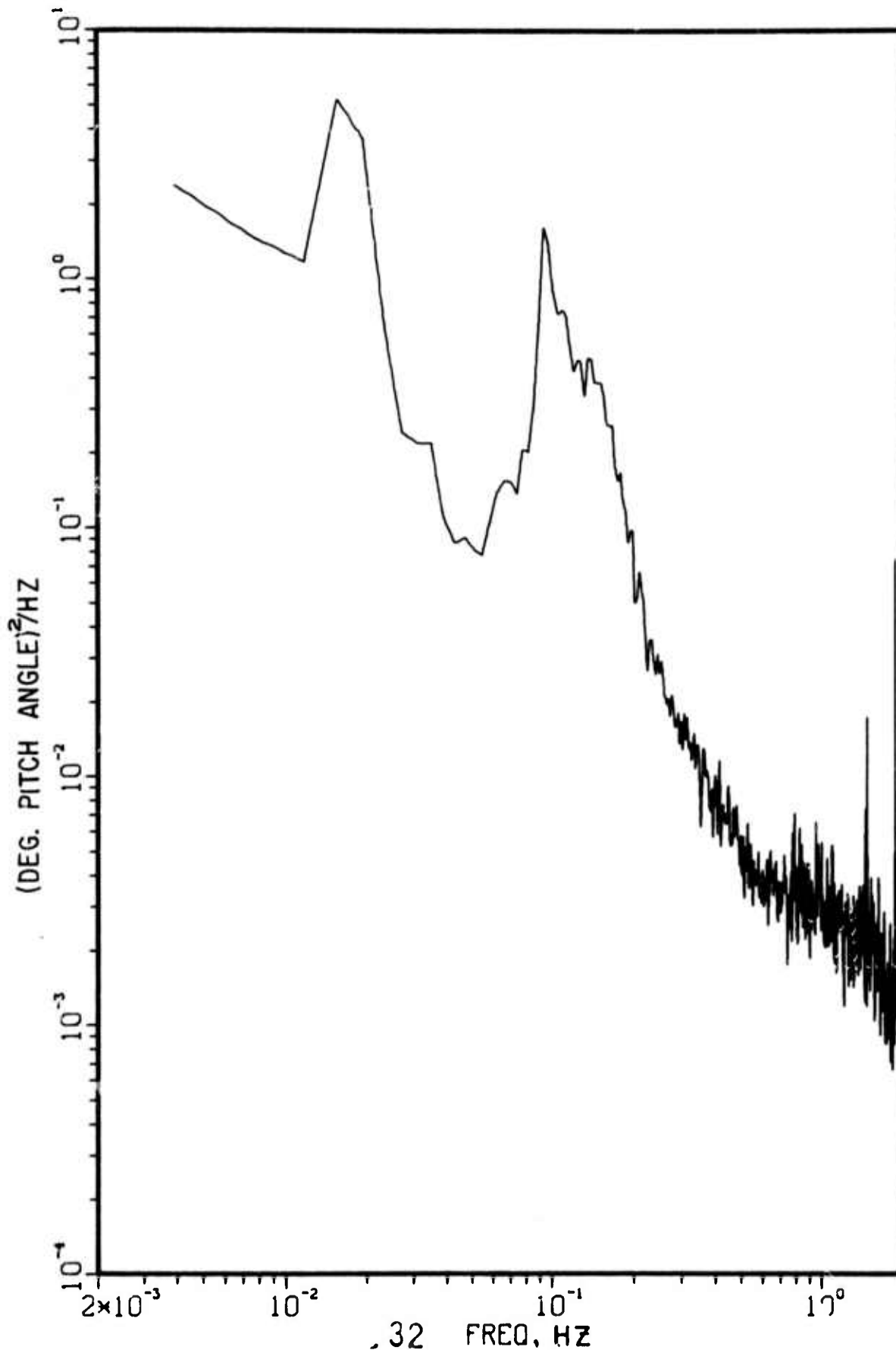
FIGURE 4 M3D4 GYRO FILE 6 , DEG.
