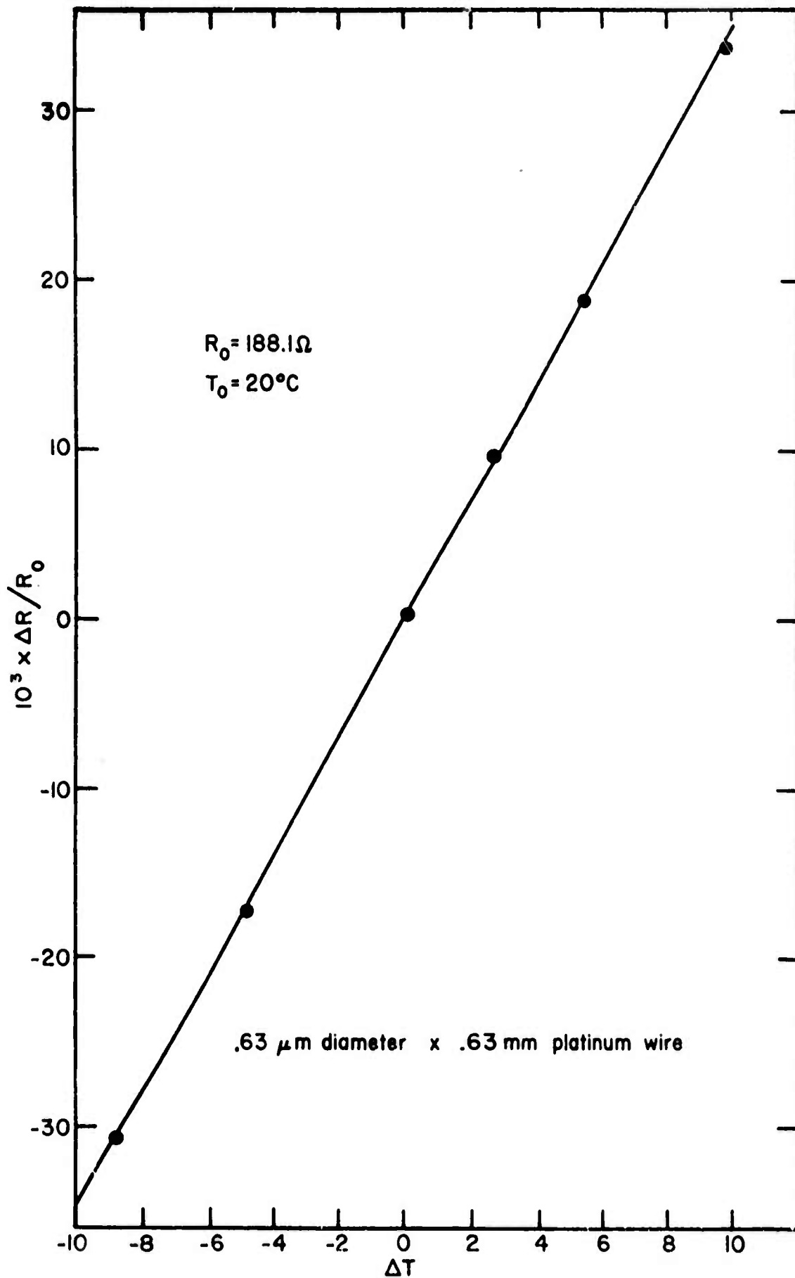
FIGURE 3: RESISTANCE VS TEMPERATURE.
