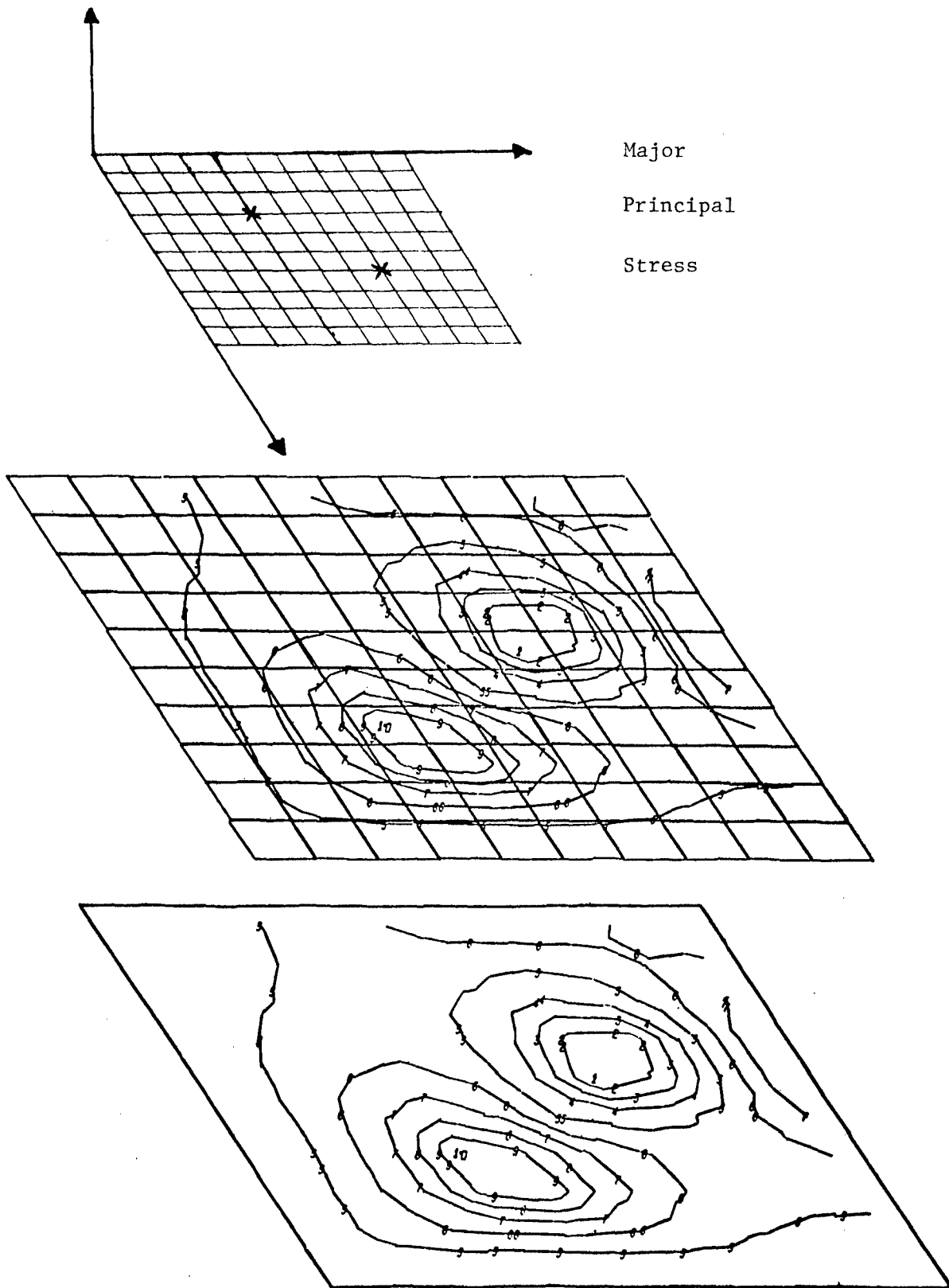
Figure 3. Sample Output - Major Principal Stress
