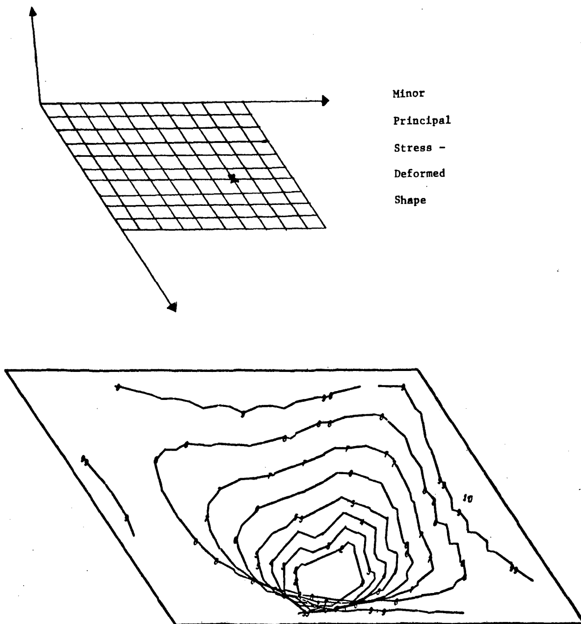
Figure 4. Sample Output - Minor Principal Stress
