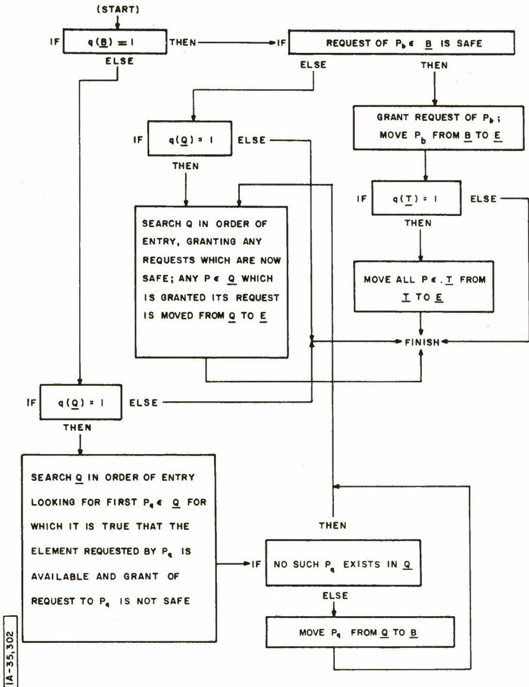
Figure 1. Scheduler Algorithm: Release of an Element
