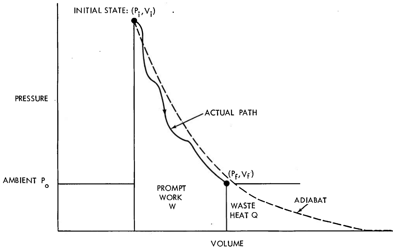
FIG. 1.3-1 PROMPT BLAST ENERGY AND WASTE HEAT.
