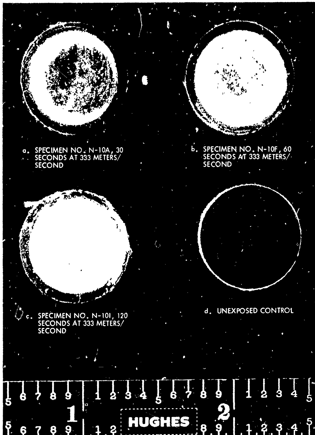
Figure 1. Four ex 120 film specimens (top) and 120 film (bottom) exposed at 333 meters/second for 30, 60, and 120 seconds.
