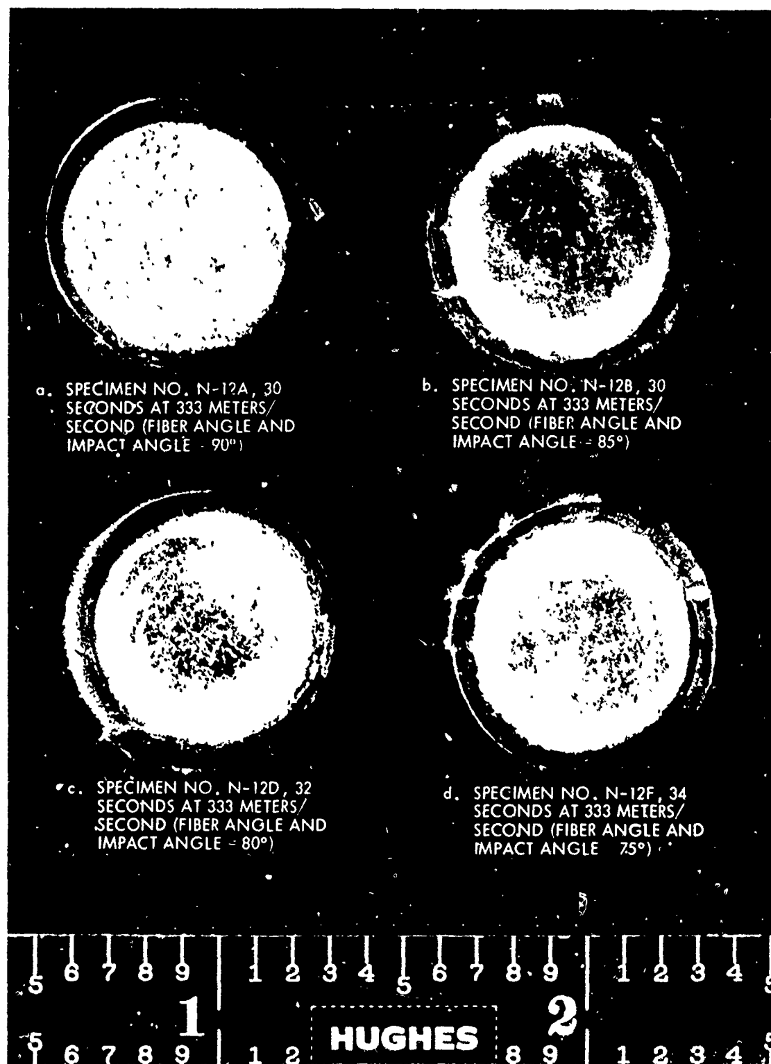
Figure 4. N-12 ex 1200 fiber-reinforced polymer (FRP) specimens showing average reinforcement content (1.2% to 1.4% by weight).
