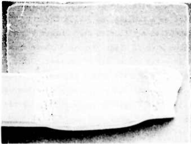
Figure 2: SEM photomicrograph of a ribbon wire first bond made with low power [20-min. (0.5- \mu\text{m} ) peak-to-peak tip amplitude] and long time [155 ms] (Magnification \sim 470\text{X} ).
