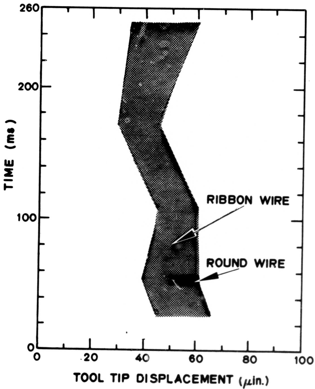
Figure 10: Time and tool tip displacement settings used in this work that yield bonds with a pull strength of 10 gf or greater.
