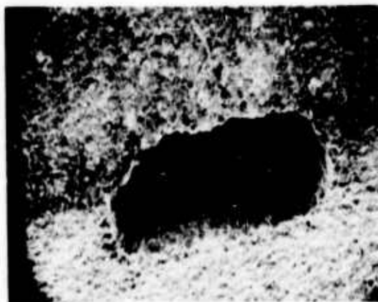
Figure 1: SEM photomicrograph of a rectangular wire-feed hole in an ultrasonic bonding tool. (There is a slight build up of aluminum in the upper left corner of the hole. Magnification: about 750X.)
