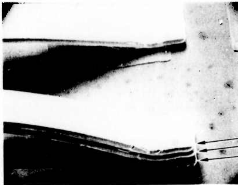
Figure 5: SEM photomicrograph of three stacked bonds (shown by arrows) made with aluminum ribbon wire with cross-sectional dimensions 3 by 0.5 mils on a 5-mil square bonding pad (Magnification \sim 200X)
