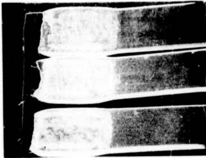
Figure 4: SEM photomicrograph of three bonds made with aluminum ribbon wire with cross-sectional dimensions 1.5 by 0.5 mils on a bonding pad 5-mils square. (The bonding schedule was low power [32- \mu in. (0.8- \mu m) peak-to-peak tool tip amplitude] and medium time [80 ms]. Magnification \sim 460X).
