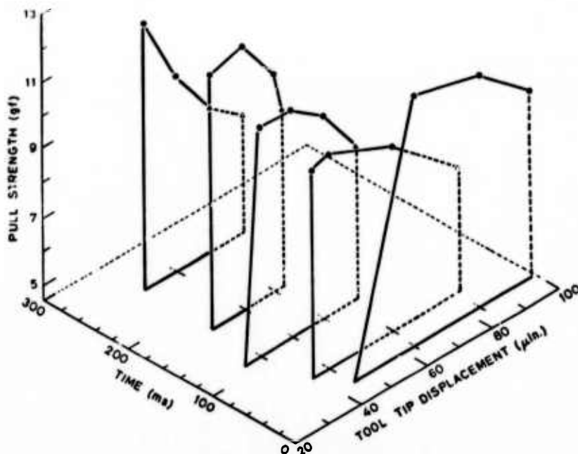
Figure 8: Pull strength of ribbon wire bonds as a function of time and tool tip displacement; bonding force of 35 gf. (Bond pull strength range is shown as in figure 6.)
