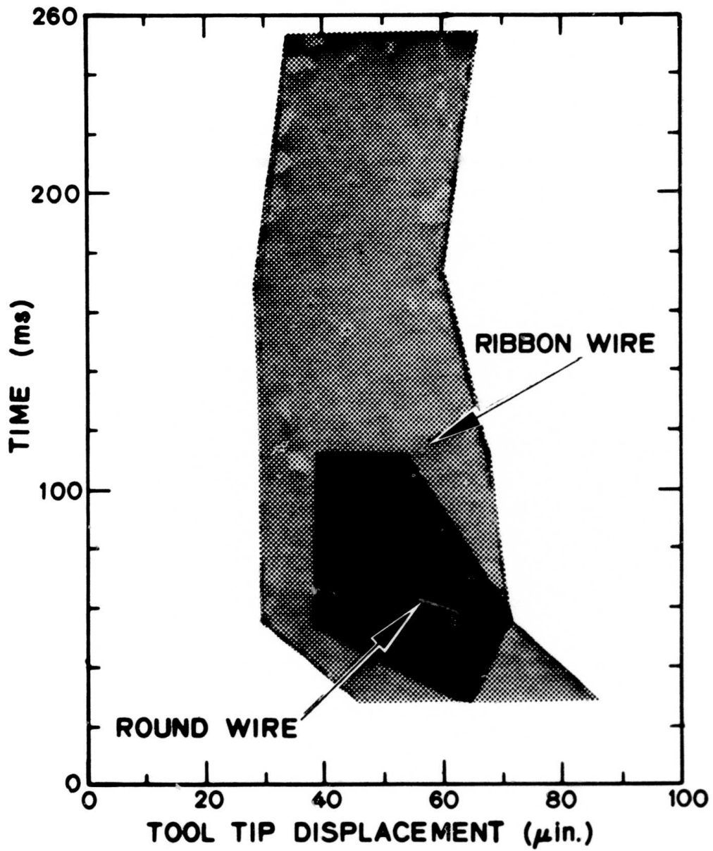
Figure 9: Time and tool tip displacement settings used in this work that yield bonds with a pull strength of 7 gf or greater.
