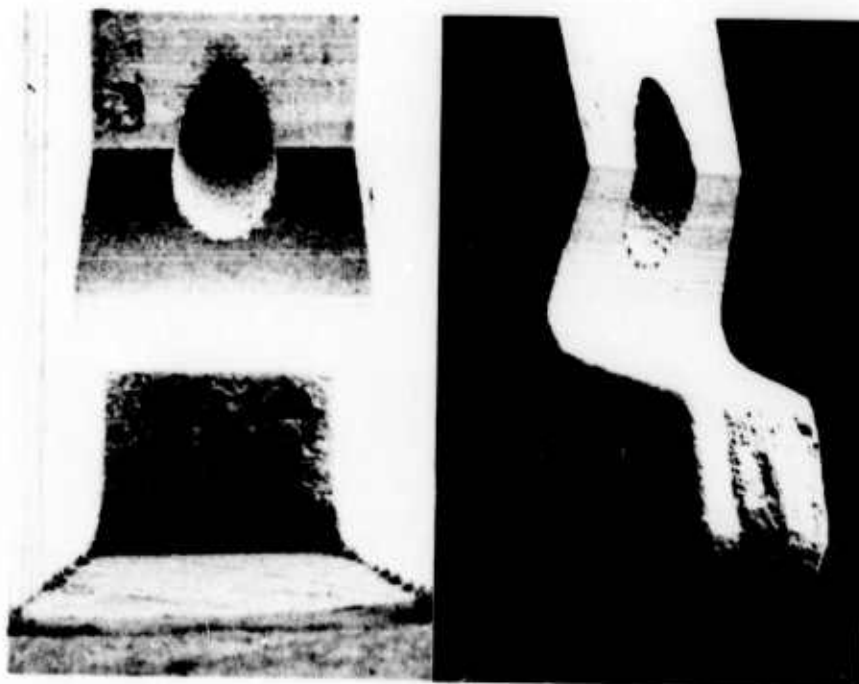
Figure 15: SEM photomicrograph (magnification ~200X) of two views of a tungsten carbide bonding tool showing build-up of gold at the wire feed hole.
