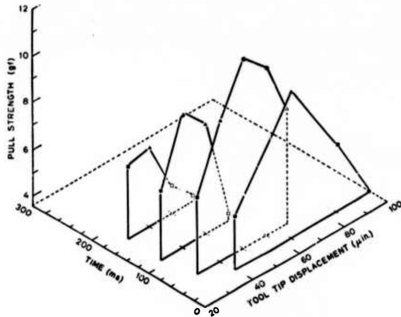
Figure 7: Pull strength of round wire bonds as a function of time and tool tip displacement. (Bond pull strength range is shown as in figure 6.)
