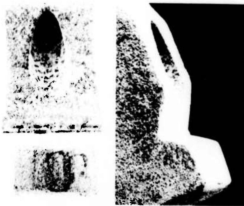
Figure 12: SEM photomicrograph (magnification 240X) of two views of a bonding tool showing rough surface finish.
