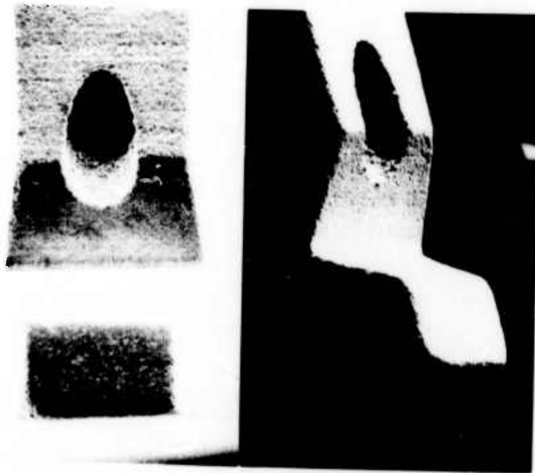
Figure 14: SEM photomicrograph (magnification ~190X) of two views of a bonding tool showing pin holes in the surface finish.
