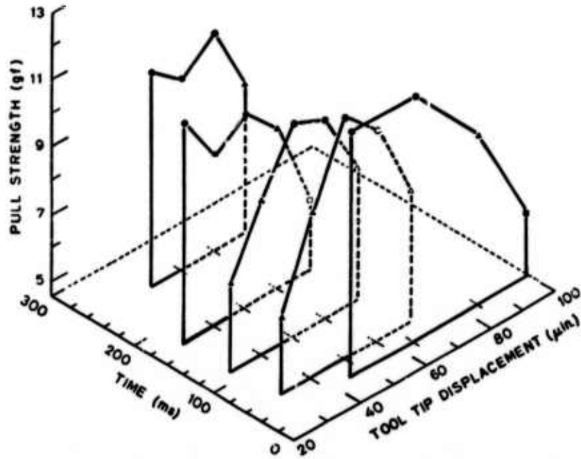
Figure 6: Pull strength of ribbon wire bonds as a function of time and tool tip displacement. (Bond pull strength range is shown by symbols: ●, ○ > 10 gf; ▲, △ 7-10 gf; and ■, □ < 7 gf.)
