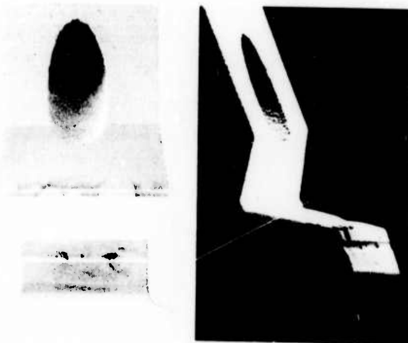
Figure 13: SEM photomicrograph (magnification 200X) of two views of a bonding tool with a relatively smooth surface finish.
