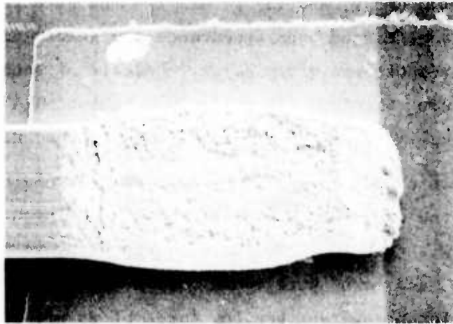
Figure 3: SEM photomicrograph of a ribbon wire first bond made with high power [82-min. (2.1- \mu\text{m} ) peak-to-peak tool tip amplitude] and relatively short time [40 ms] (Magnification \sim 500\text{X} ).
