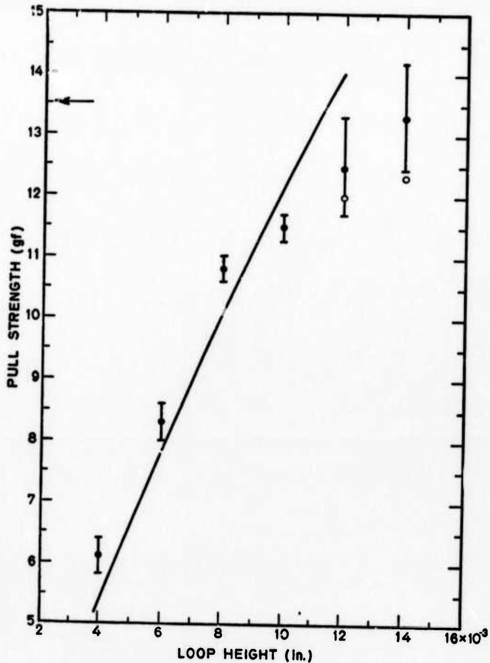
Figure 11: Pull strength of ribbon wire bonds as a function of loop height. (The data points represent the mean for up to 10 bonds. Solid circles include only bonds which ruptured at the heel; open circles include both bonds which ruptured at the heel and which failed by lift off. Error bars represent one sample standard deviation. The solid curve is calculated from resolution-of-forces using the wire tensile strength indicated by the arrow.)
