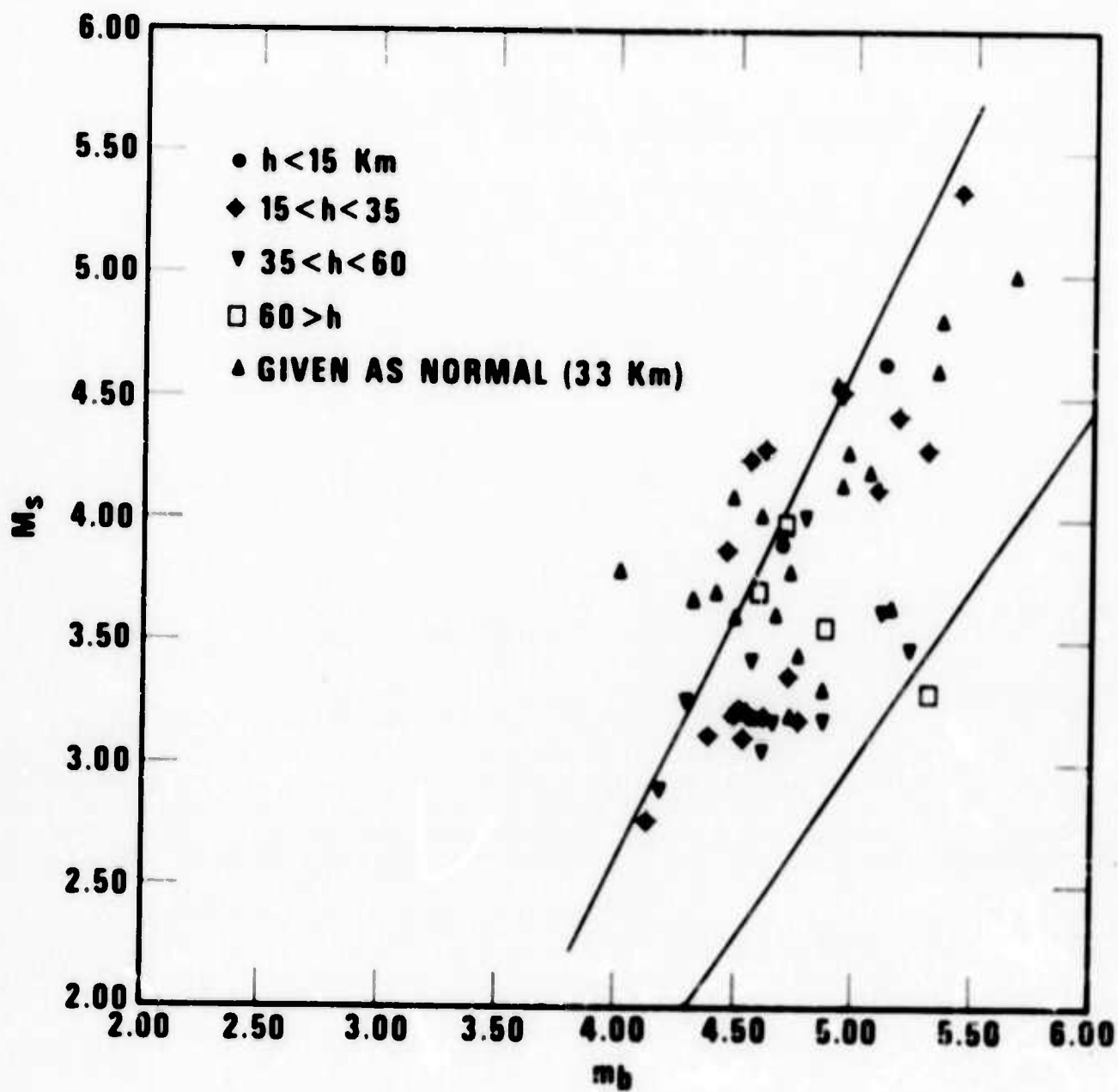
Figure 14. M_s vs m_b values corrected for mean station magnitude differences prior to averaging. Marshall and Basler method was used for M_s . No depth corrections were applied.
