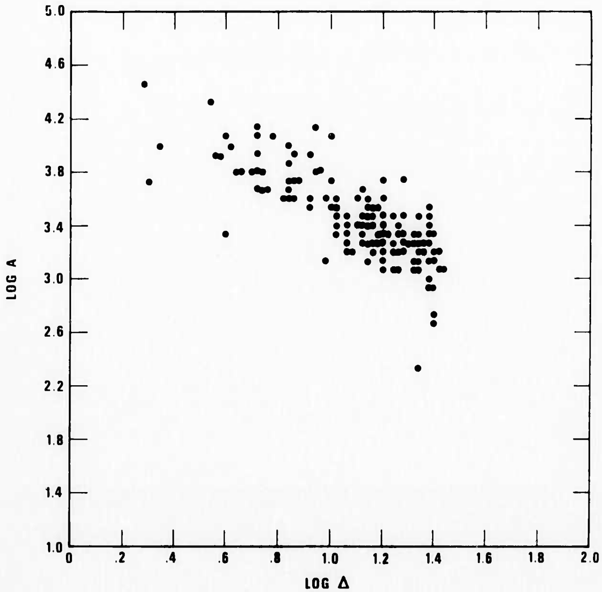
Figure 22b. Rayleigh wave log A vs log Δ plots before and after the application of station corrections determined by the joint magnitude determination method.
