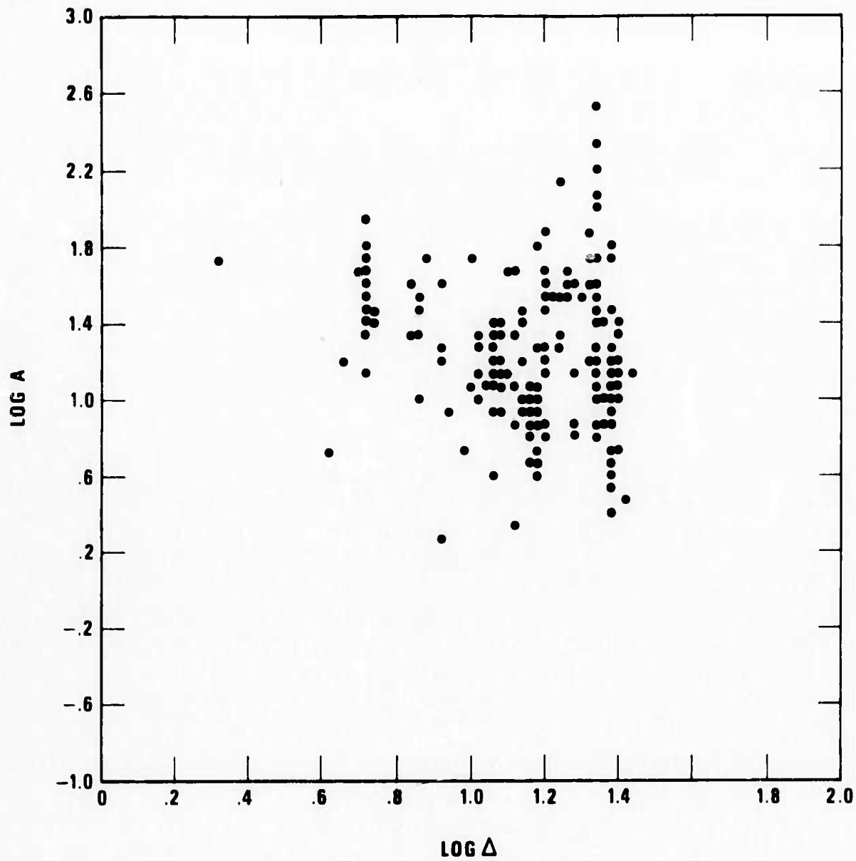
Figure 21a. P wave log A vs log Δ plots before and after the application of station corrections determined by the joint magnitude determination method.
