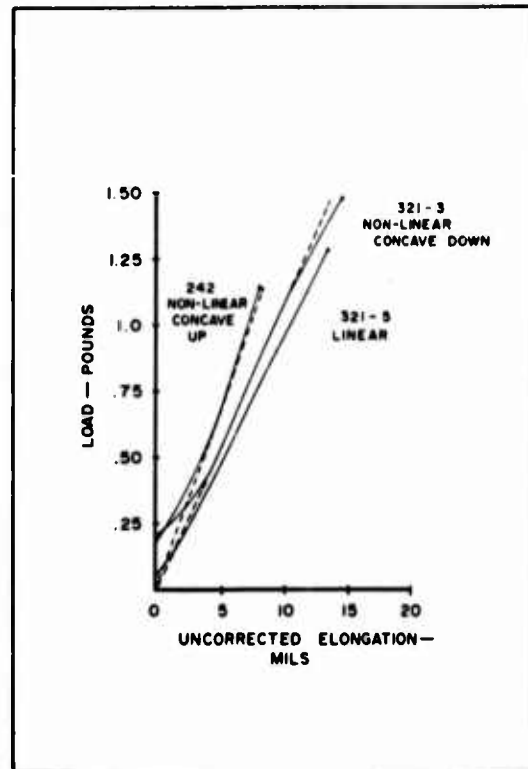
FIGURE 37. LOAD ELONGATION TENSILE CURVES
