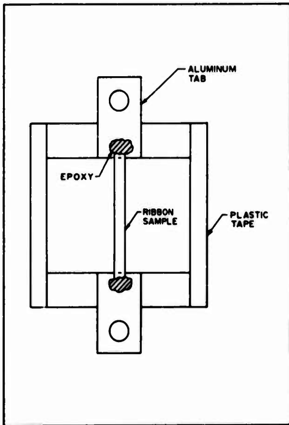
FIGURE 8. FILM SPECIMEN MOUNT
