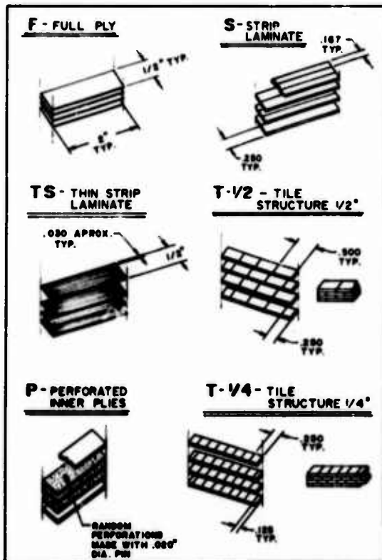
FIGURE 56. TEST LAMINATE STRUCTURES
