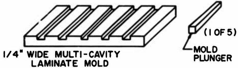
FIGURE 15. MULTI-CAVITY MOLD
