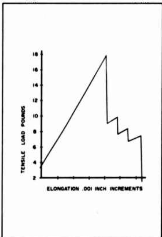
FIGURE 28. LOAD ELONGATION NO. 316-4
