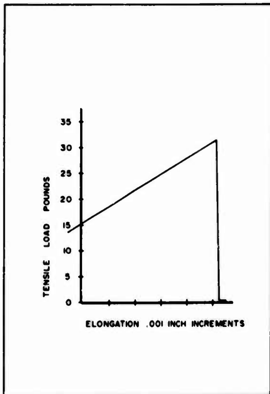
FIGURE 26. LOAD ELONGATION NO. T-14-A
