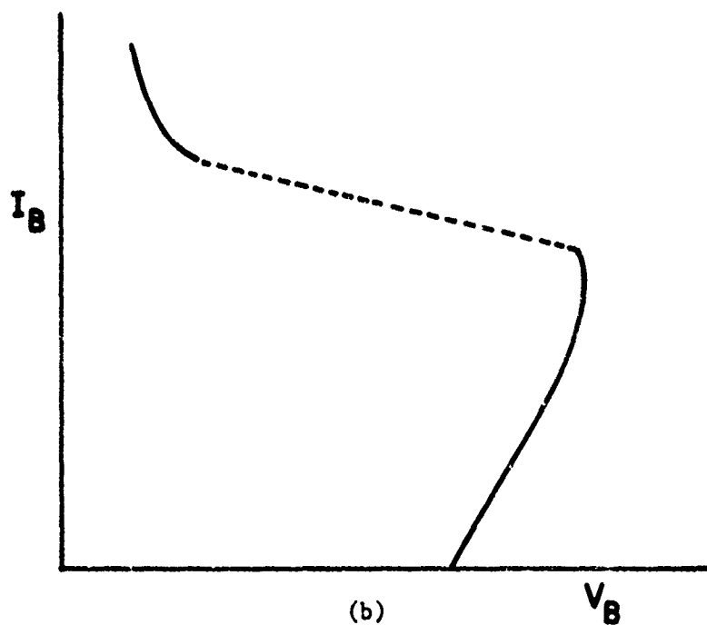
Fig. 20. Second breakdown characteristics of semiconductor devices. (a) Transistors, showing breakdown under forward F, open O, and reverse R base biasing. (b) Diode breakdown in the reverse biased direction.
