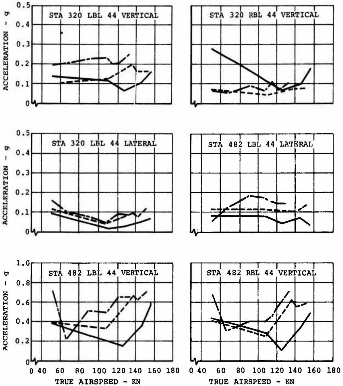
Figure 82. Effect of Gross Weight on 3/Rev Vibration Levels at Stations 320 and 482 During Flight Test of Boron Blades.
