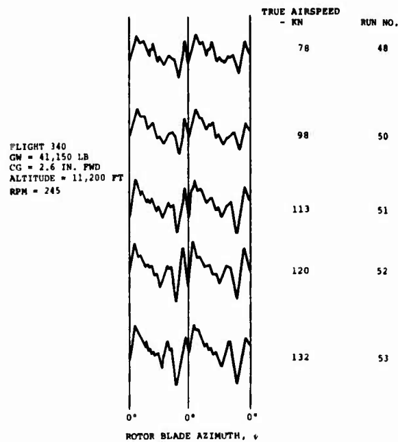
Figure 111. Pitch Link Load Waveforms During Flight Test of the Boron Advanced-Geometry Blades.
