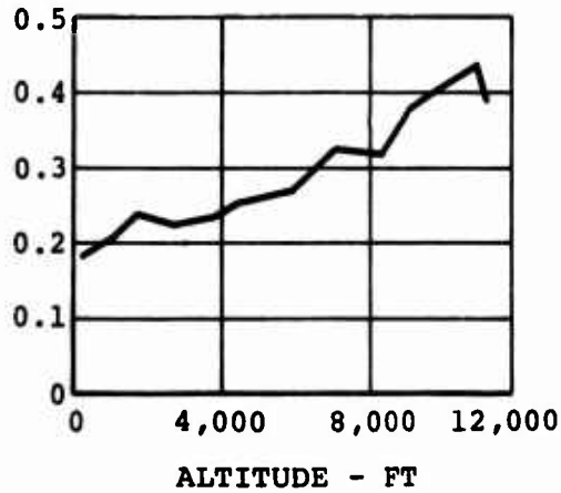
Figure 86. Effect of Altitude on 3/Rev Vibration Levels at Stations 320 and 482 and at Pilot Seat During Flight Test of Boron Blades.
