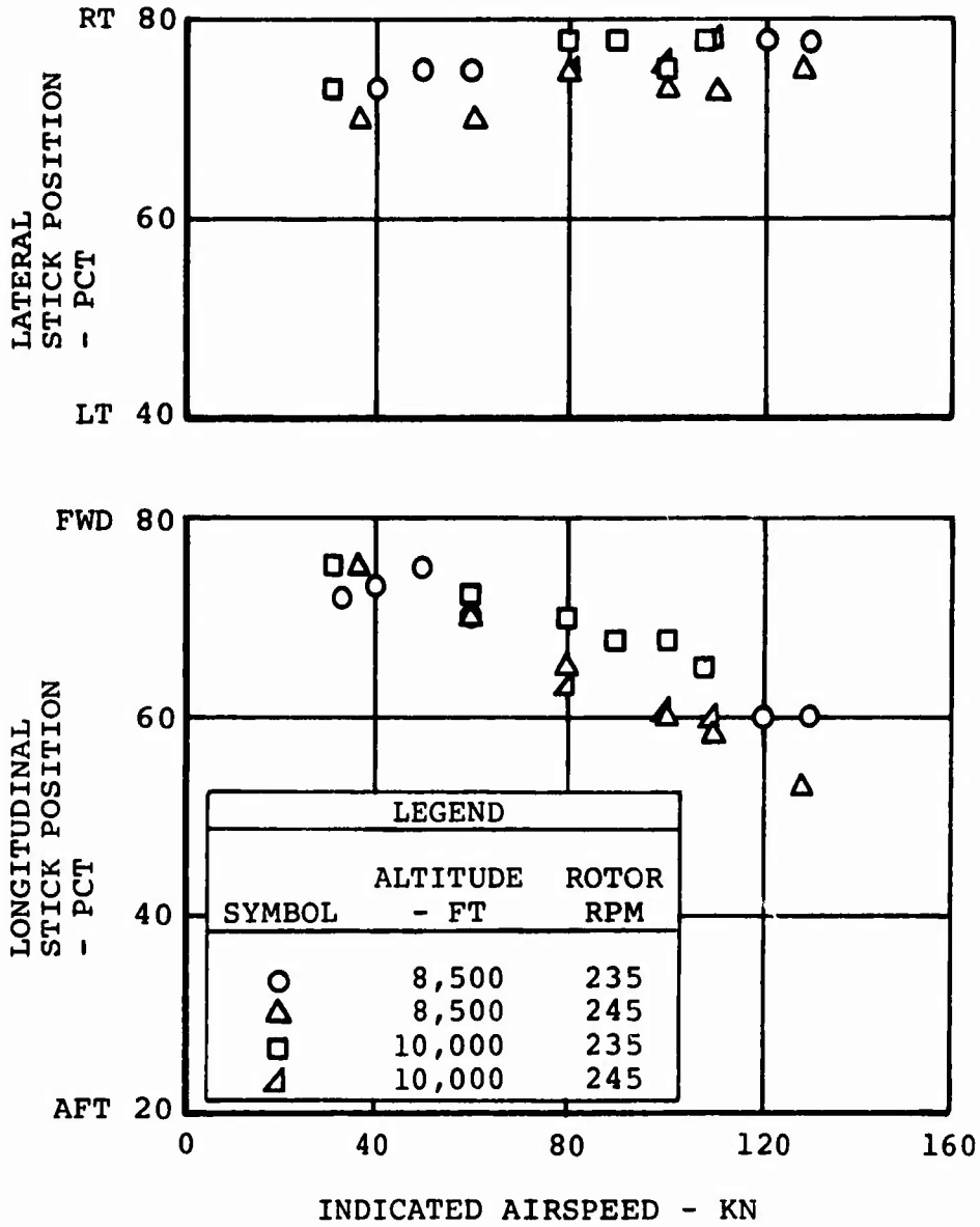
Figure 95. Aircraft Trim Control Positions During Flight Test of the Boron Advanced-Geometry Blades.
