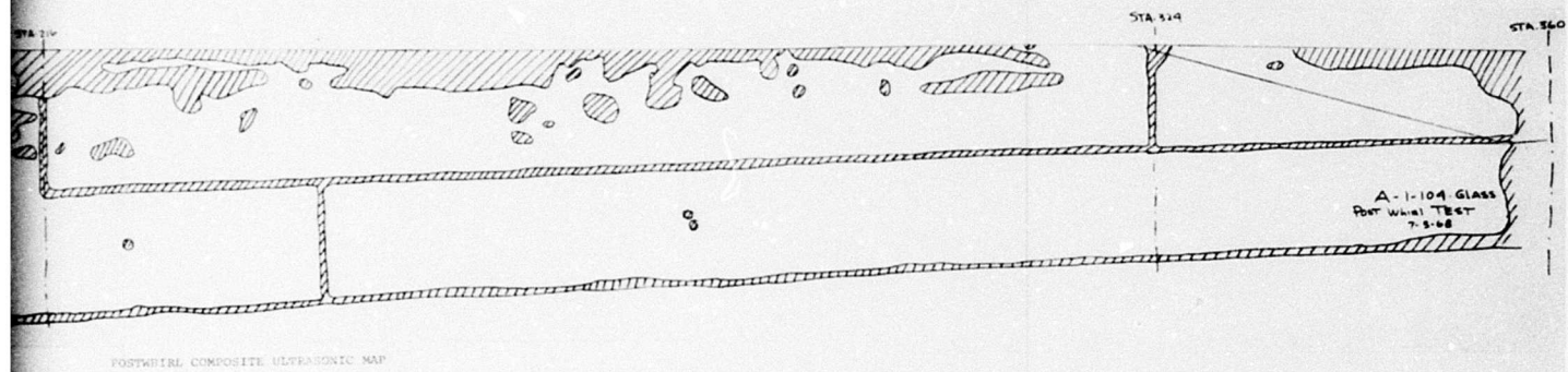
POSTFLIGHT COMPOSITE ULTRASONIC MAP
