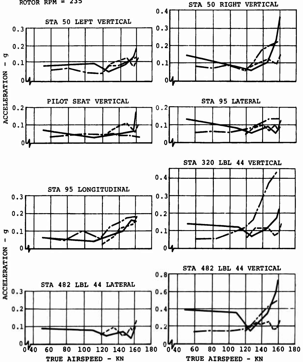
Figure 87. Comparison of 3/Rev Vibration Levels of Fiberglass and Boron Advanced-Geometry Blades and CH-47C Blades at Normal Gross Weight.
