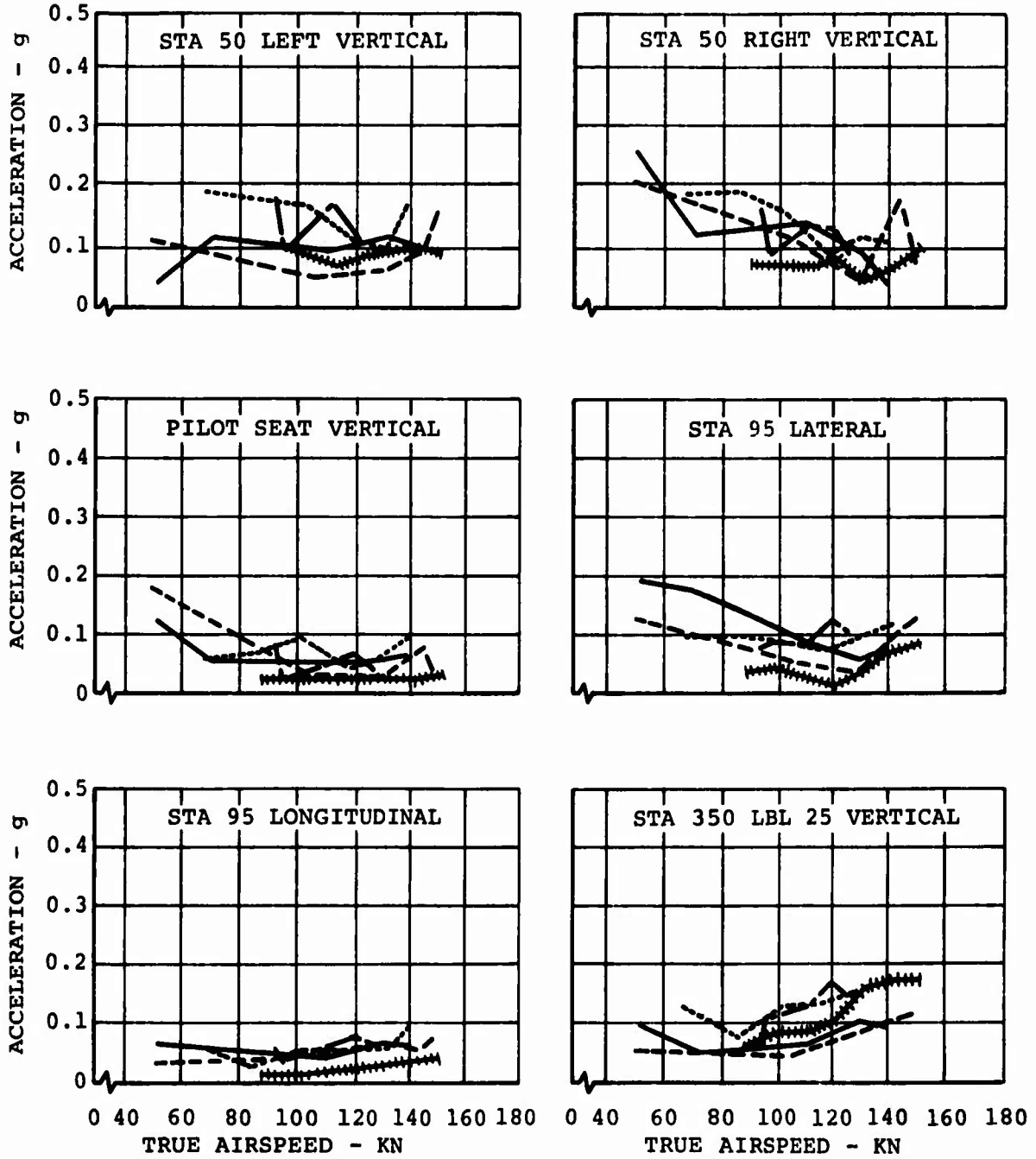
Figure 84. Effect of Altitude on 3/Rev Vibration Levels at Stations 50, 95, and 350 and at Pilot Seat During Flight Test of Boron Blades.
