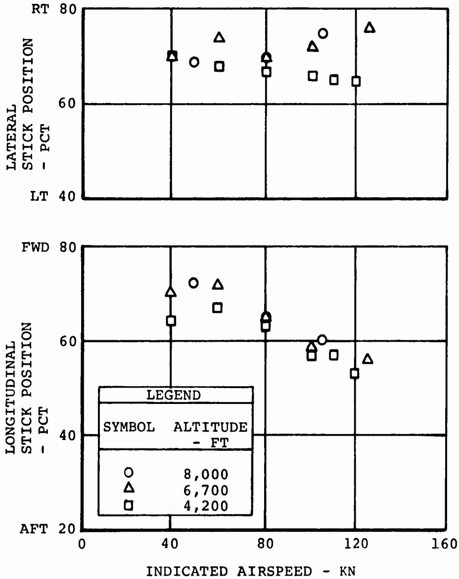
Figure 93. Aircraft Trim Control Positions During Flight Test of the Boron Advanced-Geometry Blades.
