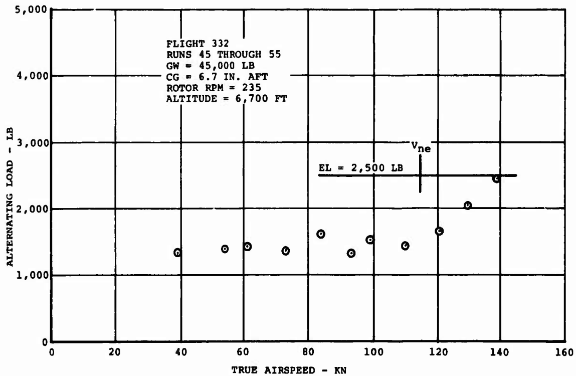
Figure 133. Fixed Link Loads on CH-47C Helicopter Equipped With Boron Advanced-Geometry Blades ( V_{ne} for Glass AGB Shown for Reference).
