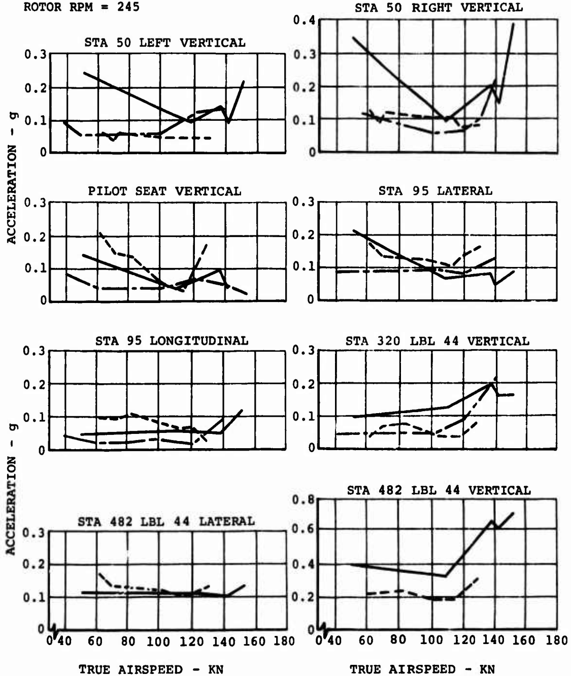
Figure 88. Comparison of 3/Rev Vibration Levels of Fiberglass and Boron Advanced-Geometry Blades and CH-47C Blades at Heavy Gross Weight.
