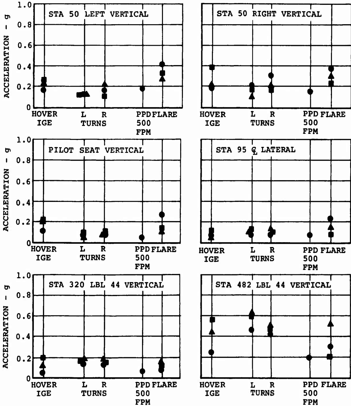
Figure 83. Effect of Gross Weight and Maneuvers on 3/Rev Vibration Levels During Flight Test of Boron Blades.
