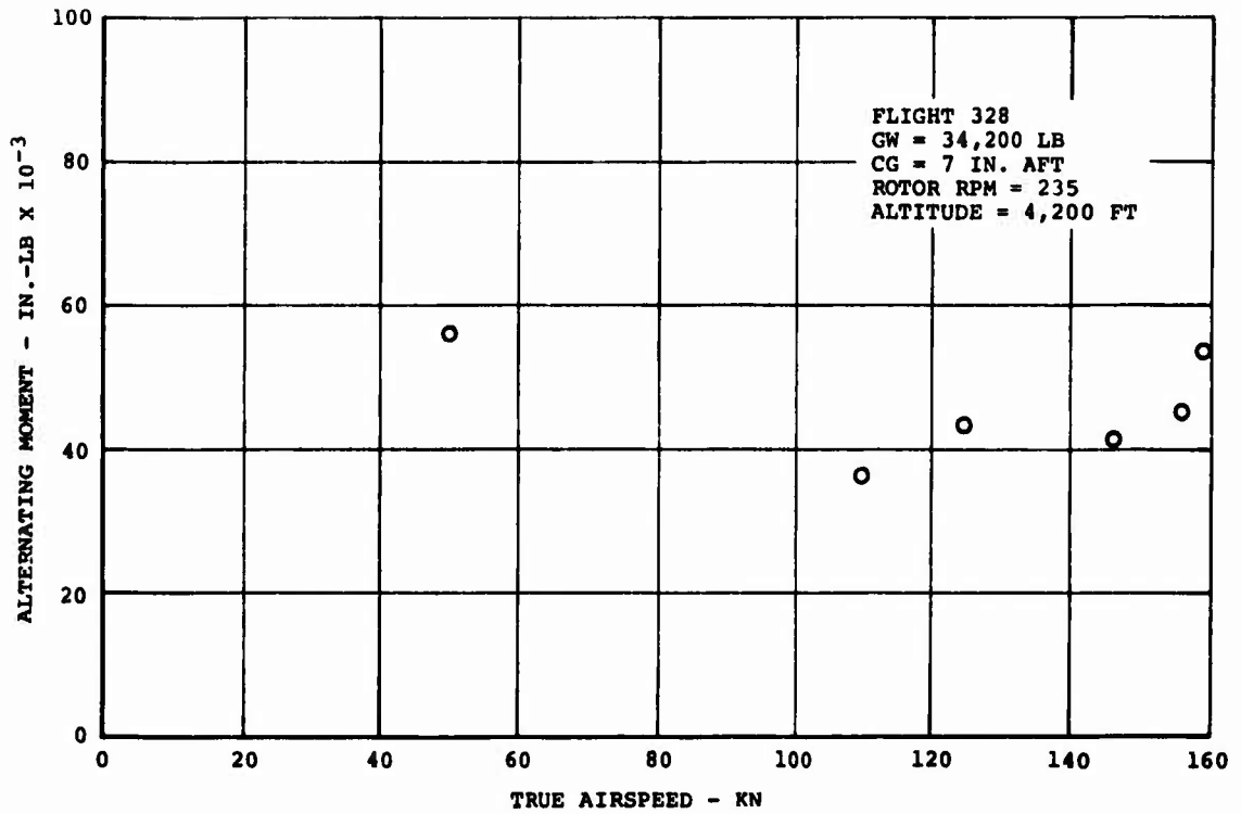
Figure 46. Flapwise Bending of the Blade Socket (Station 49.5).
