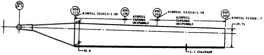
ADVANCED-GEOMETRY BLADE
