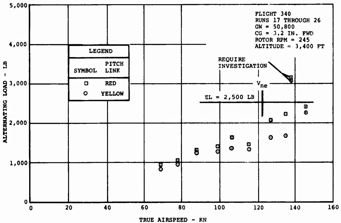
Figure 127. Pitch Link Loads on CH-47C Helicopter Equipped With Boron Advanced-Geometry Blades ( V_{ne} for Glass AGB Shown for Reference).
