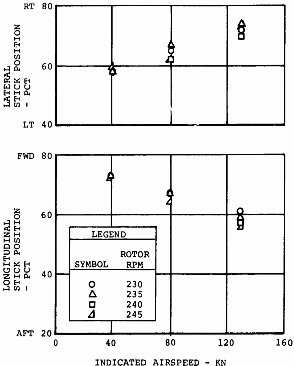
Figure 94. Aircraft Trim Control Positions During Flight Test of the Boron Advanced-Geometry Blades.
