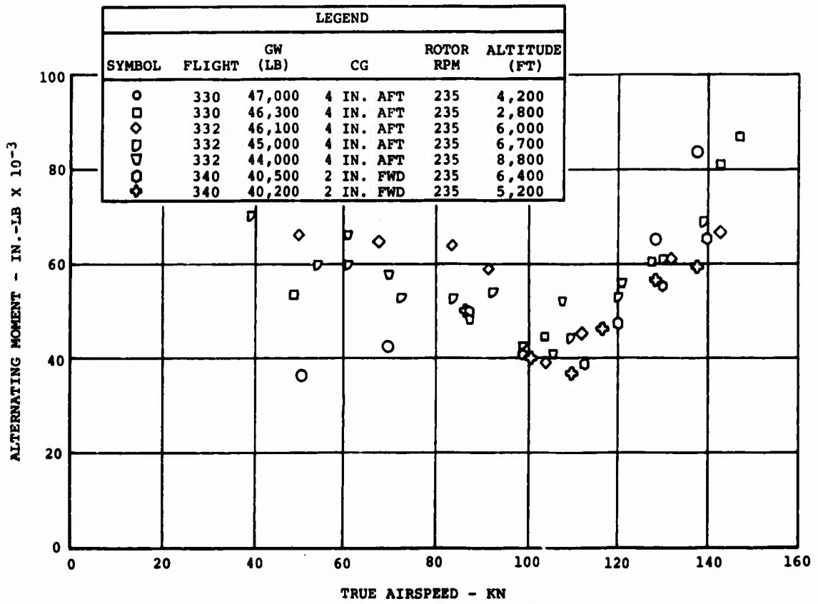
Figure 54. Flapwise Bending of the Blade Spar (Station 252).
