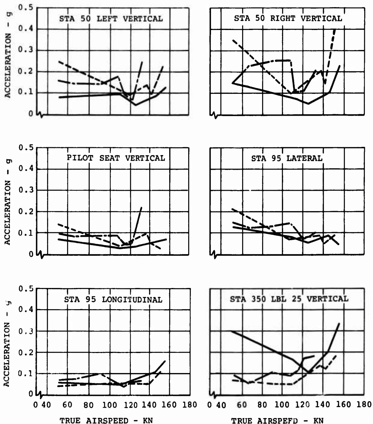
Figure 81. Effect of Gross Weight on 3/Rev Vibration Levels at Stations 50, 95, and 350 and at Pilot Seat During Flight Test of Boron Blades.
