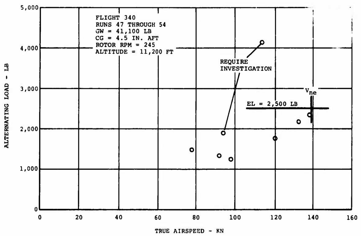
Figure 131. Fixed Link Loads on CH-47C Helicopter Equipped With Boron Advanced-Geometry Blades ( V_{ne} for Glass AGB Shown for Reference).
