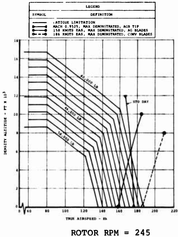
Figure 66. Structural Airspeed Limits of CH-47C Helicopter Equipped With Fiberglass Advanced-Geometry Blades at 235 and 245 Rotor RPM.
