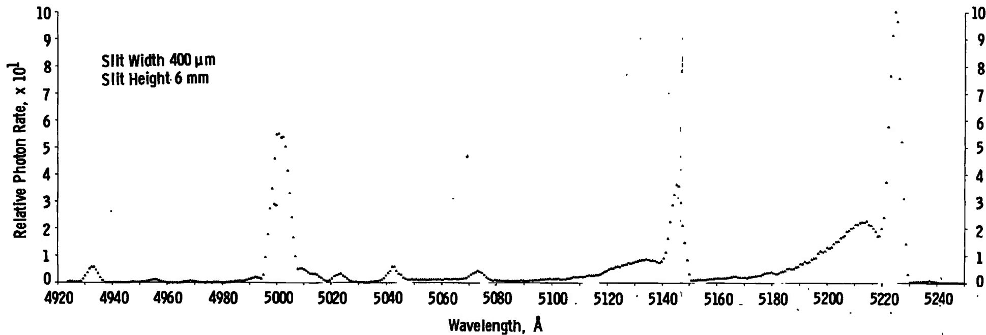
Fig. 22 N 2 (1-) \Delta v = -3 Sequence at 300°K
