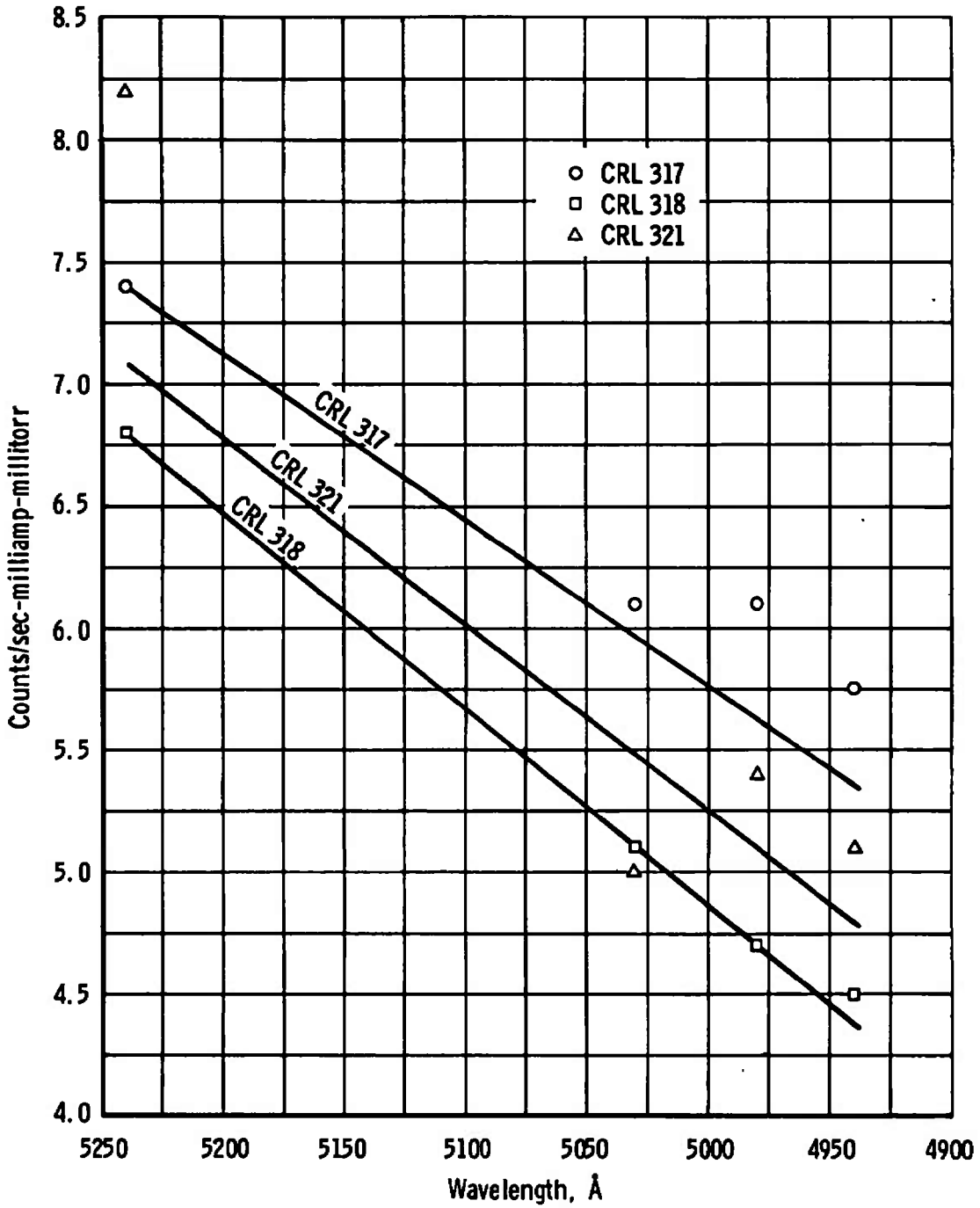
Fig. 26 Lowest Count Rate Points for \Delta v = -3 Sequence at 660^\circ\text{K}
