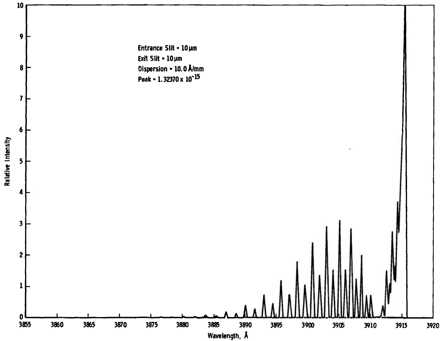
Fig. 20 Computer Plot of N_2^+(1-)(0,0) Band at 300°K
