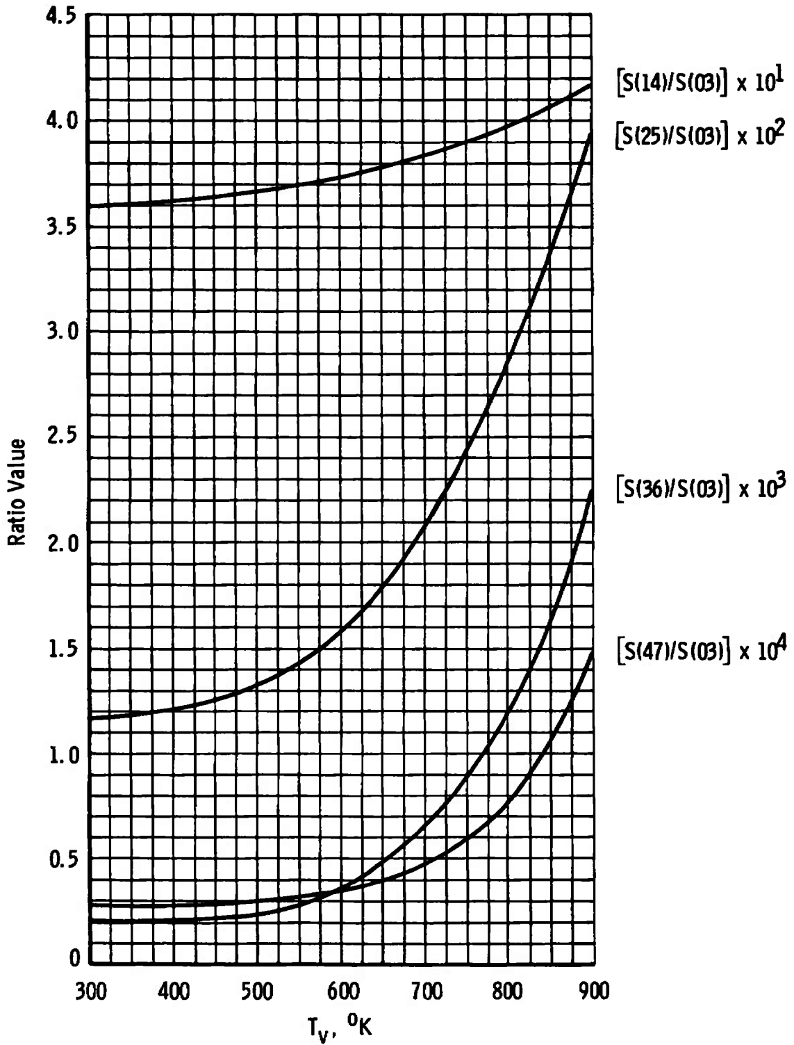
Fig. 2 N_2^+(1-) \Delta v = -3 Sequence Band Intensity Ratios versus Vibrational Temperature
