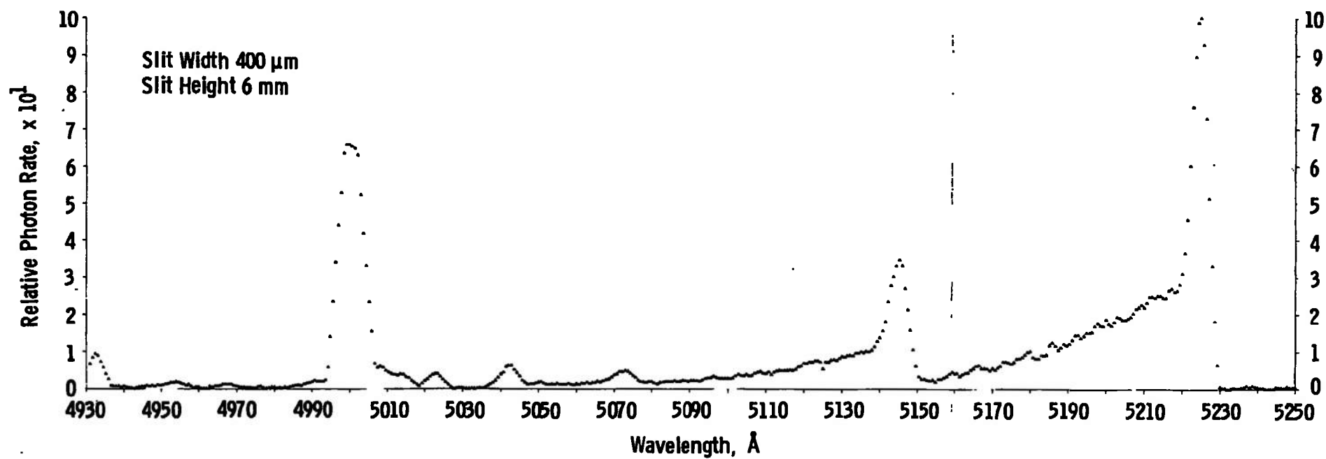
Fig. 23 N 2 (1-) \Delta v = -3 Sequence at 660°K
