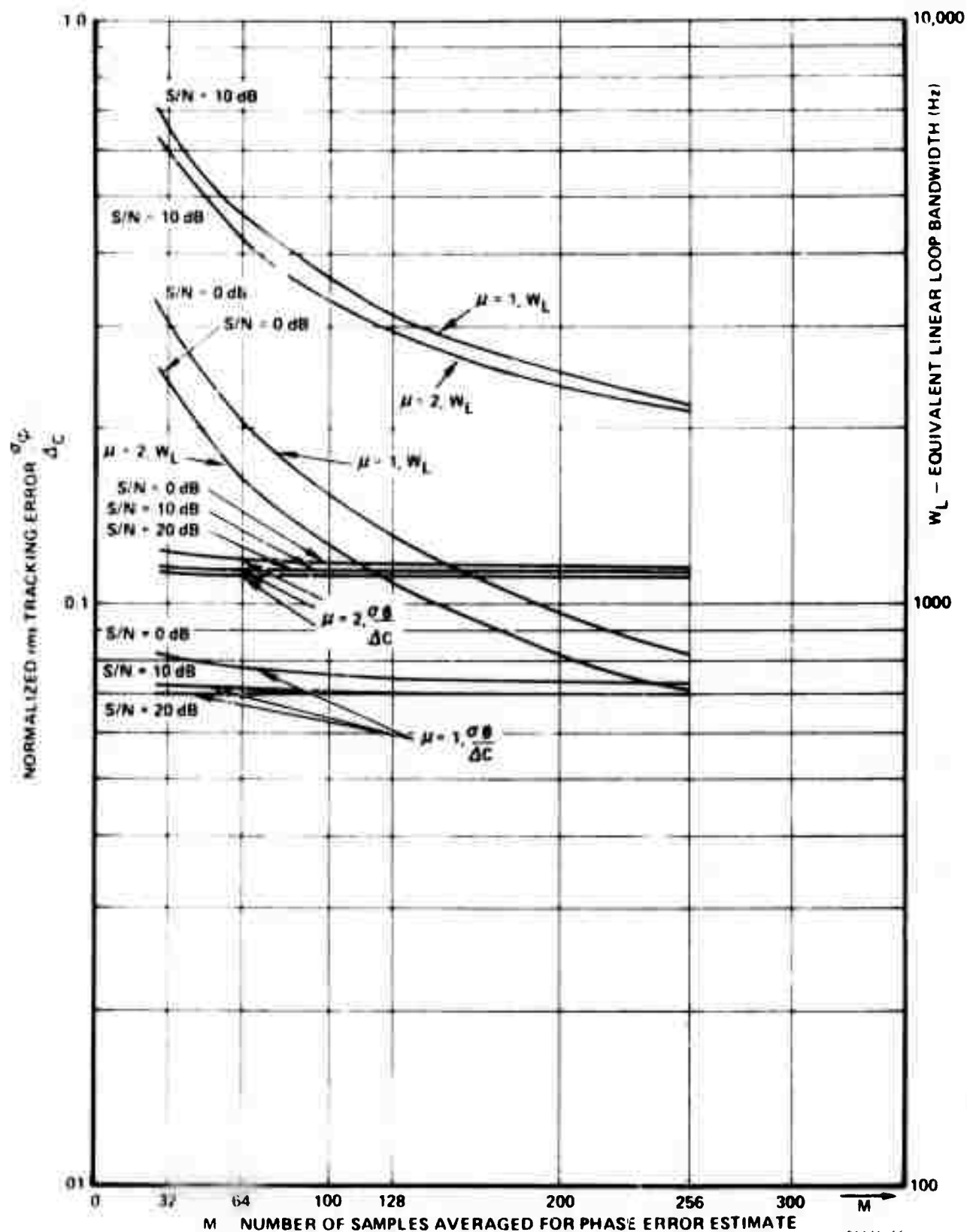
Figure 3.3.2-3. Prediction Phase Error
