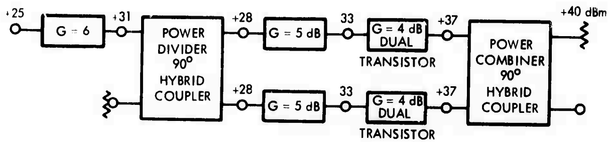
Figure 5.1-3B. Low Power Module for 1975-1980 Time Frame
